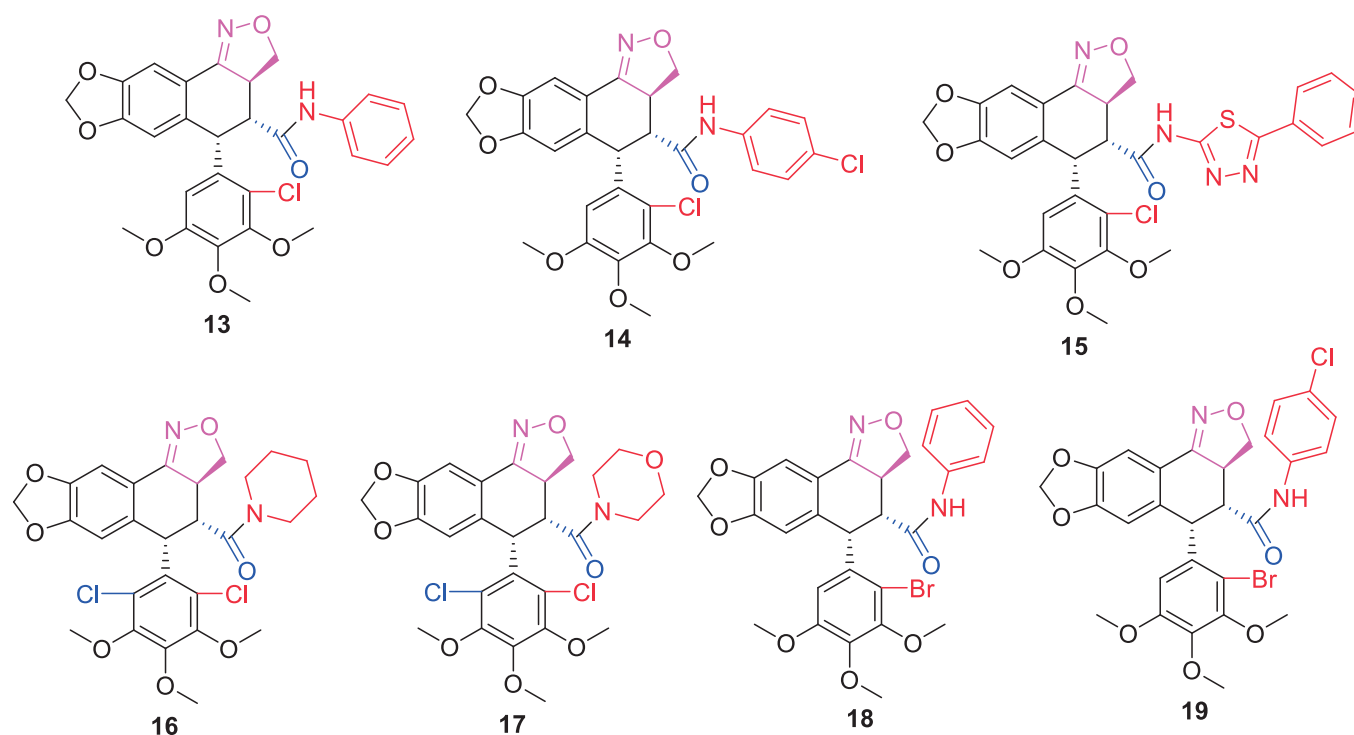
Figure 2. Chemical structures of 2'(2',6')-(di)halogenoisoxazolopodophyllinic acids-based amides ( 13–19 )
