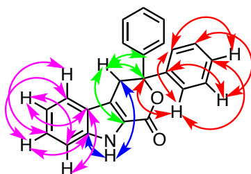
HMBC Study of 5aa
