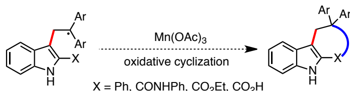
Scheme 3. Reaction of 3-Substituted Indoles Having Another Functionality X at the C-2 Position
