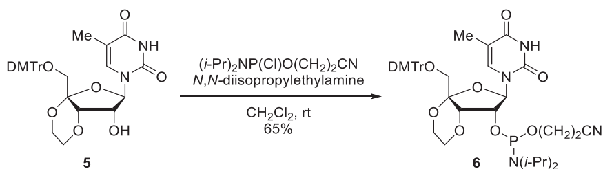
Scheme 1. Synthesis of 3',4'-EoNA-T-phosphoramidite 6
