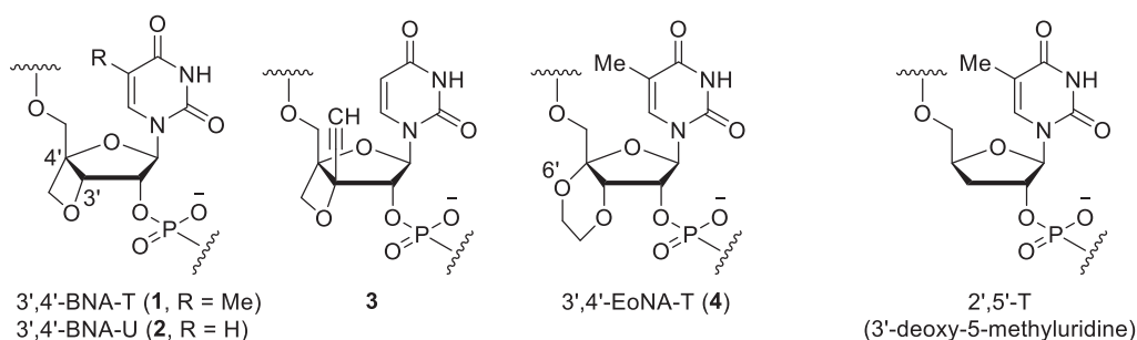
Figure 1. Structures of 3',4'-bridged nucleic acids 1–4
