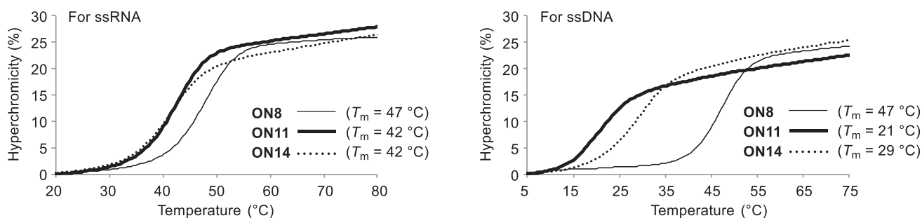
Figure 2. Representative UV-melting curves of duplexes
