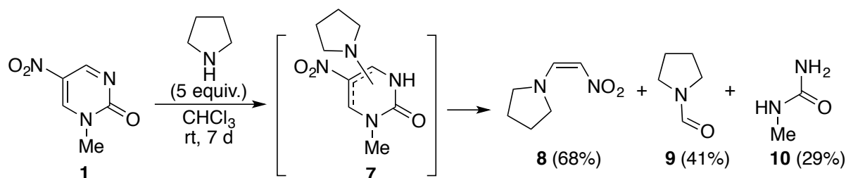
Scheme 4. Ring opening reaction of adduct ( 7 ) leading to nitroenamine ( 8 ), N -formylpyrrolidine ( 9 ) and N -methylurea ( 10 ). Yields were determined based on pyrimidinone ( 1 ).
