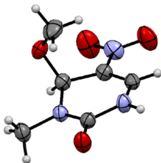
Figure 1. An ORTEP showing the 6-methoxy-1-methyl-5-nitropyrimidine-2(1H)-one ( 6 ) (color labels: gray, carbon; white, hydrogen; violet, nitrogen; red, oxygen). Thermal ellipsoids are drawn at the 50% probability level. Deposition number is CCDC-1813483.
