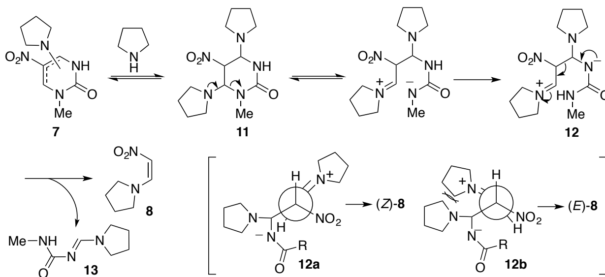
Scheme 5. A plausible mechanism for the formation of nitroenamine ( 8 )
