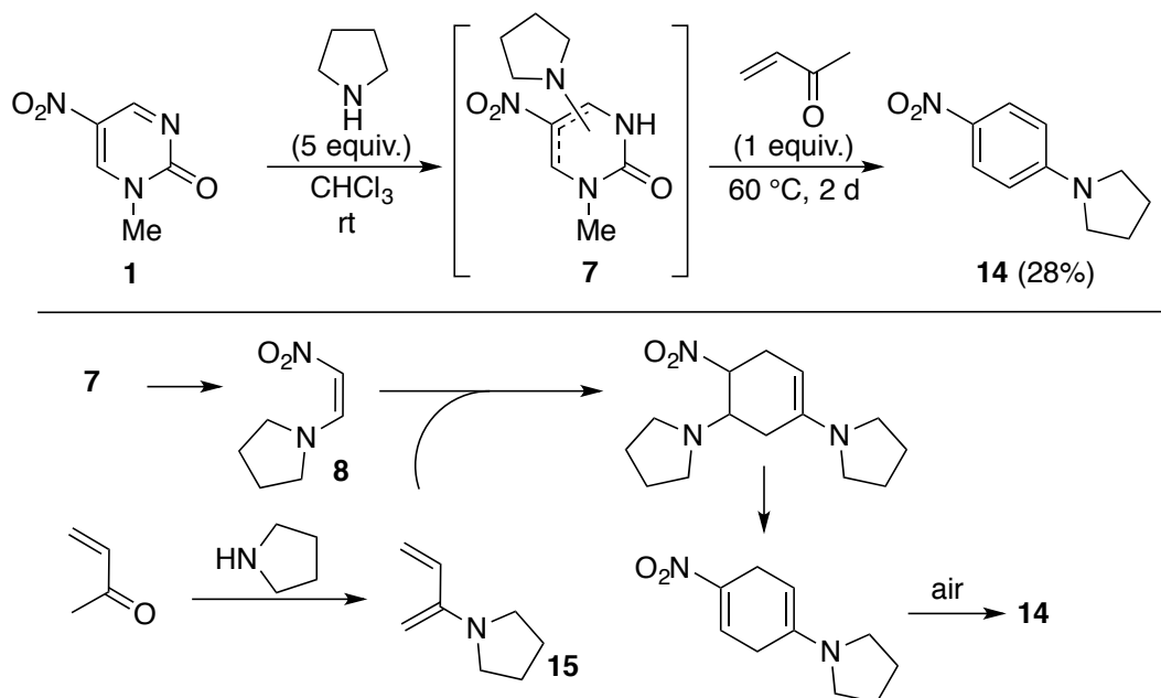
Scheme 6. Cycloaddition of nitroenamine ( 8 ) and dienamine ( 15 ) leading to nitroaniline ( 14 )
