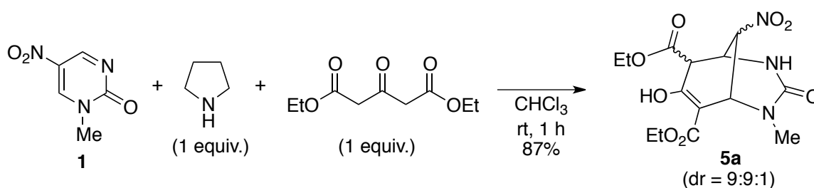
Scheme 3. Synthesis of diazabicyclic compound ( 5a ) under mild conditions
