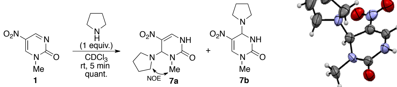
Scheme 2. Addition of pyrrolidine to nitropyrimidinone ( 1 ) and an ORTEP showing the 1-methyl-5-nitro-6-pyrrolidinopyrimidin-2(1H)-one ( 7a ) (color labels: gray, carbon; white, hydrogen; violet, nitrogen; red, oxygen). Thermal ellipsoids are drawn at the 50% probability level. Deposition number is CCDC-1813484.
