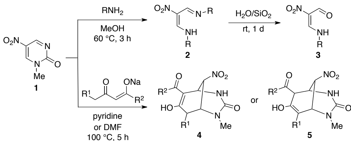
Scheme 1. Chemical conversions of nitropyrimidinone ( 1 )
