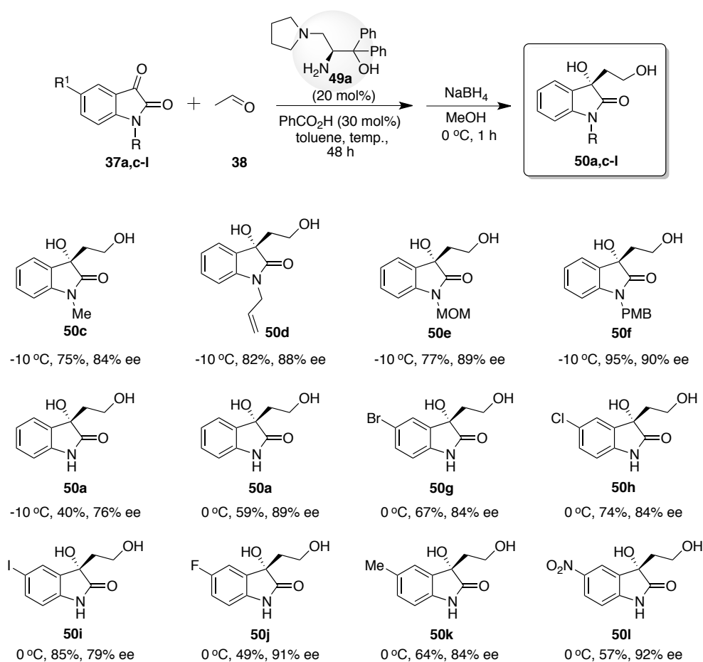
Scheme 15. Substrate scope of crossed-aldol reaction
