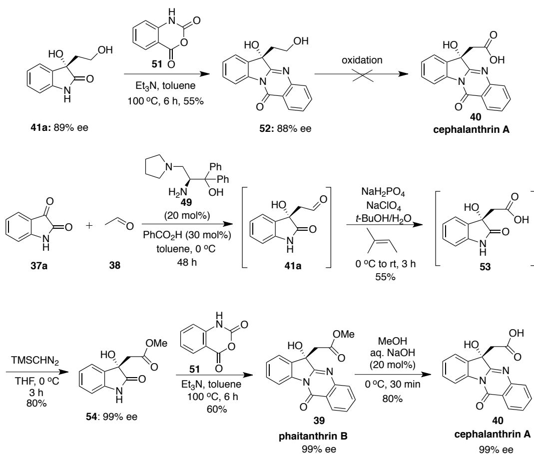
Scheme 16. Total synthesis of phaitanthrin B and cephalanthrin A
