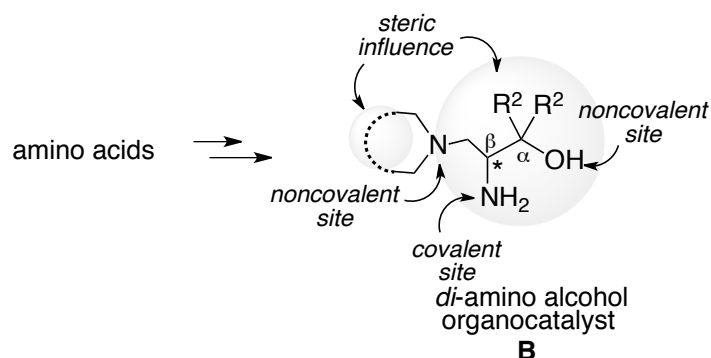
Scheme 12. Functionality of fk -amino alcohol organocatalysts
