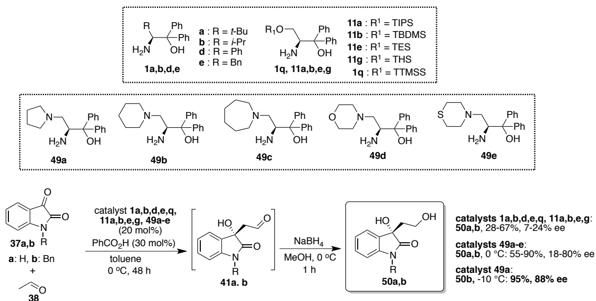
Scheme 14. Aldol reaction using γ -amino alcohol organocatalysts
