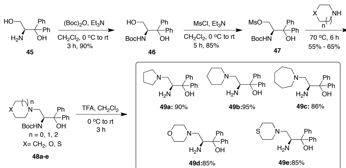
Scheme 13. Preparations of new fk -amino alcohol organocatalysts
