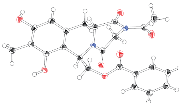
Figure 3. X-Ray structure of compound cis-32
