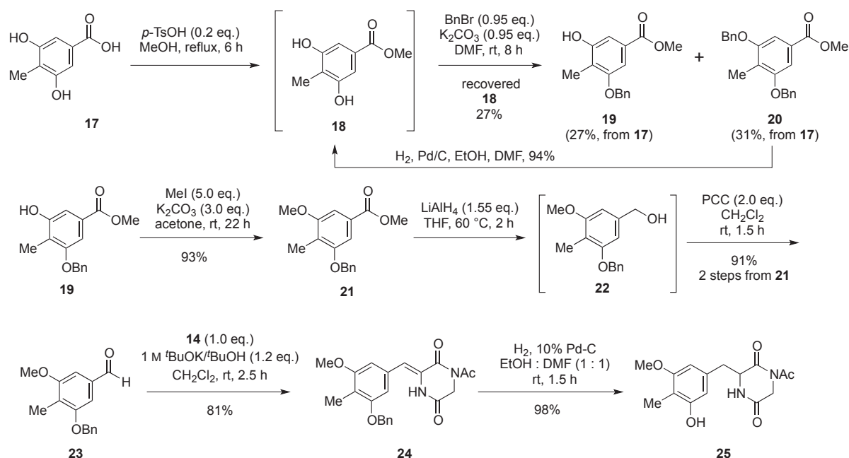
Scheme 3. 7 Steps transformation of 17 into 25
