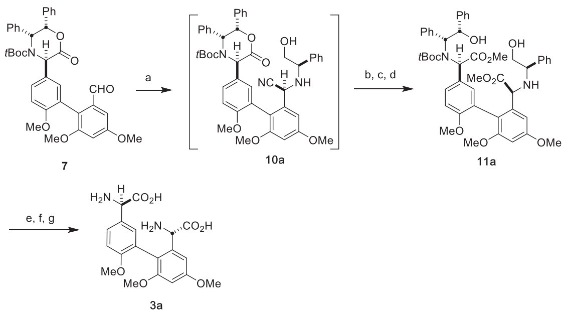
Scheme 2. Synthesis of actinoidic acid trimethyl ether ( 3 ) from 7
