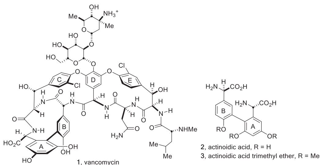
Figure 1. Structures of vancomycin ( 1 ) and actinoidic acid ( 2 ) and actinoidic acid trimethyl ether ( 3 )
