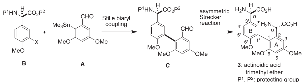
Scheme 1. Synthetic strategies for actinoidic acid trimethyl ether ( 3 )
