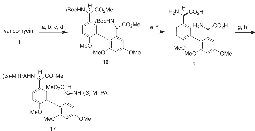
Scheme 4. Isolation of actinoidic acid trimethyl ether ( 3 ) from vancomycin ( 1 )
