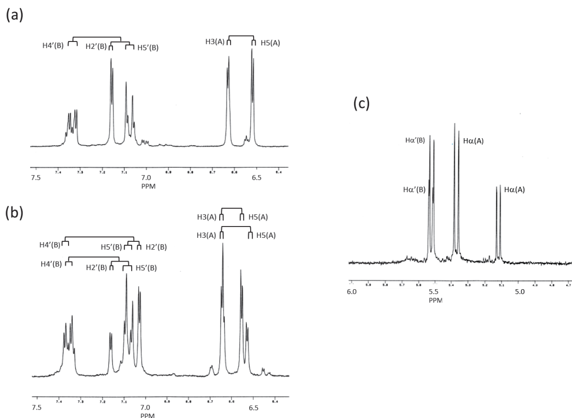
Figure 2. 1 H-NMR signals of actinoidic acid trimethyl ether ( 3 ) and its derivative ( 17 )
