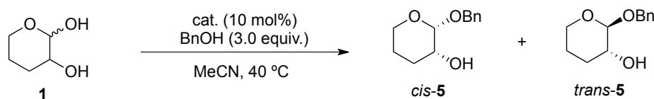
(a) Screening of electron-deficient arylboronic acids
