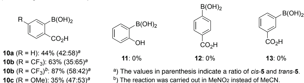
Scheme 4. Screening of arylboronic acids for the acetalization of 1 and BnOH
