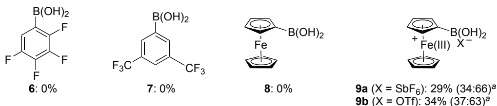
(b) Screening of bifunctional arylboronic acids
