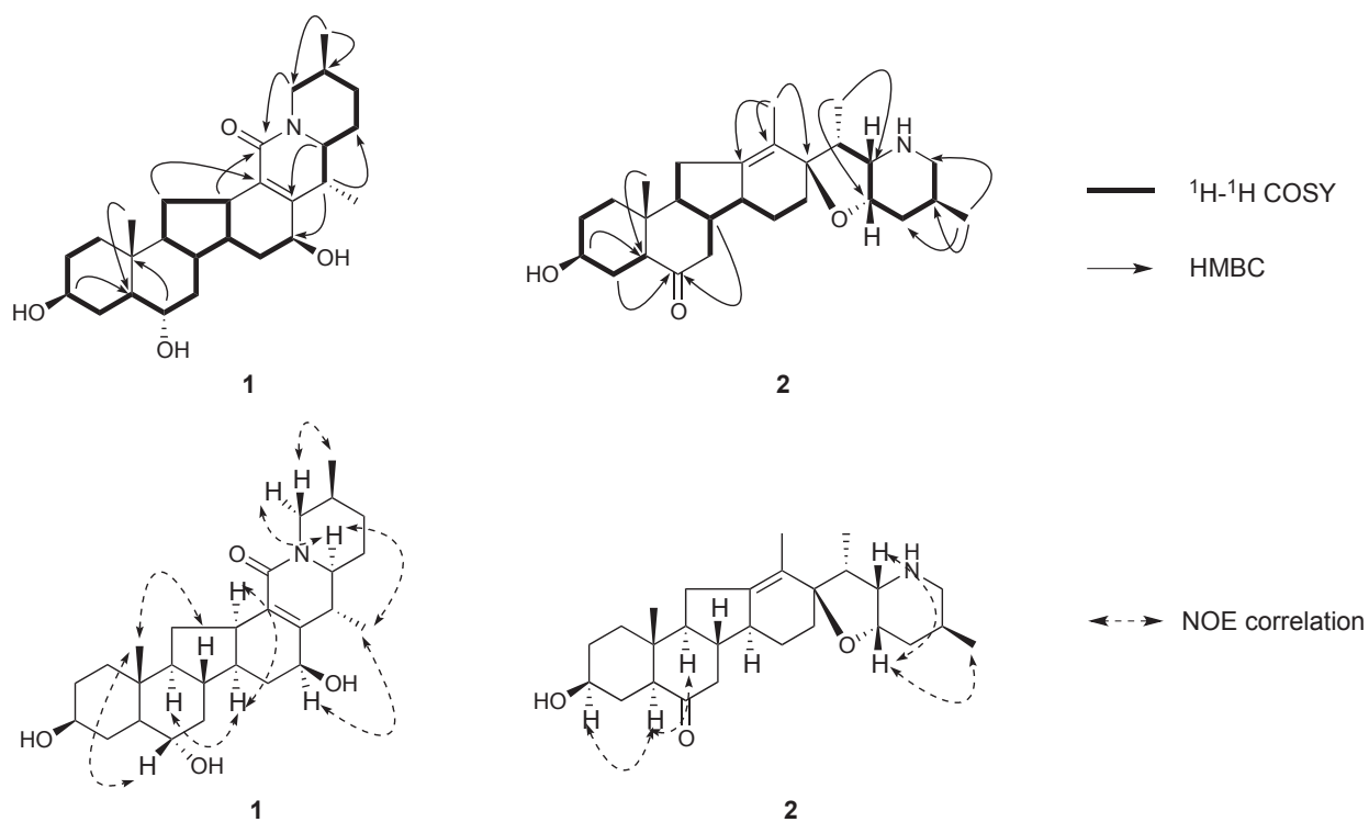
Figure 2. Key 1 H- 1 H COSY, HMBC, and NOESY correlations of 1 and 2
