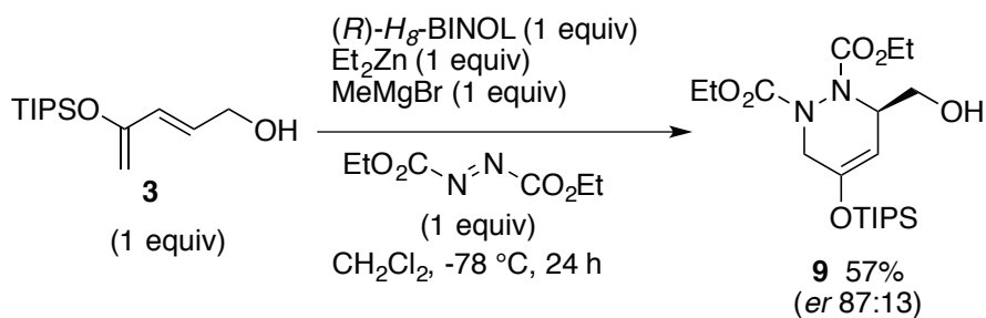
Scheme 3. Formation of dihydropyridazine by the Lewis acid template-mediated hetero-Diels-Alder reaction
