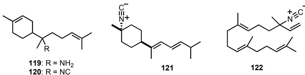
Figure 9. Structures of (±)-Aminobisabolenes, Theonelline Isocyanide and (±)-Geranylinaloisocyanide
