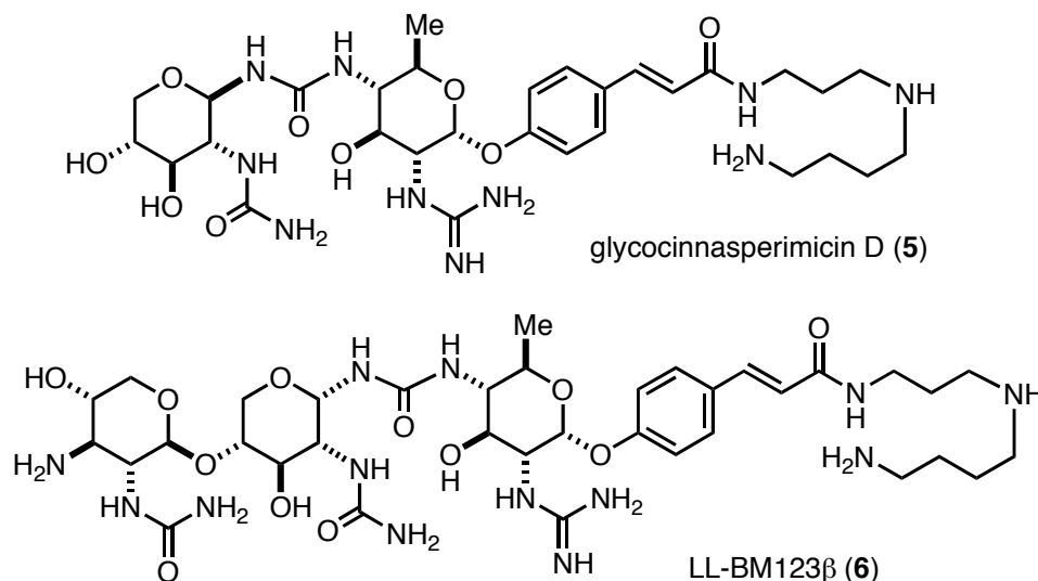
Figure 2. Glycocinnamoylspermidine Antibiotics
