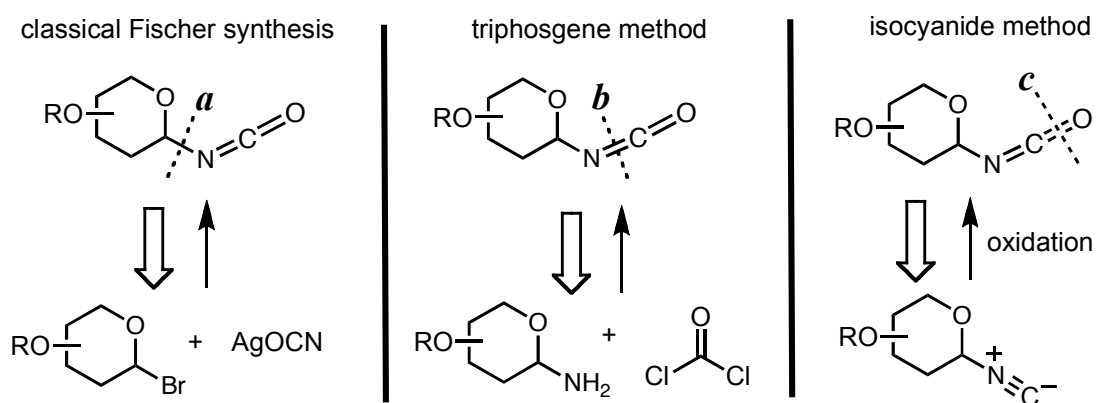
Figure 3. Retrosynthetic Analysis of Glycopyranosyl Isocyanate
