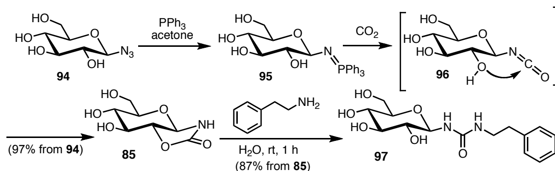
Scheme 33. Urea Glucosylation of Steyermark's Glucopyranosyl Oxazolidinone in Water
