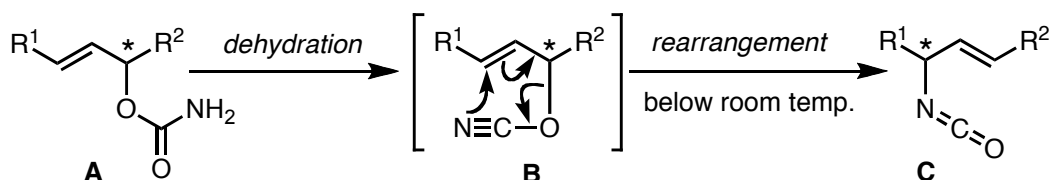
Scheme 39. Ichikawa Rearrangement 68
