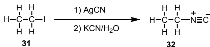
Scheme 7. Synthesis of Ethyl Isocyanide by the Procedure of Gautier
