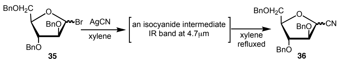
Scheme 9. Reaction of Arabinofuranosyl Bromide with Silver Cyanide
