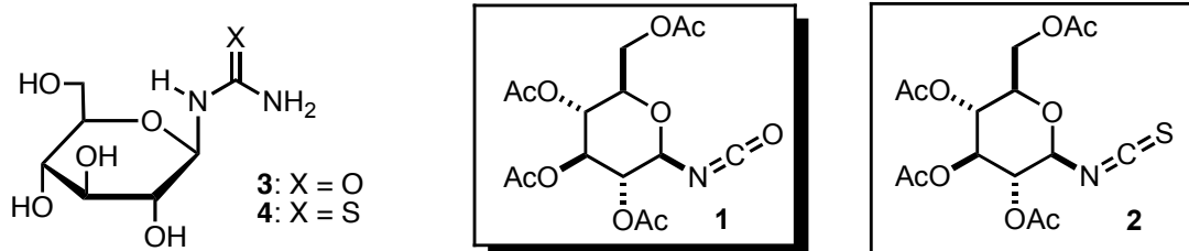
Figure 1. \beta -Pyranosyl Structures of Glucosyl Urea, Thiourea, Isocyanate and Isothiocyanate
