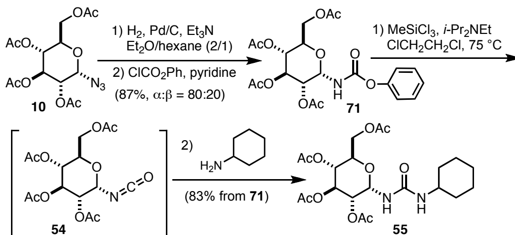
Scheme 26. Carbamate Method for the Synthesis of \alpha -Glucopyranosyl Isocyanate and Urea
