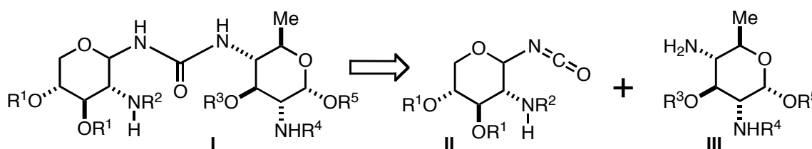
Scheme 2. Retrosynthetic Analysis of Urea Glycosyl Bond
