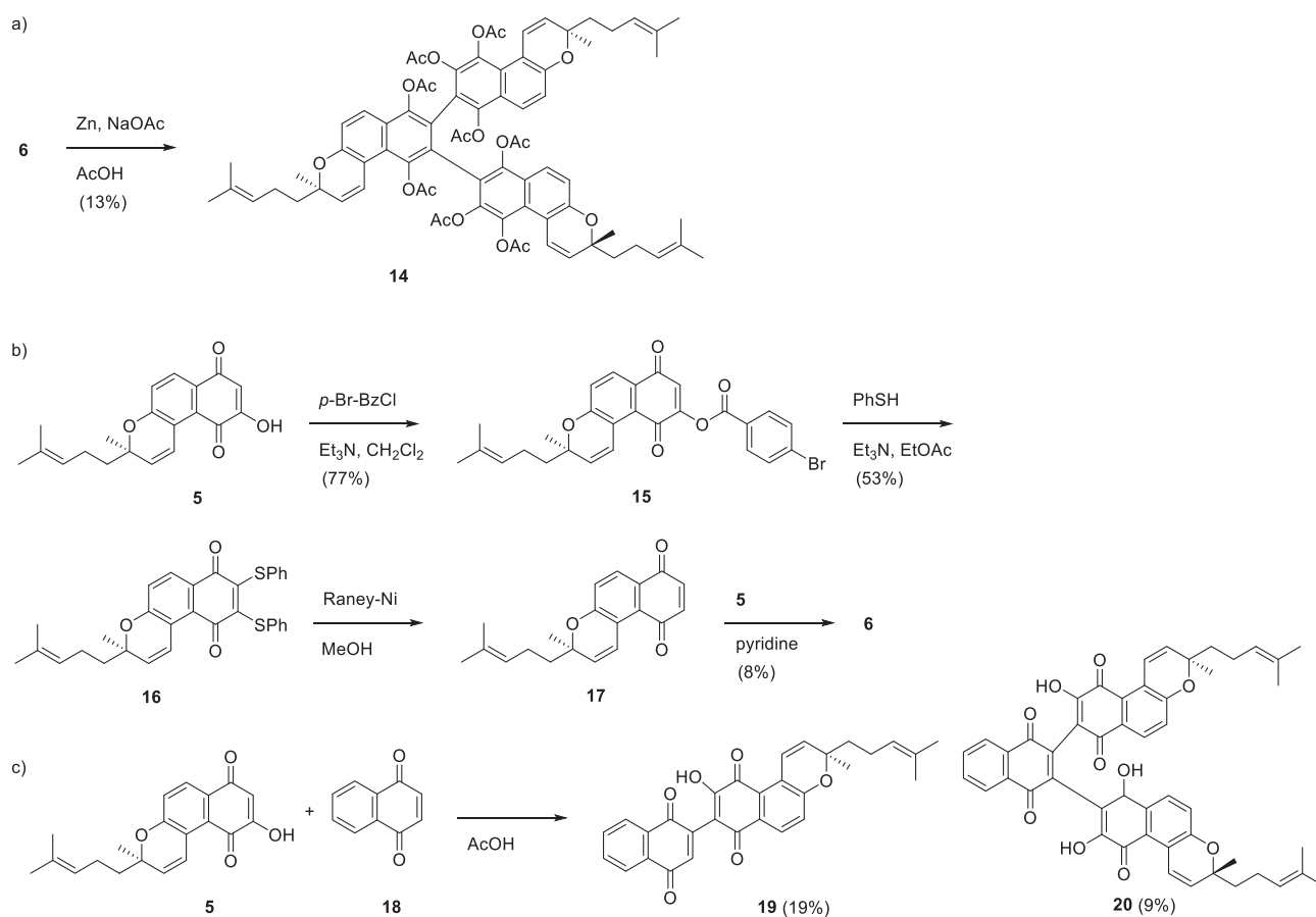
Scheme 1. Derivatization of conoquone (6) and teretifolione B (5)
