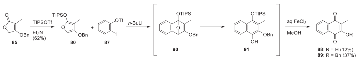
Scheme 11. Synthesis of naphthoquinones 88 and 89 via DAR of iodophenyl triflate 87 and furan 88
