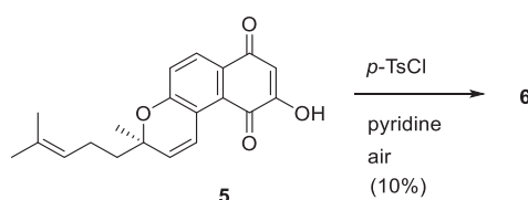
Scheme 2. Direct semisynthesis of conoquone (6) from teretifolione B (5)
