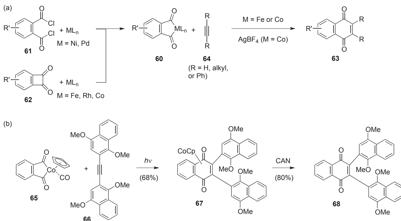
Scheme 8. Synthesis of monomeric 63 and trimeric naphthoquinones 68
