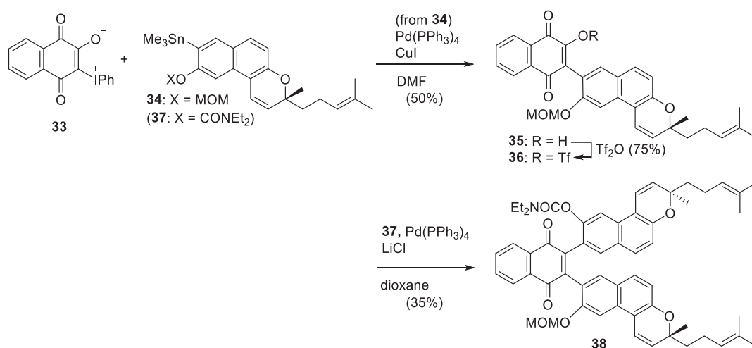
Scheme 4. Synthesis of 2,3-bis(naphthyl)naphthoquinone 38 by double Stille coupling
