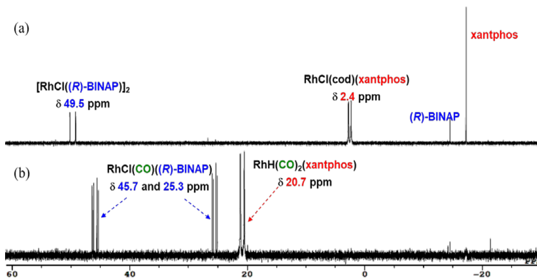
Figure 1. 31 P NMR spectra of (a) a mixture of [RhCl(cod)] 2 , (R)-BINAP, and xantphos (molar ratio 1/0.6/1.8) in toluene- d 8 solution and (b) the addition of excess formaldehyde into the reaction mixture (a)
