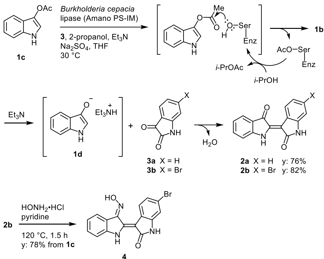
Scheme 3. Lipase-mediated synthesis of indirubins 2a and 2b and derivatization to 4
