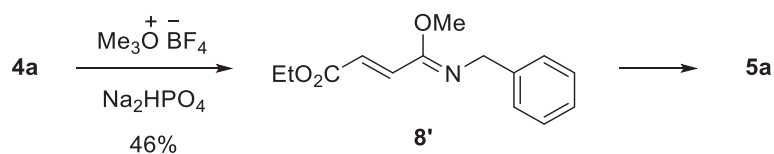
Scheme 5. Experiment to elucidate the reaction mechanism
