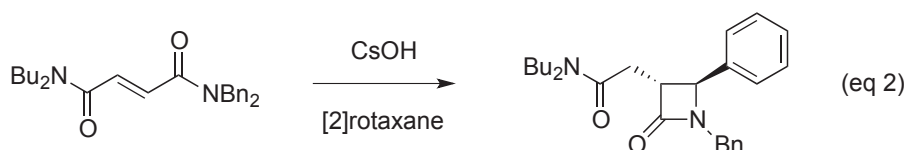
Scheme 2. \beta -Lactam synthesis through anionic 4-exo-trig cyclization
