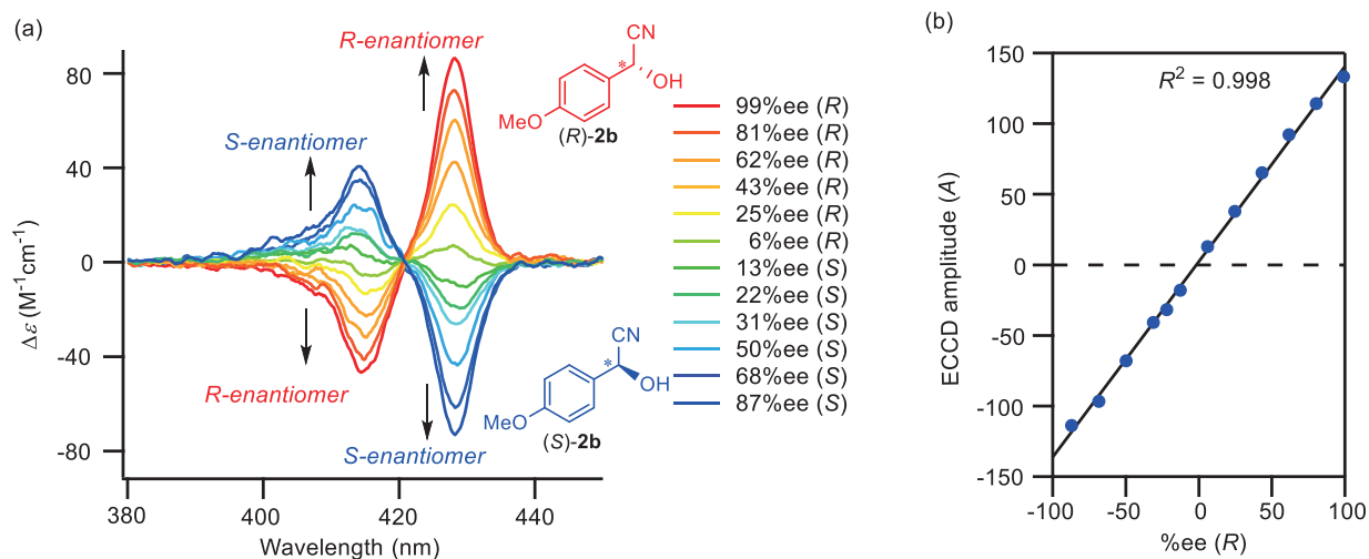
Figure 10. (a) ECCD spectra of BP1 ( 1.5 \times 10^{-6} M) complexed with 2b (10 equiv) at different enantiomeric excesses (ECCD spectra were recorded in 5% \text{CH}_2\text{Cl}_2/n -hexane at 0 °C). (b) Plot of ECCD amplitude ( A = \Delta\varepsilon_{(428 \text{ nm})} - \Delta\varepsilon_{(416 \text{ nm})} ) versus % ee of ( R )- 2b in complex with BP1 .
