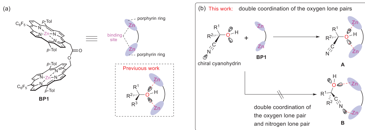
Figure 2. (a) Binding of monoalcohol with BP1 (b) Possible binding modes of cyanohydrin with BP1
