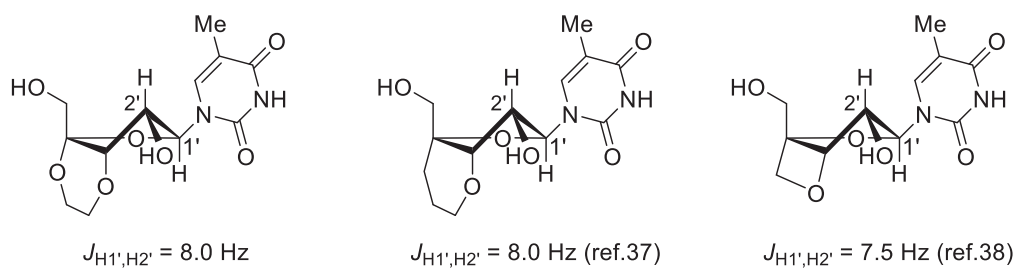
Figure 8. The J_{\text{H}1',\text{H}2'} values of 3',4'-bridged nucleosides
