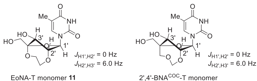
Figure 4. The J_{H1',H2'} values of EoNA-T and 2',4'-BNA COC -T monomers
