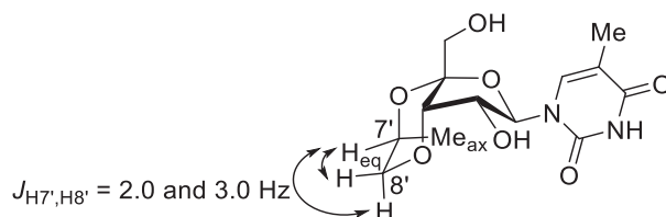
Figure 9. The bridge conformation of ( S )-Me-3',4'-EoNA-T monomer 23b
