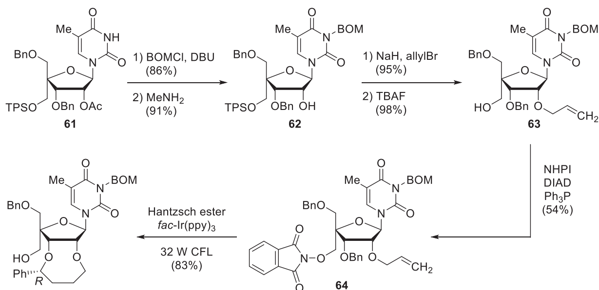
Scheme 12. Synthesis of intermediate 64 and the radical reaction
