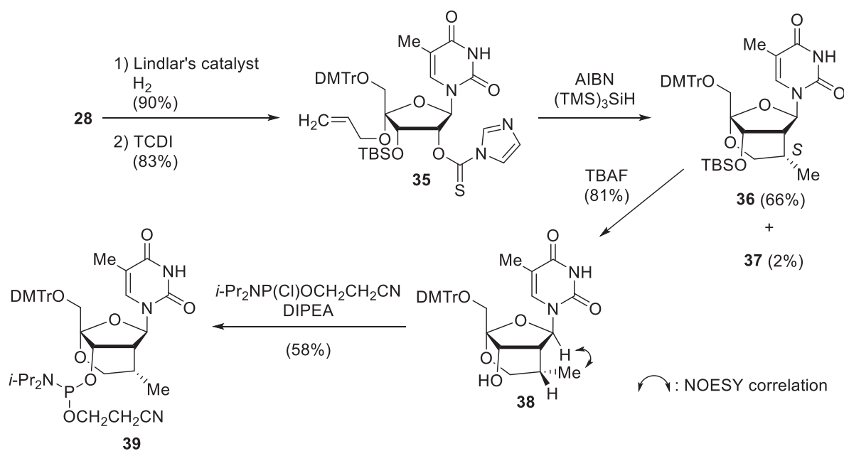
Scheme 8. Synthesis of ( S )-Me-methylene-EoDNA-T phosphoramidite 39
