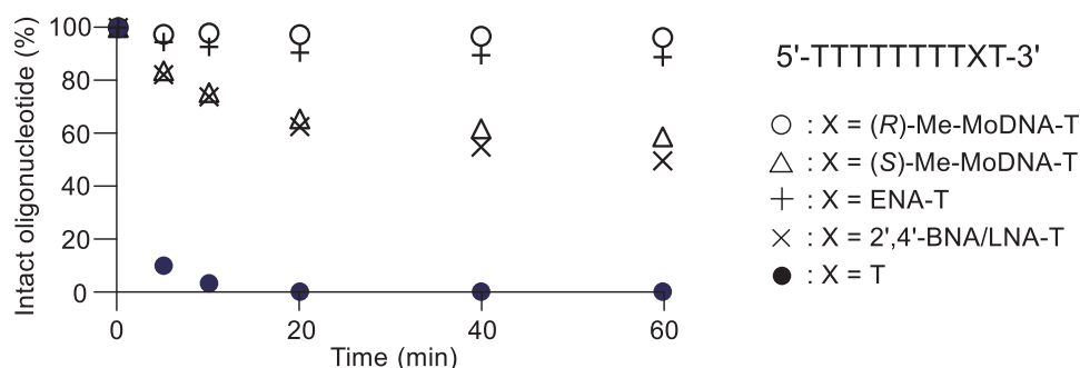
Figure 17. Degradation experiments by 3'-exonuclease. Conditions: 0.05 unit/mL Crotalus adamanteus venom phosphodiesterase, 50 mM Tris-HCl (pH 8.0), 10 mM MgCl 2 , and 7.5 μM of oligonucleotide at 37 °C.
