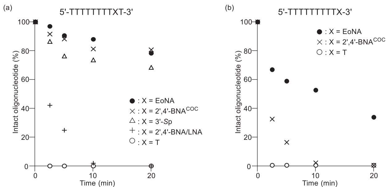
Figure 5. Degradation experiments by 3'-exonuclease. Conditions: 4 \mu\text{g/mL} Crotalus admanteus venom phosphodiesterase, 50 mM Tris-HCl (pH 8.0), 10 mM \text{MgCl}_2 , and 7.5 \mu\text{M} of oligonucleotide at 37 ^\circ\text{C} .
