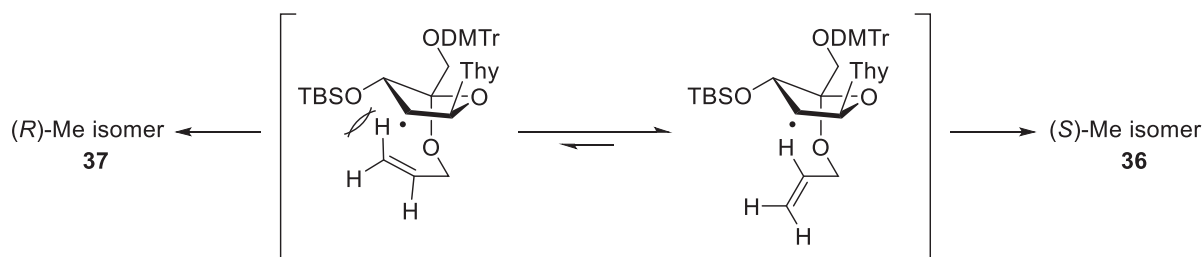
Figure 12. Stereoselectivity of intramolecular radical cyclization
