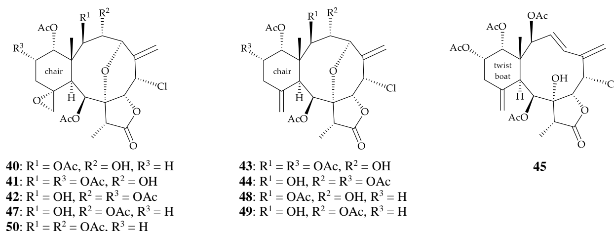
Figure 3. Structures of fragilolides B–Q (24–39), 3-deacetylpraelolide (40), 13 \alpha -acetoxy-3-deacetylpraelolide (41), 13 \alpha -acetoxy-2-deacetylpraelolide (42), 13 \alpha -acetoxy-3-deacetyljunceellin (43), and frajunolide N (46), fragilide J (47), 3-deacetyljunceellin (48), 2-deacetyljunceellin (49), and praelolide (50)
