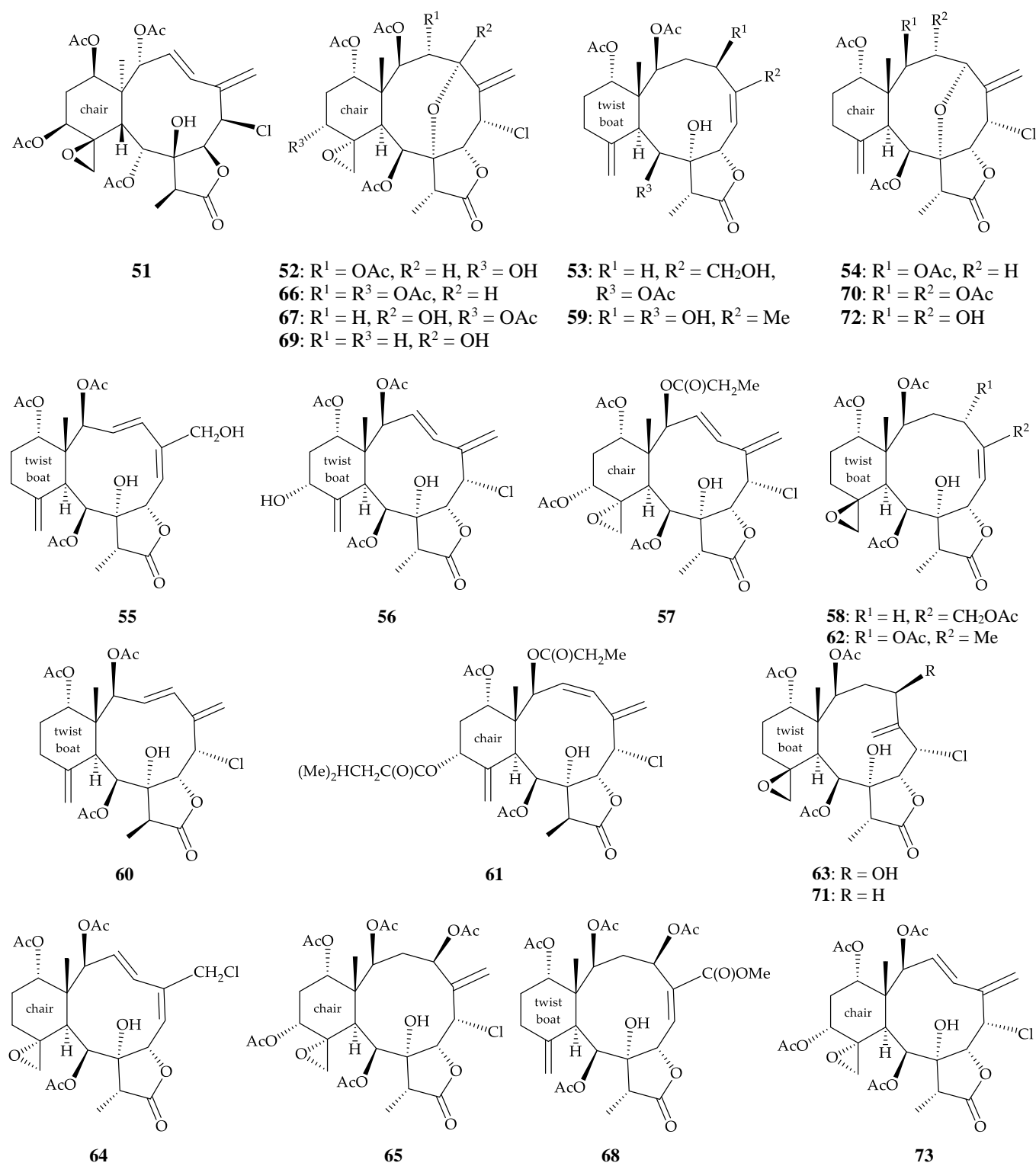
Figure 4. Structures of (+)-12- epi -fragilide G ( 51 ), fragilides K–W ( 52–64 ), gemmacolides V ( 65 ) and X ( 66 ), juncins P ( 67 ), Z ( 68 ), and ZI ( 69 ), junceellin ( 70 ), robustolide F ( 71 ), junceellonoid D ( 72 ), and (–)-12- epi -fragilide G ( 73 )
