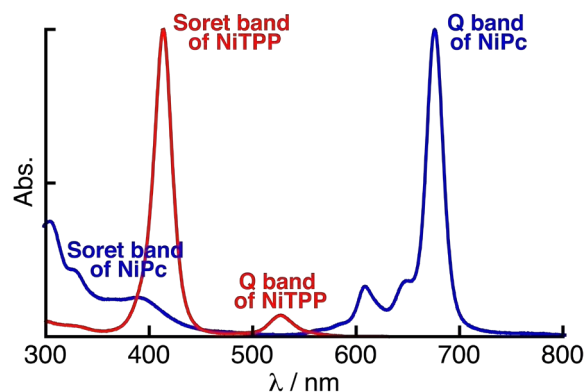
Figure 3. UV/vis absorption spectra of porphyrin and Pc (nickel complexes of meso -tetraphenyl-substituted porphyrin (NiTPP) (red)) and tetra- tert -butyl-substituted phthalocyanine (NiPc) (blue)) in \text{CHCl}_3
