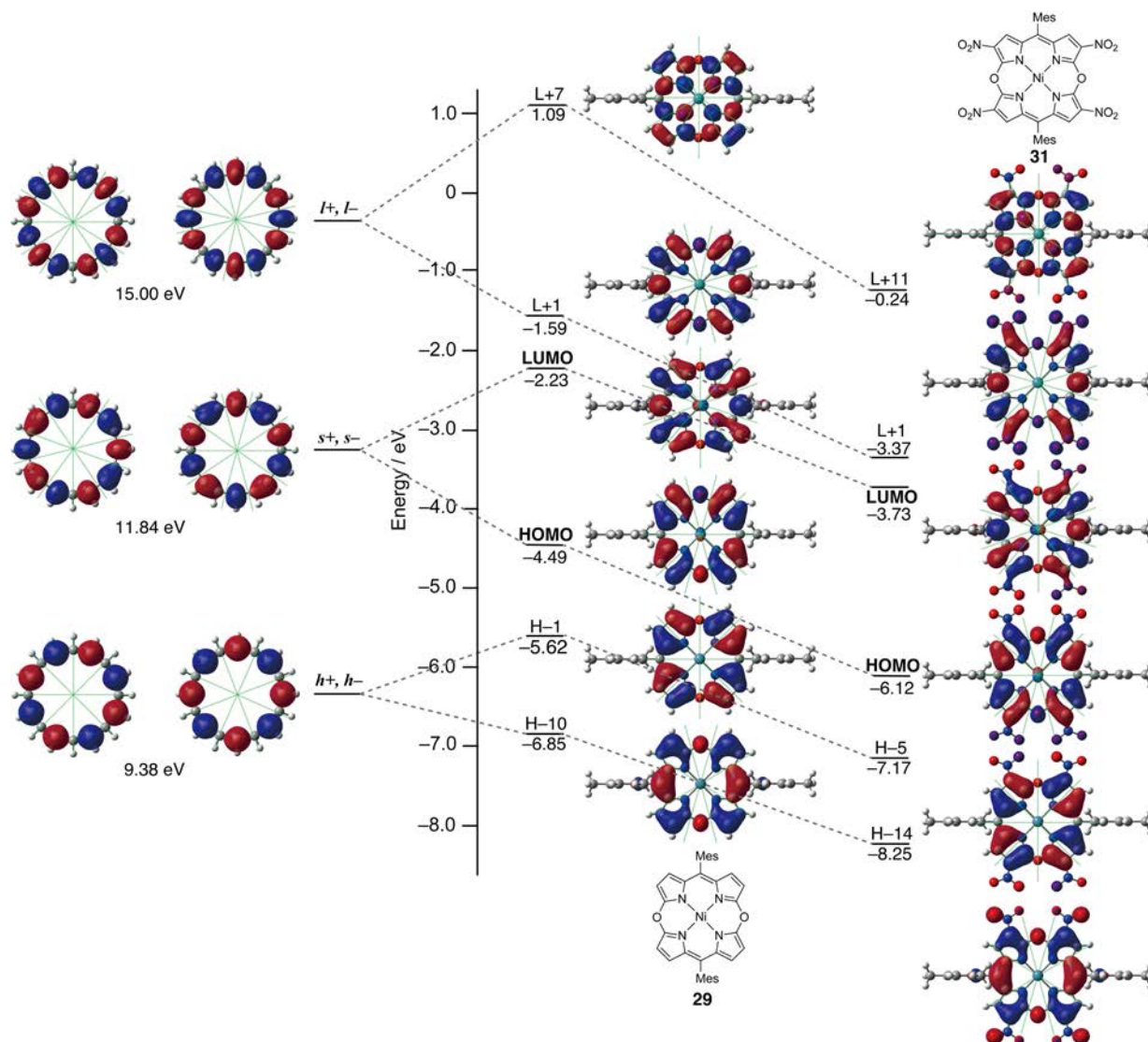
Figure 22. Frontier MO diagrams of 29 , 31 , and 20\pi -electron [16]annulene ( C_{16}H_{16}^{4-} ) perimeter at the B3LYP/6-31G(d) level. Nodal planes are drawn with pale green lines. Redrawn from ref. 68.
