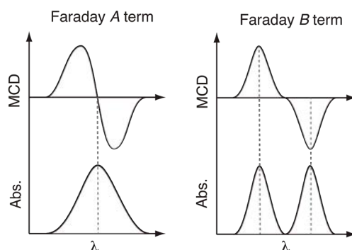
Figure 5. MCD Faraday A and B terms
