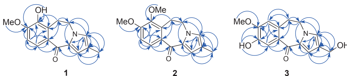
Figure 2. Key HMBC( \curvearrowright ) correlations of compounds 1-3
