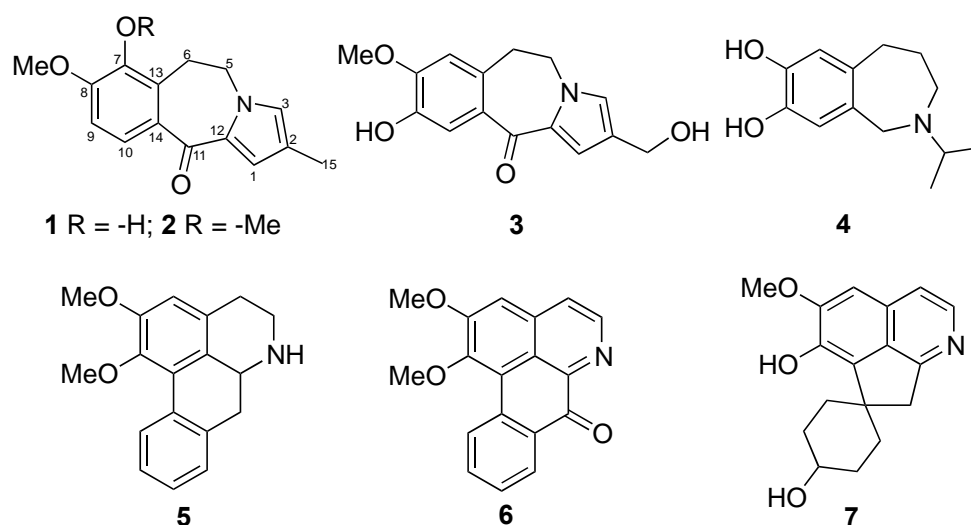
Figure 1. The alkalids from T.cultratum
