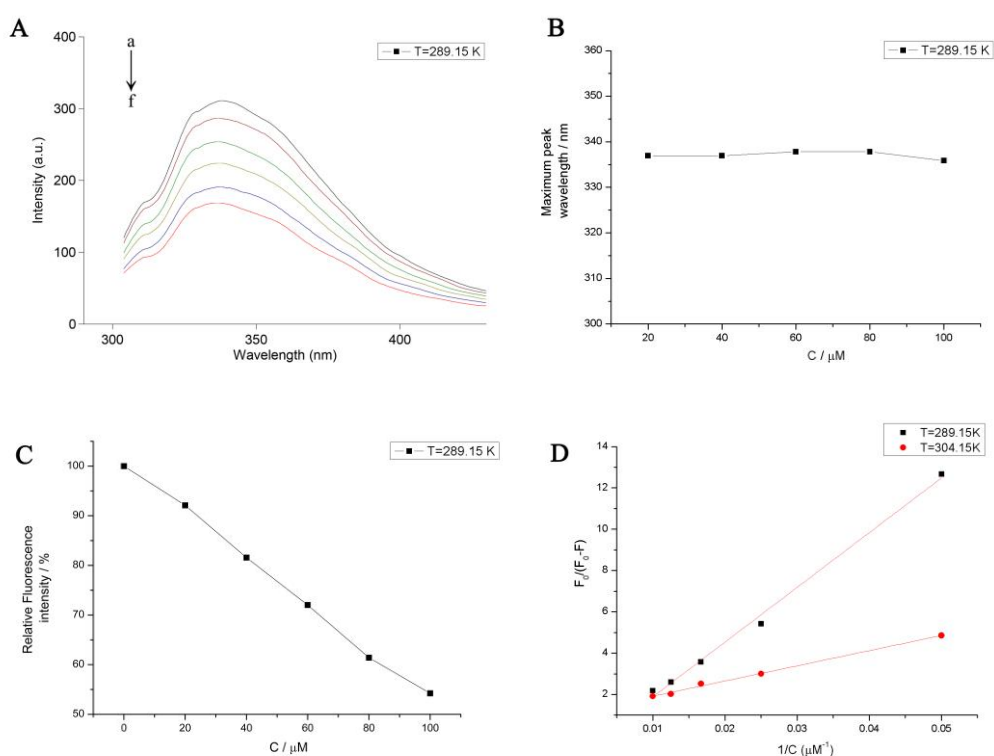
Figure 3. (A) Changes in the tyrosinase fluorescence at different concentrations of compound Z8 ( \lambda_{\text{ex}}=280 nm, T = 289.15 K). The final enzyme concentration was 0.1 mg/mL, and c (compound Z8 ) = 0 \mu\text{M} , 20 \mu\text{M} , 40 \mu\text{M} , 60 \mu\text{M} , 80 \mu\text{M} , 100 \mu\text{M} for the curves from top to bottom, respectively. (B) Changes in maximum peak at different concentrations of compound Z8 . (C) Changes in fluorescence intensity at different concentrations of compound Z8 . (D) Stern-Volmer figure of compound Z8 and tyrosinase at 289.15 and 304.15 K.
