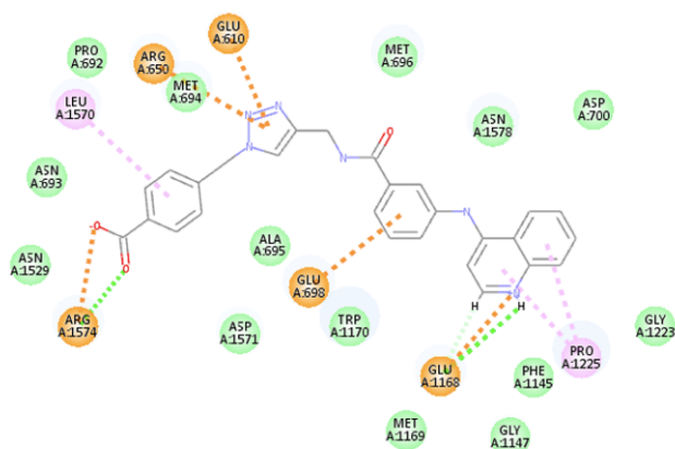
(B) compound C (benzoic acid group)
