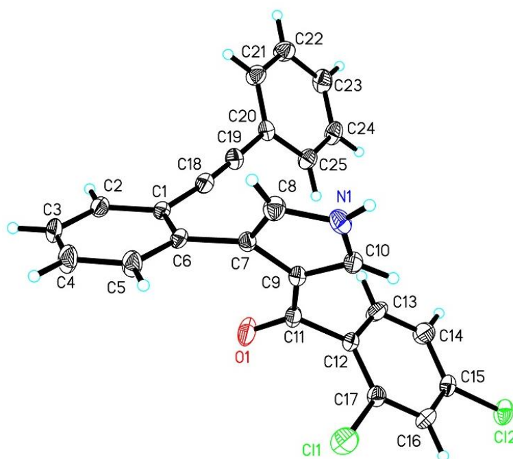
Figure 1. The crystal structure of 3e (CCDC: 2161393)
