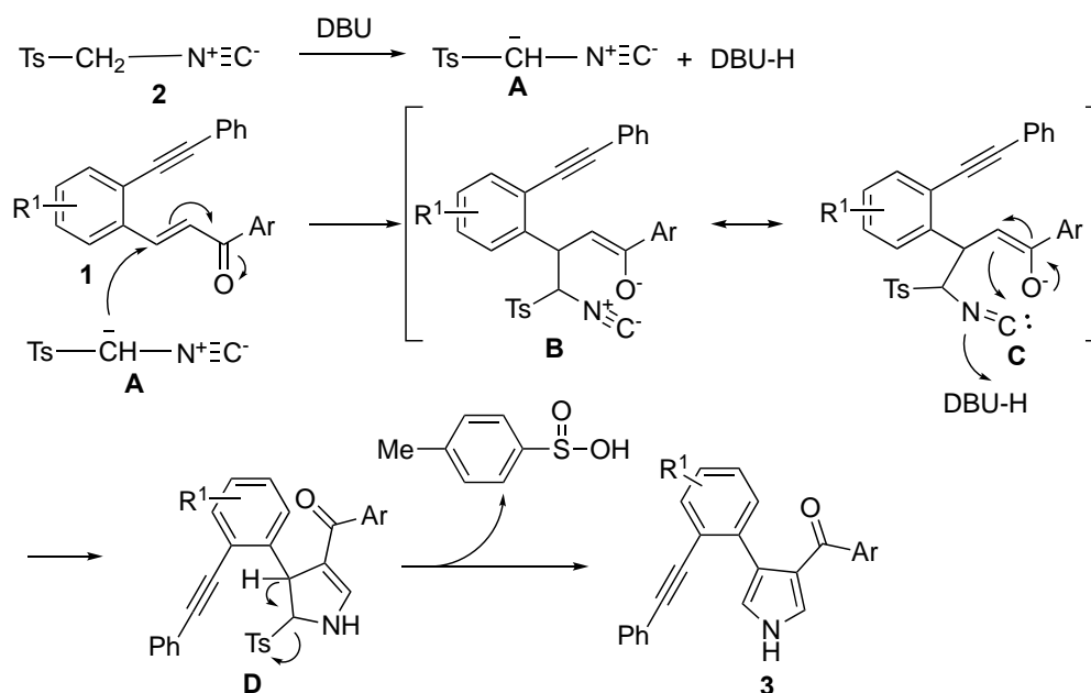
Scheme 2. The possible reaction mechanism of product 3
