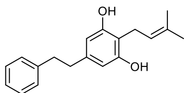
3,5-dihydroxy-4-(3-methyl-2-butenyl)biphenyl ( 26 )
