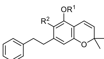
2,2-dimethyl-5-hydroxy-7-(2-phenylethyl)chromene ( 34 )
