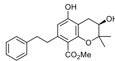
radstrictin D ( 40 )
