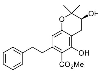
radstrictin C ( 39 )
