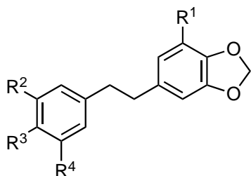
3-hydroxy-4,5-methylenedioxybibenzyl ( 3 )
