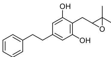
3,5-dihydroxy-4-(2,3-epoxy-3-methylbutyl)biphenyl ( 27 )
