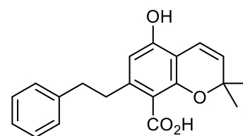
saccatene C ( 37 )
