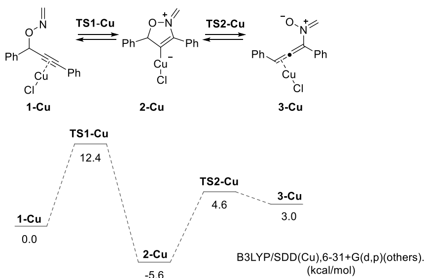
Scheme 2. Reaction profile of Cu-catalyzed [2,3]-rearrangement of O -propargylic formaldoxime
