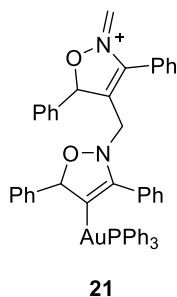
Scheme 12. A possible structure of the detected species Au2 in Figure 1
