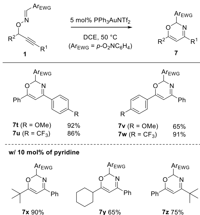
Scheme 16. Scope of Au-catalyzed reactions of 1t–z via N-O bond cleavage
