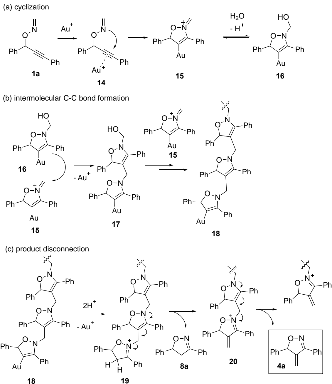
Scheme 11. Proposed mechanism for Au-catalyzed reactions of O -propargylic formaldoxime 1a
