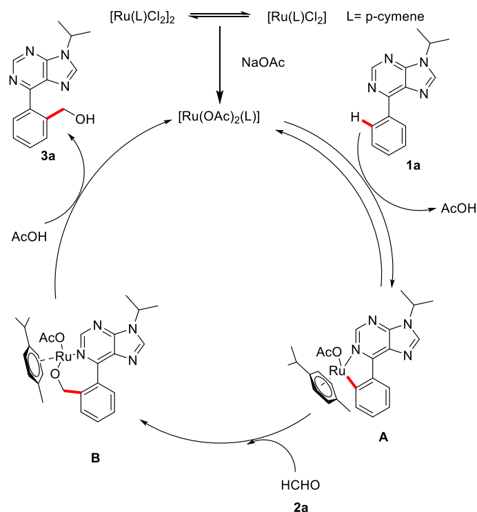
Scheme 6. Plausible mechanism
