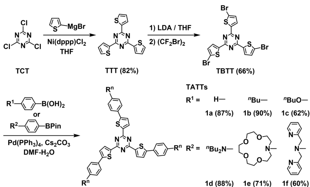
Scheme 1. Synthetic routes of TATTs 1a–f
