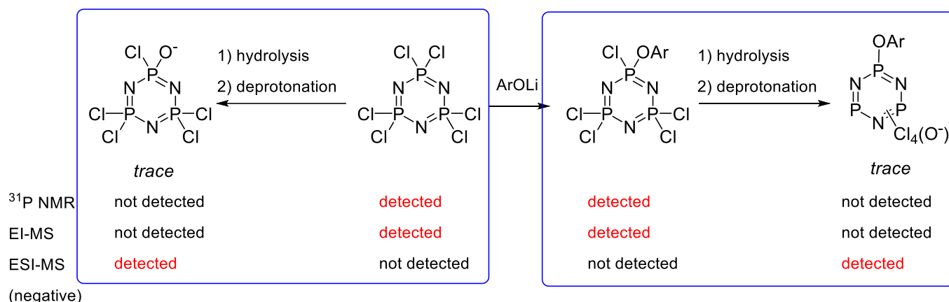
Scheme 4. ^{31}\text{P} NMR and MS identification of chlorocyclotriphosphazene derivatives
