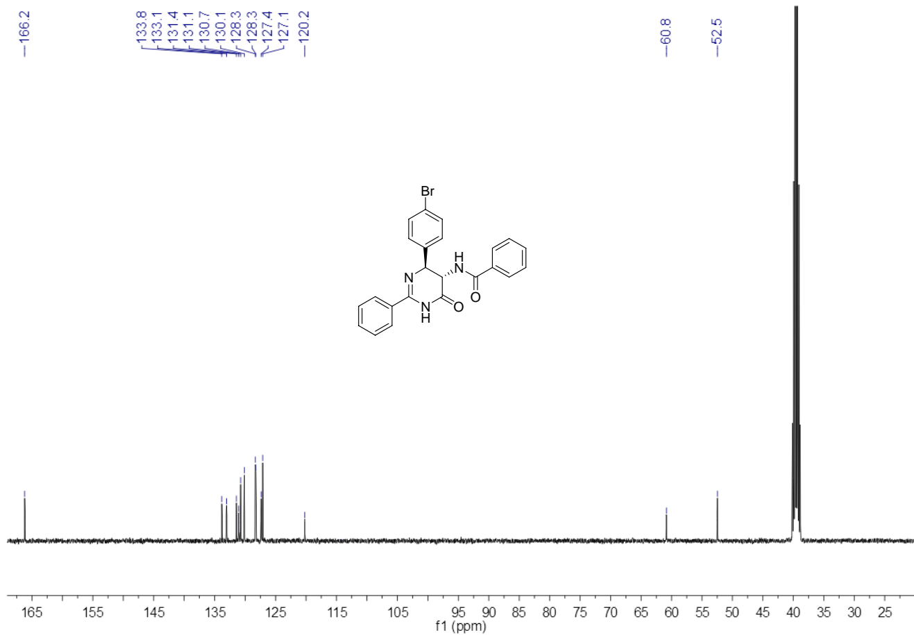
13 C NMR Spectrum of Compound 3b
