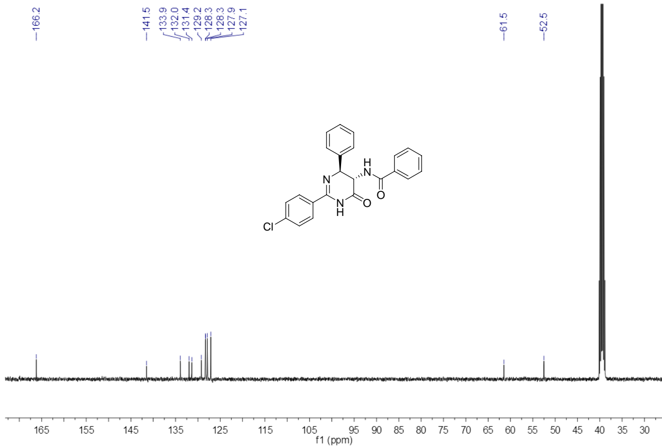
13 C NMR Spectrum of Compound 3l
