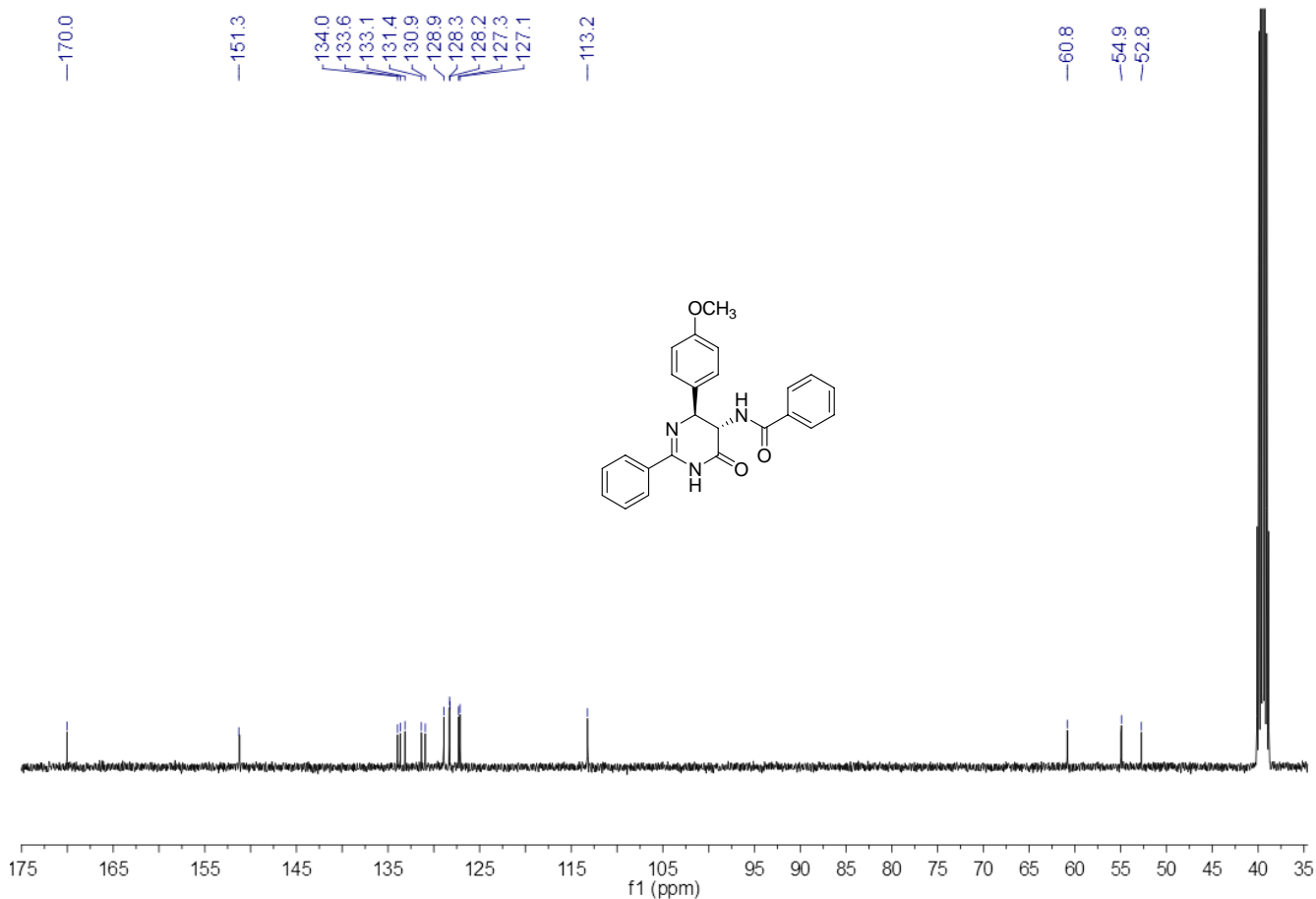
13 C NMR Spectrum of Compound 3e
