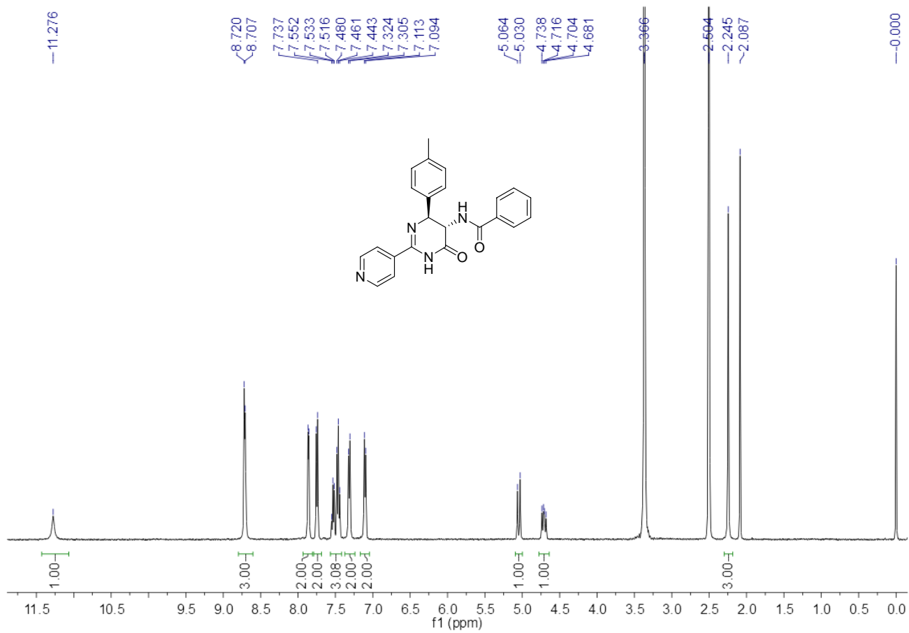
1 H NMR Spectrum of Compound 3u
