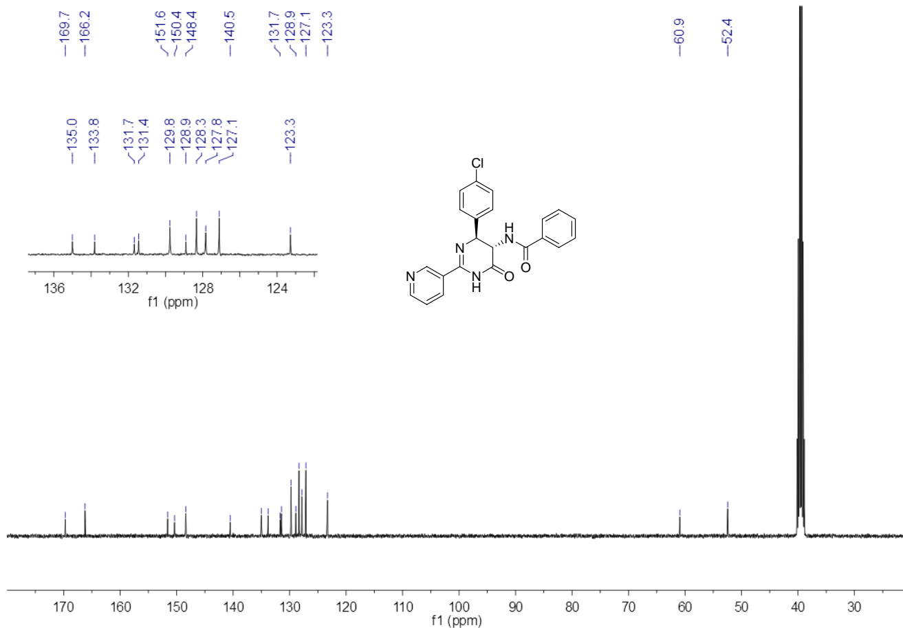
13 C NMR Spectrum of Compound 3o
