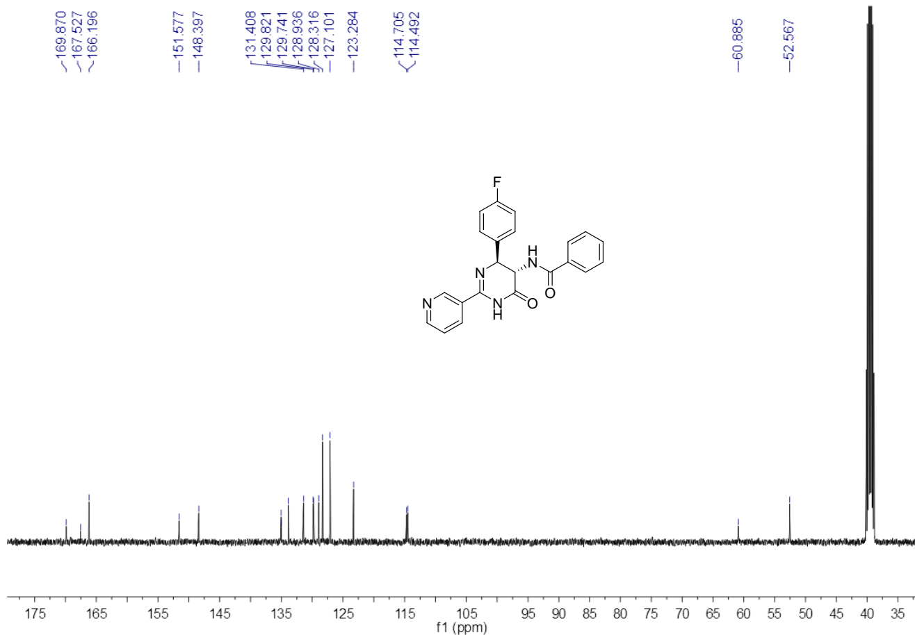
13 C NMR Spectrum of Compound 3p
