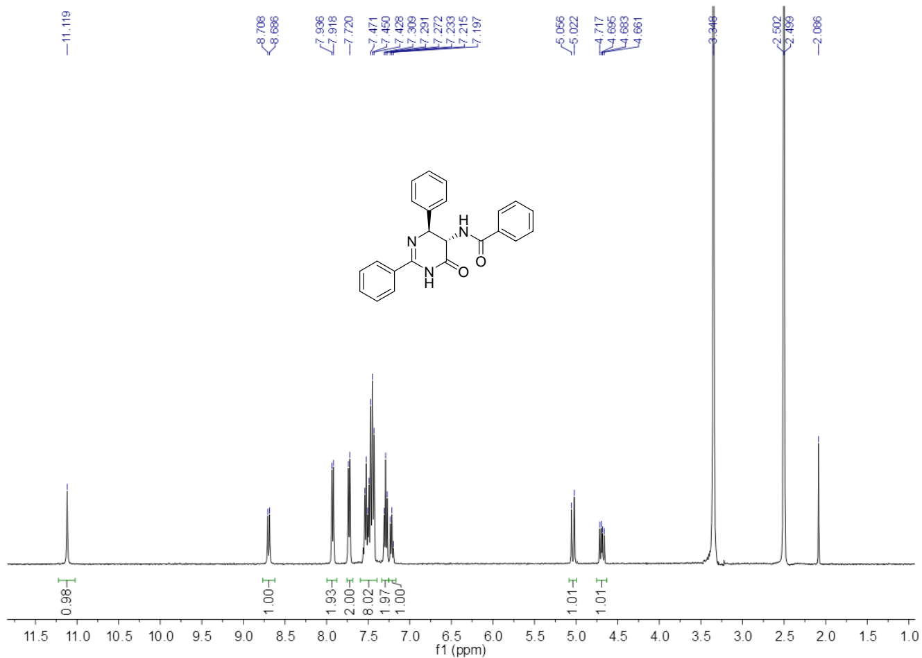
1 H NMR Spectrum of Compound 3d
