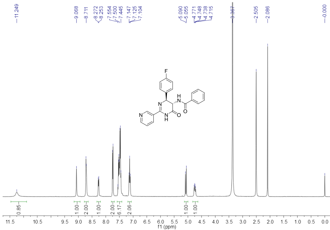
1 H NMR Spectrum of Compound 3p
