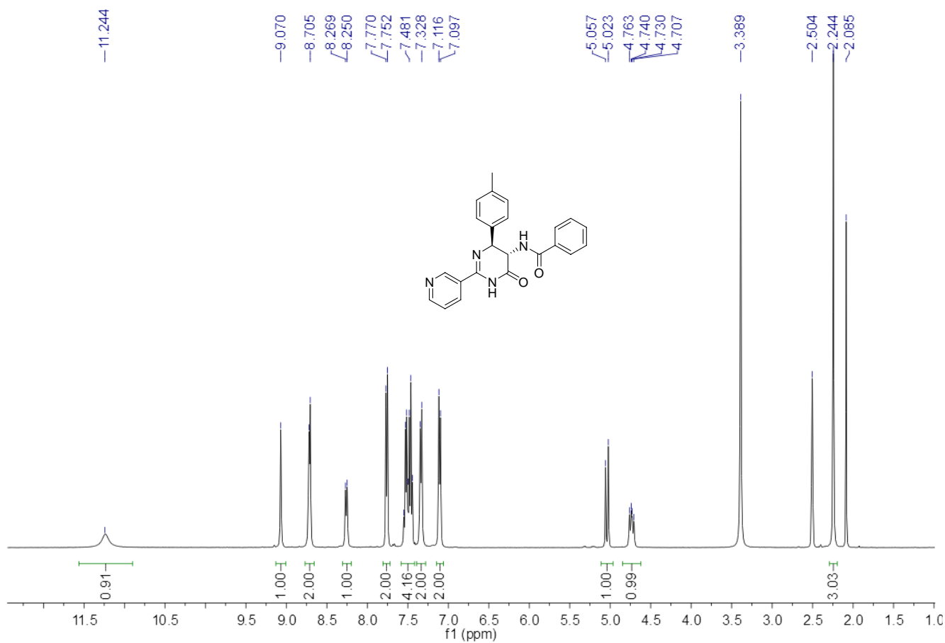
1 H NMR Spectrum of Compound 3q
