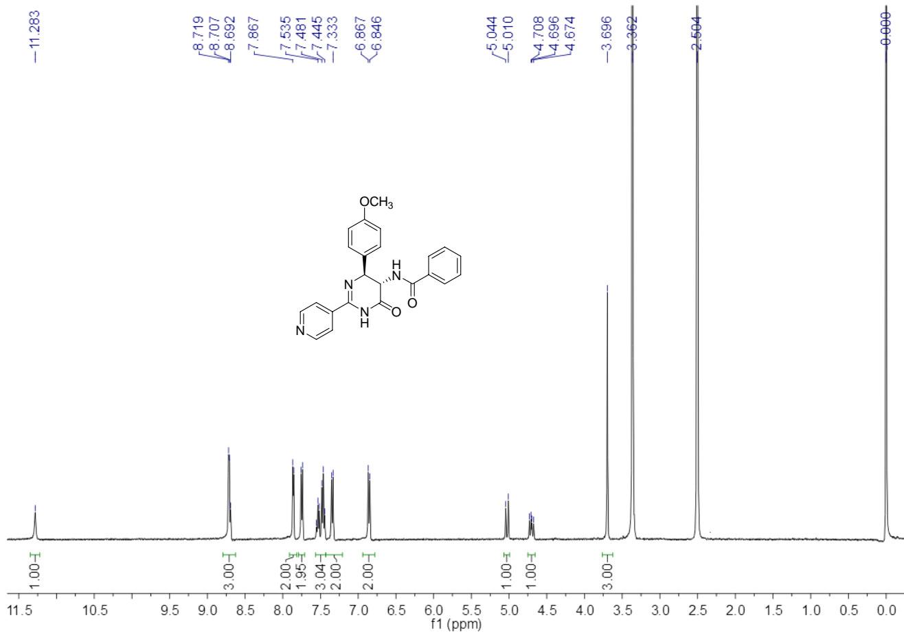
1 H NMR Spectrum of Compound 3t
