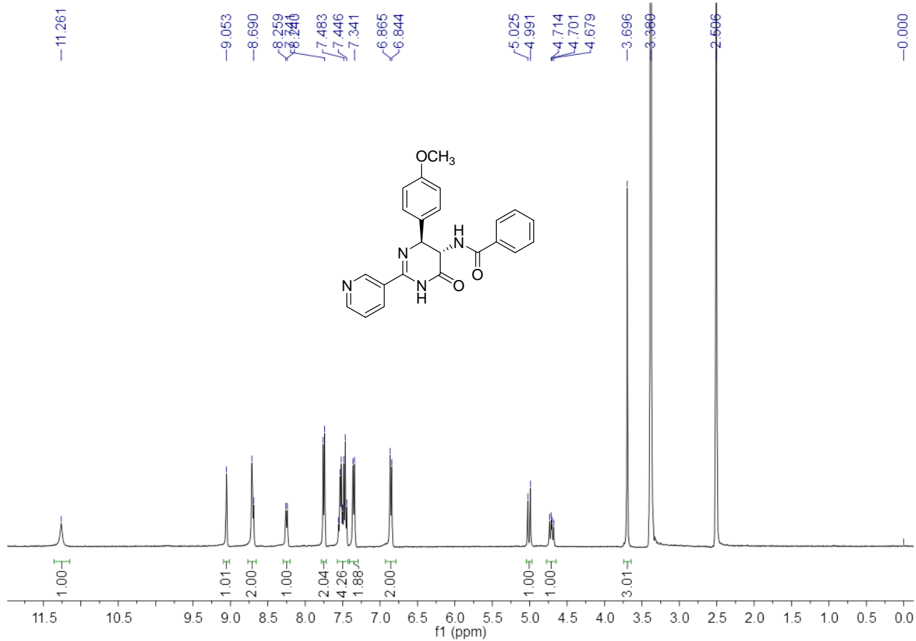
1 H NMR Spectrum of Compound 3r
