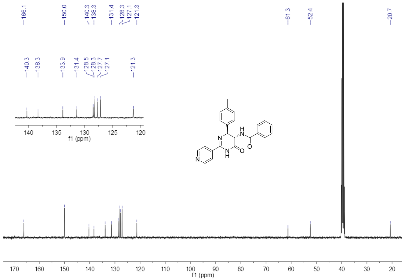
13 C NMR Spectrum of Compound 3u
