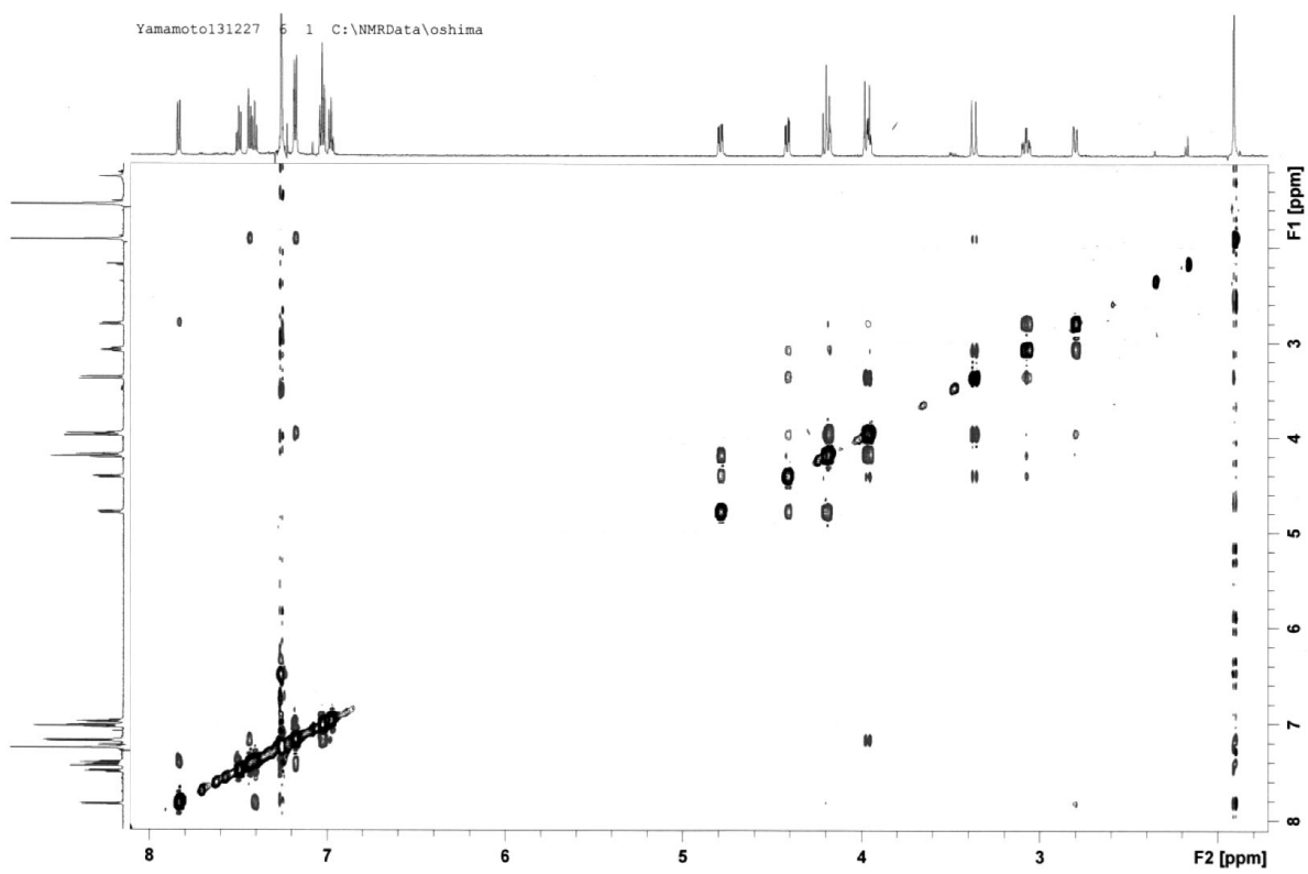
Figure S4. NOESY of 3a (in \text{CDCl}_3 )
