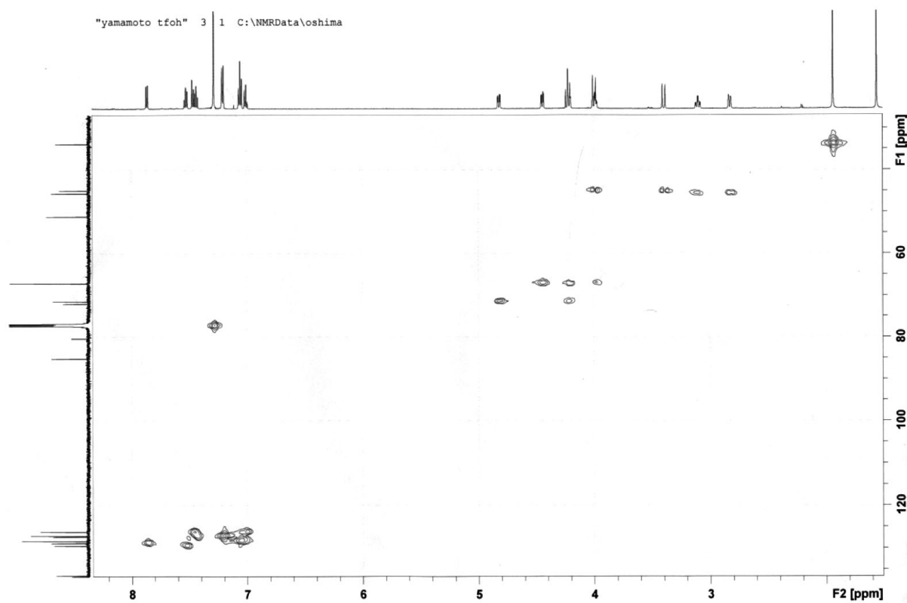
Figure S2. HSQC of 3a (in CDCl 3 )
