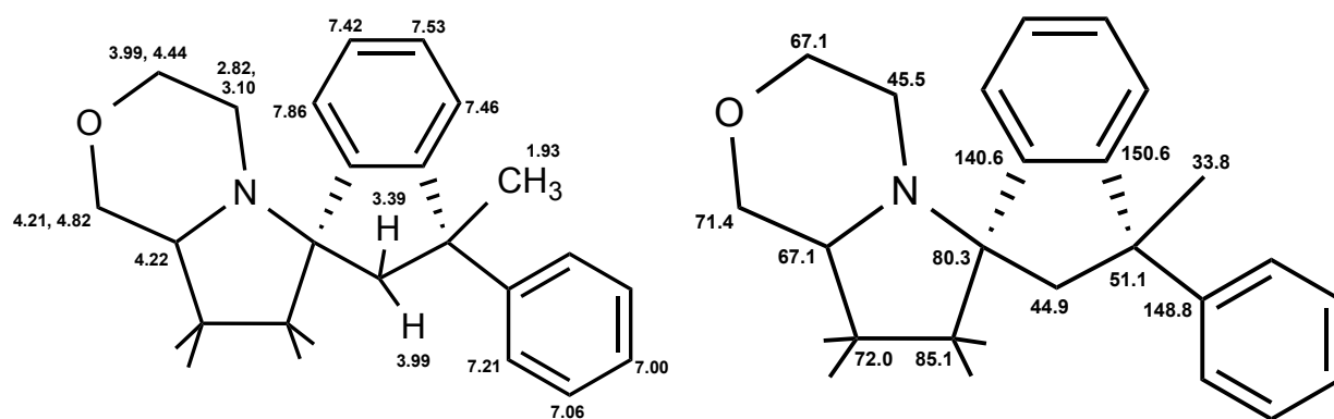
Figure S1. Plausible 1 H (left) and 13 C (right) NMR assignments for 3a
