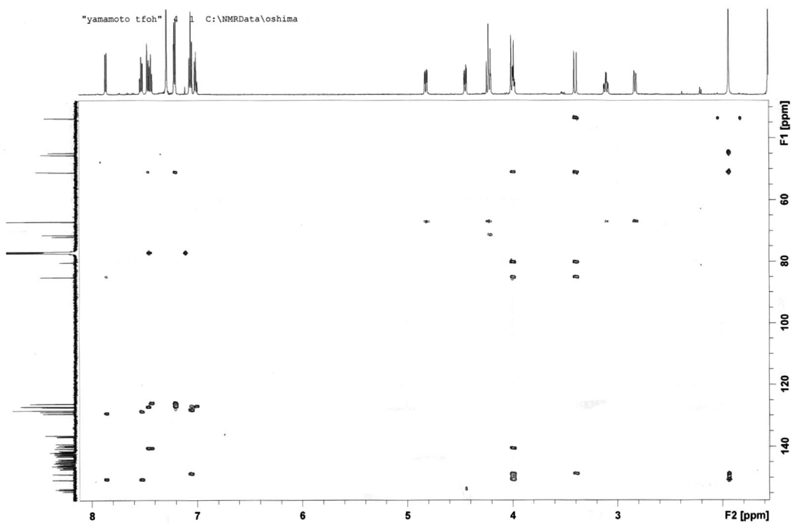
Figure S3. HMBC of 3a (in \text{CDCl}_3 )
