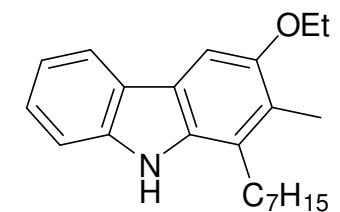
2: O-ethylcarazostatin
