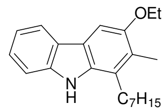
2: O-ethylcarazostatin
