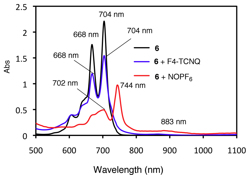
UV-vis spectra of 6 ( \text{CHCl}_3 )
