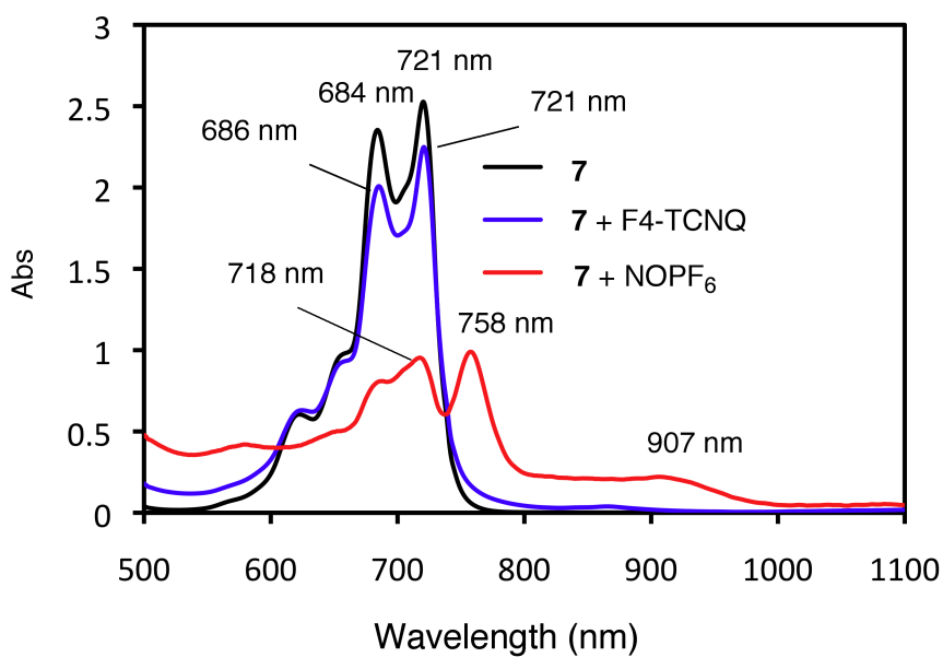
UV-vis spectra of 7 ( \text{CHCl}_3 )
