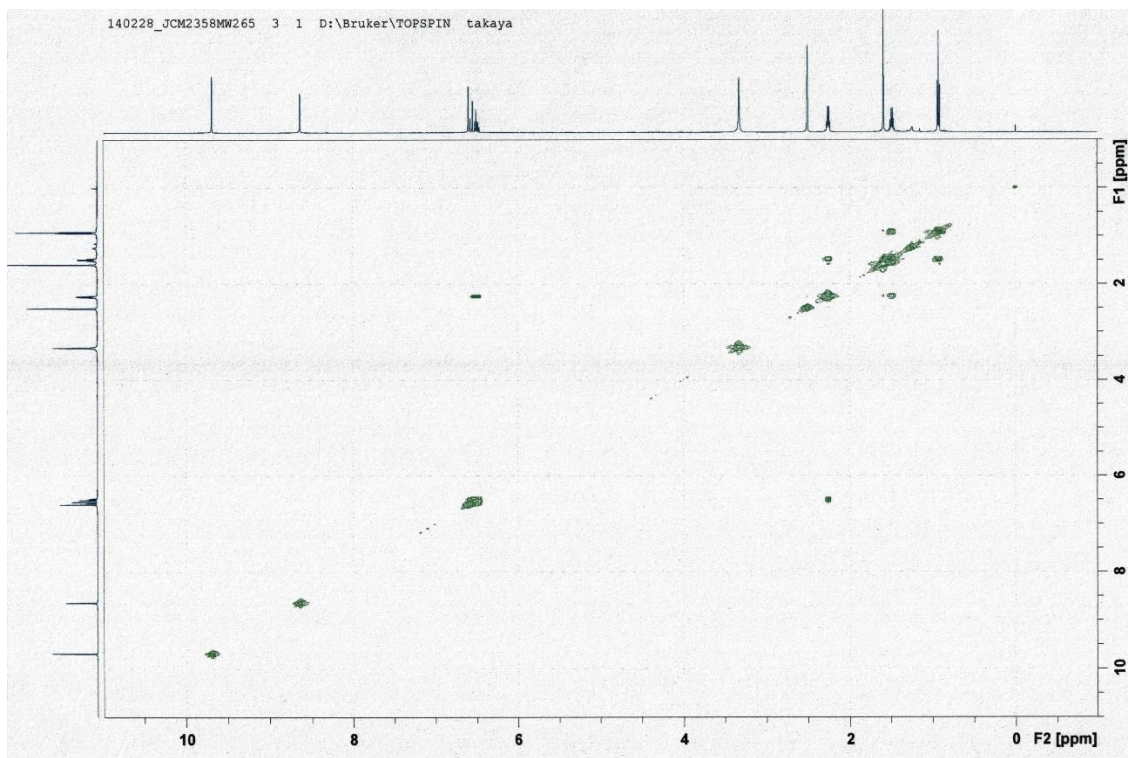
Figure S3. COSY spectrum of compound 1 (DMSO- d_6 ).
