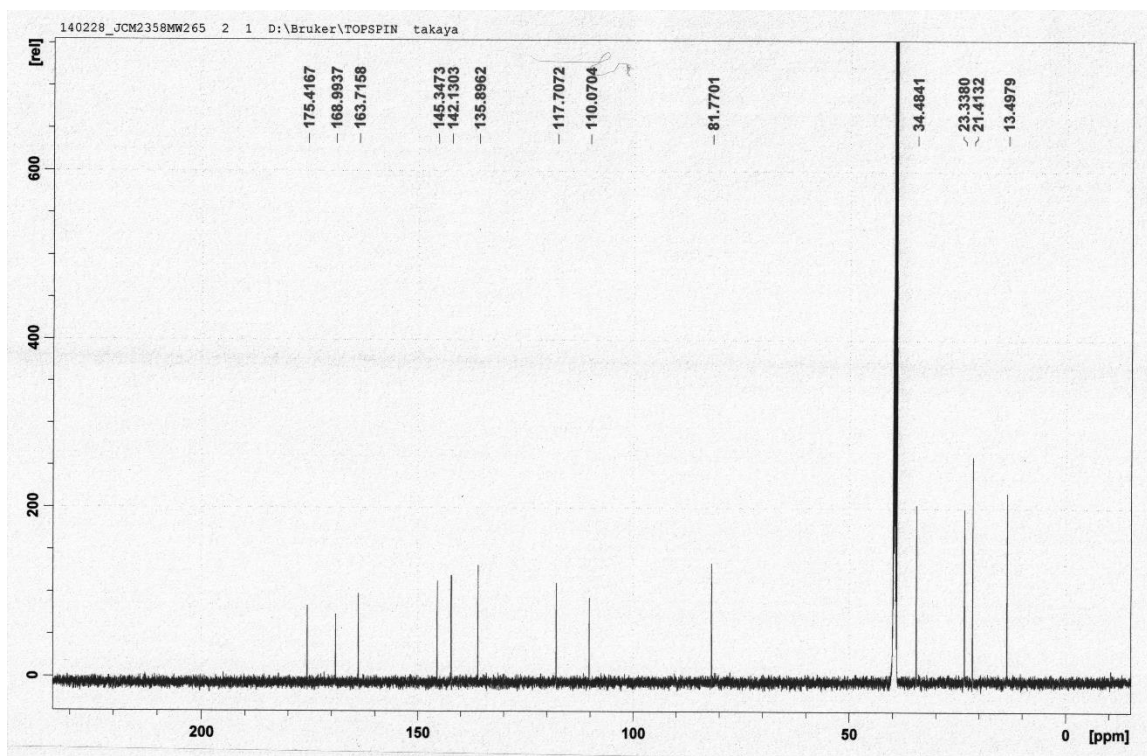
Figure S2. ^{13}\text{C} -NMR spectrum of compound 1 ( \text{DMSO-}d_6 ).
