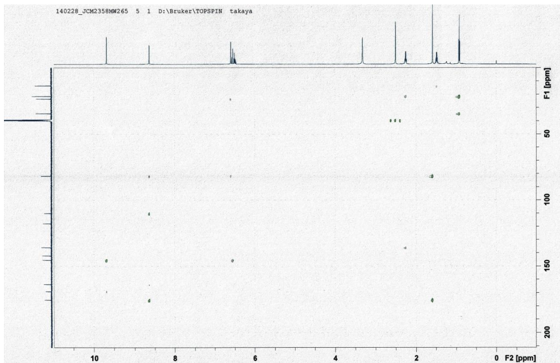
Figure S5. HMBC spectrum of compound 1 (DMSO- d_6 ).
