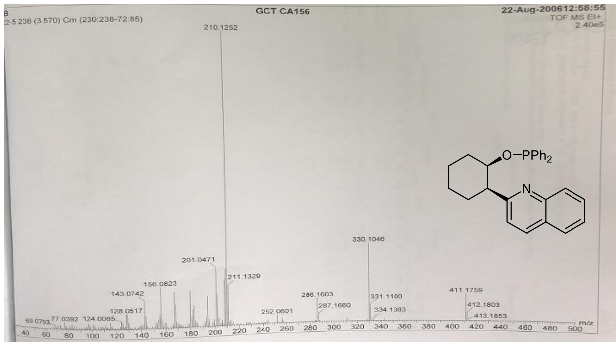
Figure S 11. HRMS spectrum of [(1 R ,2 R )- cis -2-Quinolin-2-ylcyclohexan-1-yl]diphenyl phosphine
