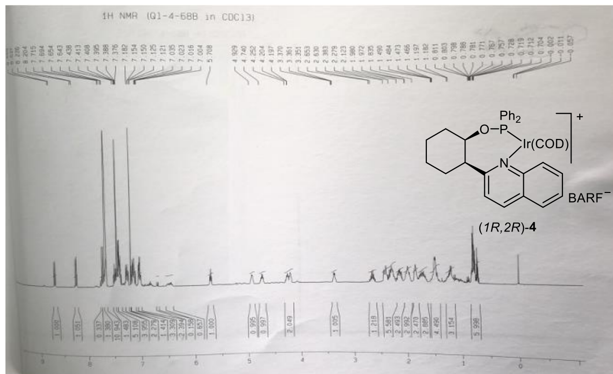
Figure S 19. 1 H-NMR spectrum of Iridium-complex (1R,2R)-4
