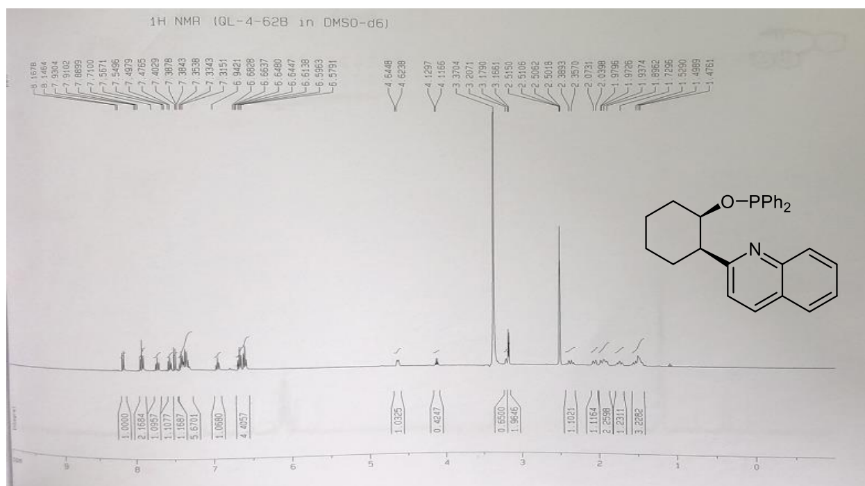
Figure S 8. ^1\text{H} -NMR spectrum of [(1 R ,2 R )- cis -2-Quinolin-2-ylcyclohexan-1-oxyl]diphenyl phosphine
