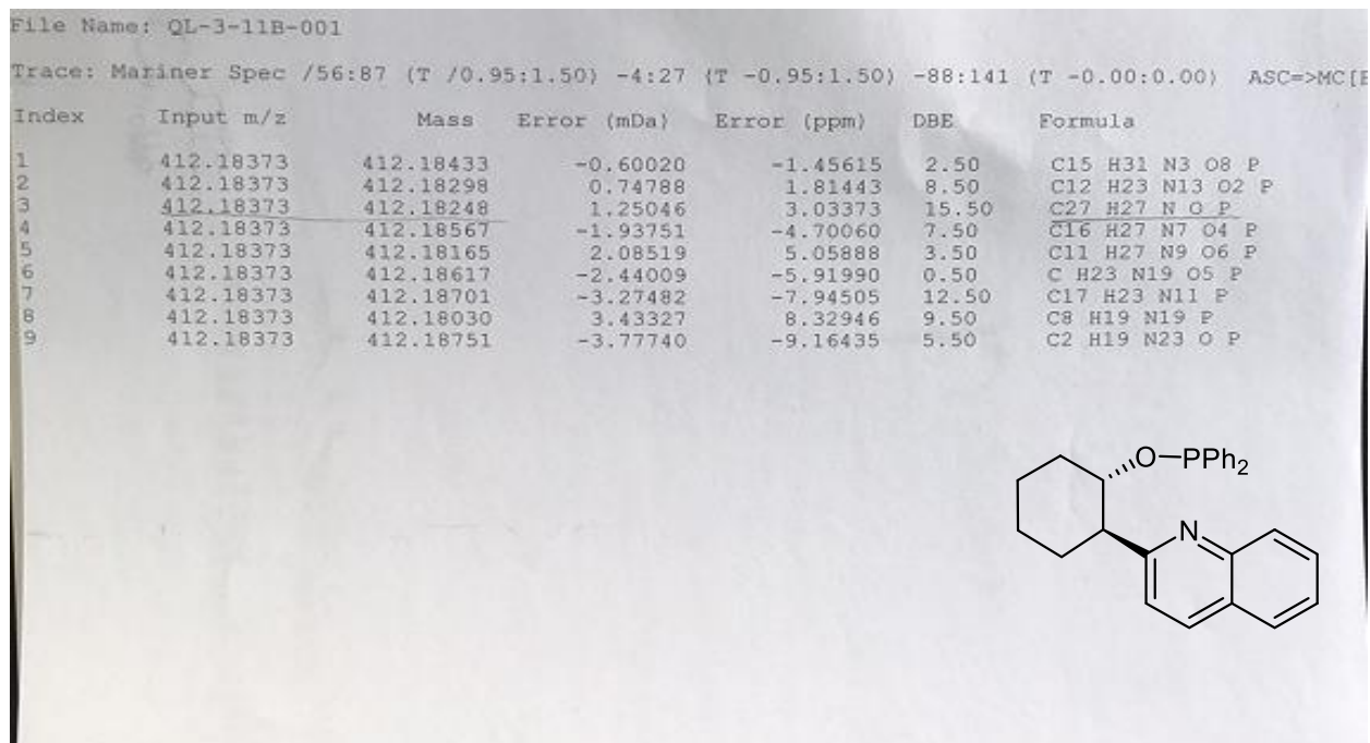
Figure S 7. HRMS spectrum of [(1S,2R)-trans-2-Quinolin-2-ylcyclohexan-1-oxy]diphenyl phosphine
