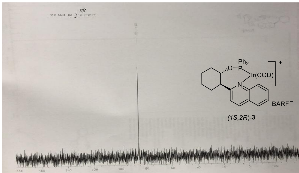
Figure S 14. 31 P-NMR spectrum of Iridium-complex (1 S ,2 R )-3
