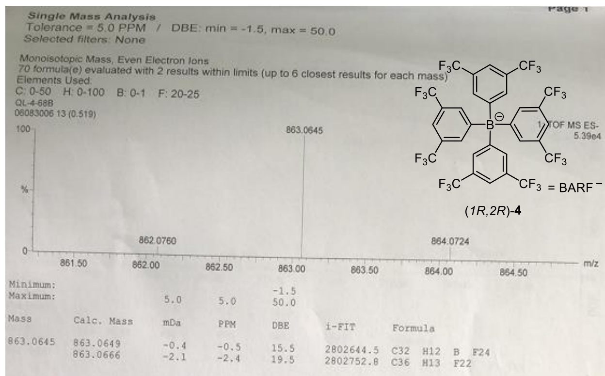
Figure S 24. HRMS (anion) spectrum of Iridium-complex (1R,2R)-4
