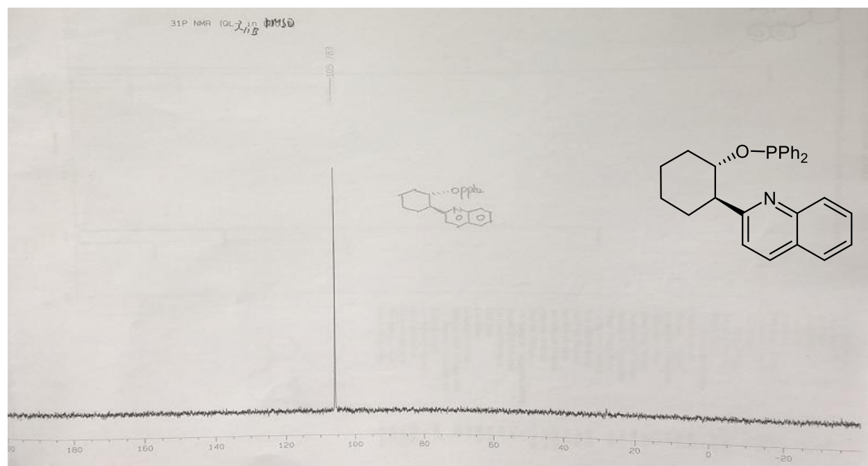
Figure S 4. ^{13}\text{C} -NMR spectrum of [(1 S ,2 R )- trans -2-Quinolin-2-ylcyclohexan-1-oxyl]diphenyl phosphine
