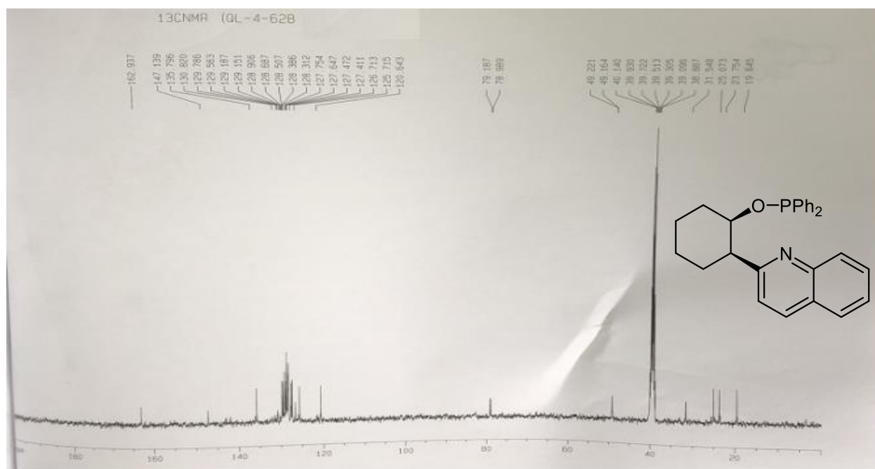
Figure S 9. ^{13}\text{C} -NMR spectrum of [(1 R ,2 R )- cis -2-Quinolin-2-ylcyclohexan-1-oxyl]diphenyl phosphine
