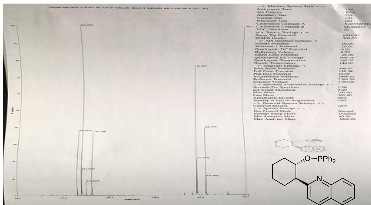
Figure S 6. HRMS spectrum of [(1S,2R)-trans-2-Quinolin-2-ylcyclohexan-1-oxy]diphenyl phosphine
