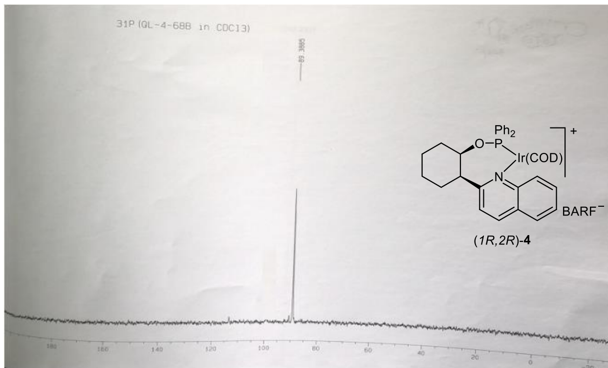
Figure S 20. 31 P-NMR spectrum of Iridium-complex (1R,2R)-4
