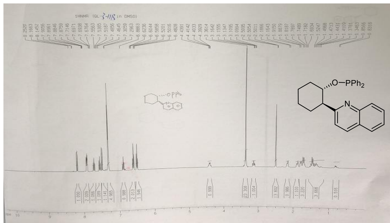
Figure S 2. Chiral HPLC spectrum of compound (1S,2R)-7
