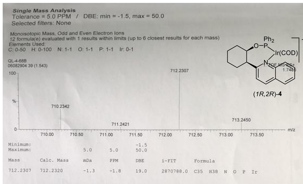
Figure S 22. HRMS (cation) spectrum of Iridium-complex (1R,2R)-4
