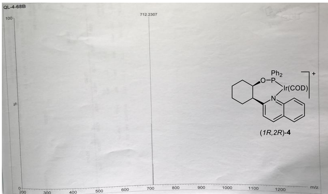
Figure S 21. HRMS (cation) spectrum of Iridium-complex (1R,2R)-4
