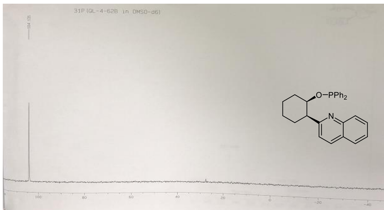
Figure S 10. ^{31}\text{P} -NMR spectrum of [(1 R ,2 R )- cis -2-Quinolin-2-ylcyclohexan-1-yl]diphenyl phosphine
