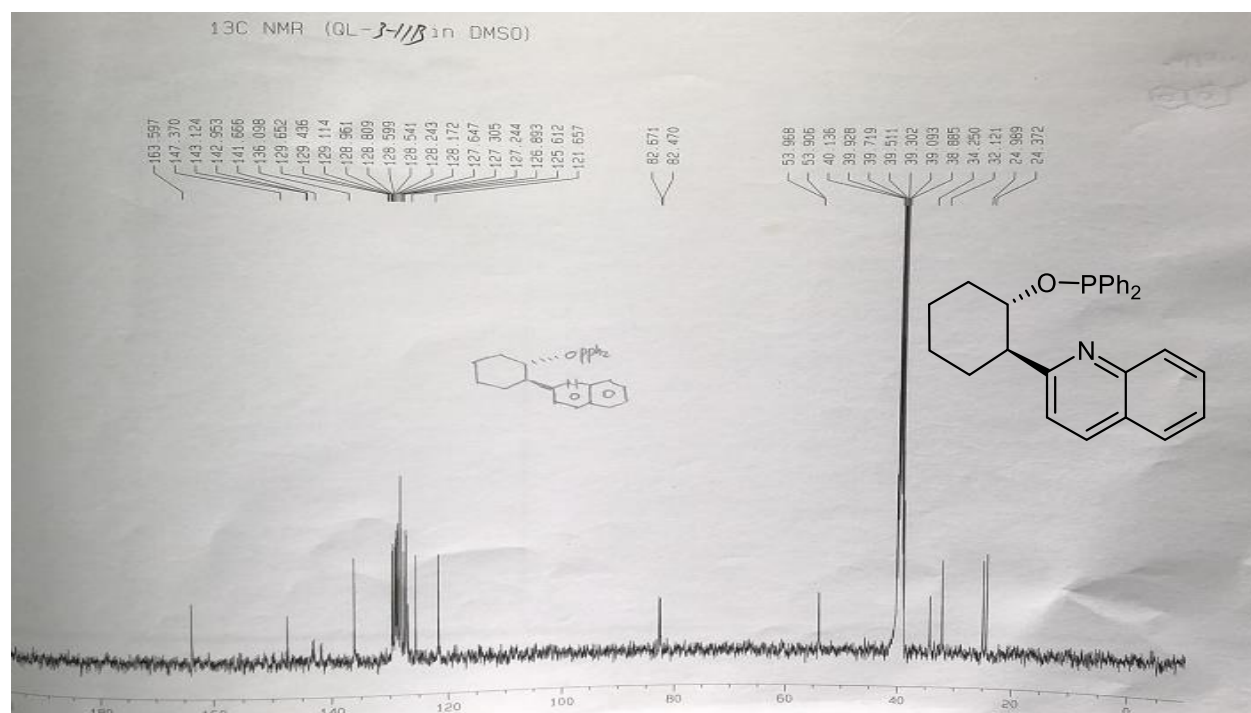
Figure S 4. ^{13}\text{C} -NMR spectrum of [(1 S ,2 R )- trans -2-Quinolin-2-ylcyclohexan-1-oxyl]diphenyl phosphine
