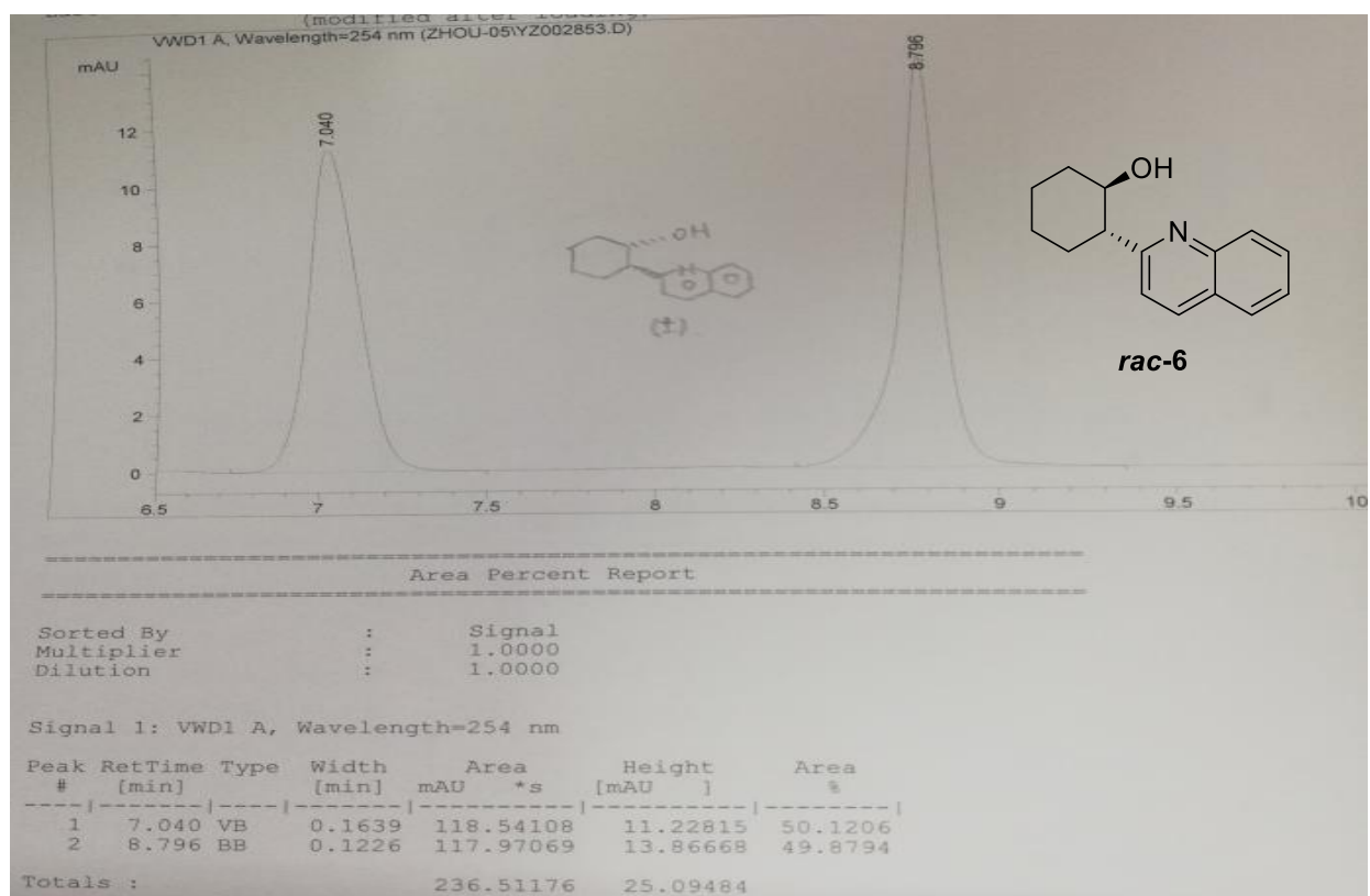
Figure S 1. Chiral HPLC spectrum of compound rac-6
