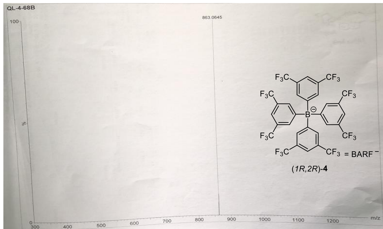
Figure S 23. HRMS (anion) spectrum of Iridium-complex (1R,2R)-4
