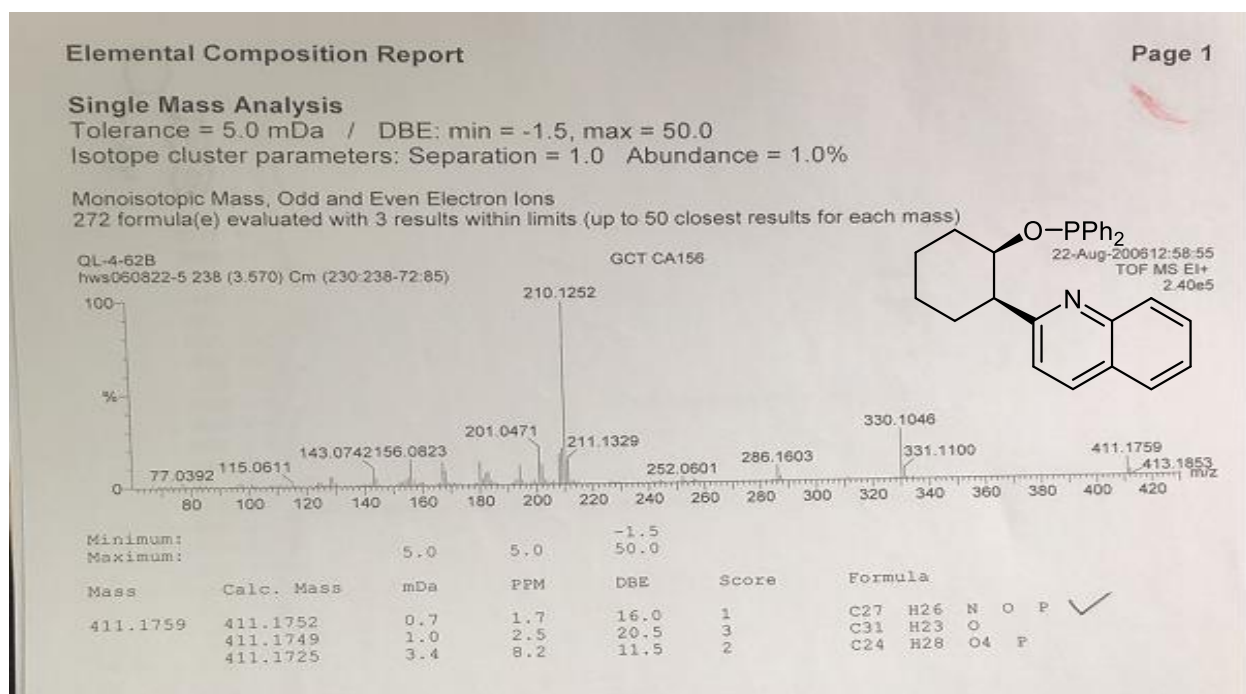
Figure S 12. HRMS spectrum of [(1 R ,2 R )- cis -2-Quinolin-2-ylcyclohexan-1-oxyl]diphenyl phosphine
