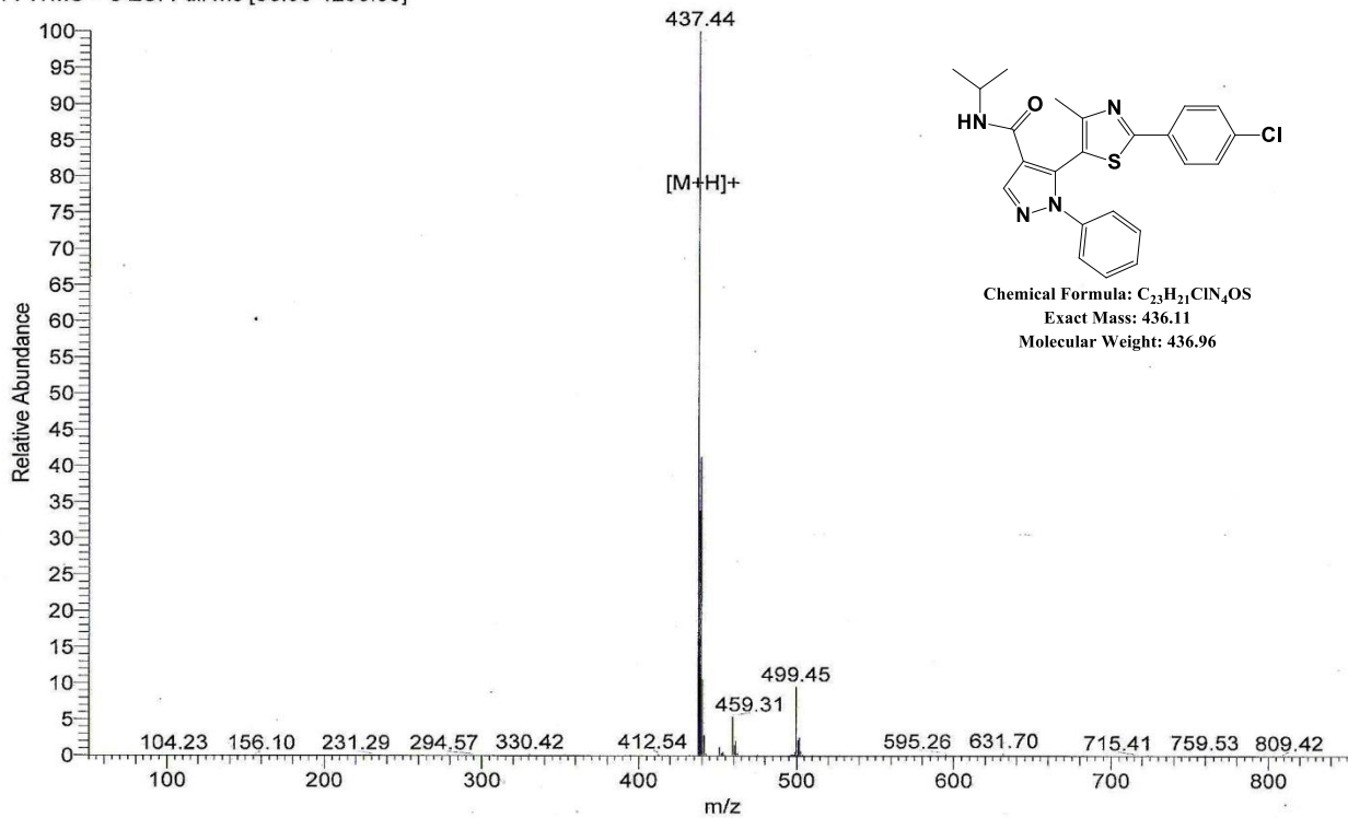
Spectrum No 51: Mass Spectra of 5-(2-(4-chlorophenyl)-4-methylthiazol-5-yl)-N-isopropyl-1-phenyl-1H-pyrazole-4-carboxamide 11d
