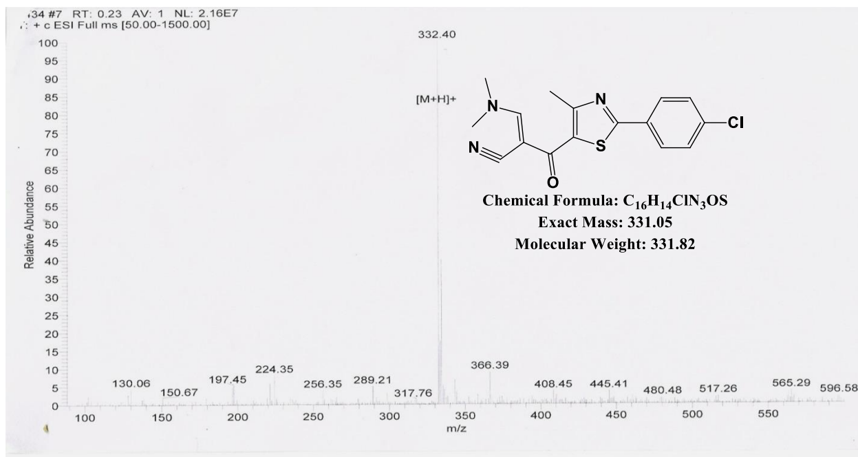
Spectrum No 10: Mass Spectra of 2-(2-(4-chlorophenyl)-4-methylthiazole-5-carbonyl)-3-(dimethylamino)acrylonitrile 7
