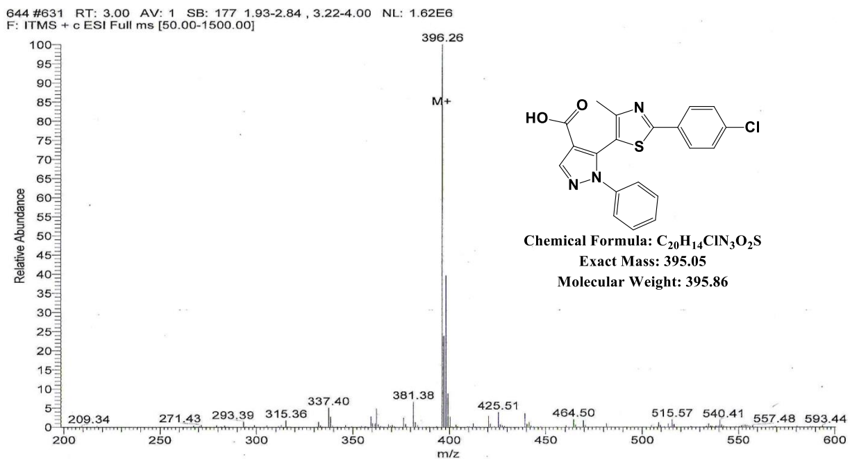
Spectrum No 35: Mass Spectra of 5-(2-(4-chlorophenyl)-4-methylthiazol-5-yl)-1-phenyl-1H-pyrazole-4-carboxylic acid 10
