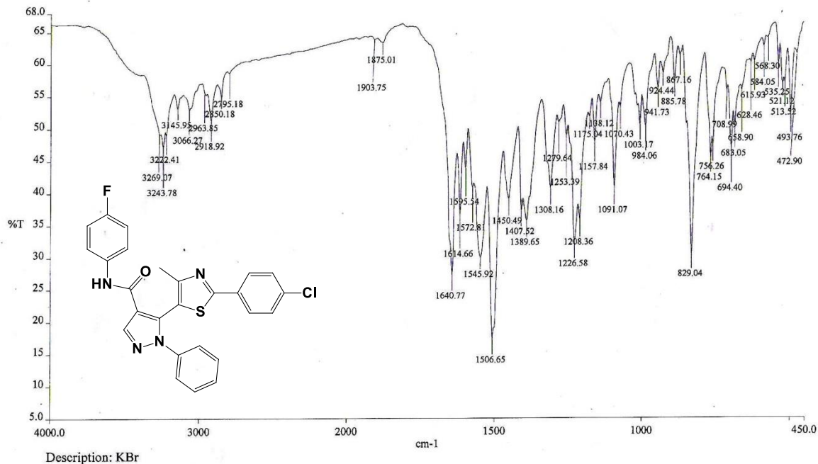
Spectrum No 36: IR Spectra(KBr) of 5-(2-(4-chlorophenyl)-4-methylthiazol-5-yl)-N-(4-fluorophenyl)-1-phenyl-1H-pyrazole-4-carboxamide 11a
