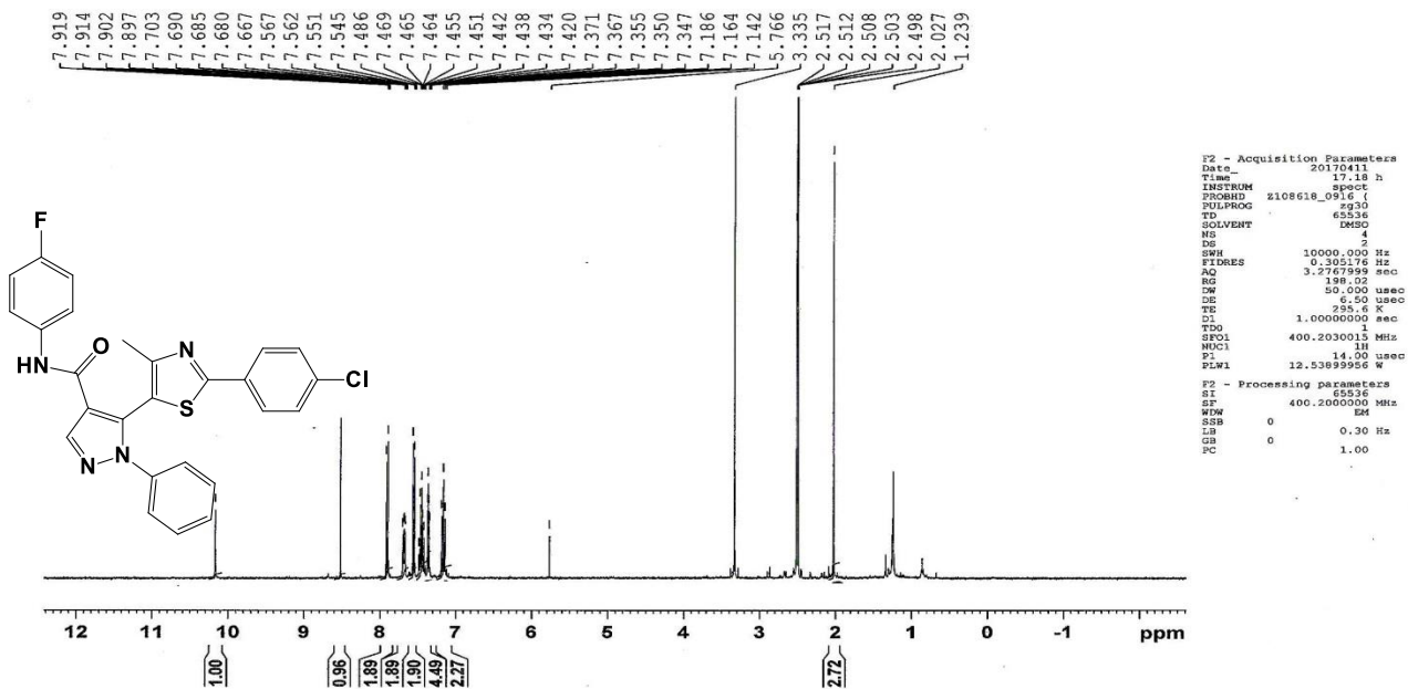
Spectrum No 37: 1 H NMR Spectra(DMSO-d 6 ) of 5-(2-(4-chlorophenyl)-4-methylthiazol-5-yl)-N-(4-fluorophenyl)-1-phenyl-1H-pyrazole-4-carboxamide 11a
