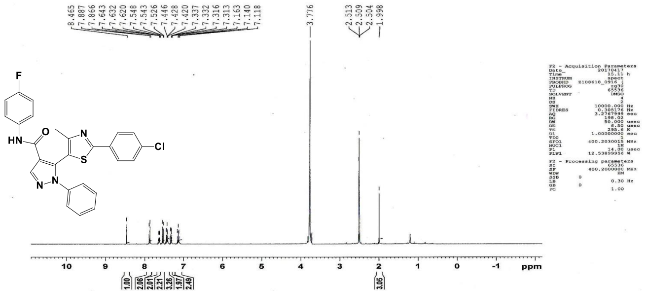
Spectrum No 38 :D 2 O NMR Spectra(DMSO-d 6 + D 2 O) of 5-(2-(4-chlorophenyl)-4-methylthiazol-5-yl)-N-(4-fluorophenyl)-1-phenyl-1H-pyrazole-4-carboxamide 11a
