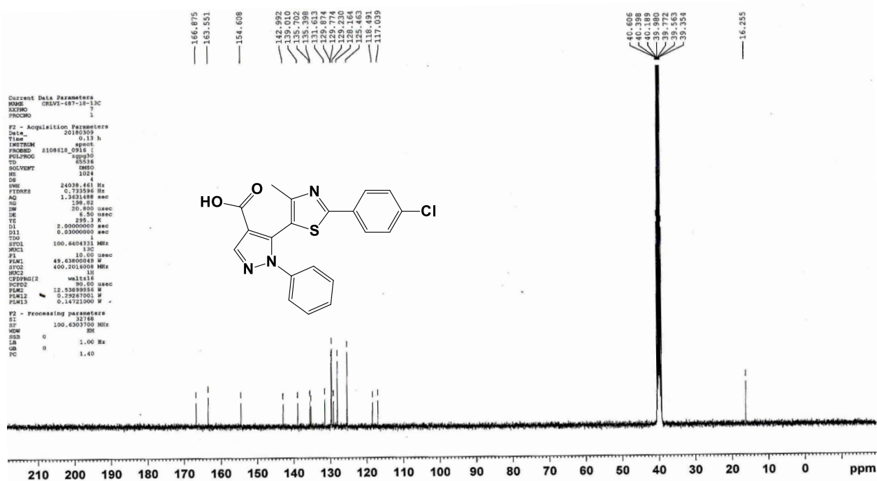
Spectrum No 34 : 13 C NMR Spectra(DMSO-d 6 ) of 5-(2-(4-chlorophenyl)-4-methylthiazol-5-yl)-1-phenyl-1H-pyrazole-4-carboxylic acid 10
