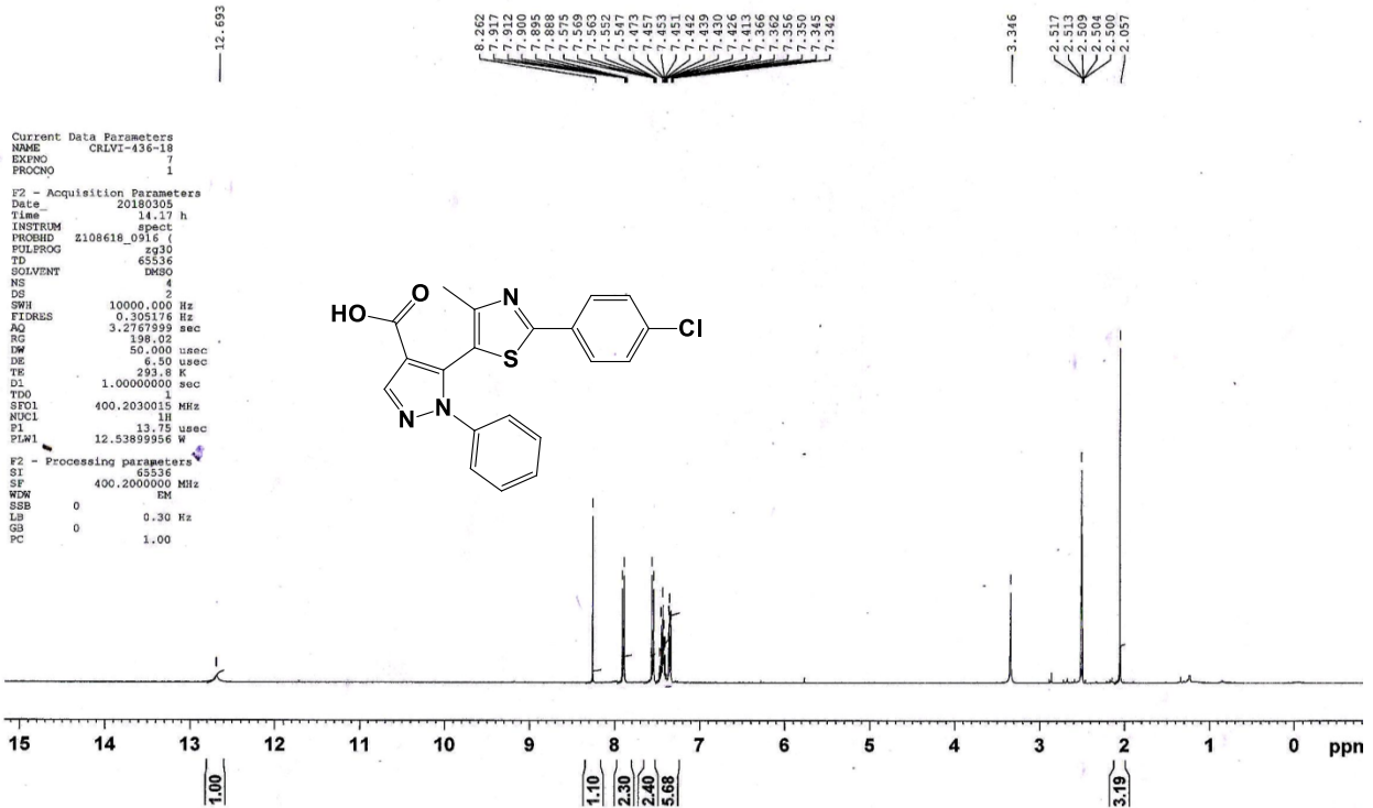
Spectrum No 32: ^1\text{H} NMR Spectra(DMSO- d_6 ) of 5-(2-(4-chlorophenyl)-4-methylthiazol-5-yl)-1-phenyl-1H-pyrazole-4-carboxylic acid 10
