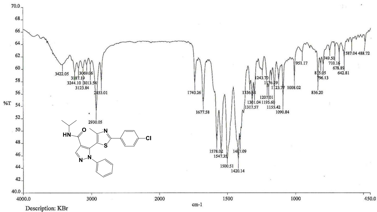
Spectrum No 49: IR Spectra(KBr) of 5-(2-(4-chlorophenyl)-4-methylthiazol-5-yl)-N-isopropyl-1-phenyl-1H-pyrazole-4-carboxamide 11d
