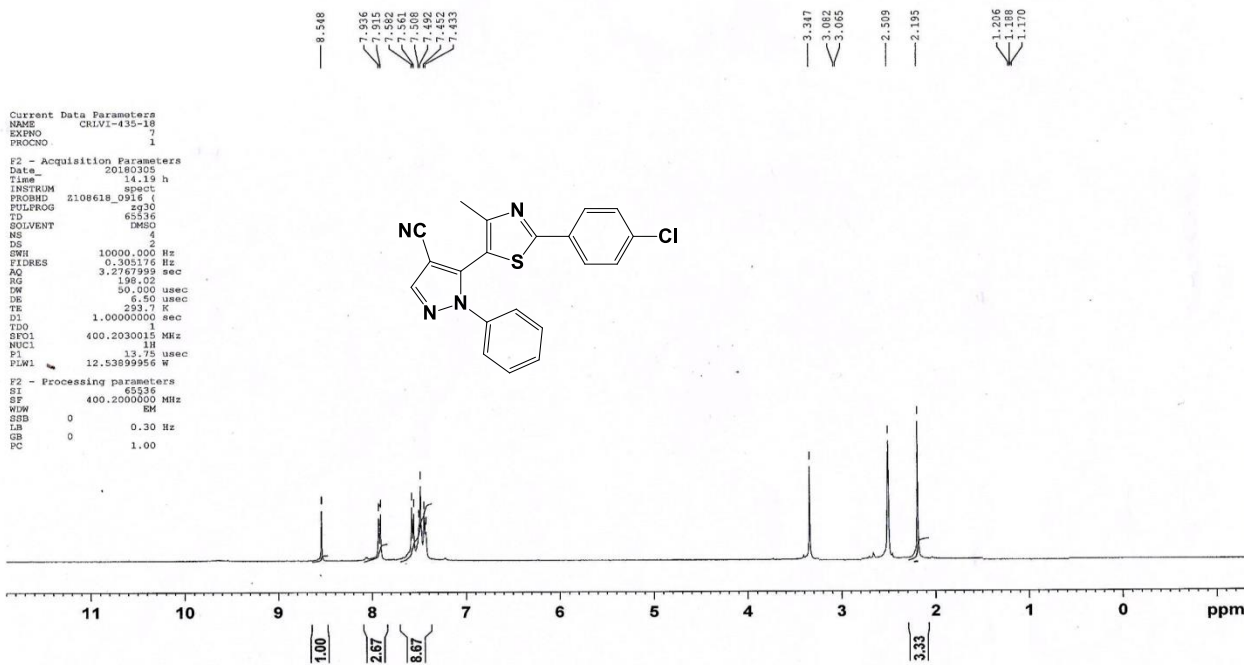
Spectrum No 12: 1 H NMR Spectra(DMSO-d 6 ) of 5-(2-(4-chlorophenyl)-4-methylthiazol-5-yl)-1-phenyl-1H-pyrazole-4-carbonitrile 8a
