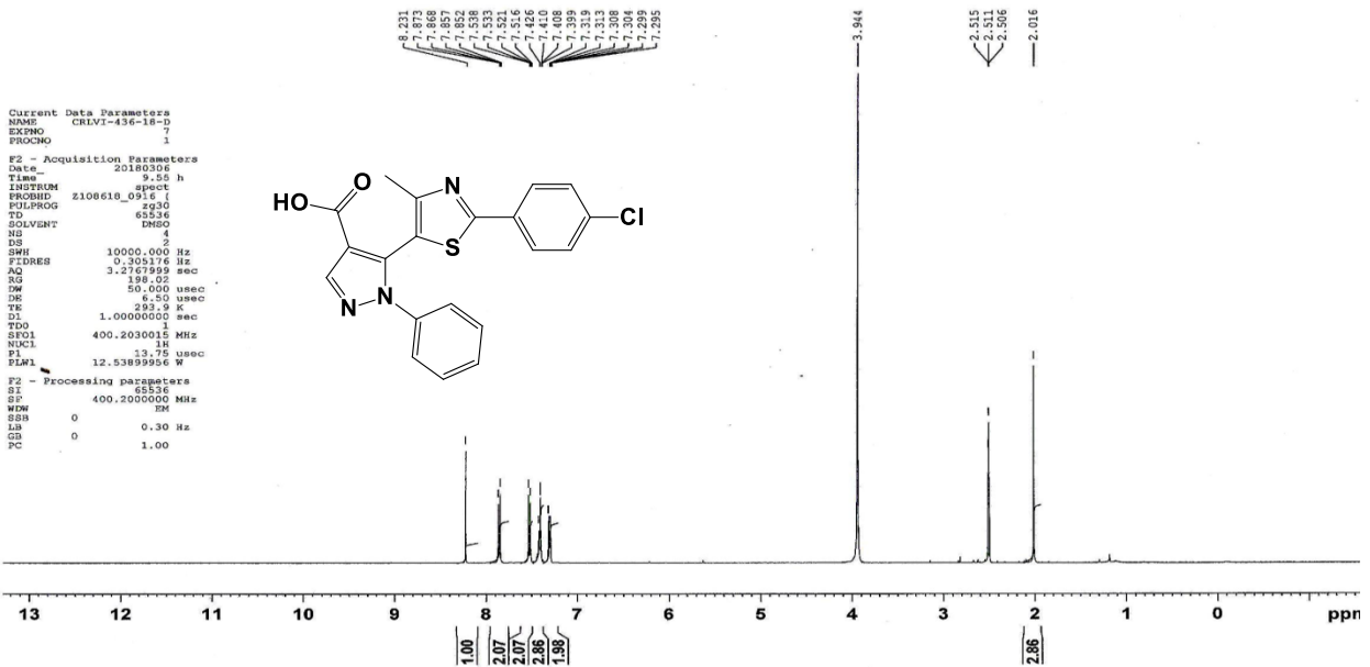
Spectrum No 33 : D_2O NMR Spectra(DMSO- d_6+D_2O ) of 5-(2-(4-chlorophenyl)-4-methylthiazol-5-yl)-1-phenyl-1H-pyrazole-4-carboxylic acid 10
