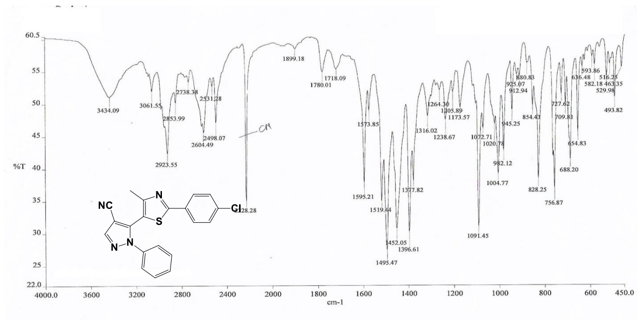
Spectrum No 11: IR Spectra(KBr) of 5-(2-(4-chlorophenyl)-4-methylthiazol-5-yl)-1-phenyl-1H-pyrazole-4-carbonitrile 8a
