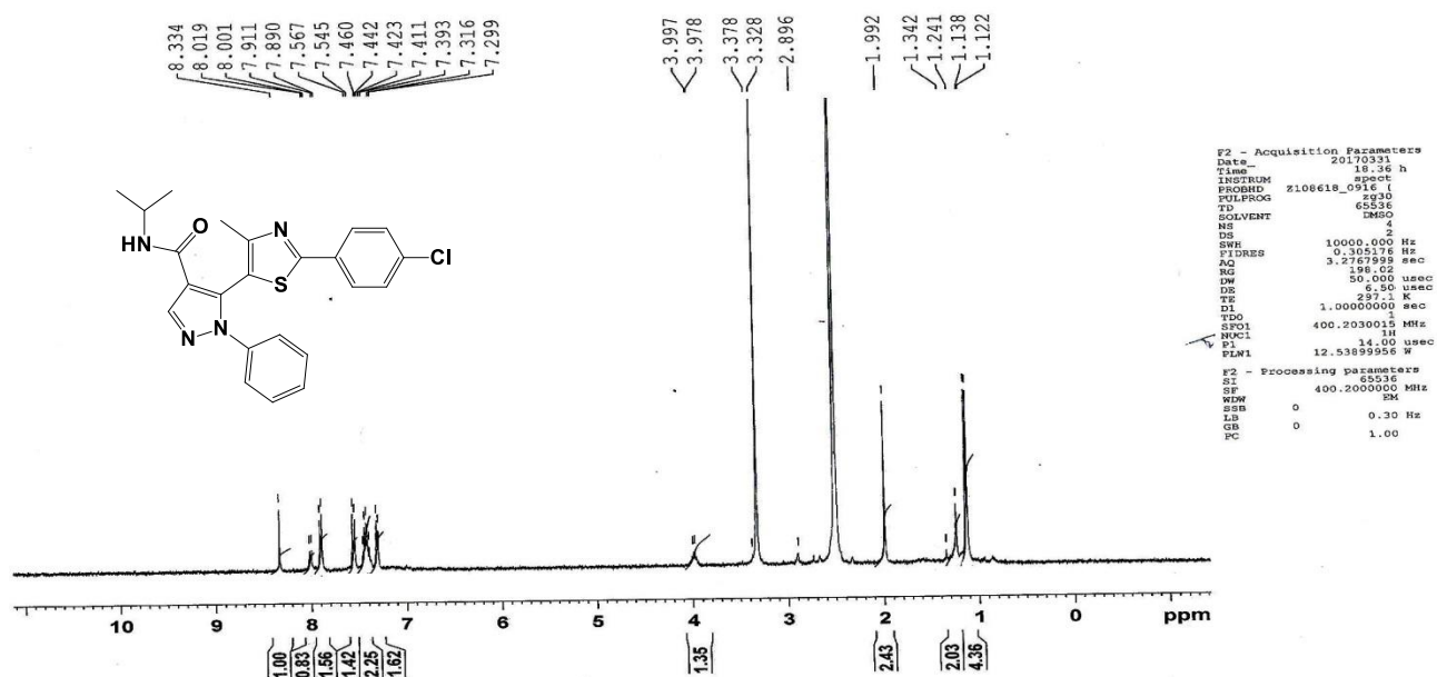
Spectrum No 50: 1 H NMR Spectra(DMSO-d 6 ) of 5-(2-(4-chlorophenyl)-4-methylthiazol-5-yl)-N-isopropyl-1-phenyl-1H-pyrazole-4-carboxamide 11d
