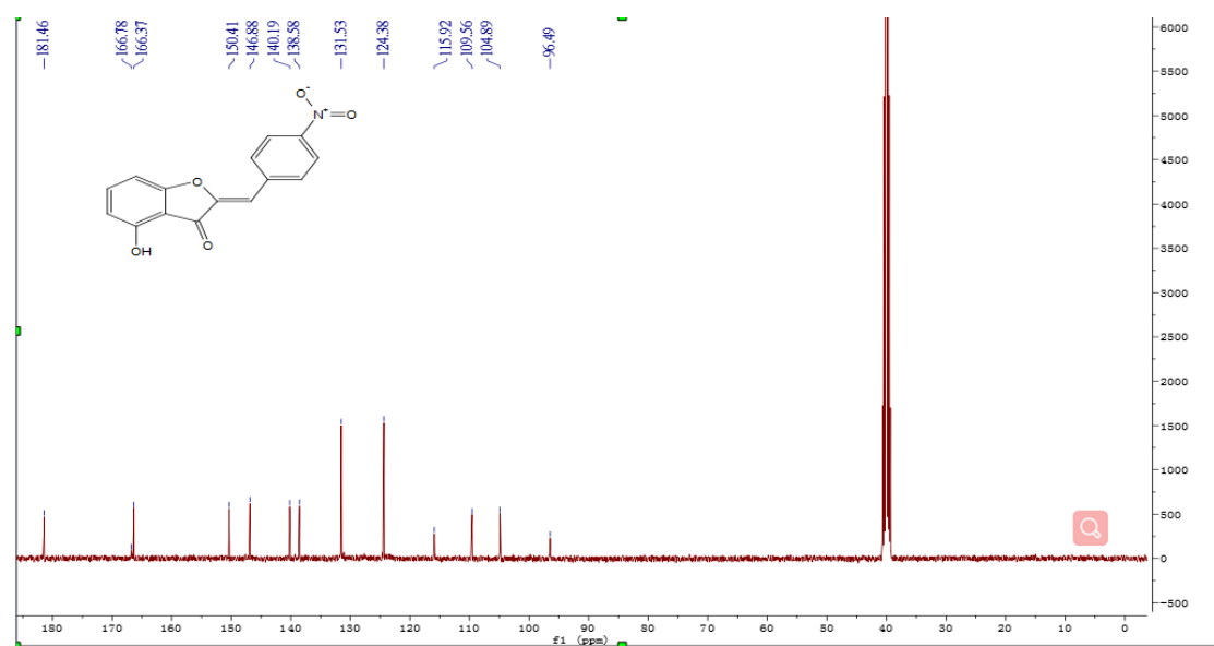
Figure S24 13 C NMR of compound 4m
