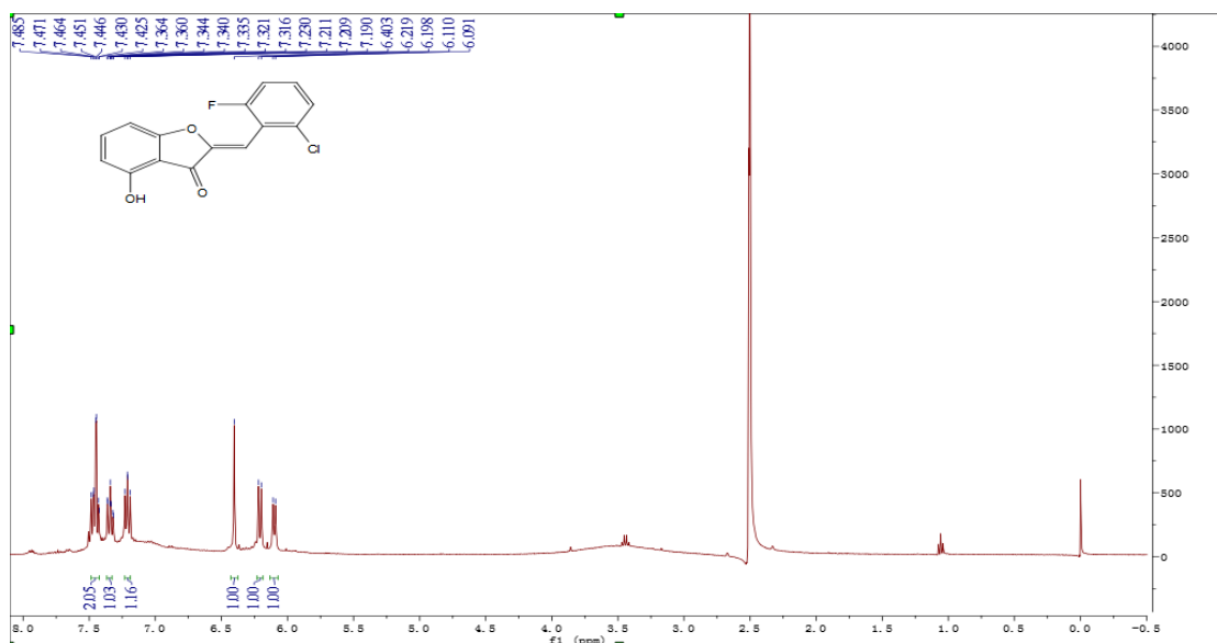
Figure S15 ^1\text{H} NMR of compound 4i
