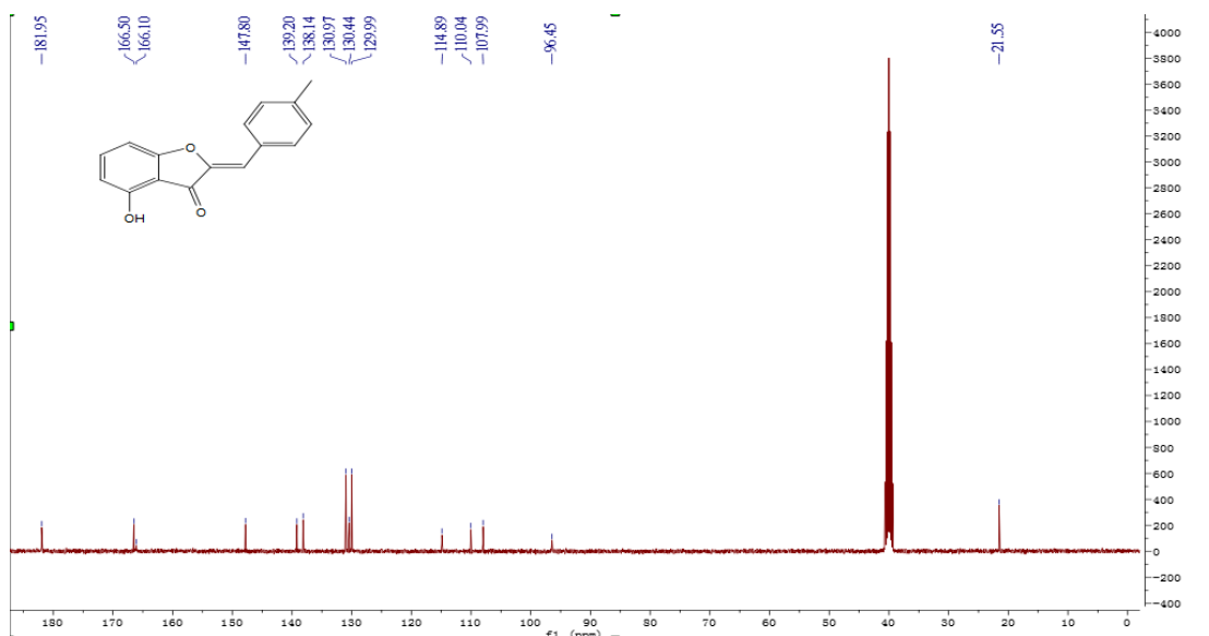
Figure S11 13 C NMR of compound 4f
