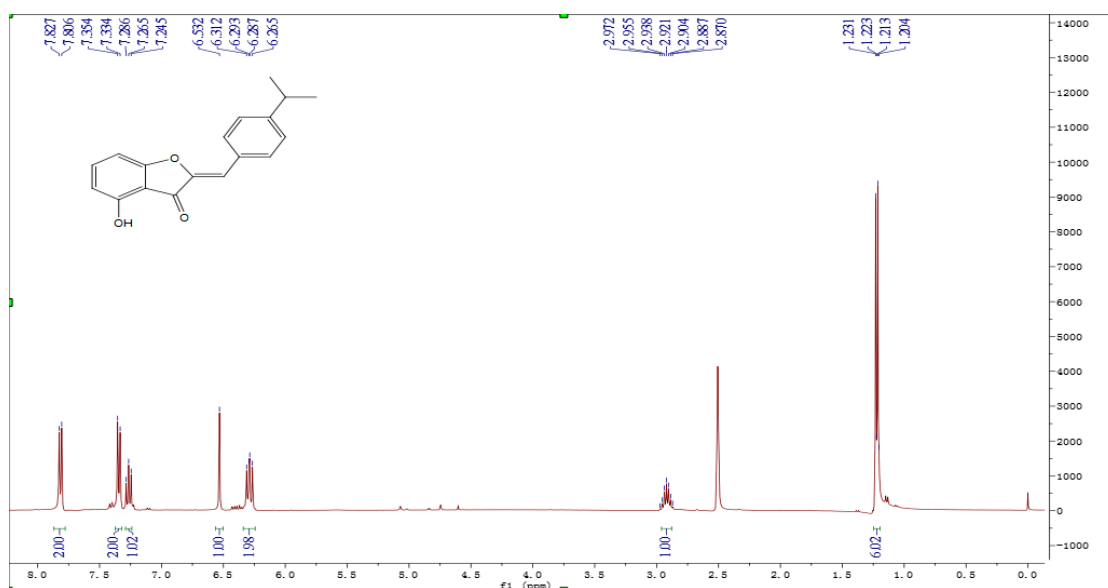
Figure S12 1 H NMR of compound 4g
