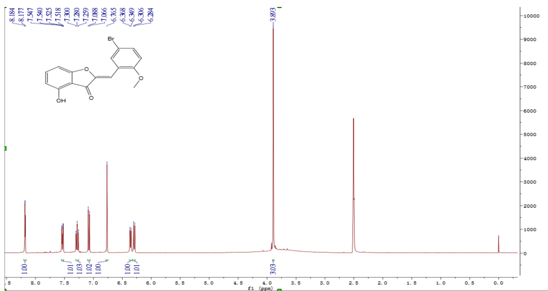
Figure S14 ^1\text{H} NMR of compound 4h
