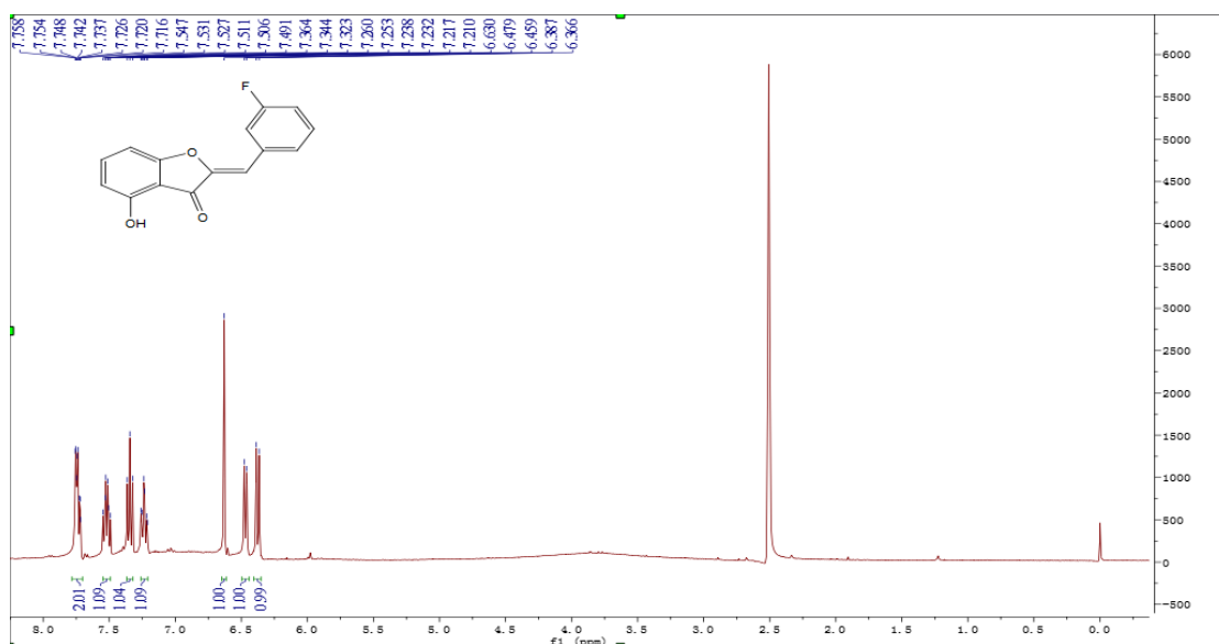
Figure S33 1 H NMR of compound 4r
