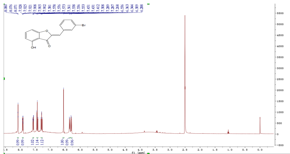
Figure S21 1 H NMR of compound 41
