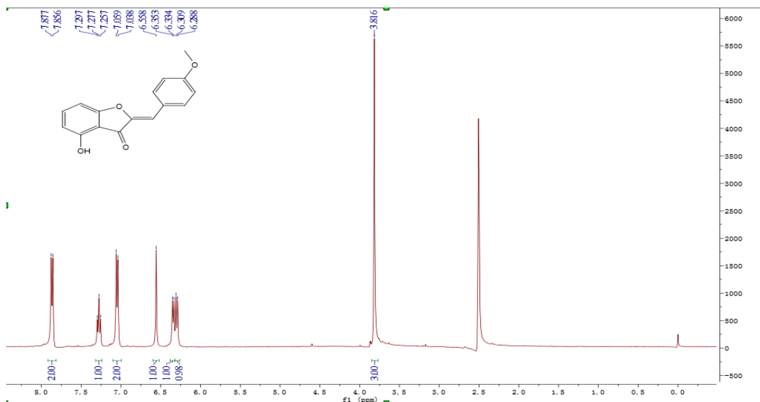
Figure S3 ^1\text{H} NMR of compound 4b
