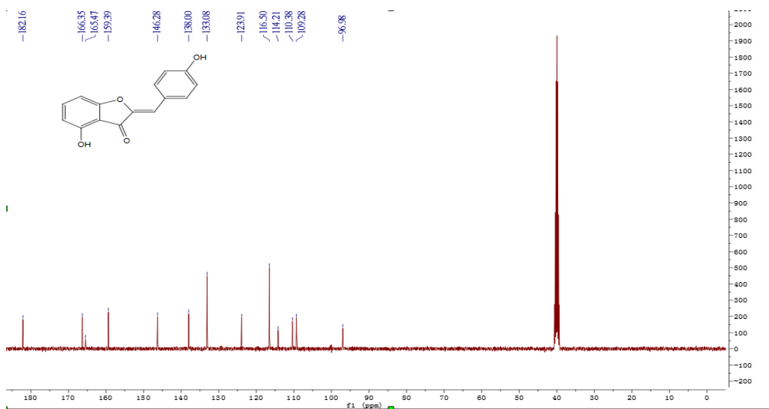
Figure S30 ^{13}\text{C} NMR of compound 4p
