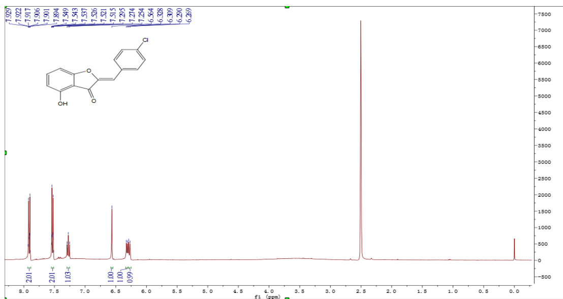
Figure S19 ^1\text{H} NMR of compound 4k
