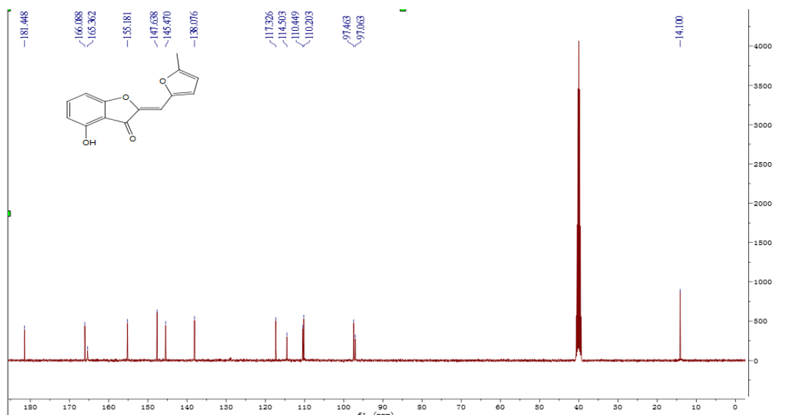
Figure S39 13 C NMR of compound 4u
