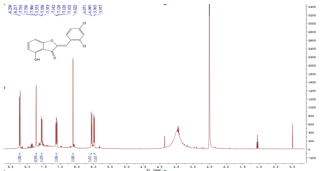
Figure S17 1 H NMR of compound 4j
