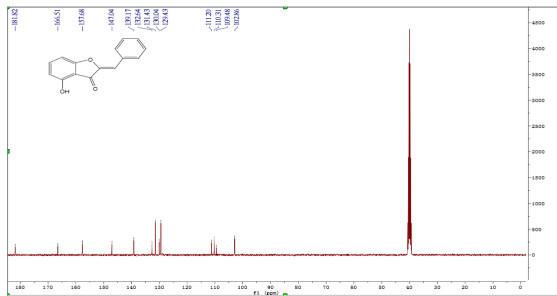
Figure S2 13 C NMR of compound 4a
