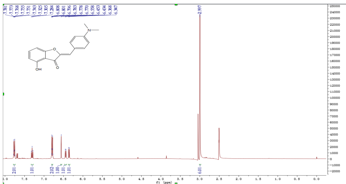
Figure S27 ^1\text{H} NMR of compound 4o
