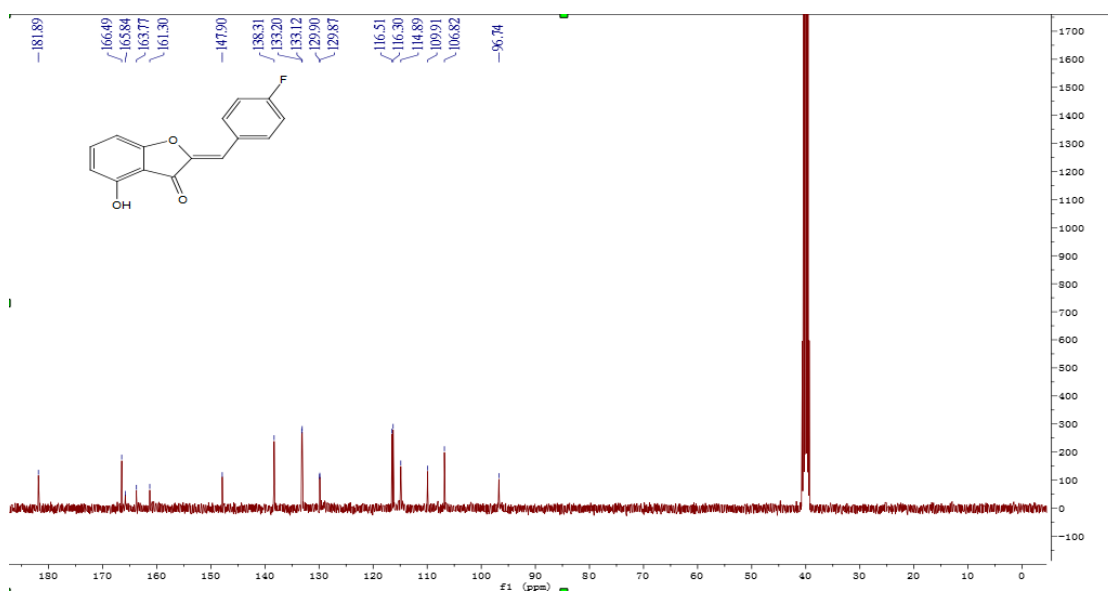
Figure S32 ^{13}\text{C} NMR of compound 4q
