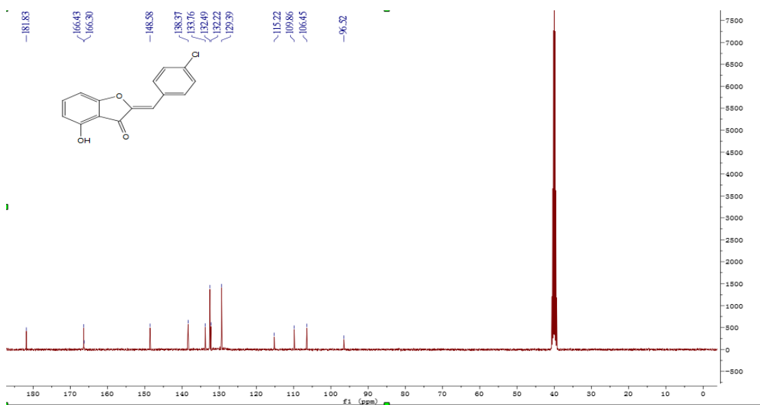
Figure S20 ^{13}\text{C} NMR of compound 4k
