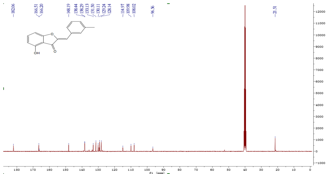
Figure S9 13 C NMR of compound 4e
