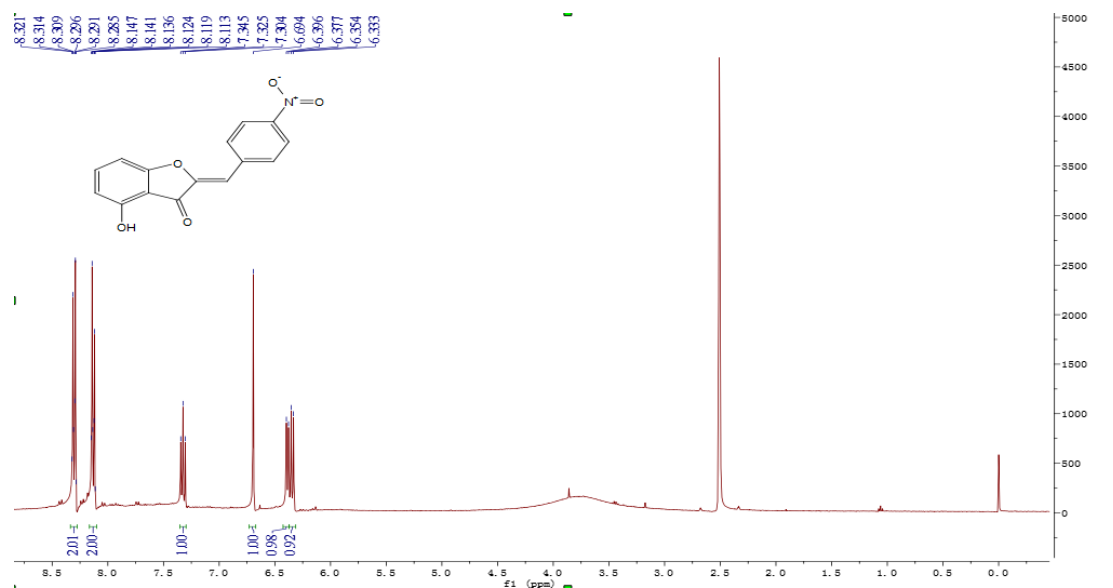
Figure S23 1 H NMR of compound 4m
