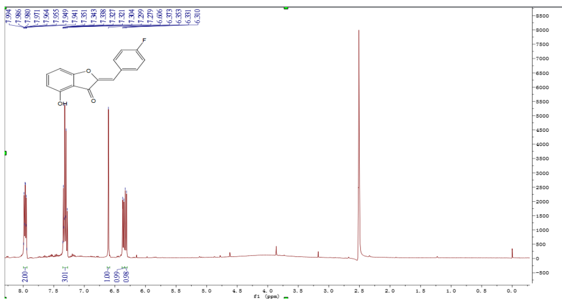
Figure S31 ^1\text{H} NMR of compound 4q
