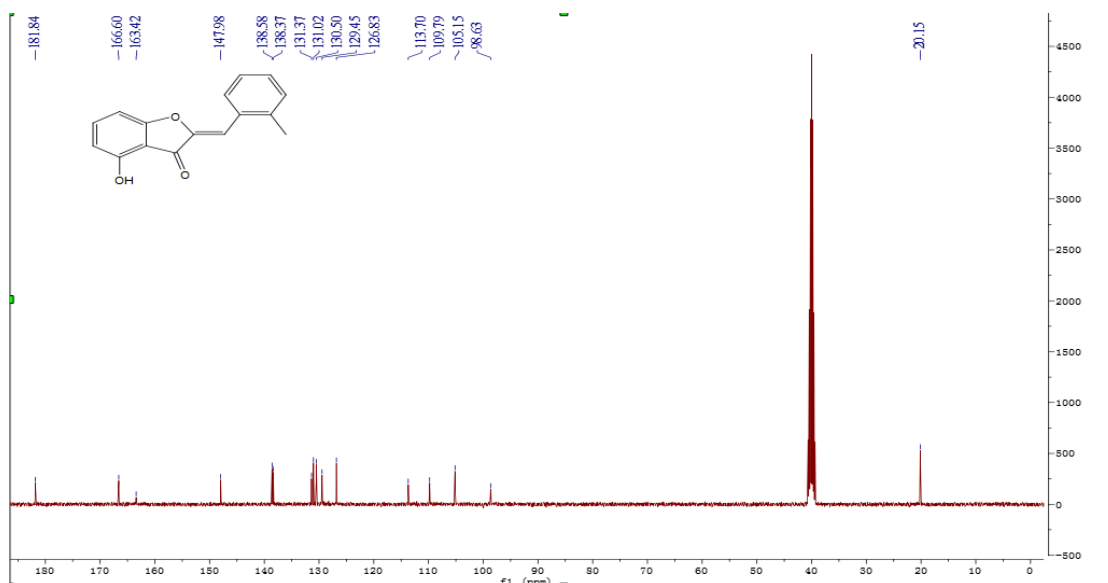
Figure S7 13 C NMR of compound 4d
