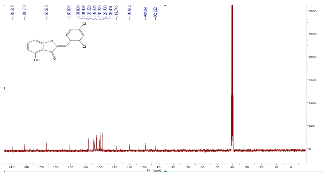
Figure S18 13 C NMR of compound 4j
