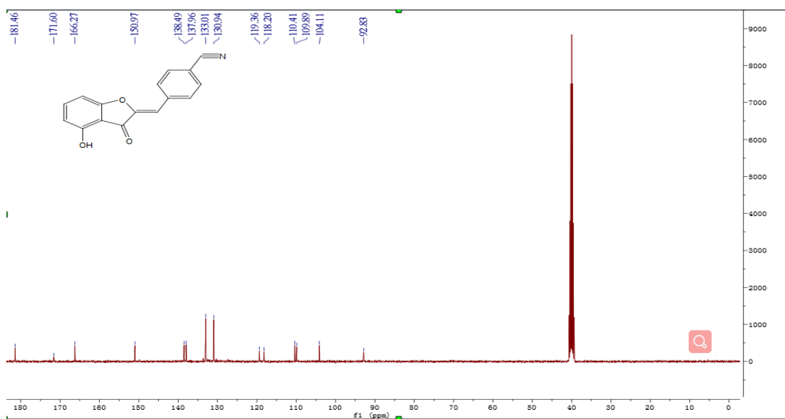
Figure S26 ^{13}\text{C} NMR of compound 4n
