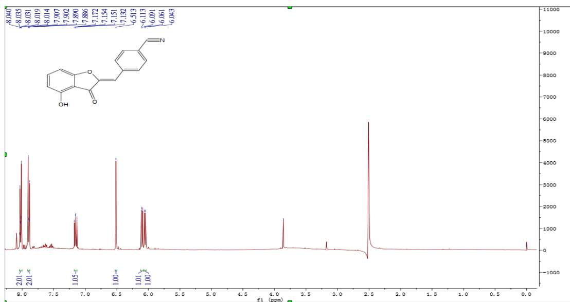
Figure S25 ^1\text{H} NMR of compound 4n
