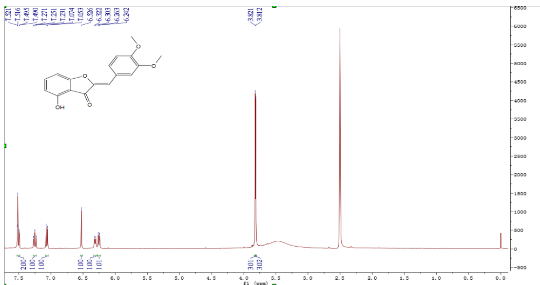
Figure S5 ^1\text{H} NMR of compound 4c
