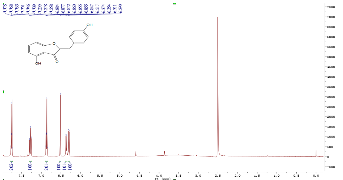
Figure S29 ^1\text{H} NMR of compound 4p
