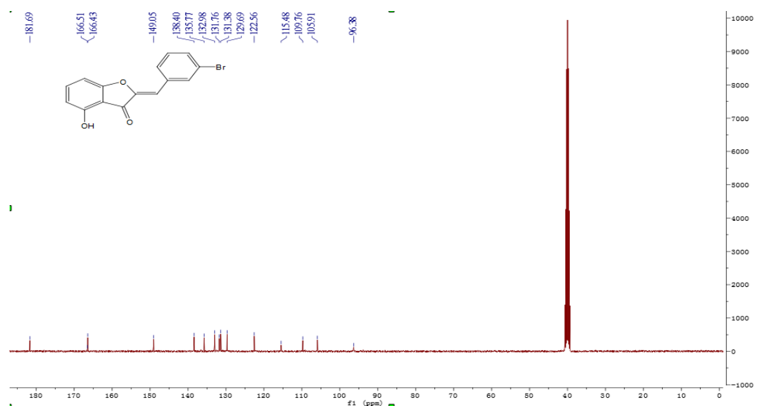
Figure S22 13 C NMR of compound 41
