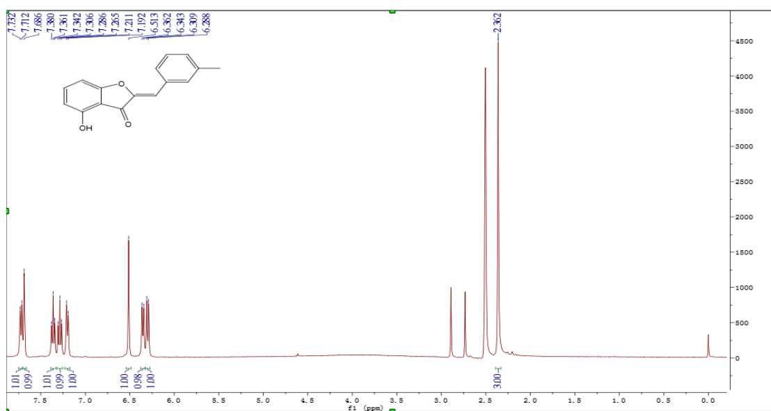
Figure S8 1 H NMR of compound 4e
