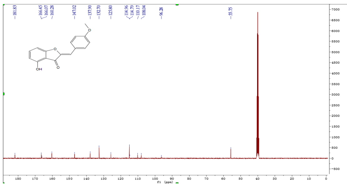
Figure S4 ^{13}\text{C} NMR of compound 4b
