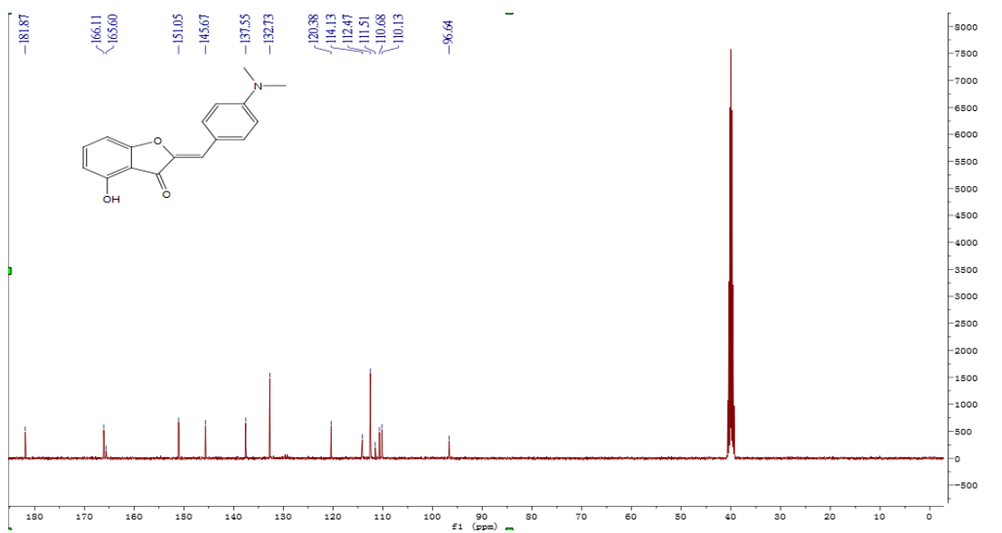
Figure S28 ^{13}\text{C} NMR of compound 4o
