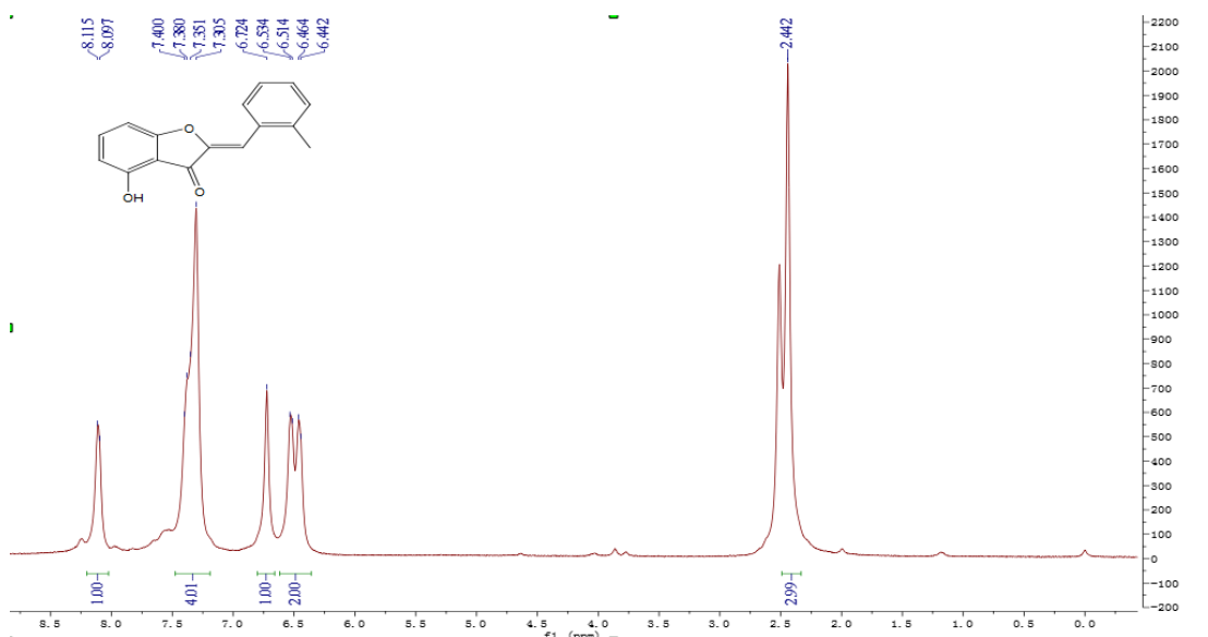
Figure S6 ^1\text{H} NMR of compound 4d
