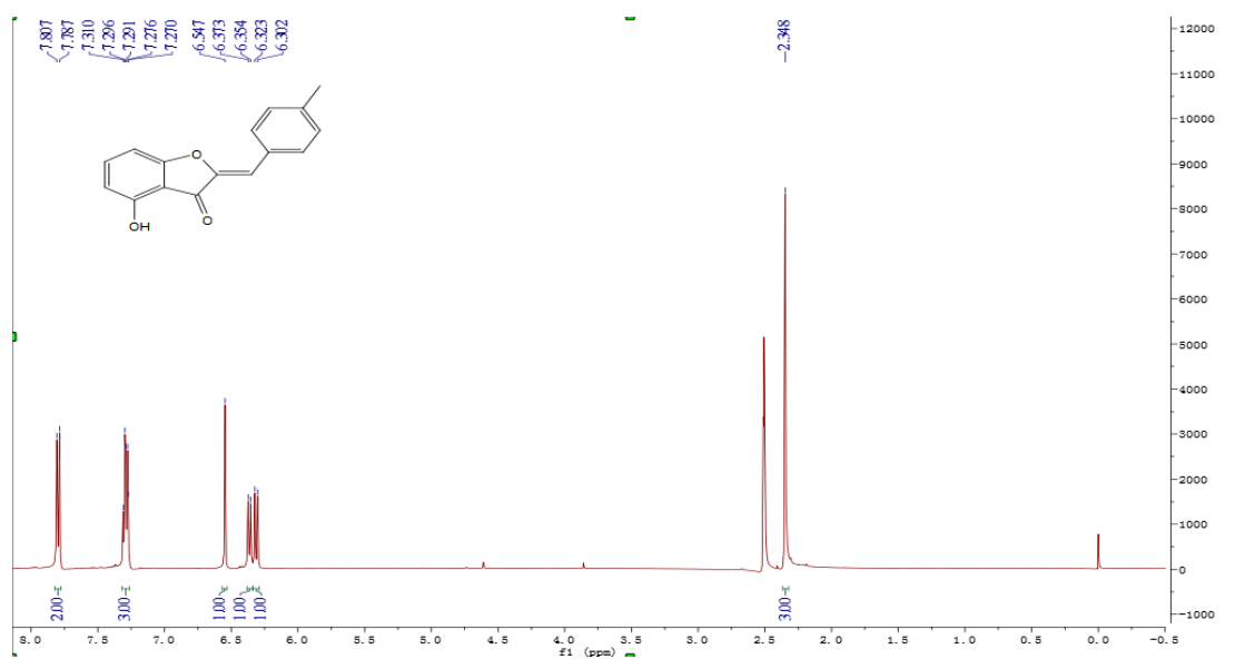
Figure S10 1 H NMR of compound 4f
