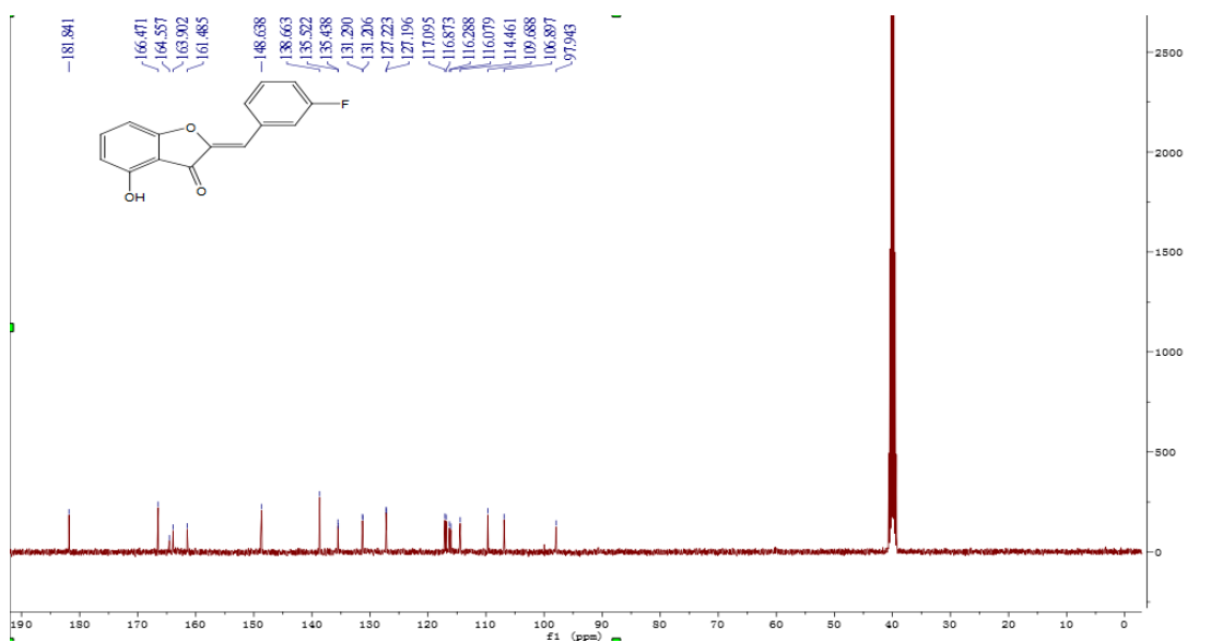
Figure S34 13 C NMR of compound 4r
