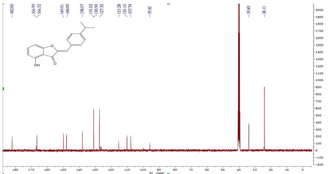
Figure S13 ^{13}\text{C} NMR of compound 4g
