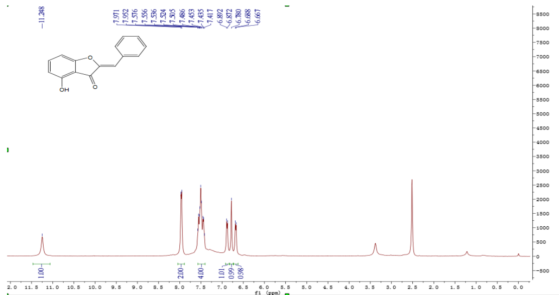
Figure S1 1 H NMR of compound 4a
