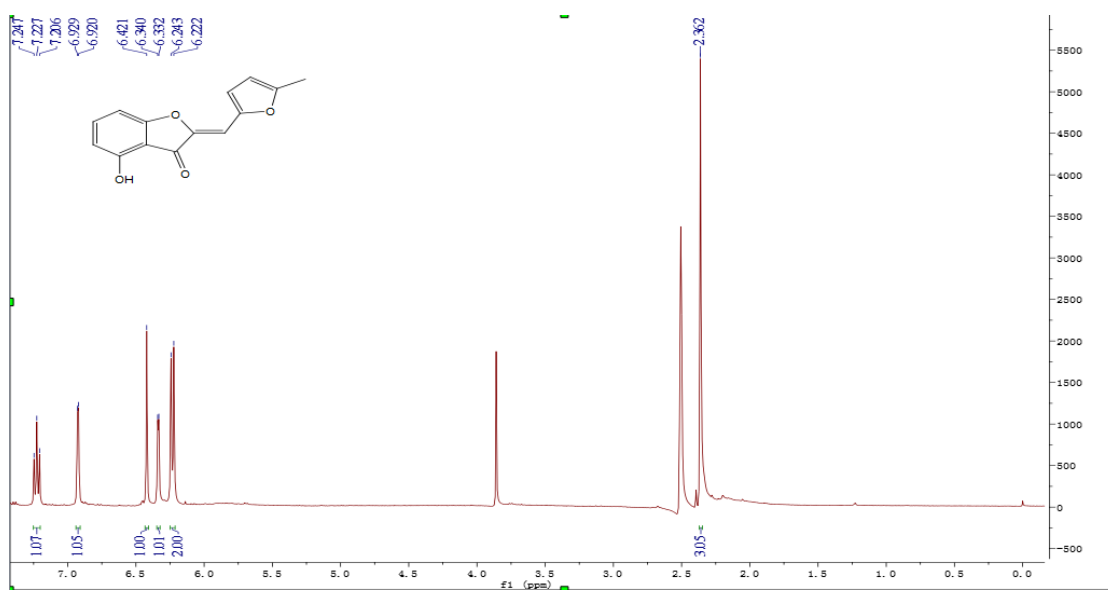
Figure S38 ^1\text{H} NMR of compound 4u
