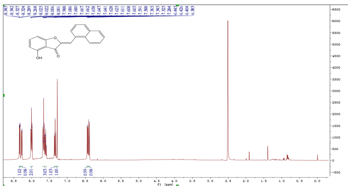
Figure S40 1 H NMR of compound 4v
