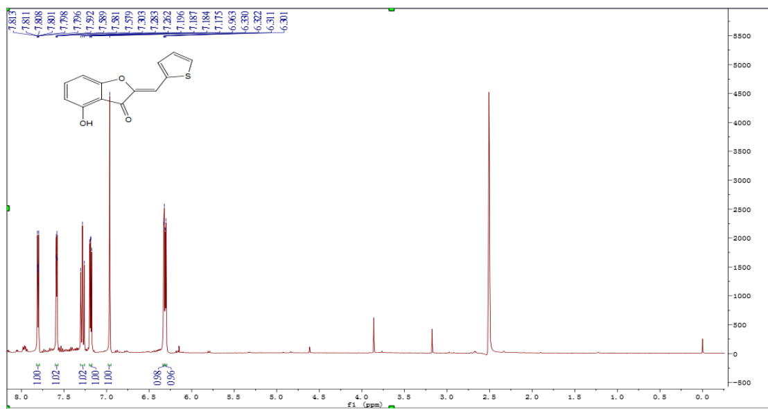
Figure S36 1 H NMR of compound 4t
