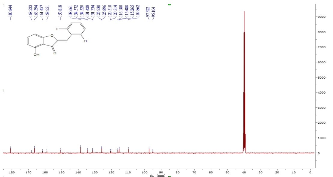
Figure S16 ^{13}\text{C} NMR of compound 4i
