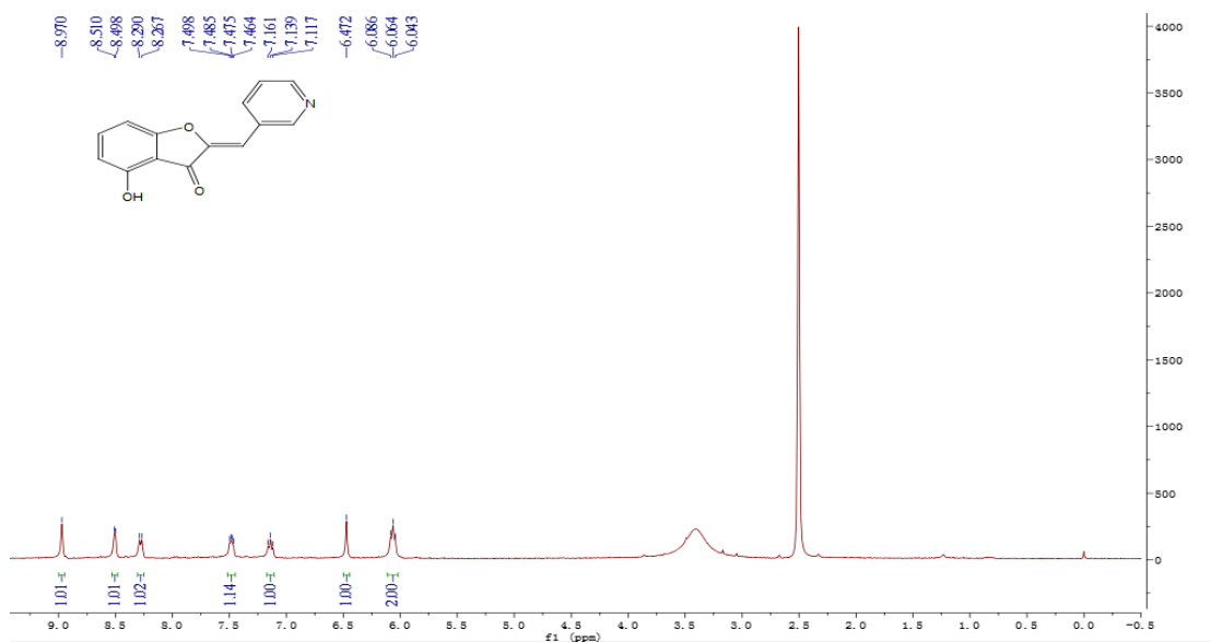
Figure S35 1 H NMR of compound 4s
