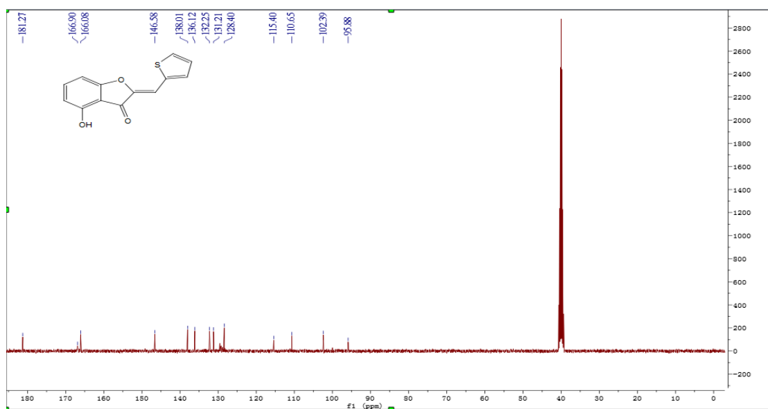
Figure S37 ^{13}\text{C} NMR of compound 4t
