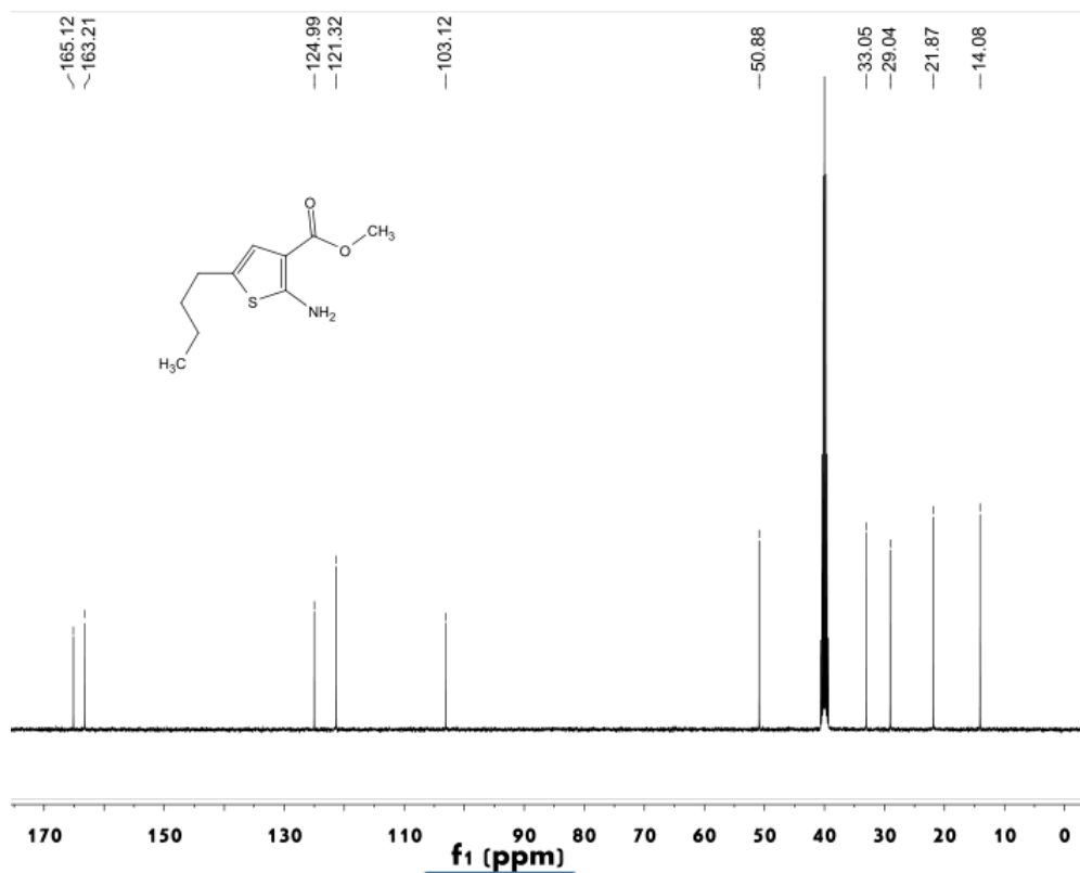
Figure S11 ^{13}\text{C} NMR spectrum of compound 3d
