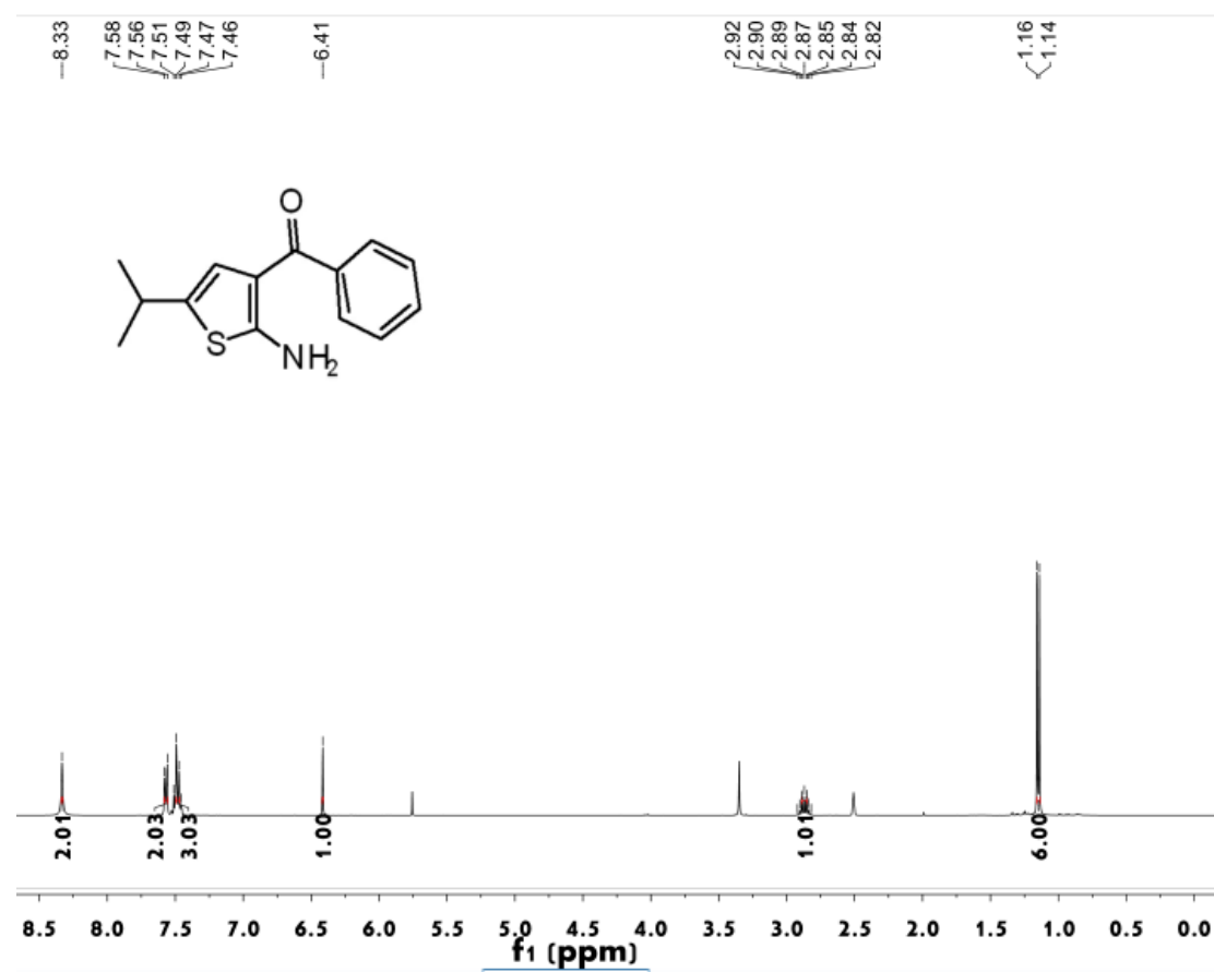
Figure S52 1 H NMR spectrum of compound 4d
