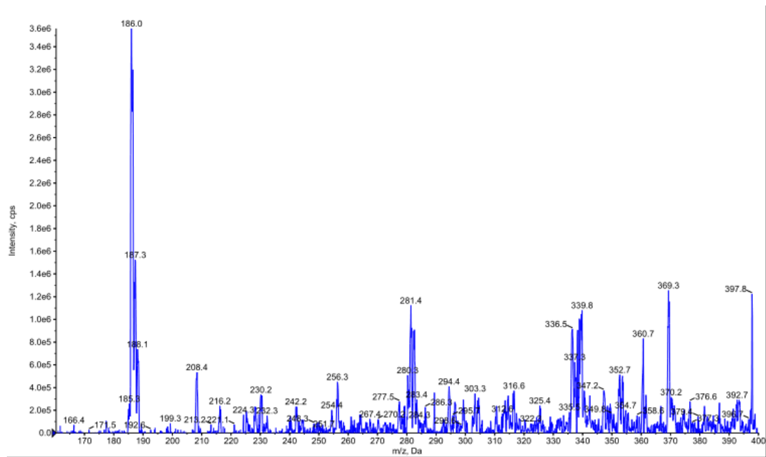
Figure S3 mass spectrum of compound 3a
