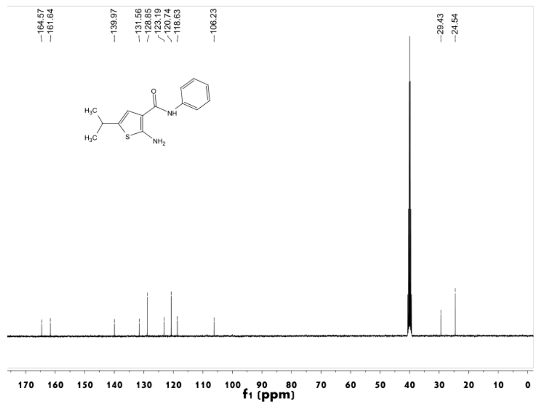
Figure S62 13 C NMR spectrum of compound 4g
