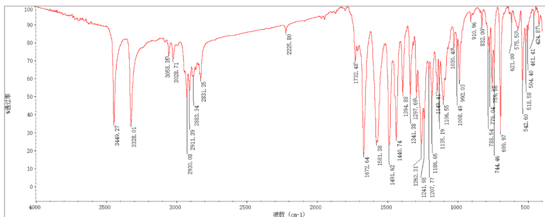
Figure S37 IR spectrum of compound 31
