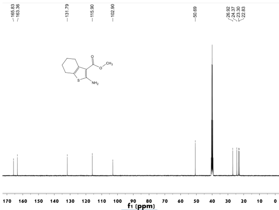
Figure S23 ^{13}\text{C} NMR spectrum of compound 3h
