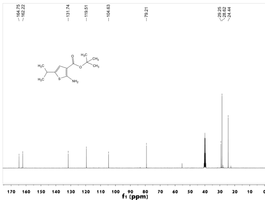
Figure S59 ^{13}\text{C} NMR spectrum of compound 4f
