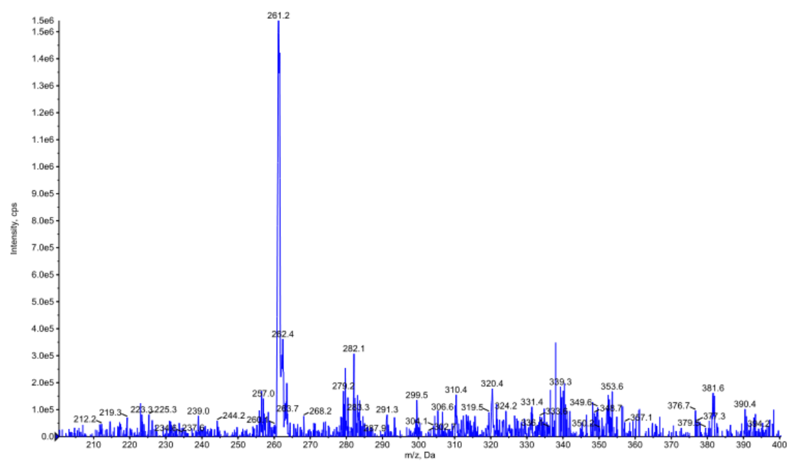
Figure S63 mass spectrum of compound 4g
