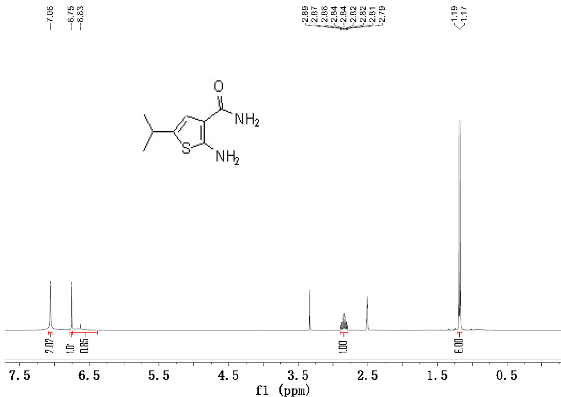
Figure S49 ^1\text{H} NMR spectrum of compound 4c
