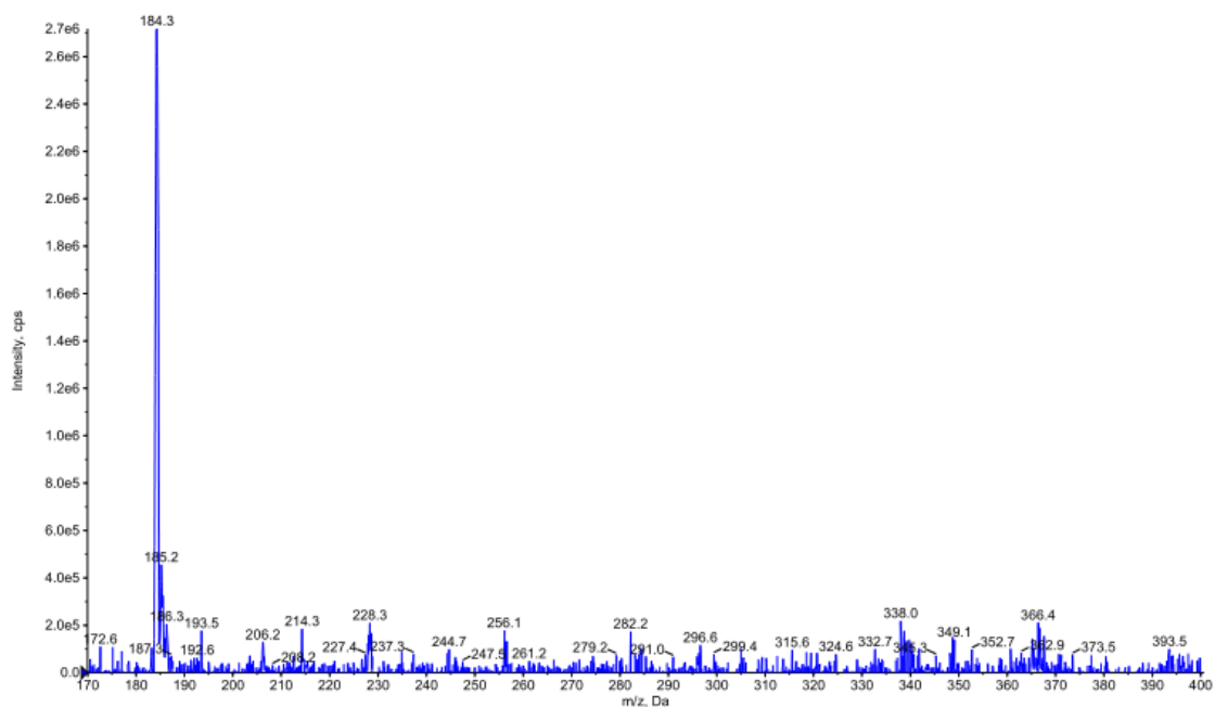
Figure S57 mass spectrum of compound 4e
