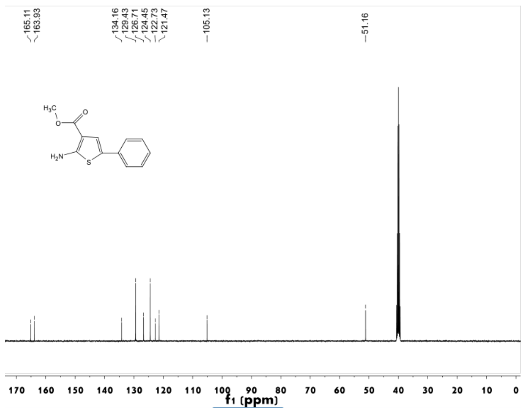
Figure S14 ^{13}\text{C NMR} spectrum of compound 3e
