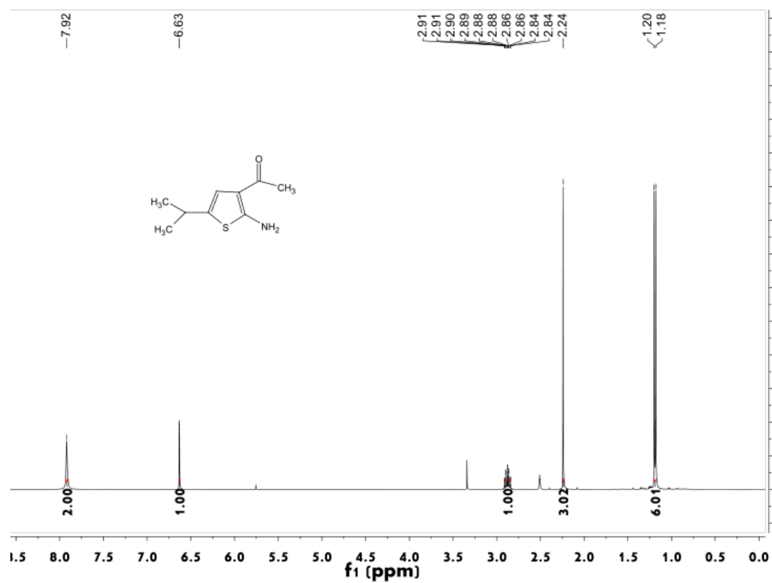
Figure S55 1 H NMR spectrum of compound 4e
