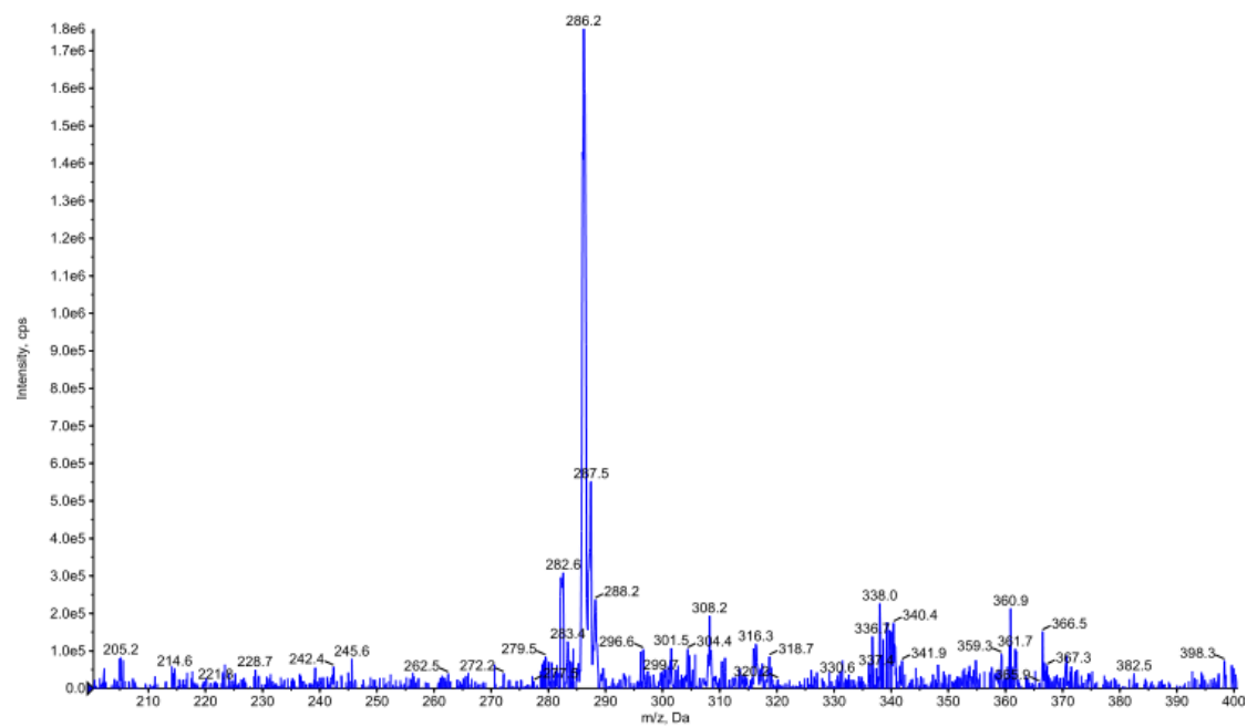
Figure S83 mass spectrum of compound 4m
