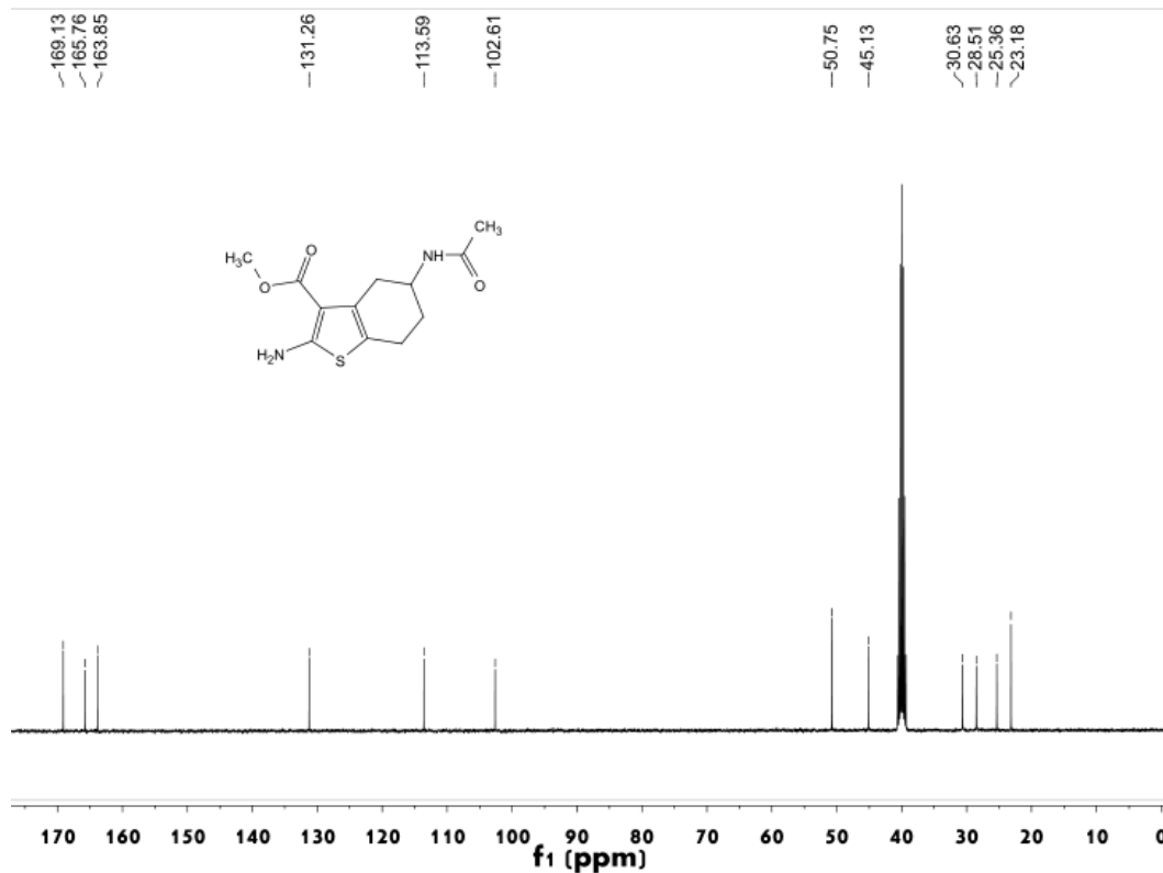
Figure S32 ^{13}\text{C} NMR spectrum of compound 3k
