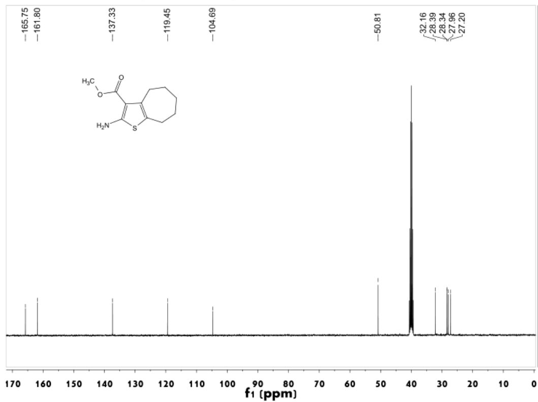
Figure S26 ^{13}\text{C NMR} spectrum of compound 3i
