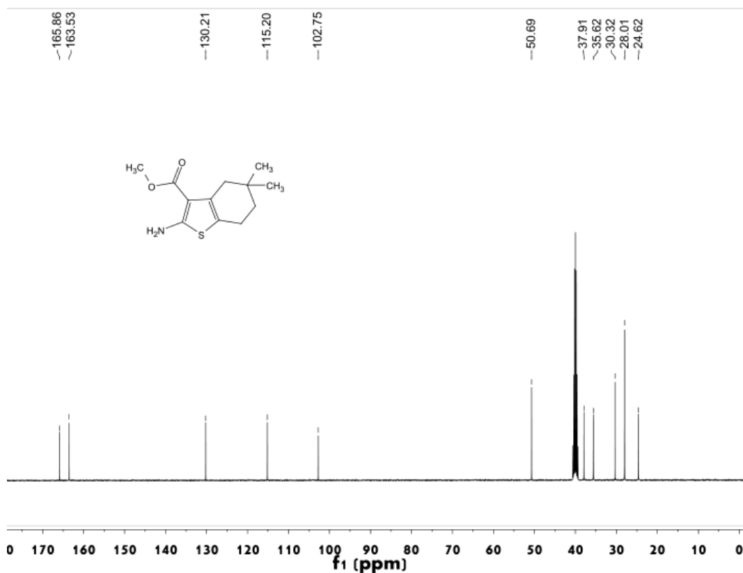
Figure S29 13 C NMR spectrum of compound 3j
