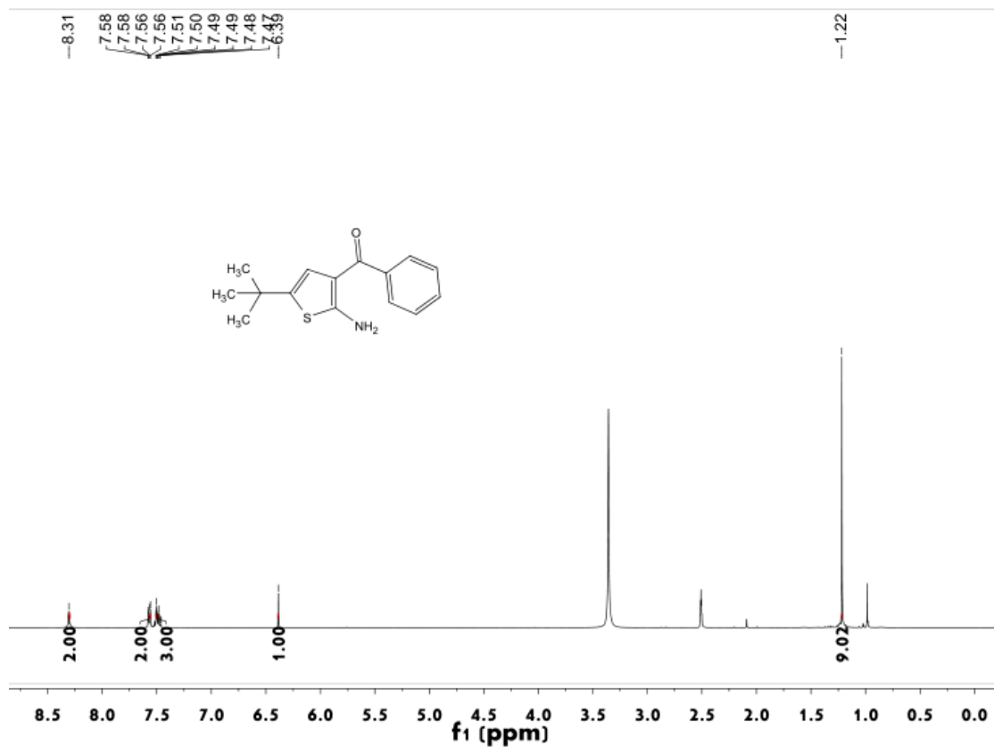
Figure S71 ^1\text{H} NMR spectrum of compound 4j
