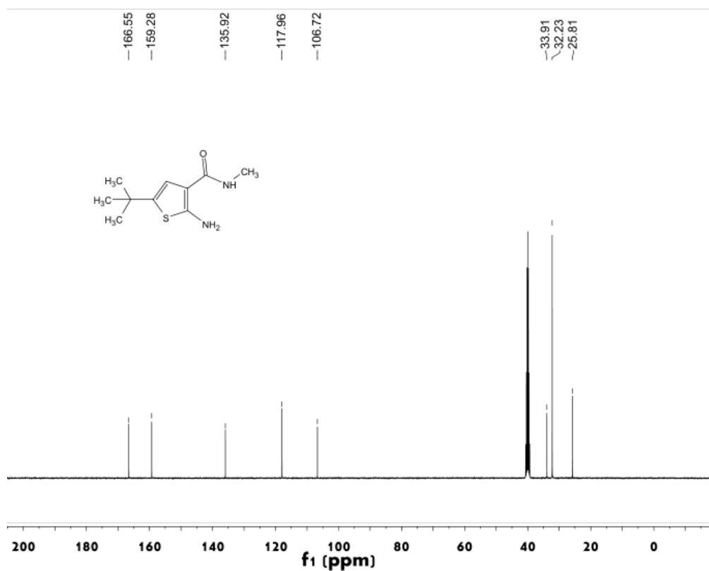
Figure S69 13 C NMR spectrum of compound 4i
