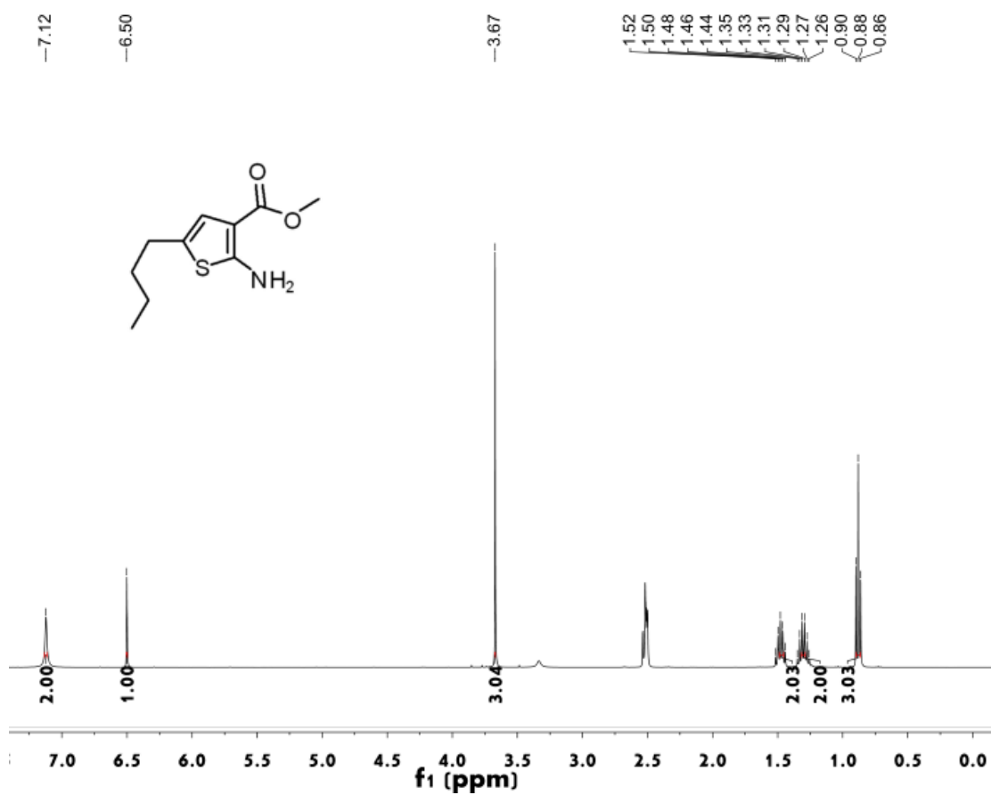
Figure S10 ^1\text{H} NMR spectrum of compound 3d
