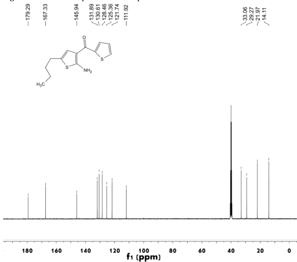
Figure S88 13 C NMR spectrum of compound 4o
