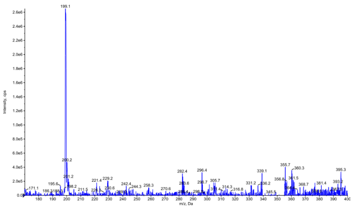
Figure S48 mass spectrum of compound 4b
