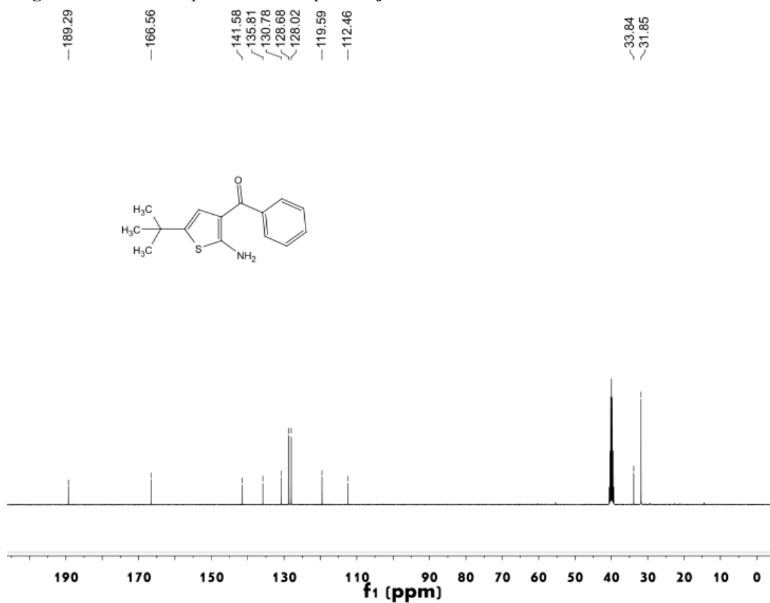
Figure S72 ^{13}\text{C} NMR spectrum of compound 4j
