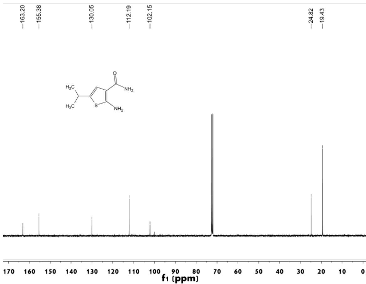
Figure S50 ^{13}\text{C} NMR spectrum of compound 4c
