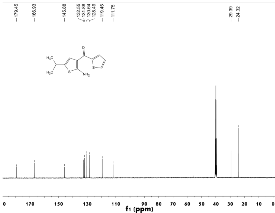
Figure S65 ^{13}\text{C} NMR spectrum of compound 4h
