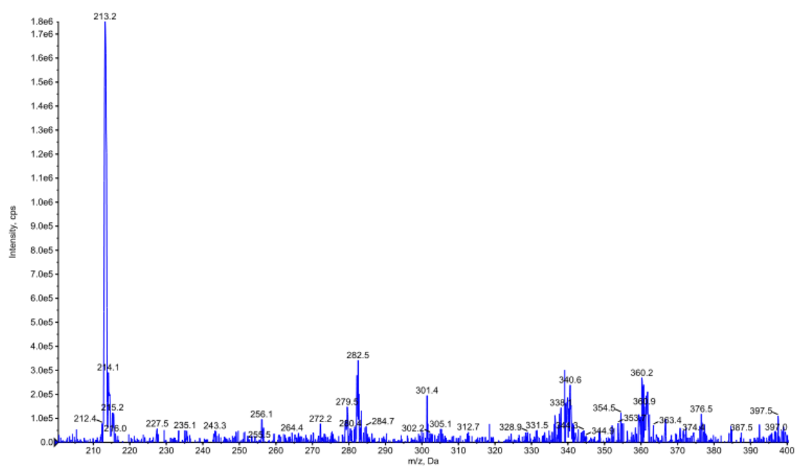
Figure S70 mass spectrum of compound 4i
