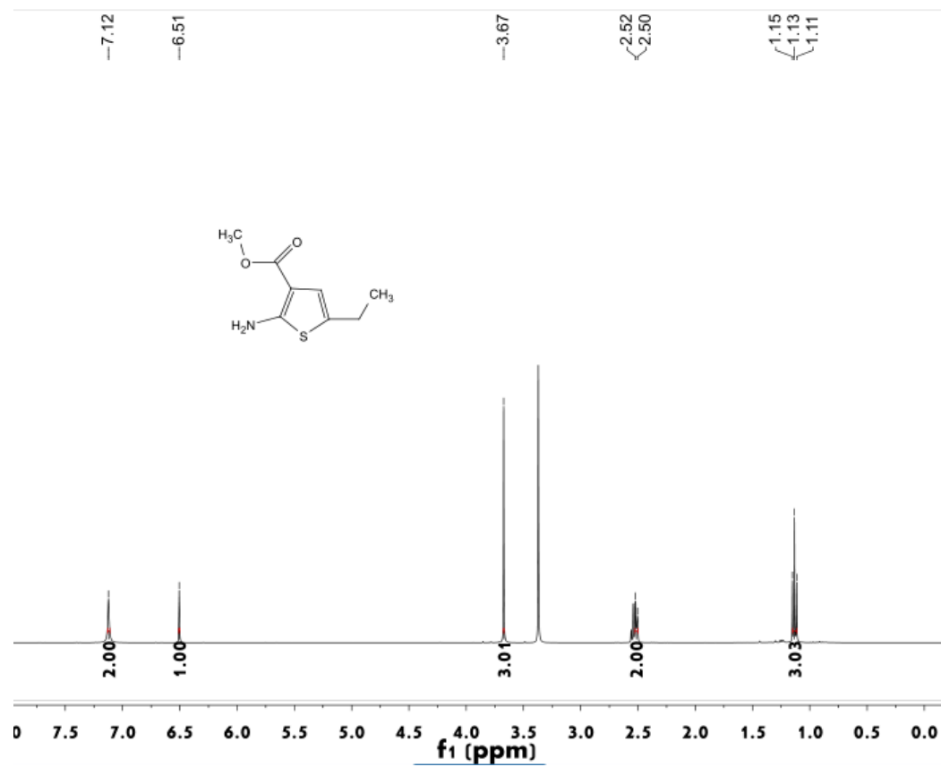
Figure S1 1 H NMR spectrum of compound 3a
