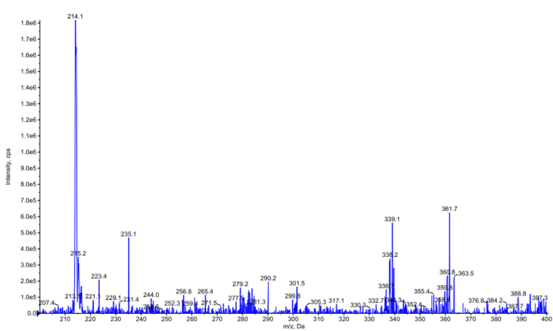
Figure S9 mass spectrum of compound 3c
