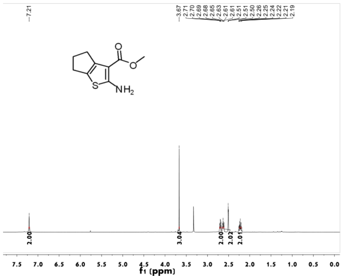
Figure S19 ^1\text{H} NMR spectrum of compound 3g
