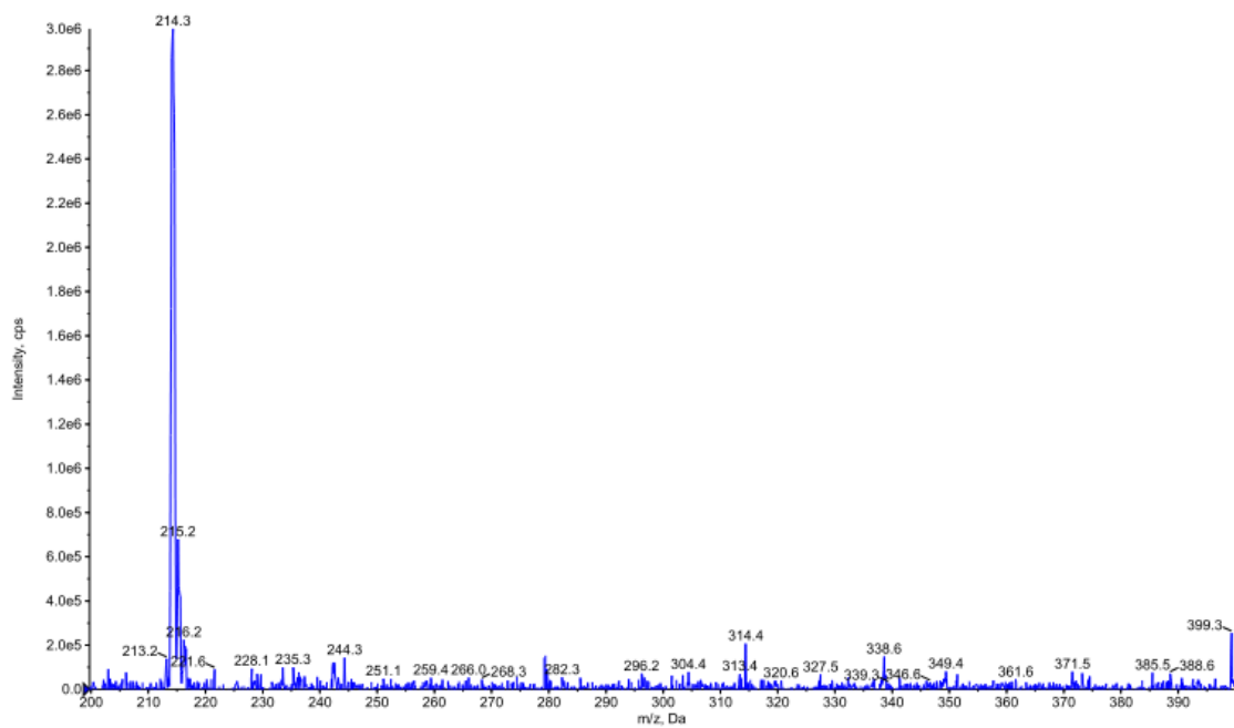
Figure S45 mass spectrum of compound 4a
