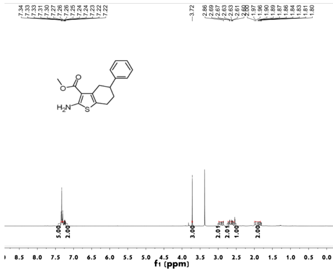
Figure S35 ^1\text{H NMR} spectrum of compound 31
