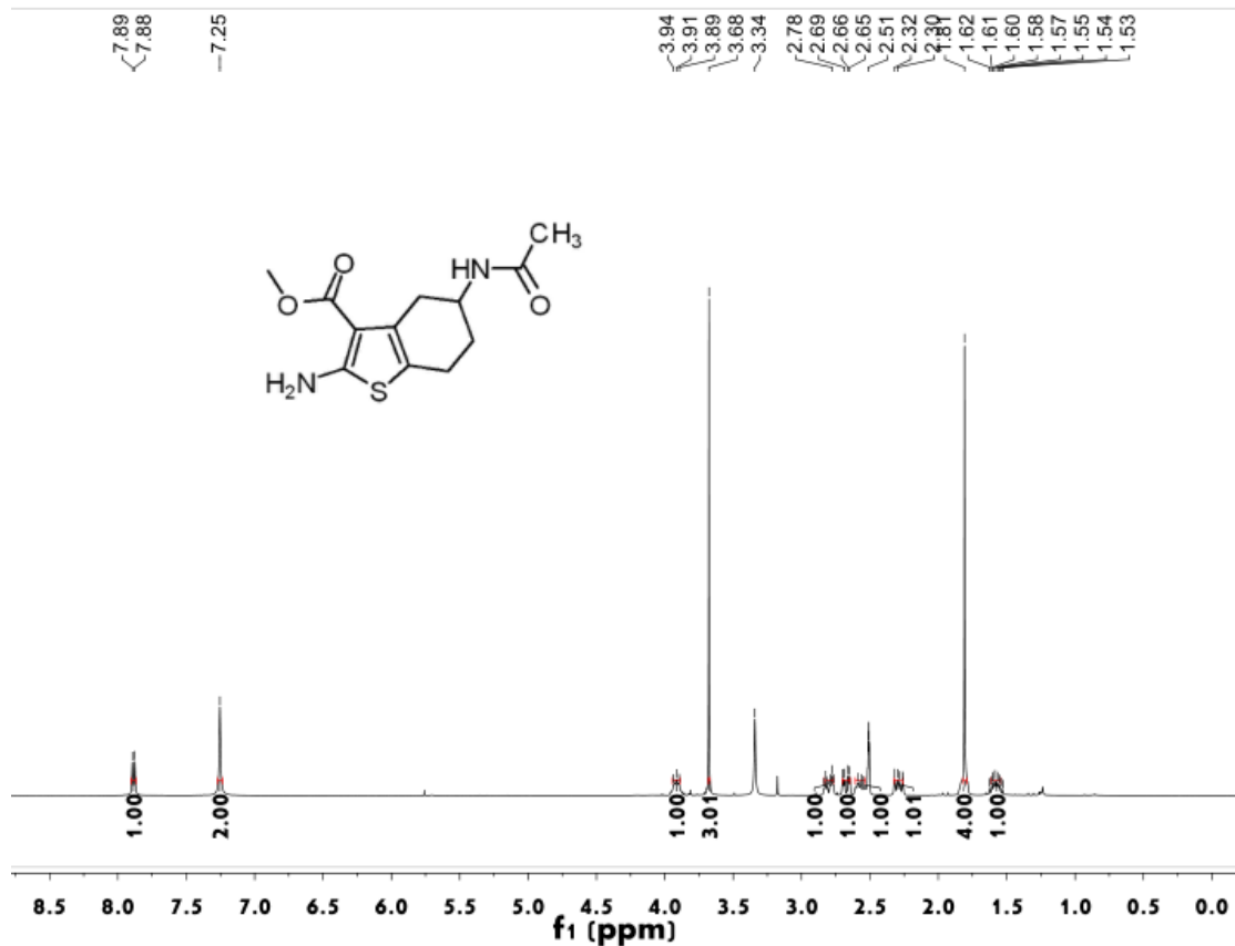
Figure S31 ^1\text{H} NMR spectrum of compound 3k
