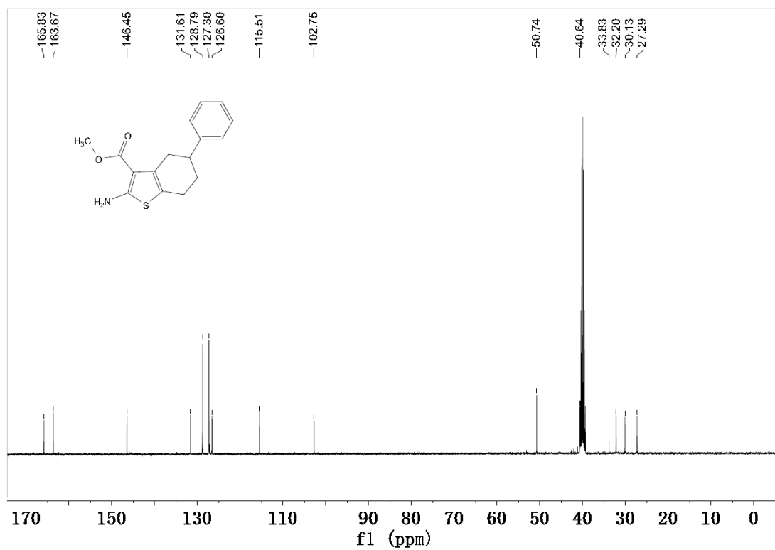
Figure S36 ^{13}\text{C NMR} spectrum of compound 31
