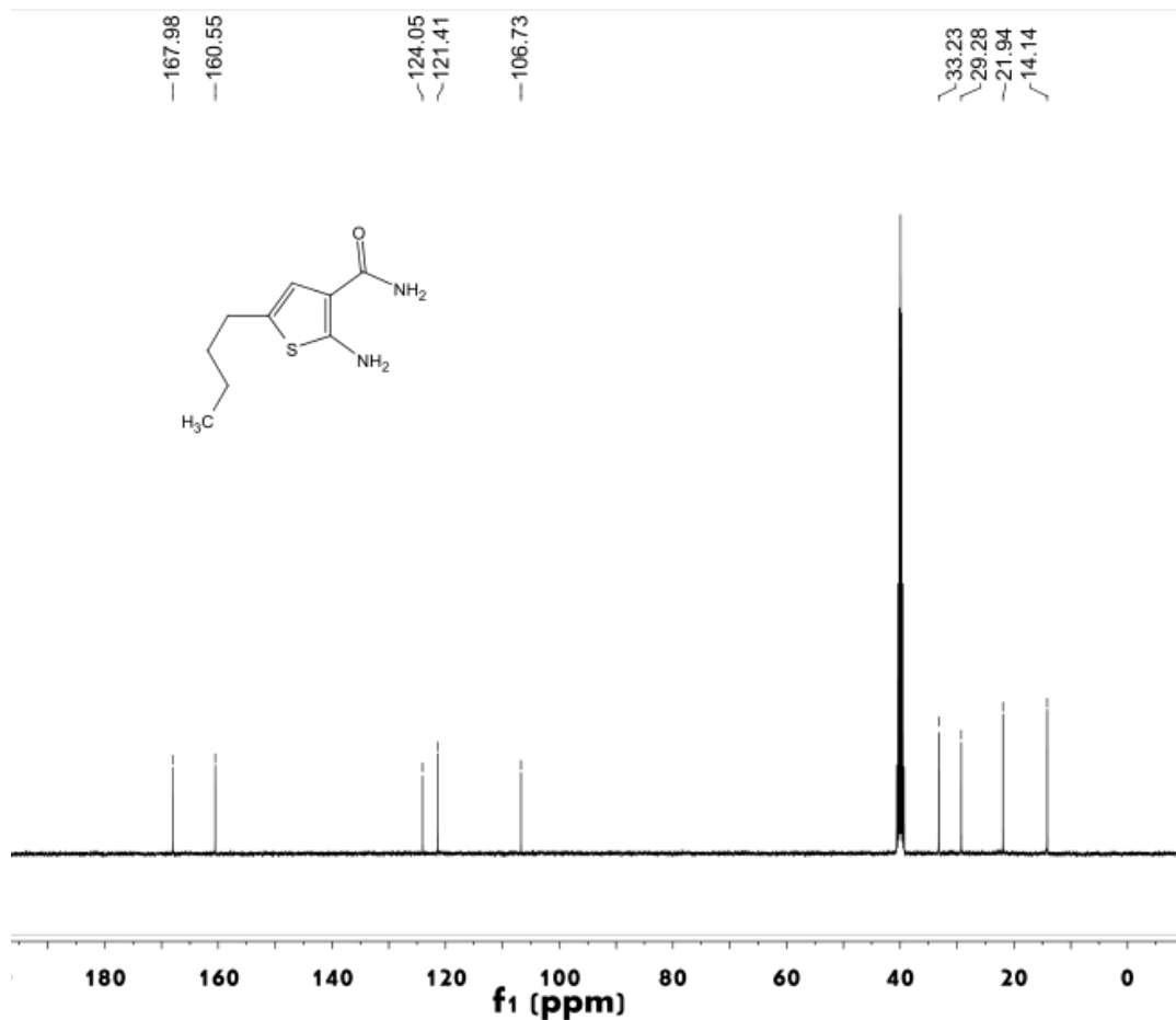
Figure S85 ^{13}\text{C} NMR spectrum of compound 4n
