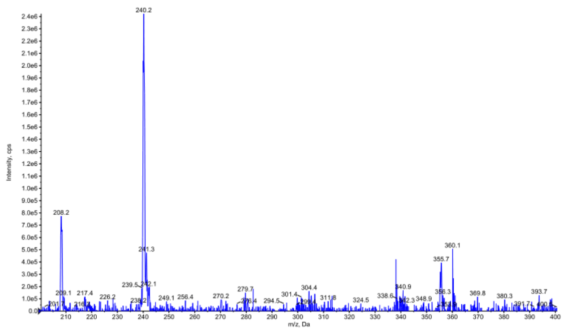
Figure S30 mass spectrum of compound 3j
