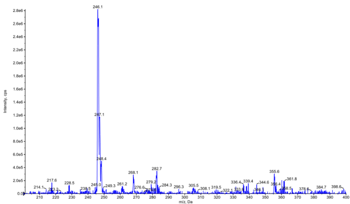
Figure S54 mass spectrum of compound 4d
