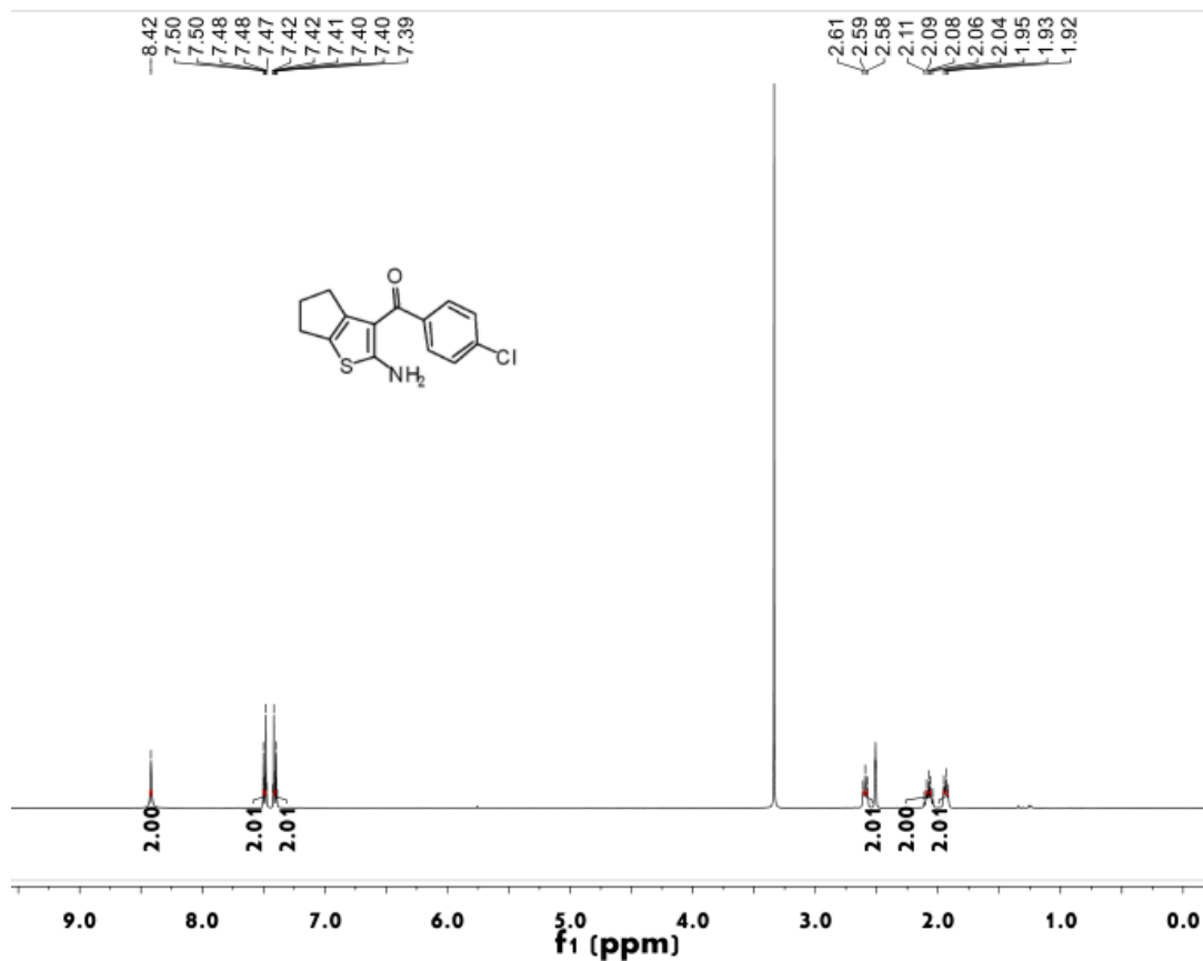
Figure S91 ^1\text{H} NMR spectrum of compound 4p
