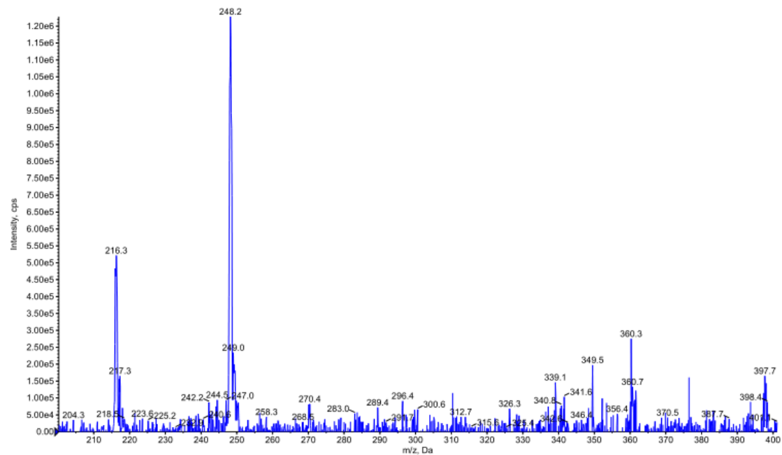
Figure S18 mass spectrum of compound 3f
