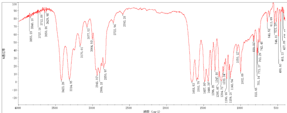
Figure S41 IR spectrum of compound 3m
