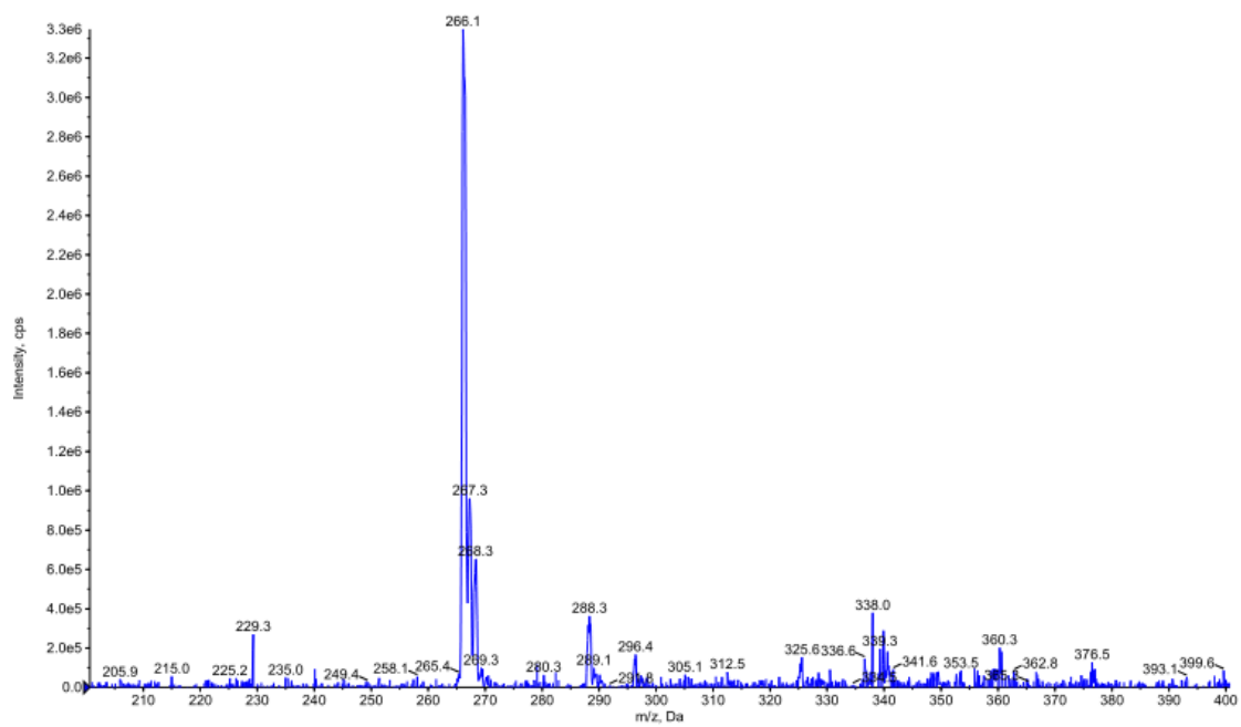
Figure S77 mass spectrum of compound 4k
