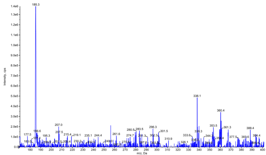
Figure S51 mass spectrum of compound 4c
