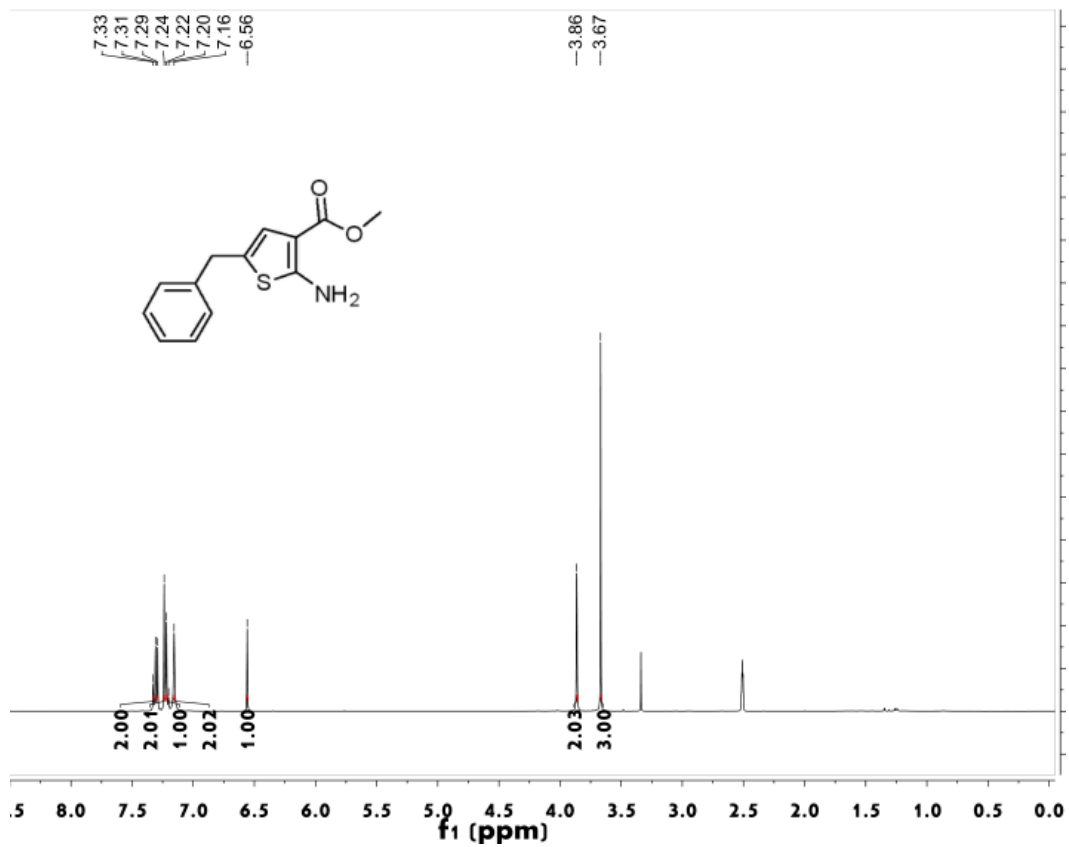
Figure S16 1 H NMR spectrum of compound 3f
