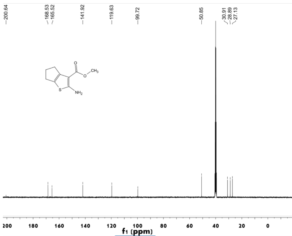
Figure S20 ^{13}\text{C} NMR spectrum of compound 3g
