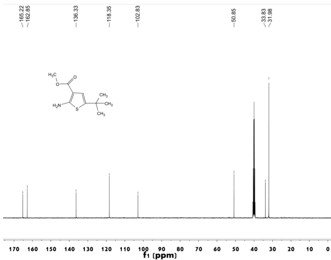
Figure S8 ^{13}\text{C} NMR spectrum of compound 3c
