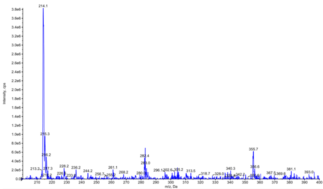
Figure S12 mass spectrum of compound 3d
