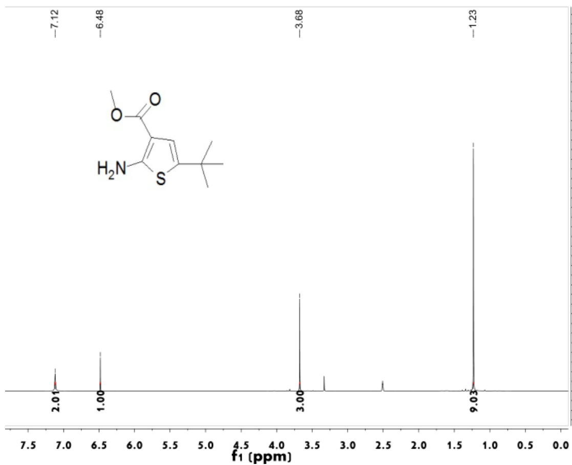
Figure S7 ^1\text{H} NMR spectrum of compound 3c
