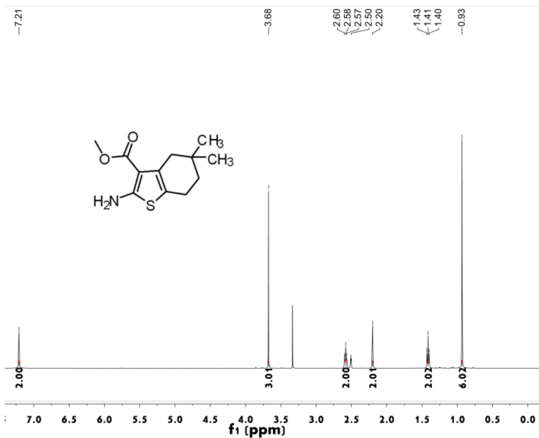
Figure S28 ^1\text{H} NMR spectrum of compound 3j
