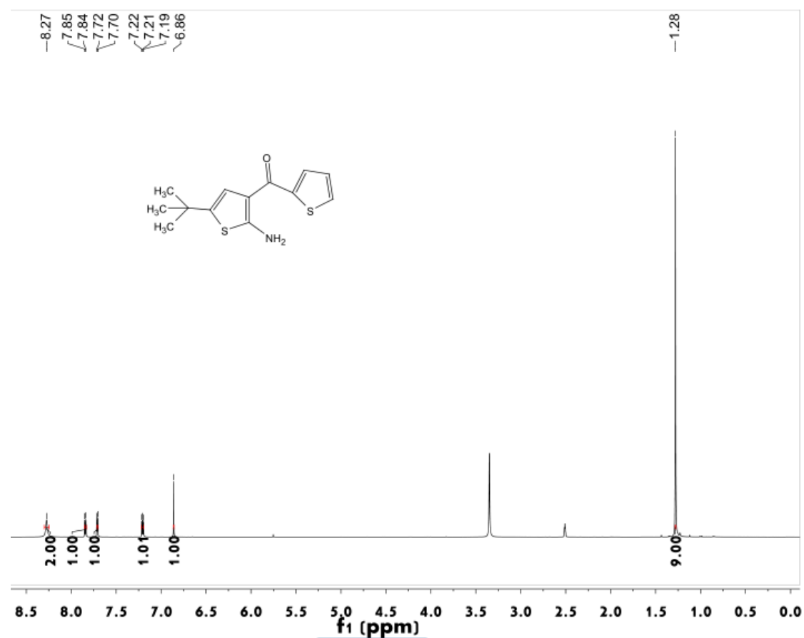
Figure S74 1 H NMR spectrum of compound 4k
