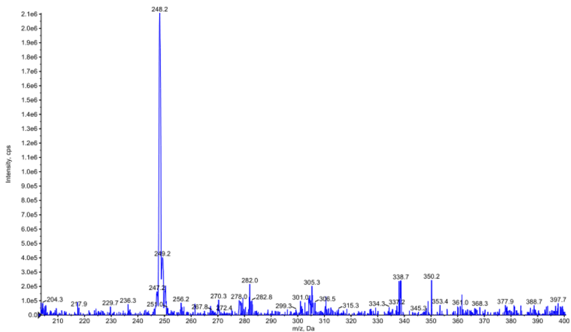
Figure S80 mass spectrum of compound 4l
