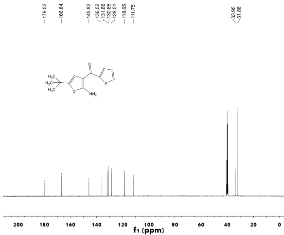
Figure S75 ^{13}\text{C} NMR spectrum of compound 4k
