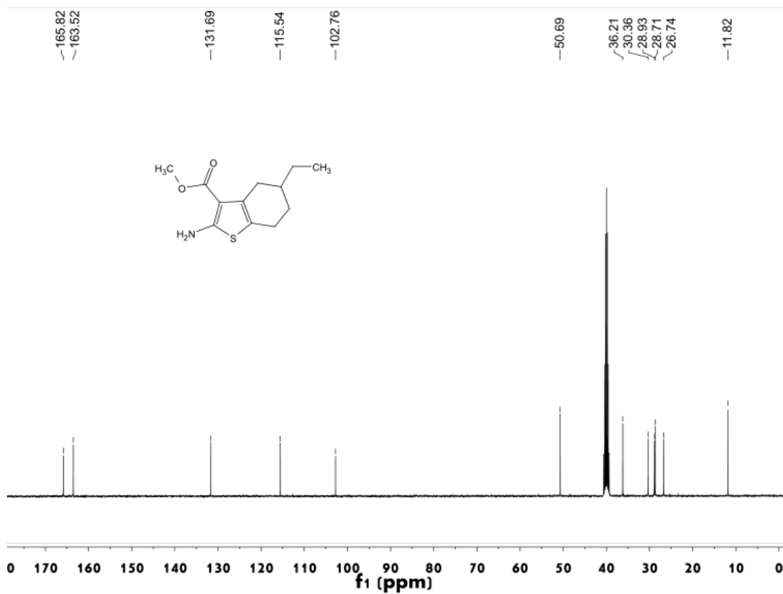
Figure S40 ^{13}\text{C} NMR spectrum of compound 3m
