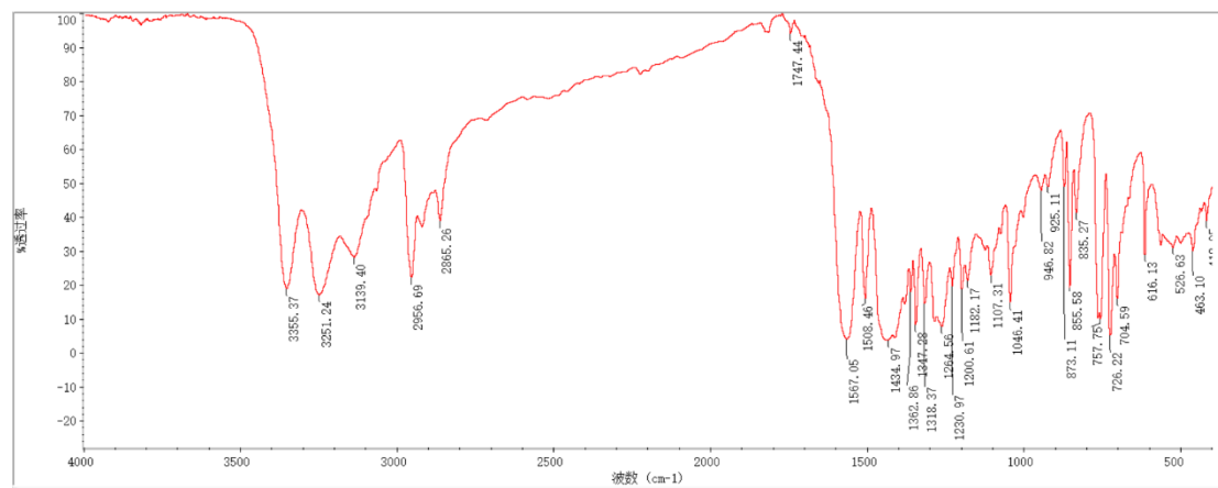
Figure S66 IR spectrum of compound 4h
