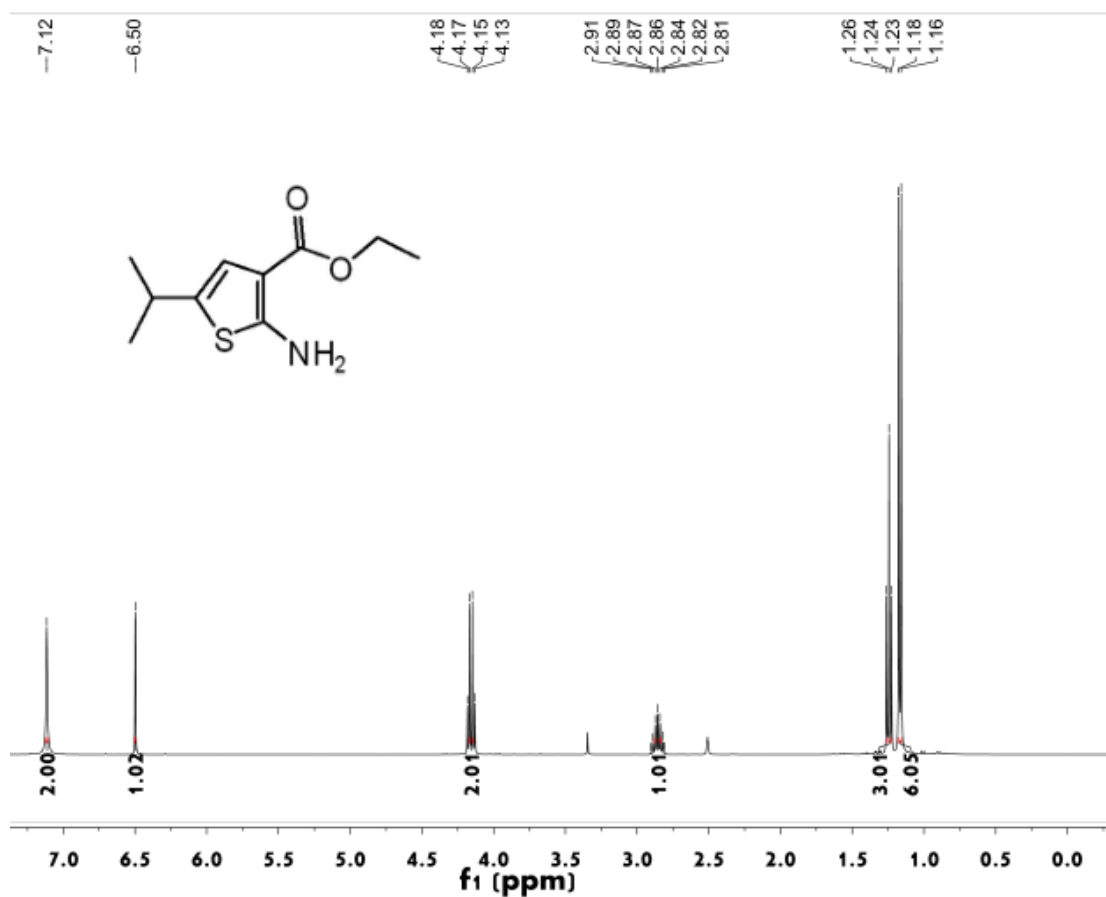
Figure S43 1 H NMR spectrum of compound 4a
