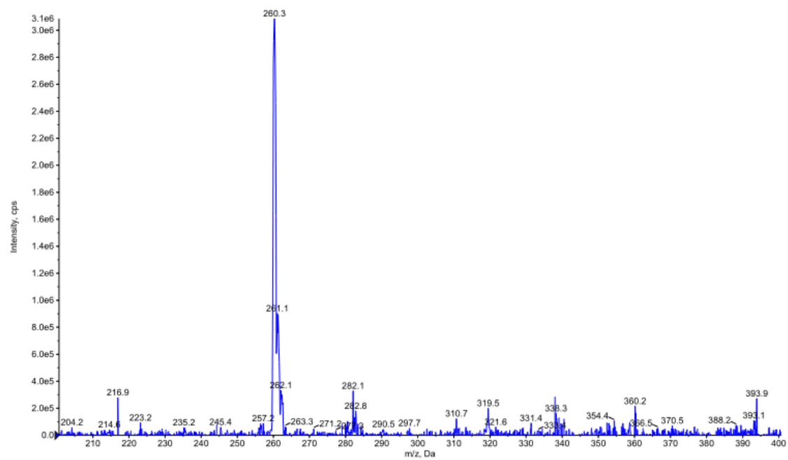
Figure S73 mass spectrum of compound 4j
