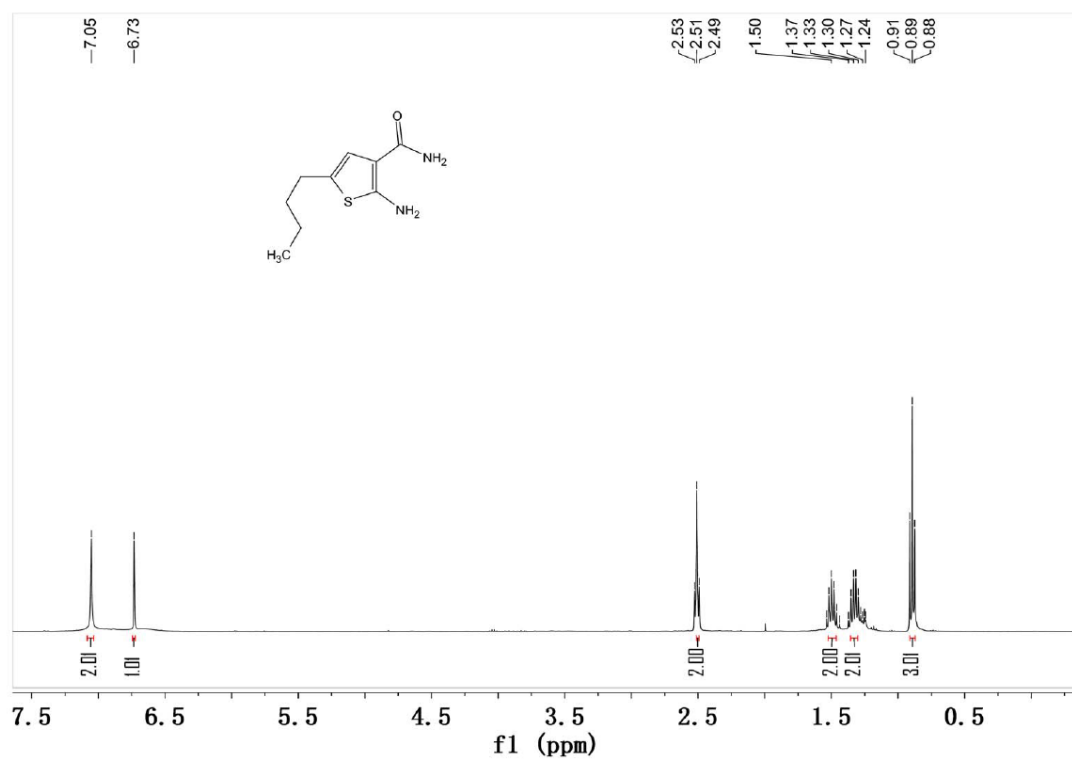
Figure S84 1 H NMR spectrum of compound 4n
