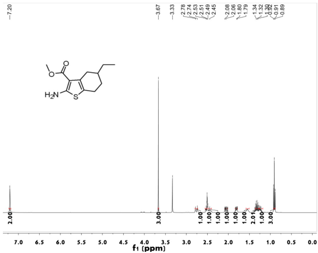
Figure S39 ^1\text{H} NMR spectrum of compound 3m
