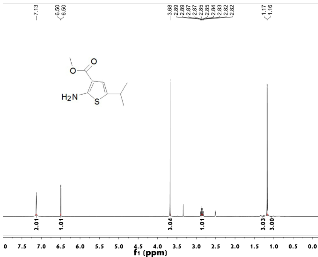
Figure S4 ^1\text{H} NMR spectrum of compound 3b
