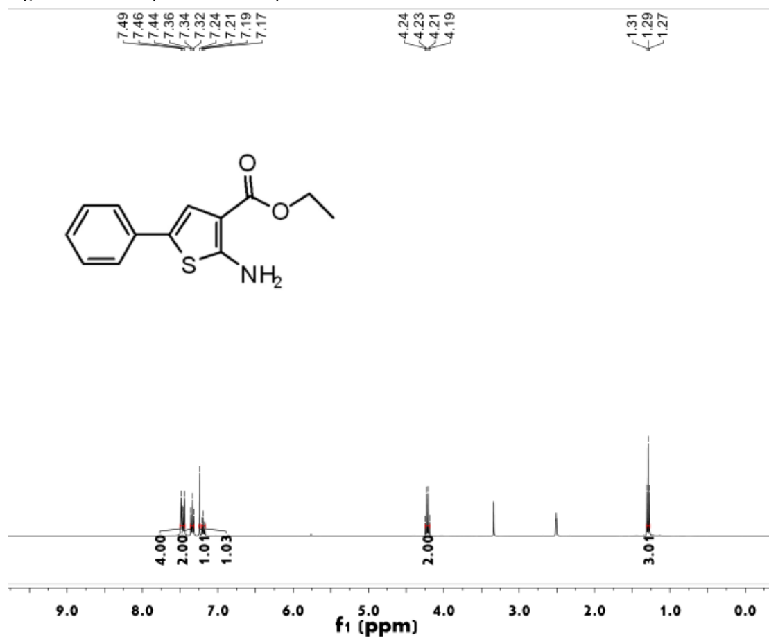
Figure S78 1 H NMR spectrum of compound 4l
