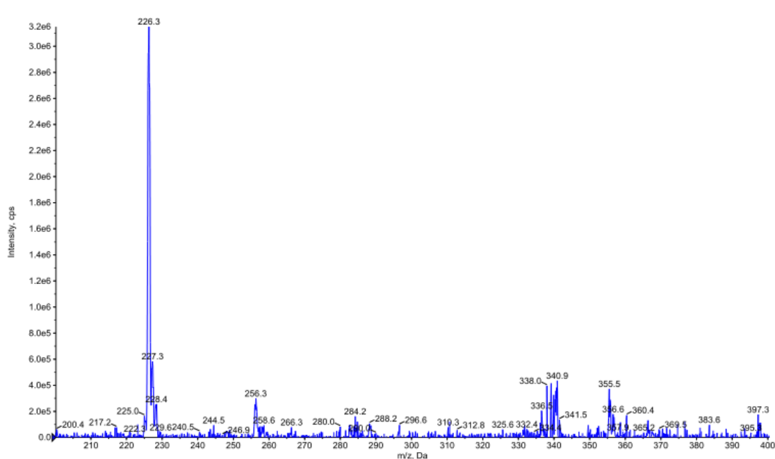
Figure S27 mass spectrum of compound 3i
