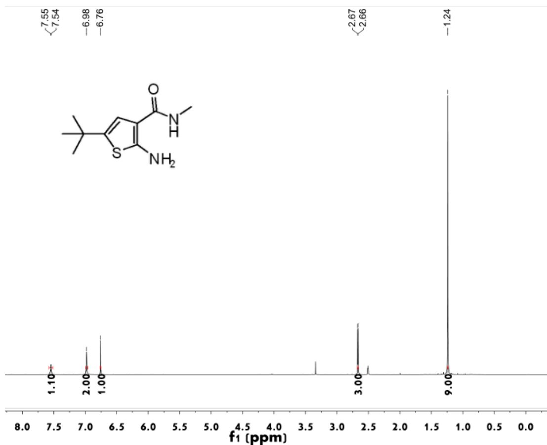
Figure S68 1 H NMR spectrum of compound 4i
