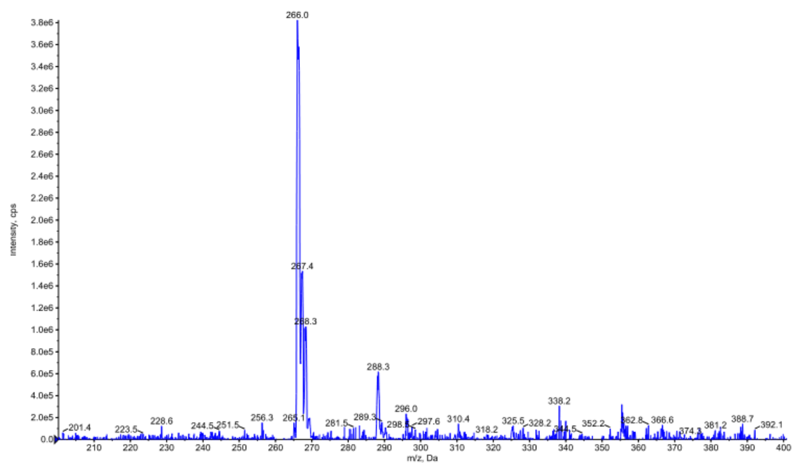
Figure S90 mass spectrum of compound 4o
