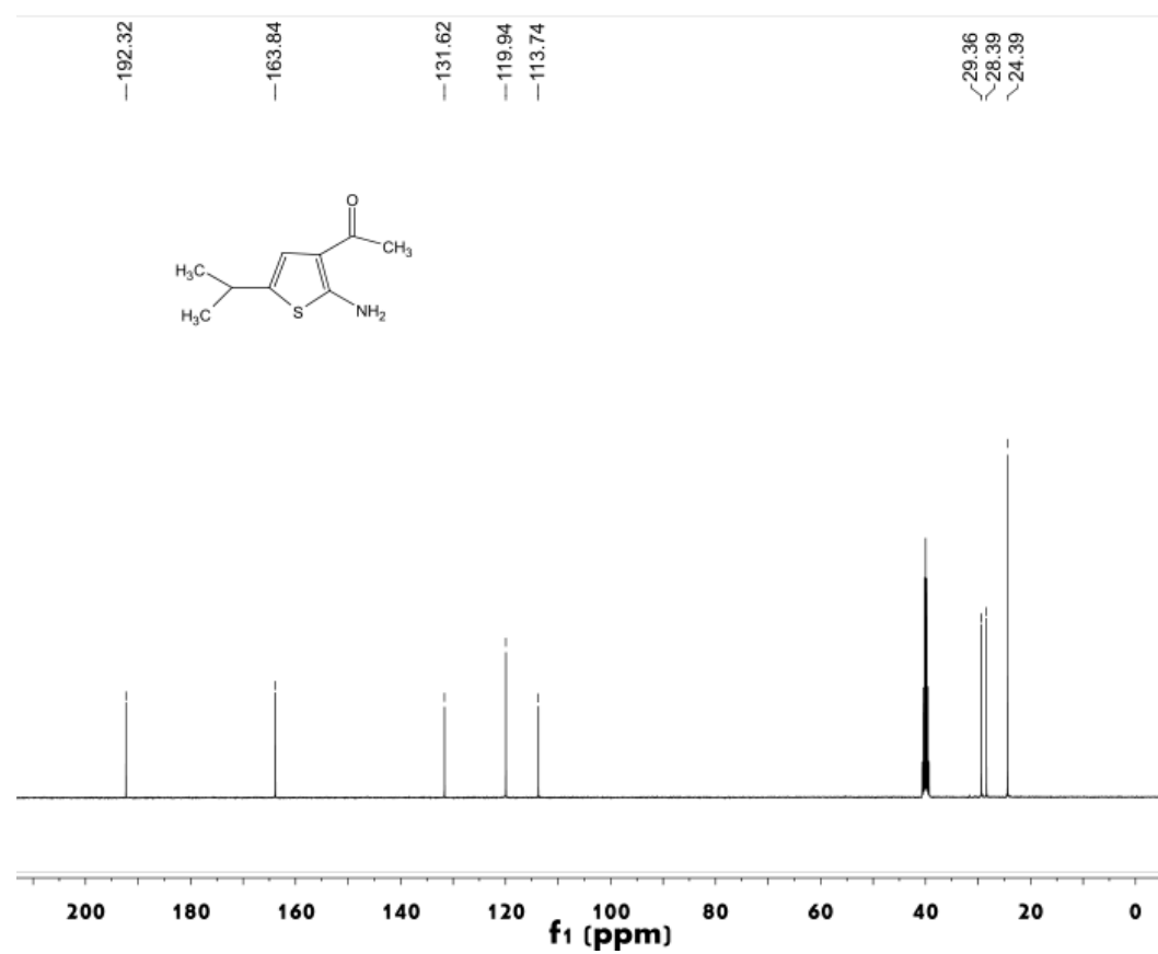
Figure S56 13 C NMR spectrum of compound 4e
