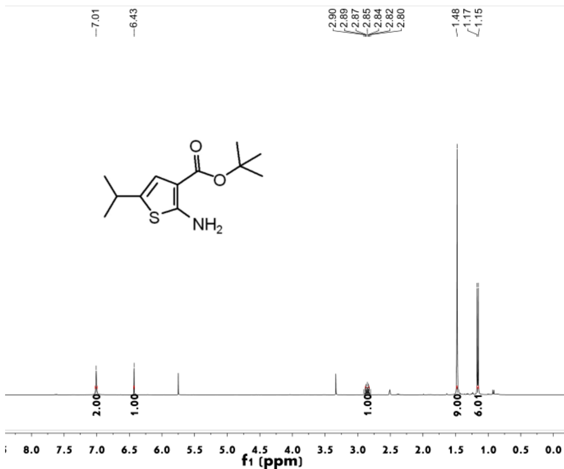
Figure S58 1 H NMR spectrum of compound 4f
