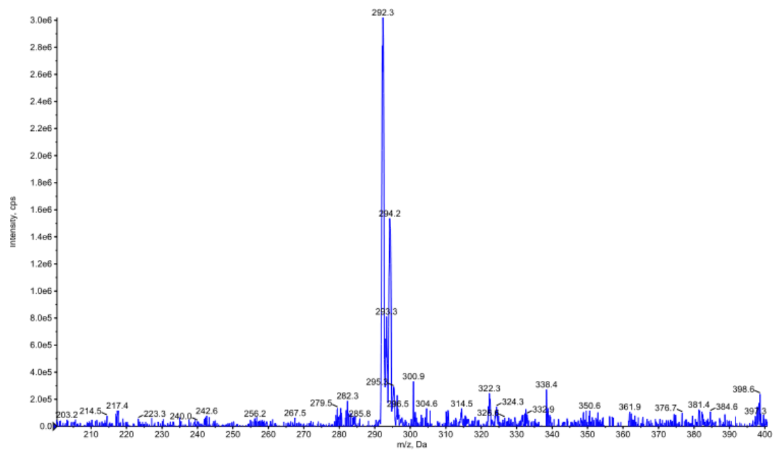
Figure S99 mass spectrum of compound 4r
