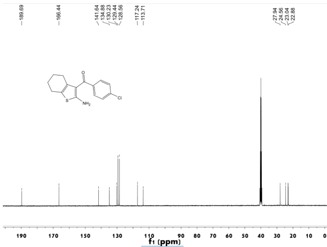
Figure S98 ^{13}\text{C NMR} spectrum of compound 4r
