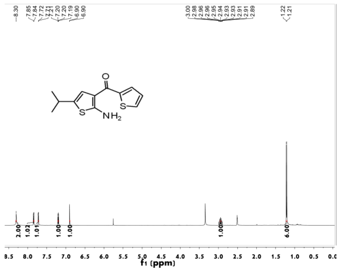
Figure S64 1 H NMR spectrum of compound 4h
