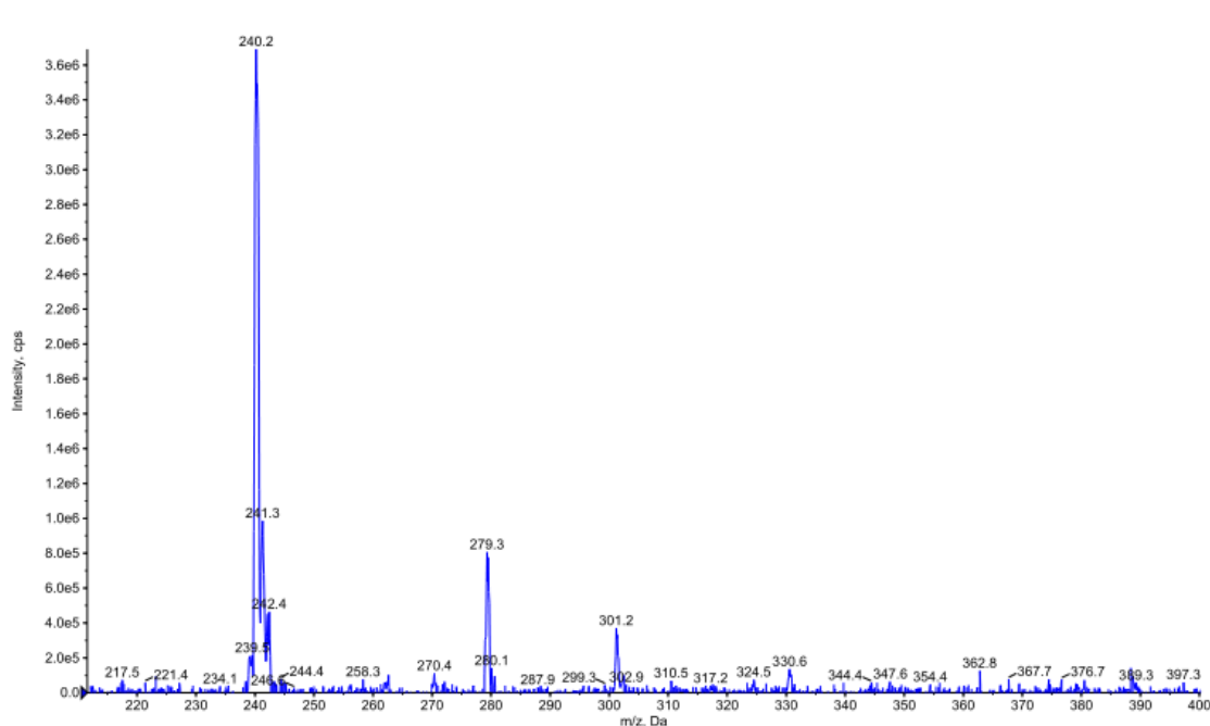
Figure S42 mass spectrum of compound 3m
