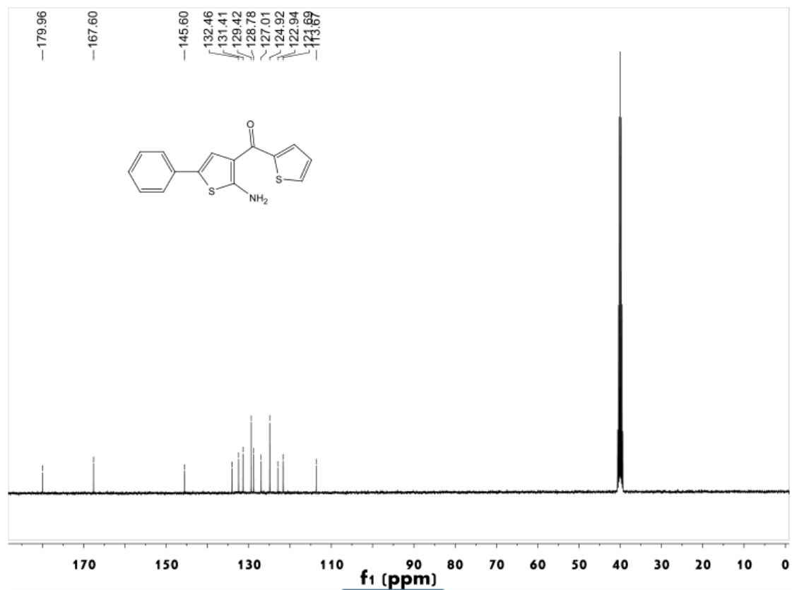
Figure S82 ^{13}\text{C} NMR spectrum of compound 4m
