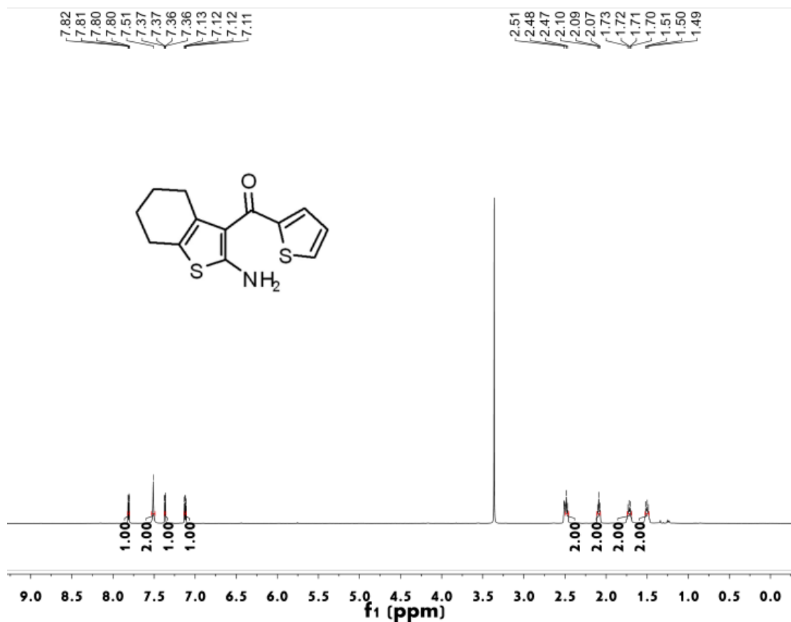
Figure S94 1 H NMR spectrum of compound 4q
