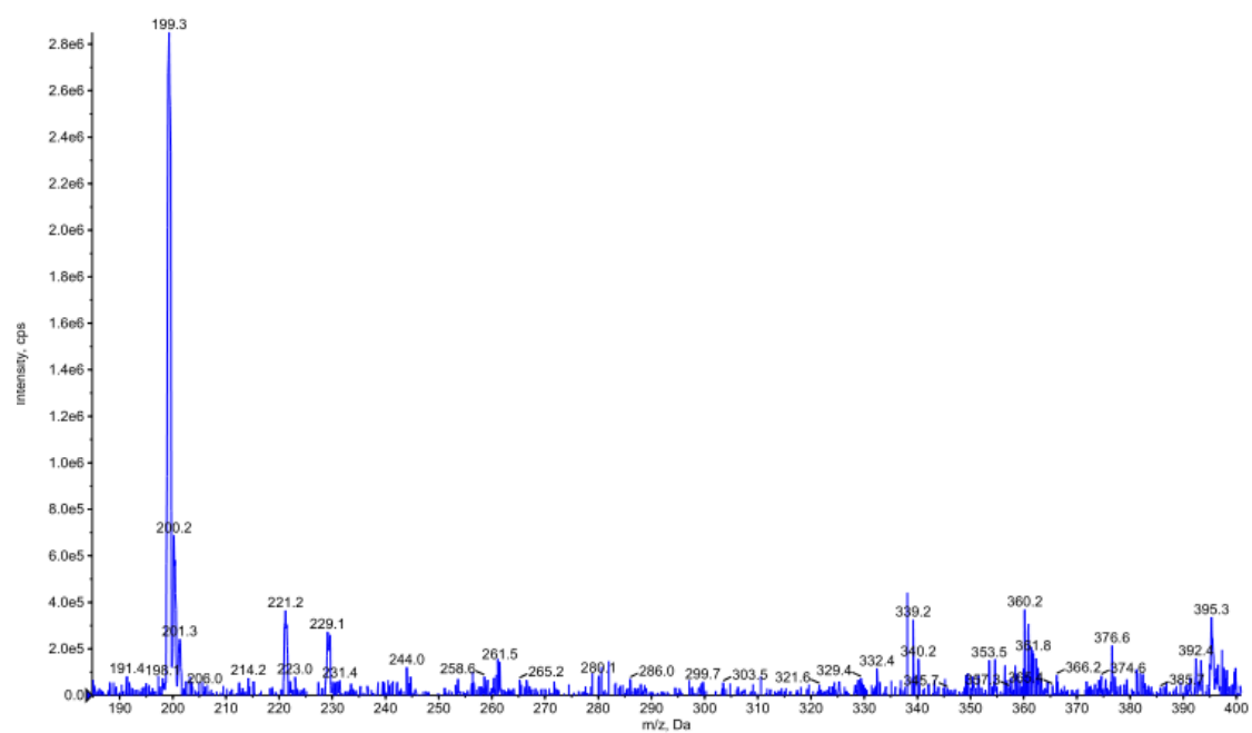
Figure S86 mass spectrum of compound 4n
