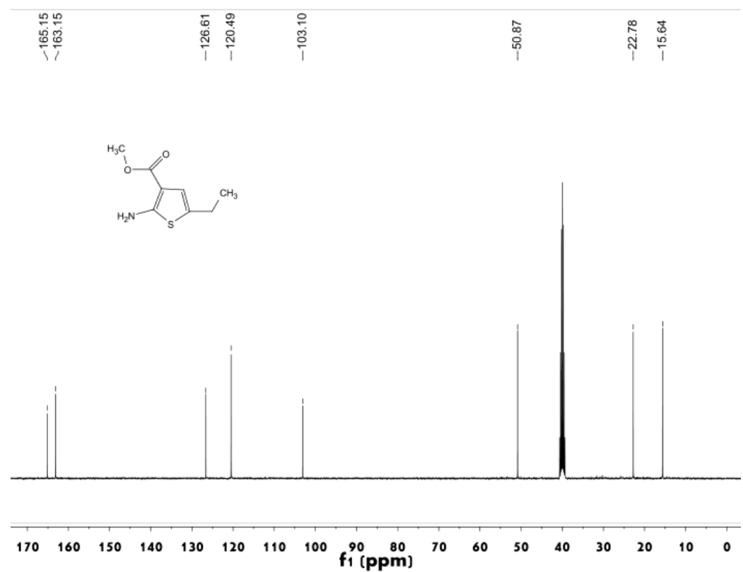
Figure S2 13 C NMR spectrum of compound 3a
