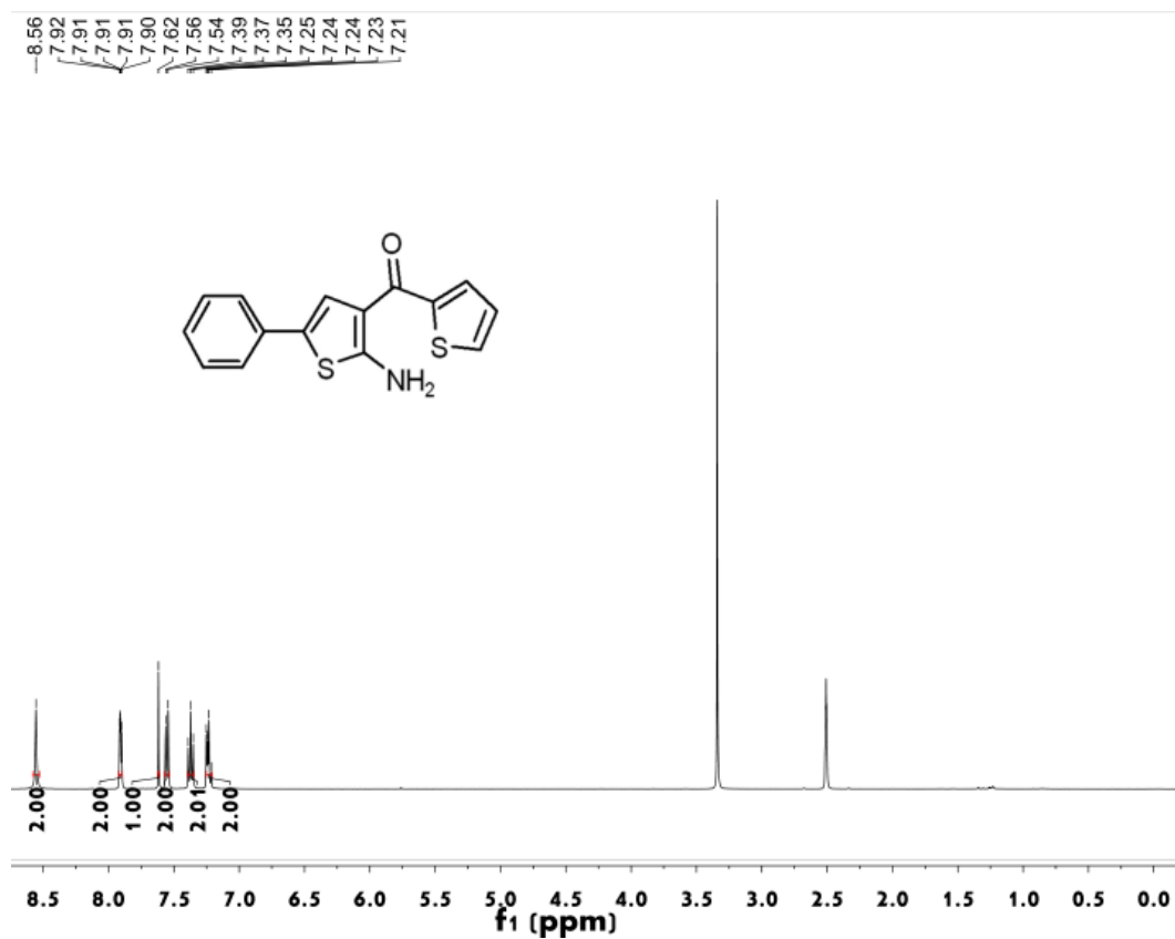
Figure S81 ^1\text{H} NMR spectrum of compound 4m
