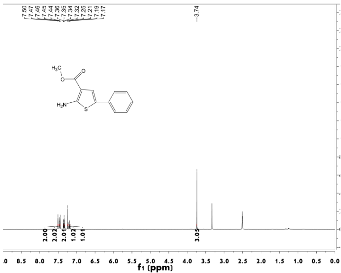
Figure S13 ^1\text{H NMR} spectrum of compound 3e
