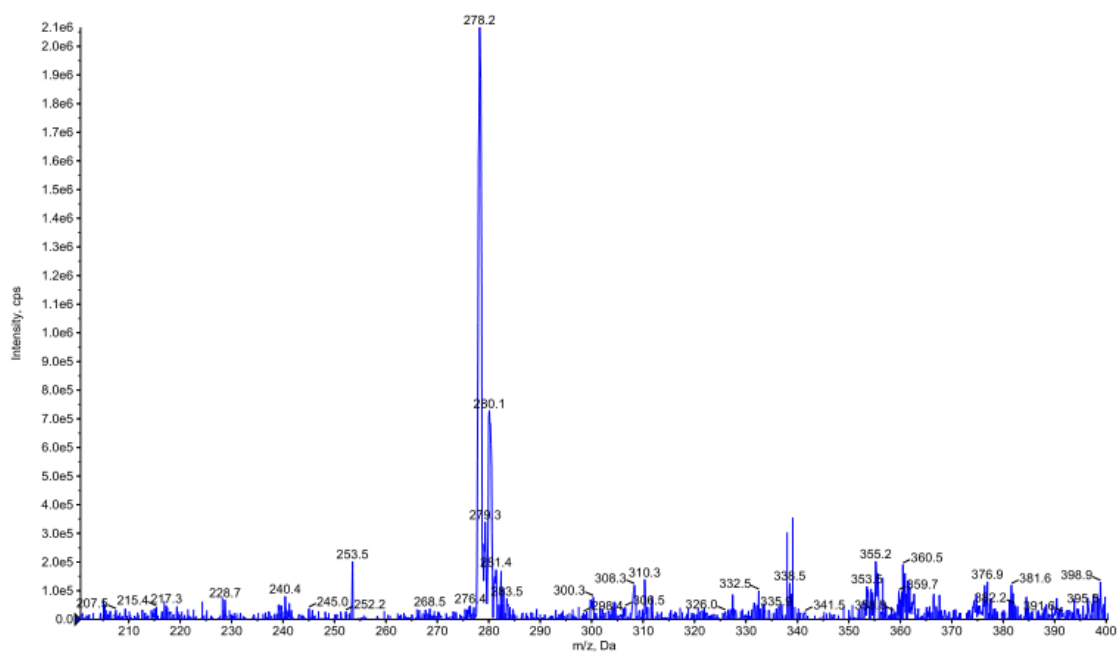
Figure S93 mass spectrum of compound 4p
