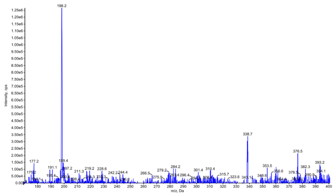
Figure S21 mass spectrum of compound 3g
