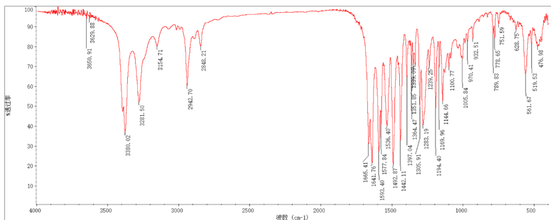
Figure S33 IR spectrum of compound 3k
