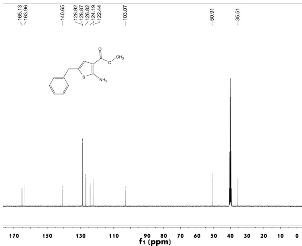
Figure S17 13 C NMR spectrum of compound 3f
