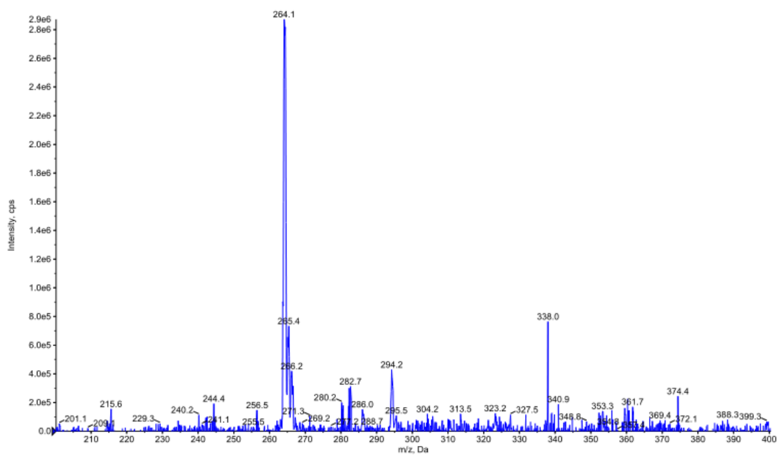
Figure S96 mass spectrum of compound 4q
