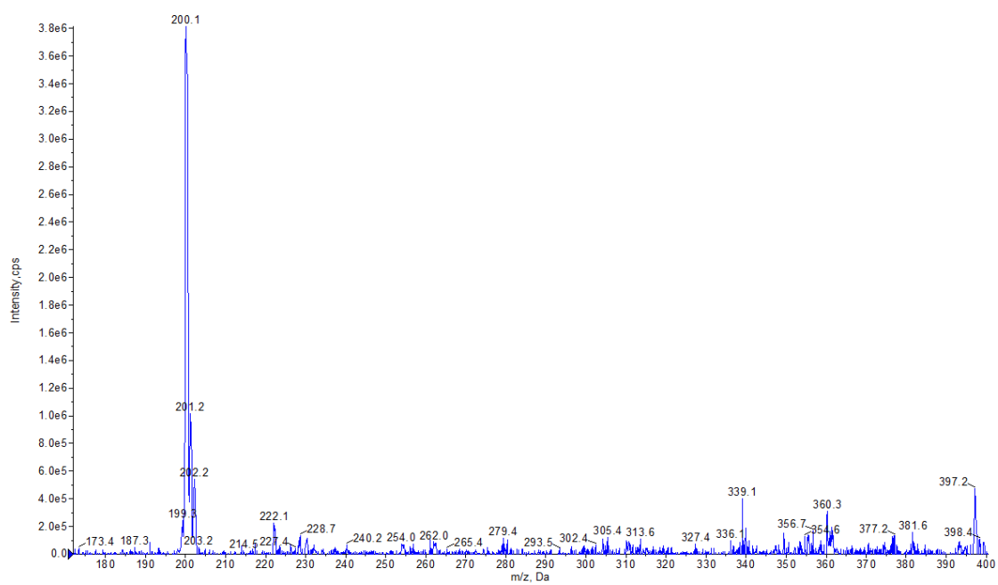
Figure S6 mass spectrum of compound 3b
