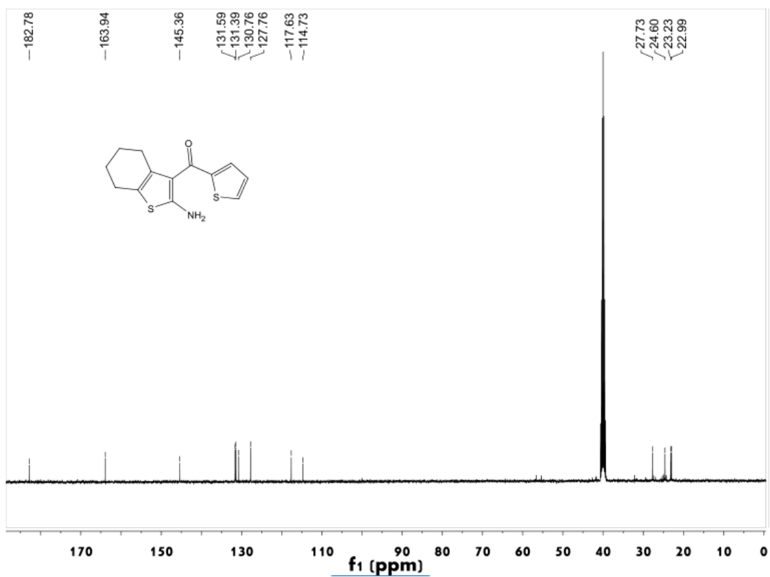
Figure S95 ^{13}\text{C} NMR spectrum of compound 4q
