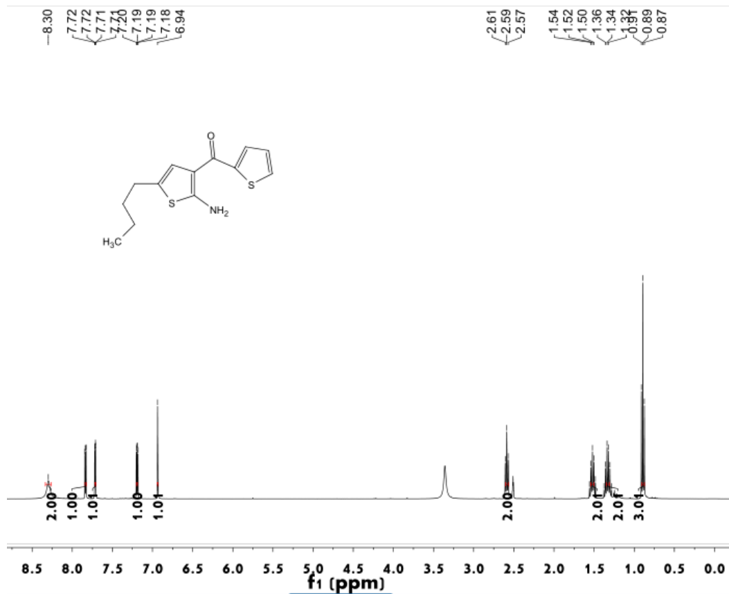
Figure S87 1 H NMR spectrum of compound 4o
