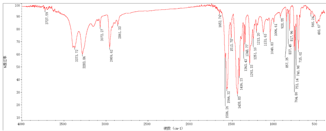
Figure S76 IR spectrum of compound 4k
