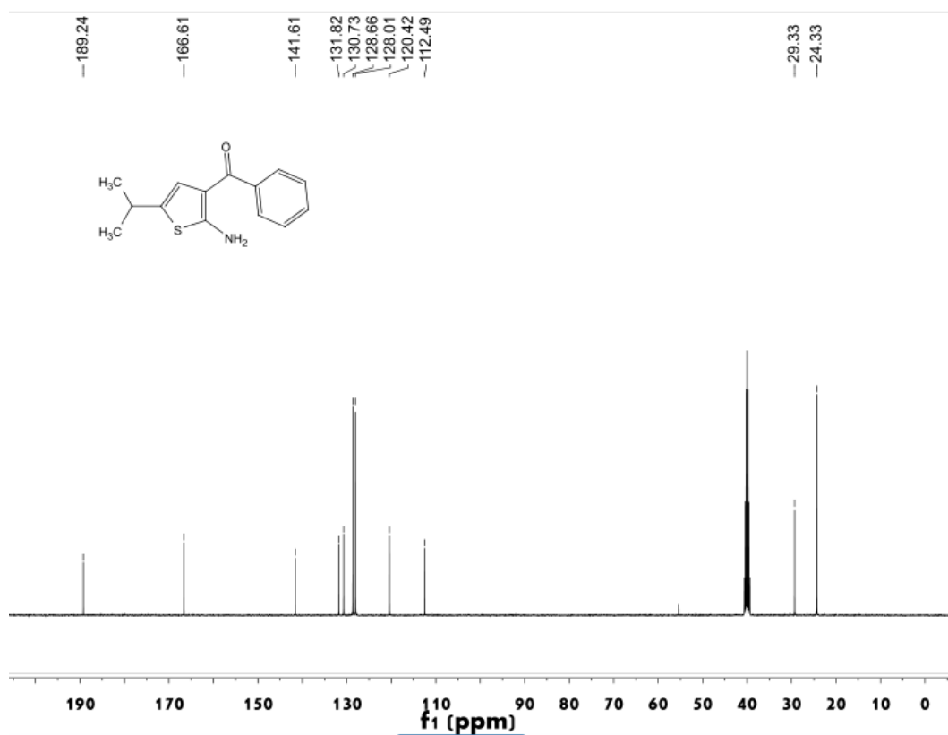
Figure S53 13 C NMR spectrum of compound 4d
