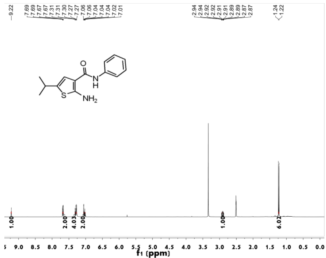
Figure S61 1 H NMR spectrum of compound 4g
