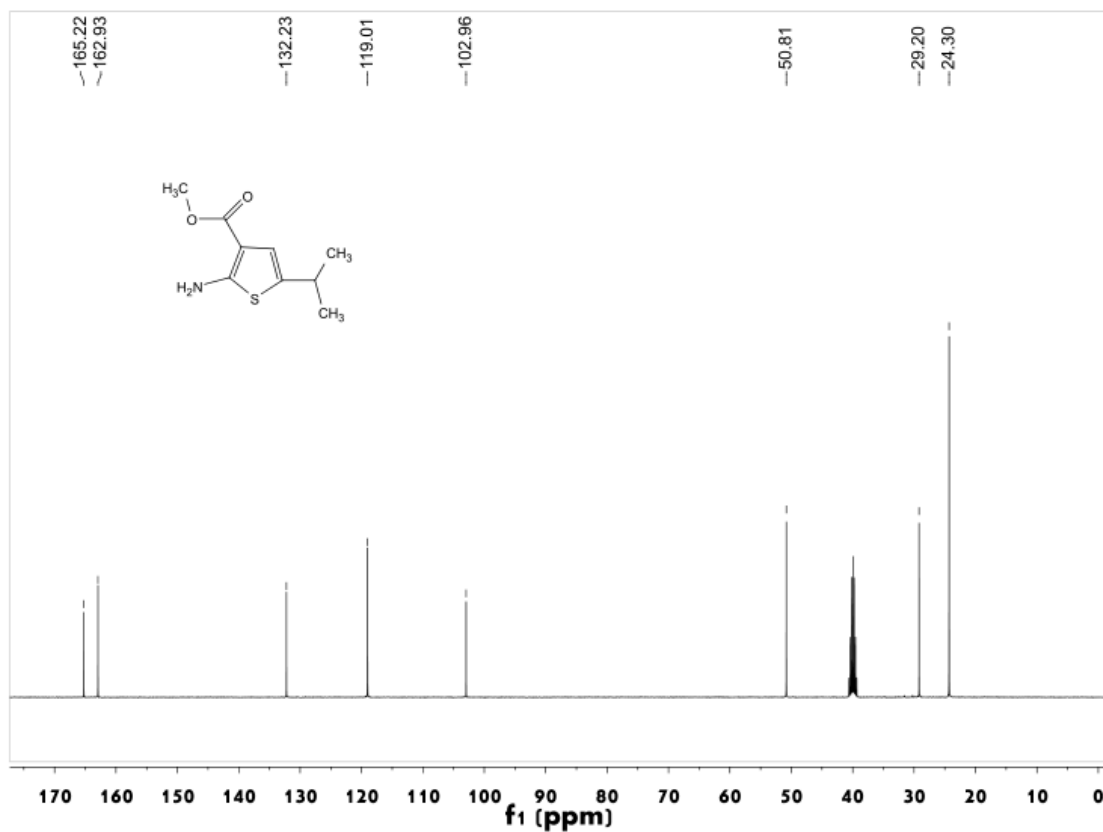
Figure S5 ^{13}\text{C} NMR spectrum of compound 3b
