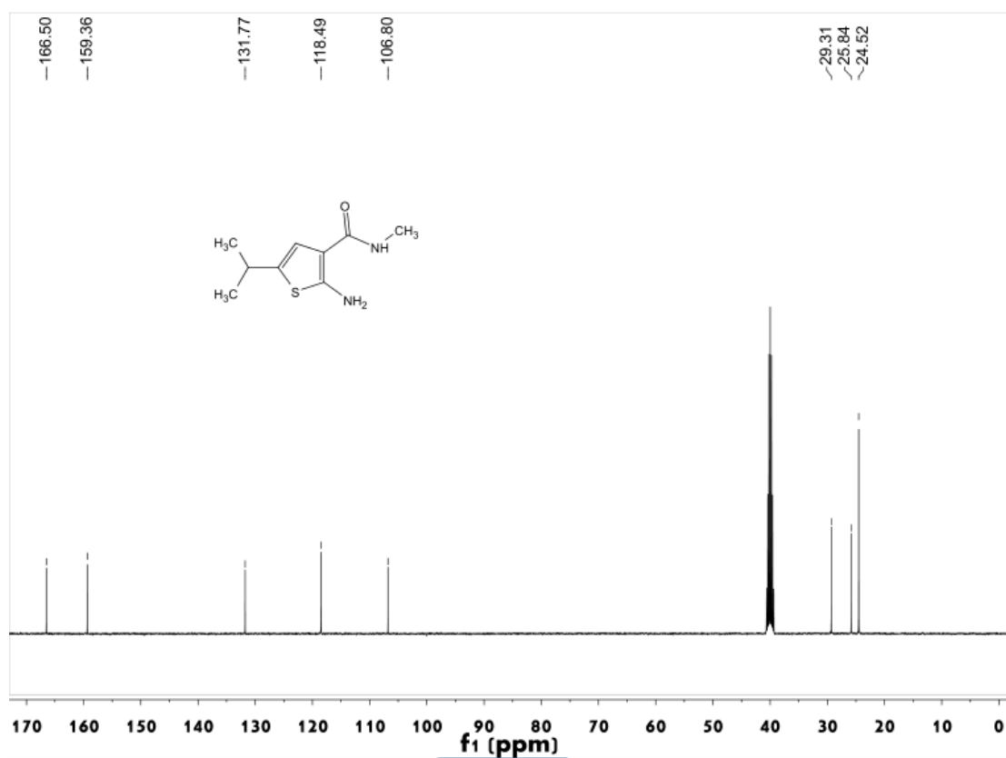
Figure S47 ^{13}\text{C} NMR spectrum of compound 4b
