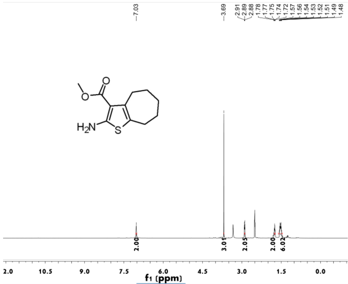
Figure S25 ^1\text{H NMR} spectrum of compound 3i
