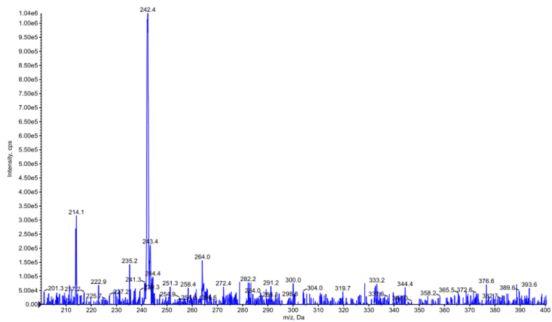
Figure S60 mass spectrum of compound 4f
