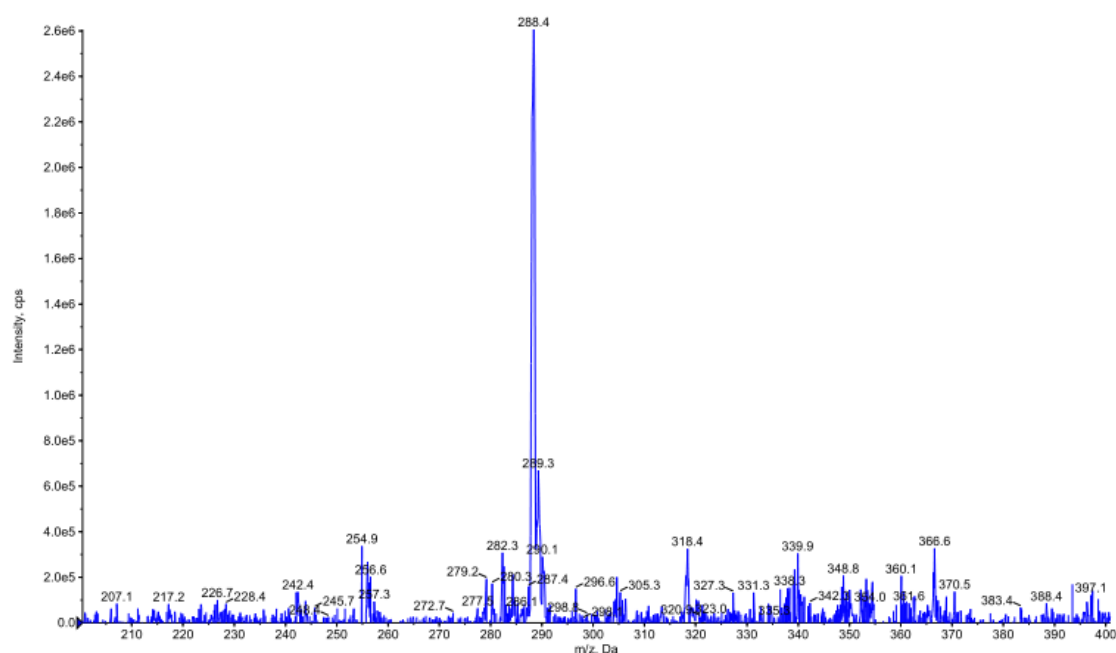
Figure S38 mass spectrum of compound 31
