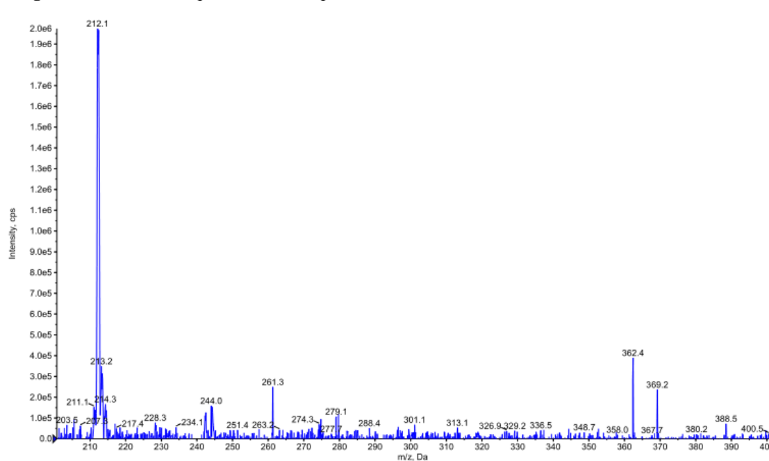
Figure S24 mass spectrum of compound 3h
