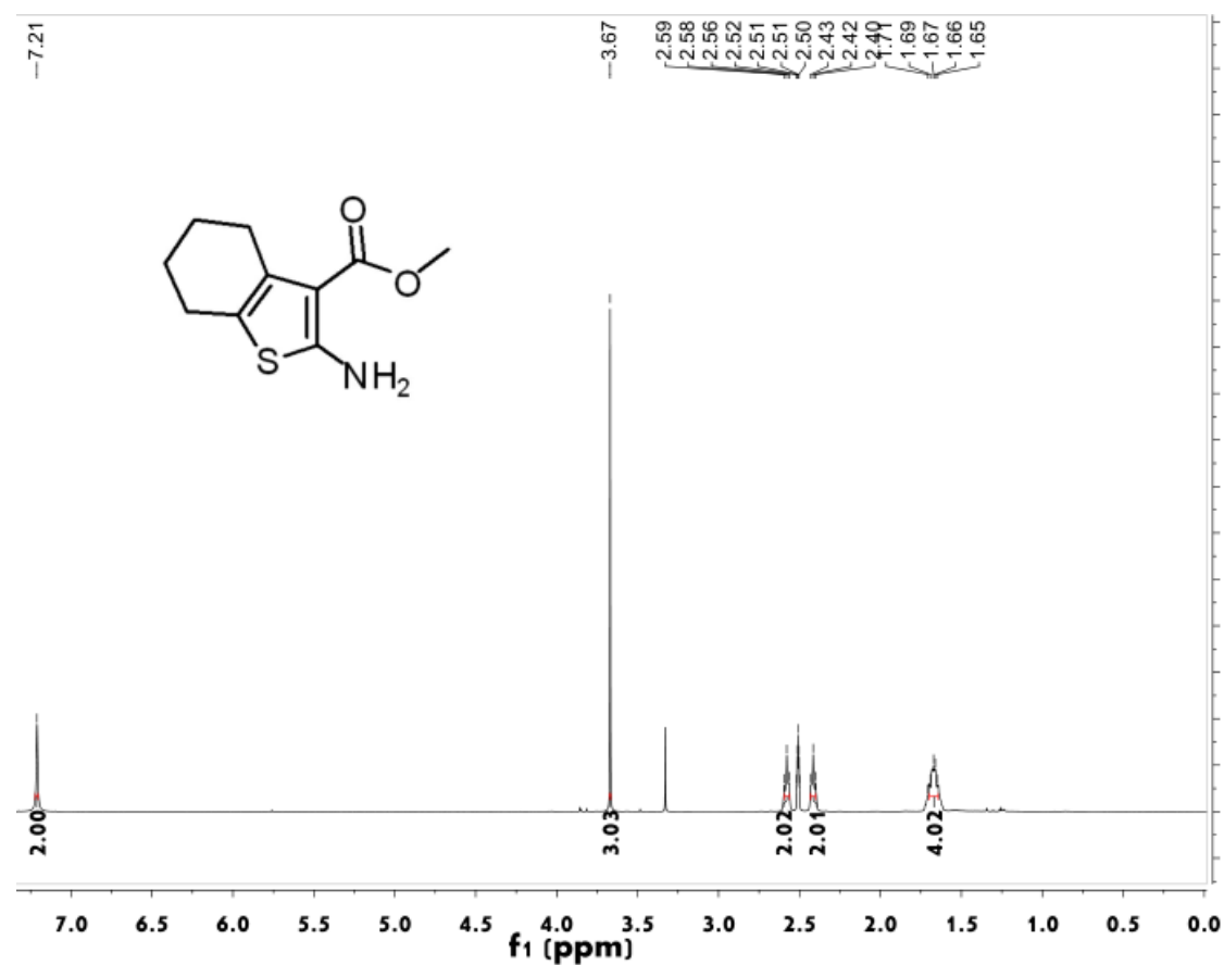
Figure S22 1 H NMR spectrum of compound 3h
