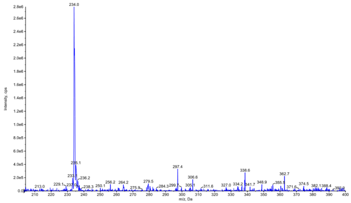
Figure S15 mass spectrum of compound 3e
