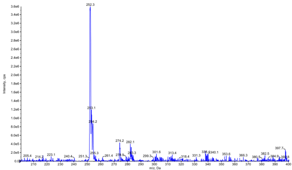
Figure S67 mass spectrum of compound 4h
