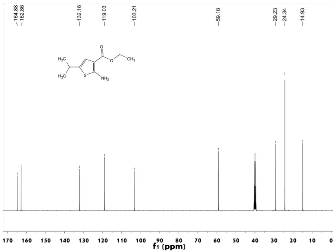
Figure S44 13 C NMR spectrum of compound 4a
