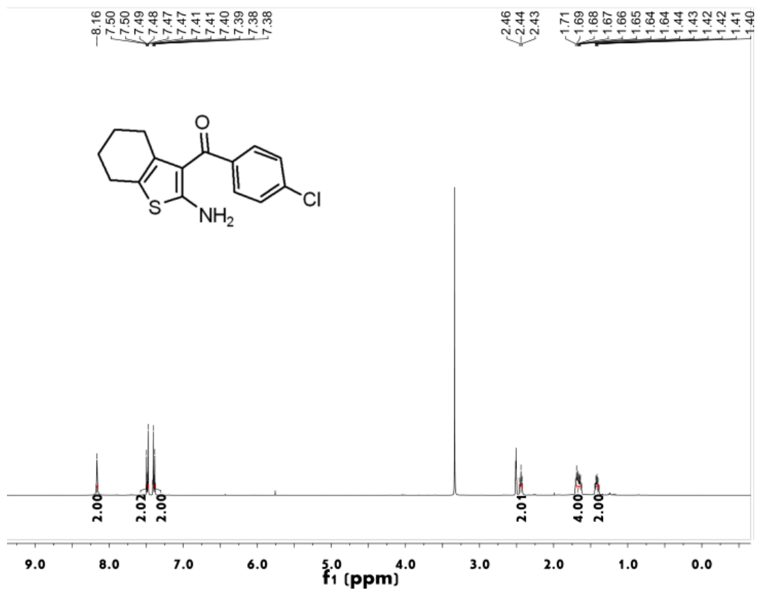
Figure S97 ^1\text{H NMR} spectrum of compound 4r
