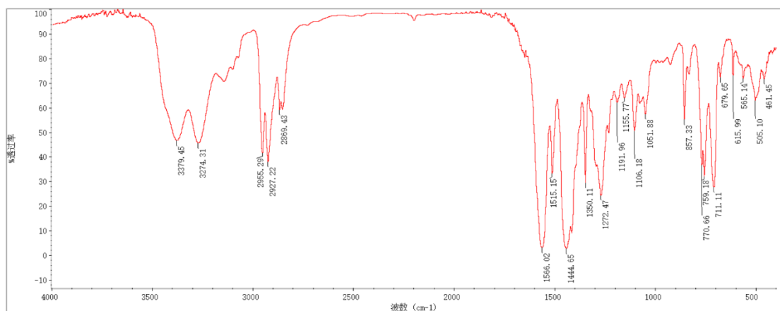
Figure S89 IR spectrum of compound 4o
