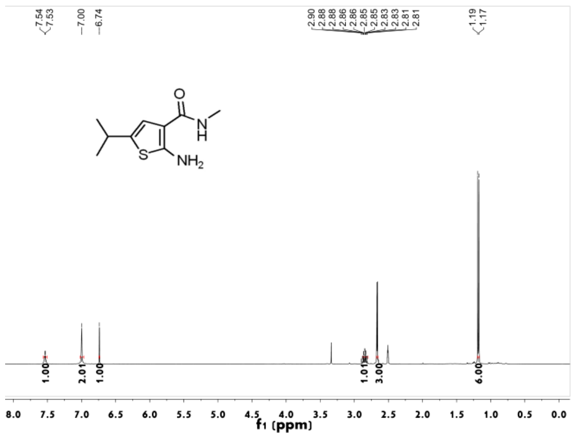
Figure S46 1 H NMR spectrum of compound 4b
