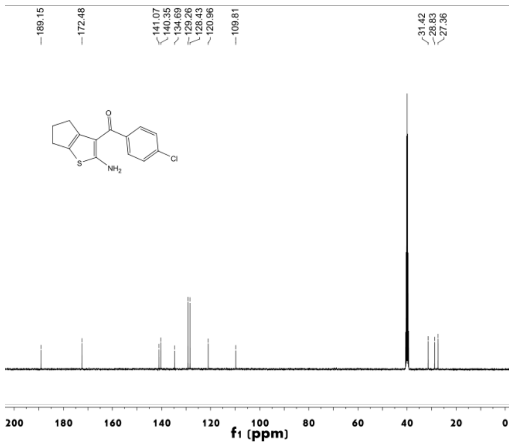
Figure S92 ^{13}\text{C} NMR spectrum of compound 4p
