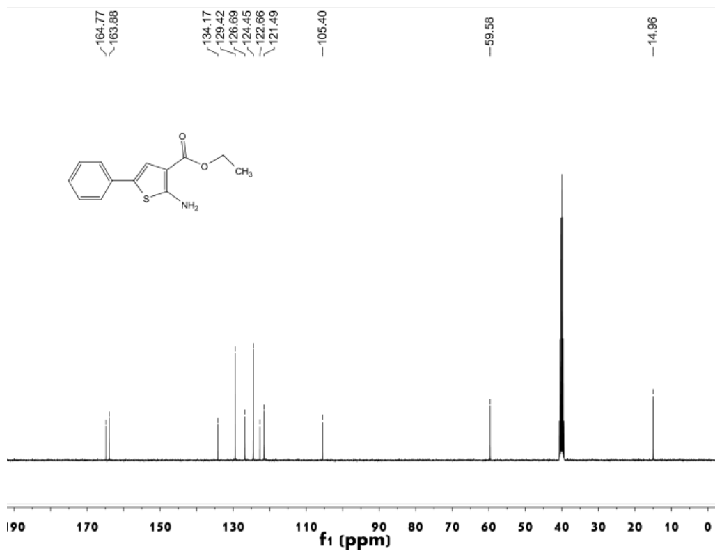
Figure S79 13 C NMR spectrum of compound 4l
