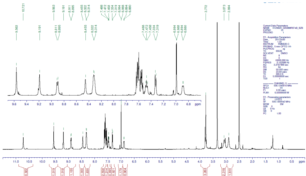
Figure S12. 1 H-NMR spectrum of 25 measured at 500 MHz in DMSO-d 6
