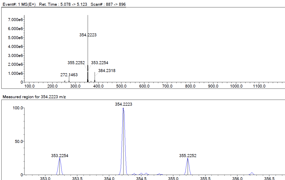
Figure S5. HRMS spectrum of 22
