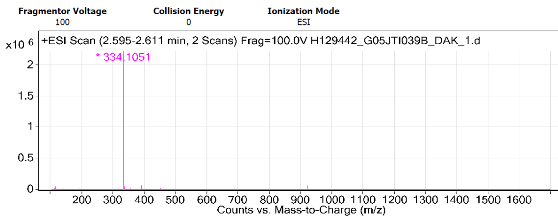
Figure S21. HRMS spectrum of 33
