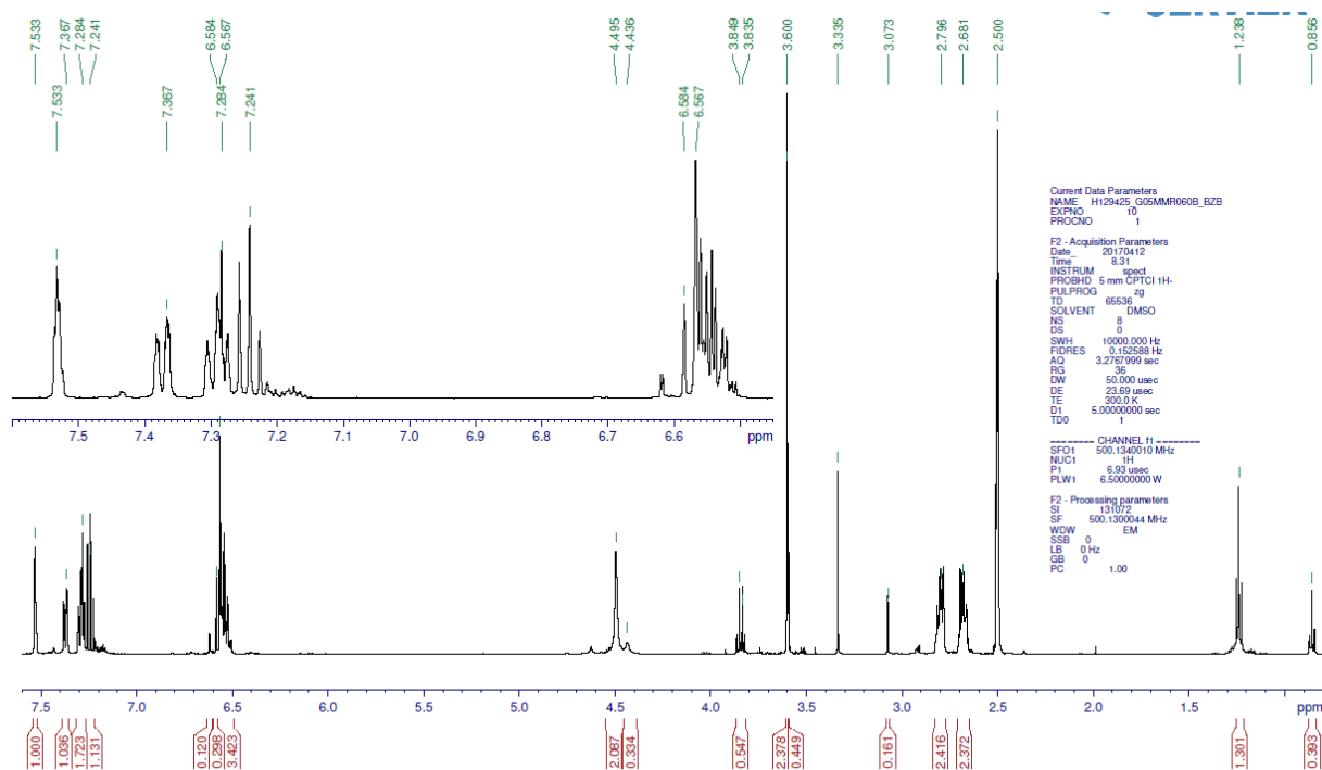
Figure S4. ^1\text{H} -NMR spectrum of 21 measured at 500 MHz in DMSO- d_6
