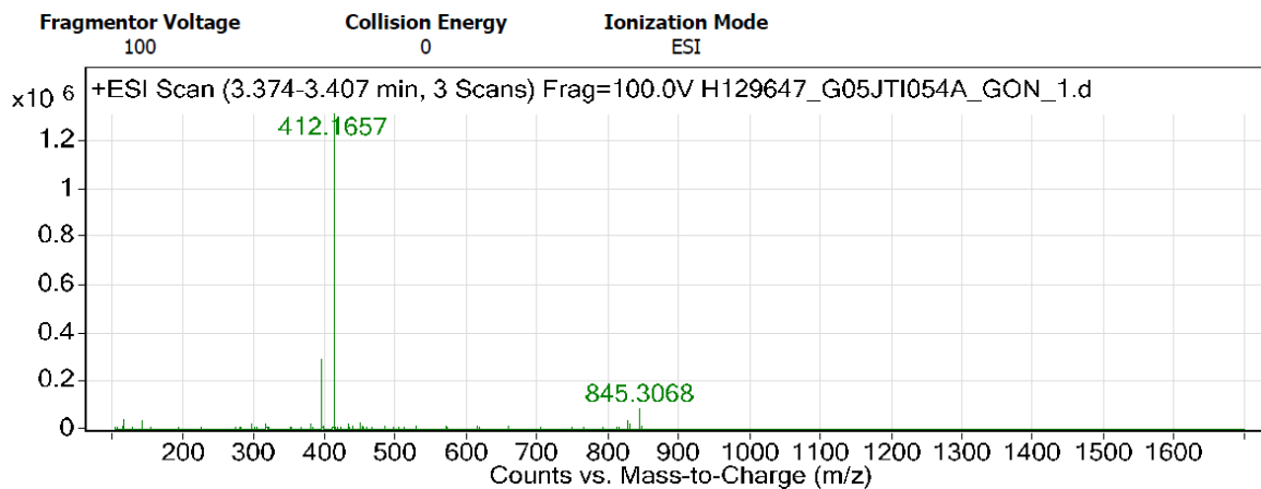
Figure S33. HRMS spectrum of 40
