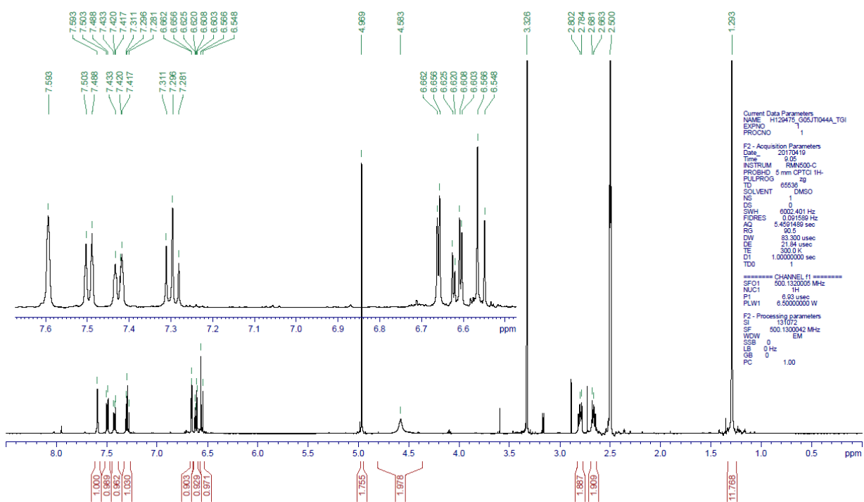
Figure S28. ^1\text{H} -NMR spectrum of 37 measured at 500 MHz in DMSO- d_6
