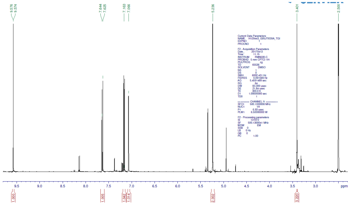
Figure S24. 1 H-NMR spectrum of 34 measured at 500 MHz in DMSO-d 6
