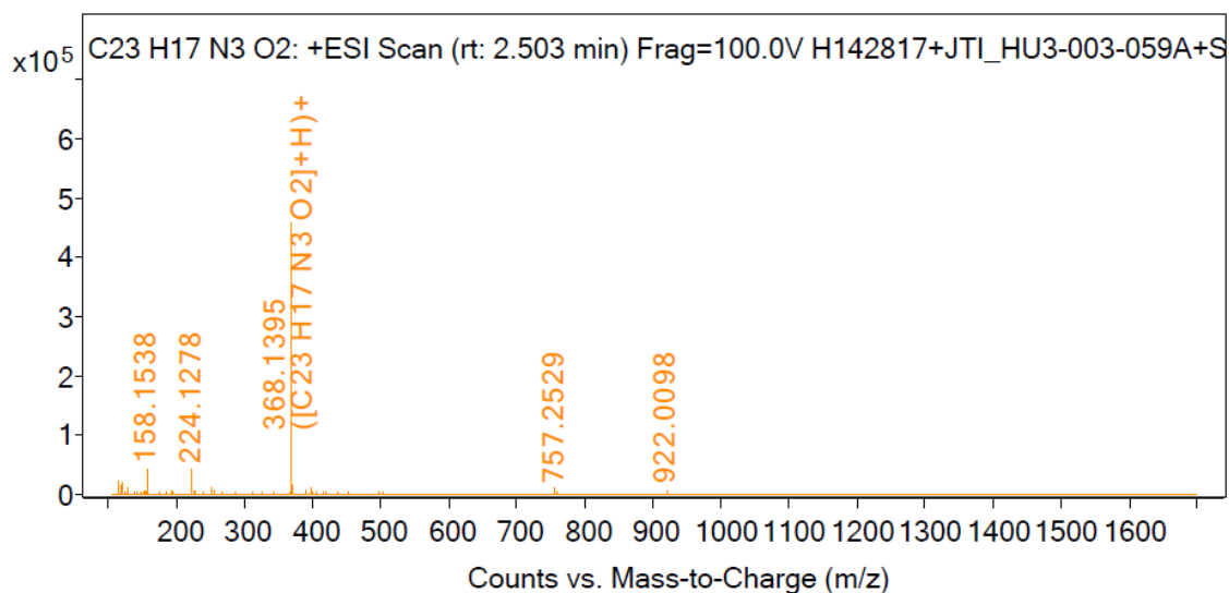
Figure S37. HRMS spectrum of 26
