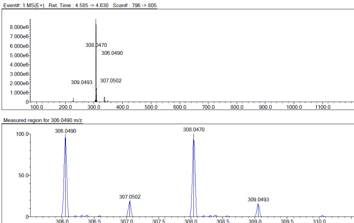
Figure S3. HRMS spectrum of 21
