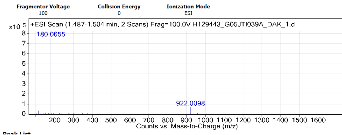
Figure S23. HRMS spectrum of 34
