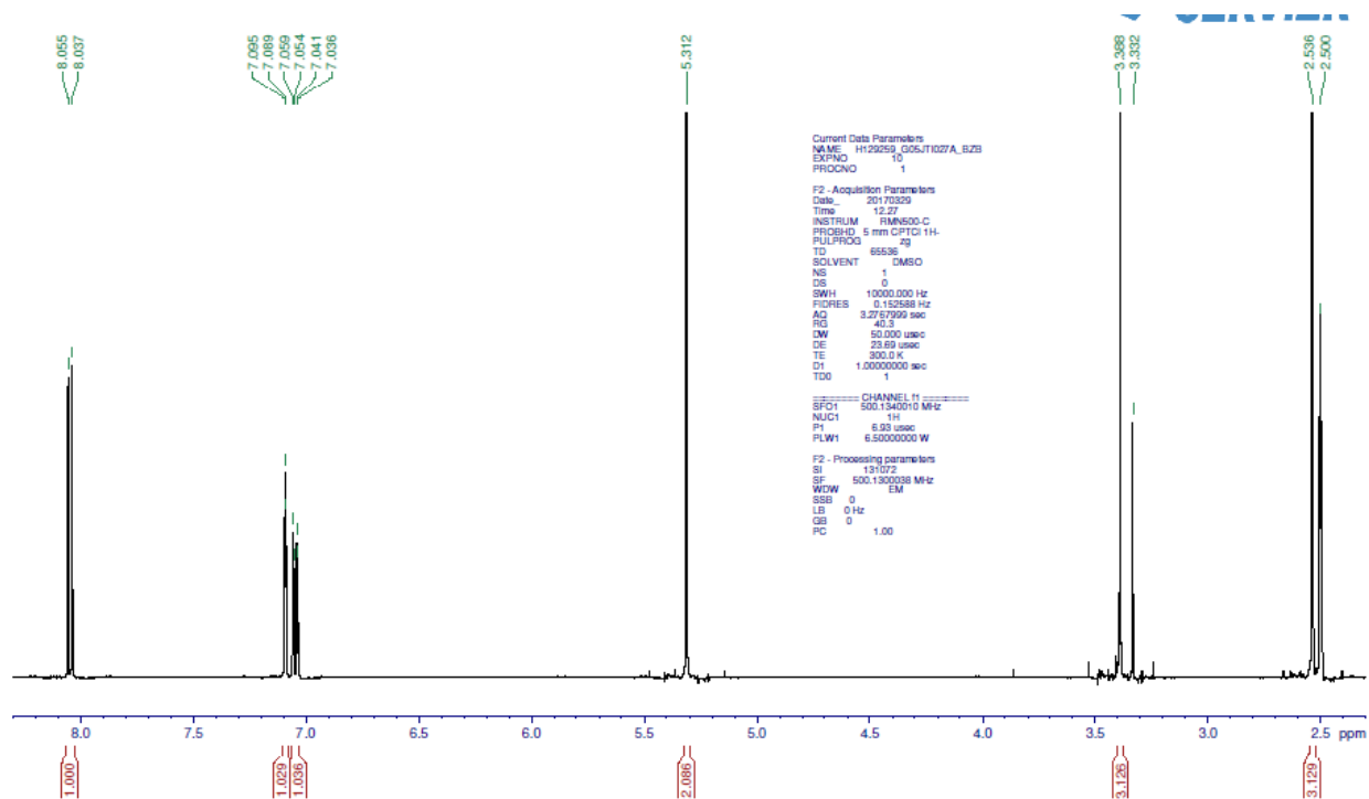
Figure S13. HRMS spectrum of 28
