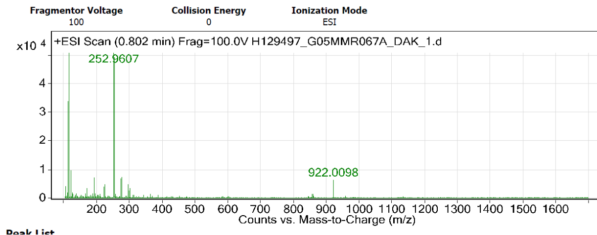
Figure S29. HRMS spectrum of 38
