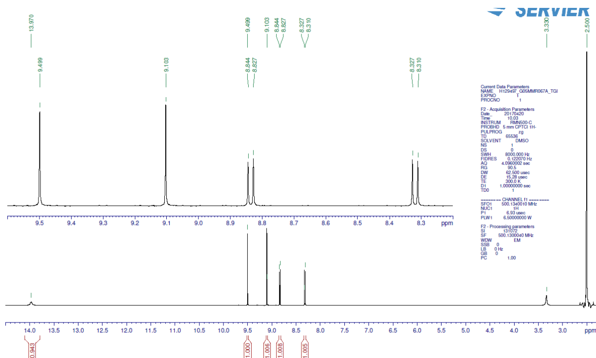
Figure S30. 1 H-NMR spectrum of 38 measured at 500 MHz in DMSO-d 6
