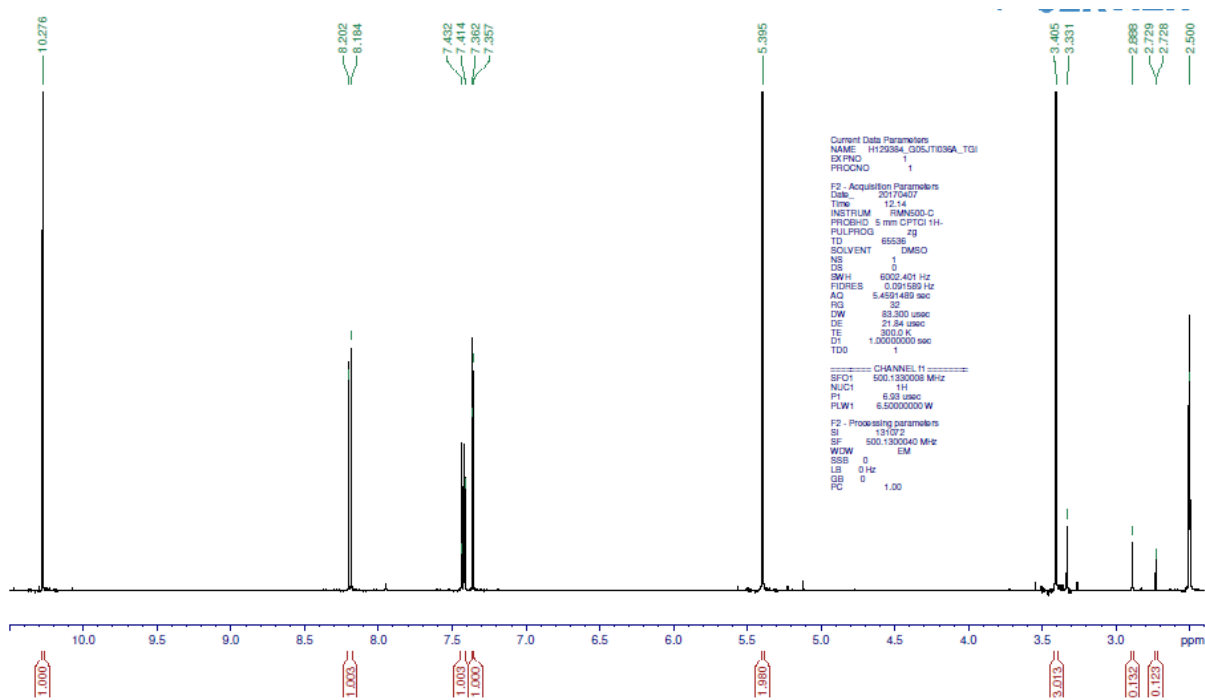
Figure S16. ^1\text{H-NMR} spectrum of 30 measured at 500 MHz in \text{DMSO-d}_6
