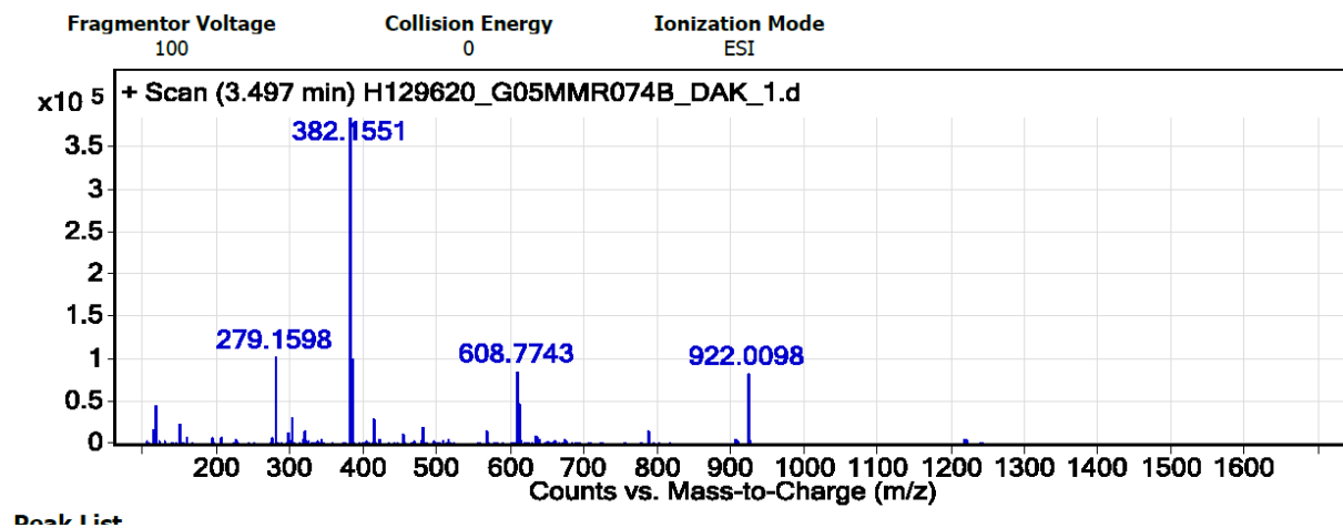
Figure S11. HRMS spectrum of 25
