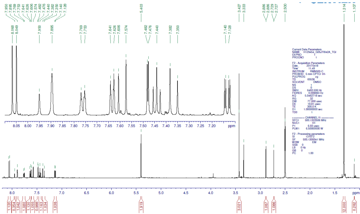
Figure S26. ^1\text{H-NMR} spectrum of 36 measured at 500 MHz in \text{DMSO-d}_6
