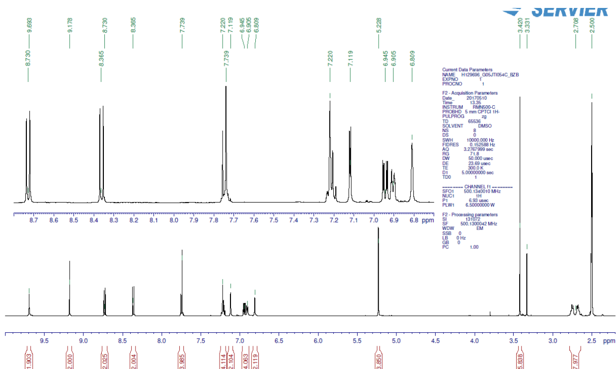
Figure S36. ^1\text{H-NMR} spectrum of 41 measured at 500 MHz in \text{DMSO-d}_6
