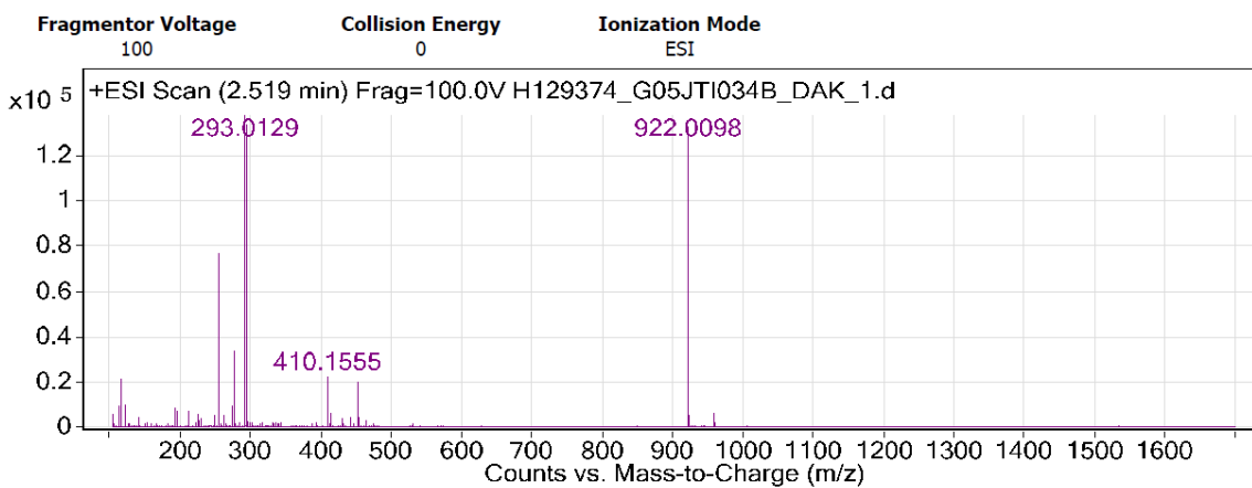
Figure S19. HRMS spectrum of 32
