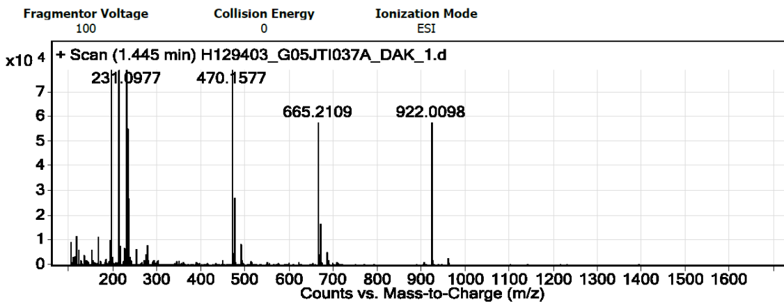
Figure S17. HRMS spectrum of 31
