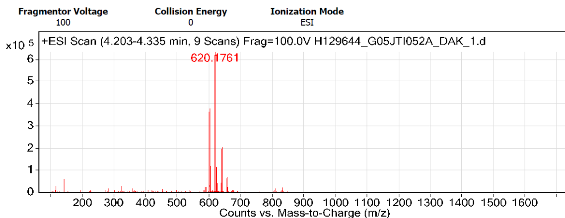
Figure S31. HRMS spectrum of 39
