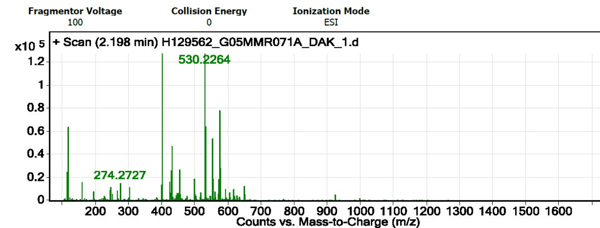
Figure S9. HRMS spectrum of 24
