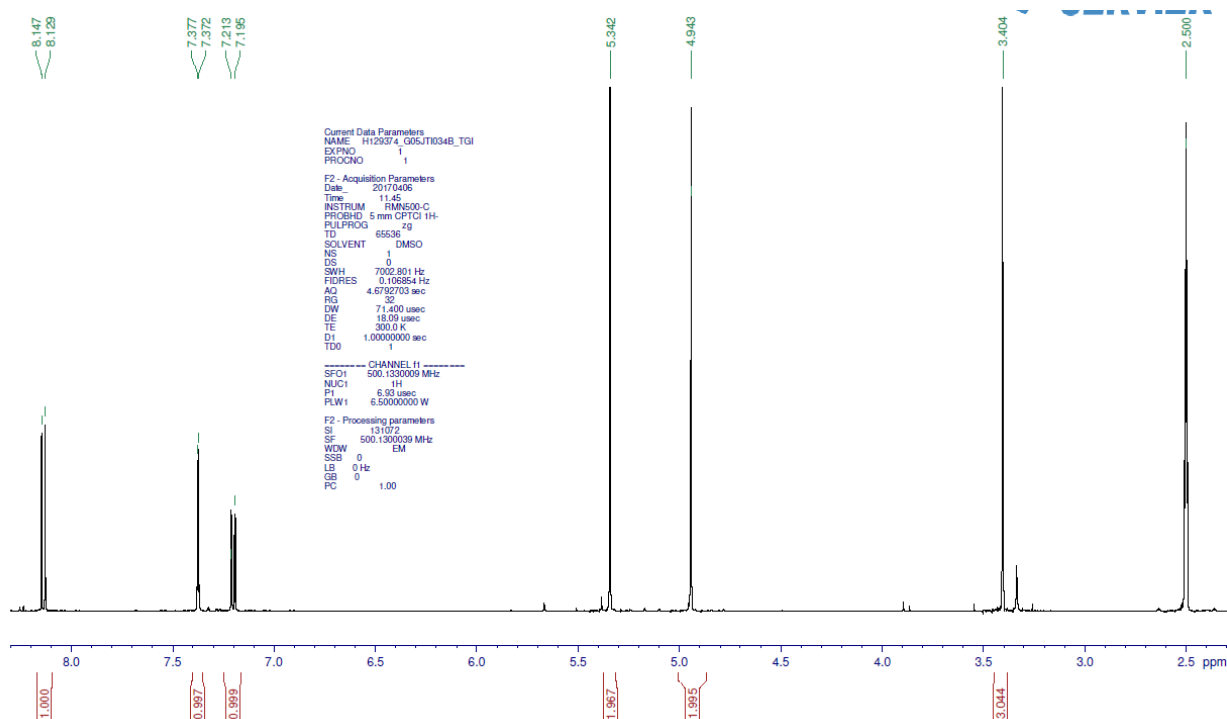
Figure S20. ^1\text{H} -NMR spectrum of 32 measured at 500 MHz in DMSO- d_6
