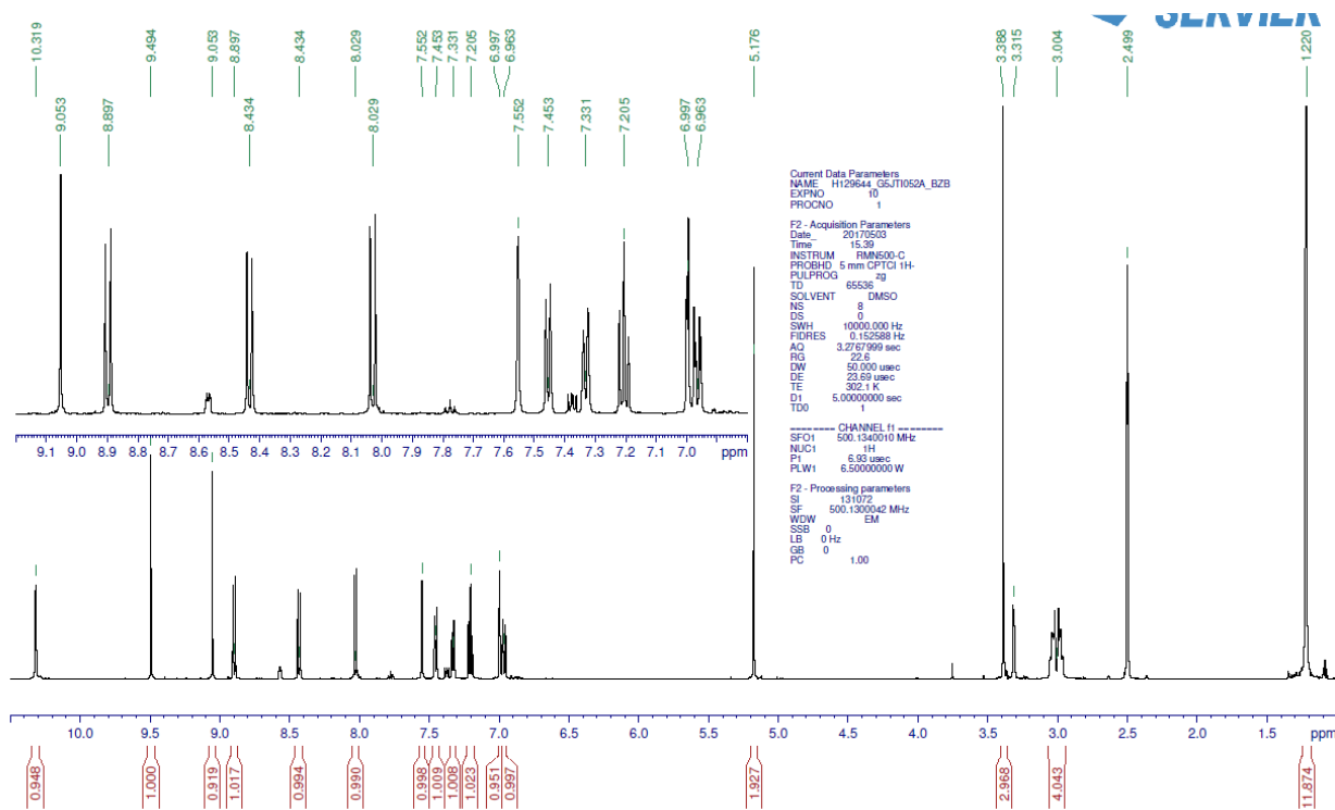
Figure S32. 1 H-NMR spectrum of 39 measured at 500 MHz in DMSO-d 6
