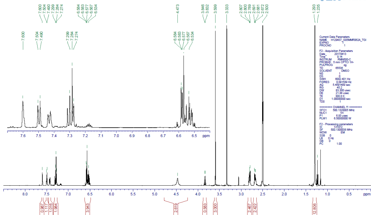
Figure S6. ^1\text{H} -NMR spectrum of 22 measured at 500 MHz in DMSO- d_6
