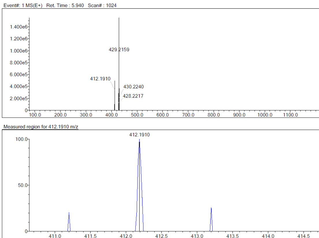
Figure S25. HRMS spectrum of 36
