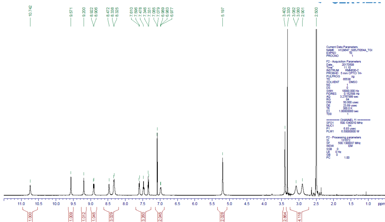
Figure S34. ^1\text{H} -NMR spectrum of 40 measured at 500 MHz in DMSO- d_6
