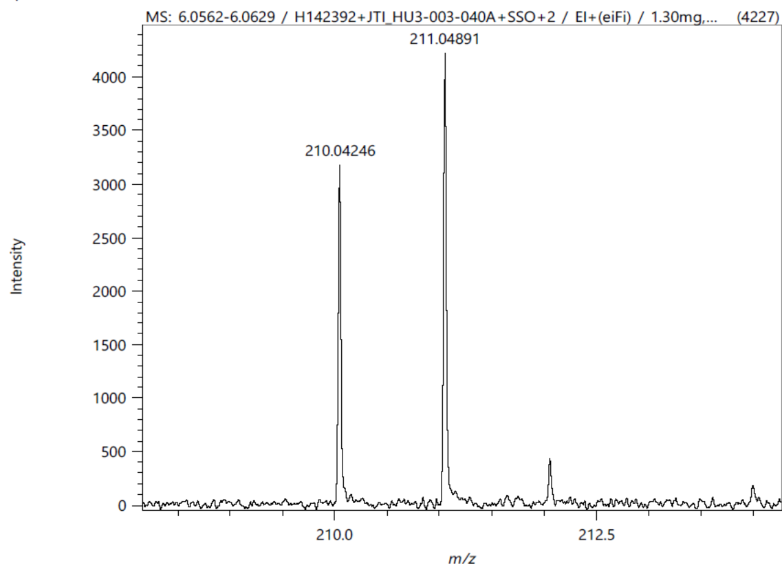
Figure S15. HRMS spectrum of 30
