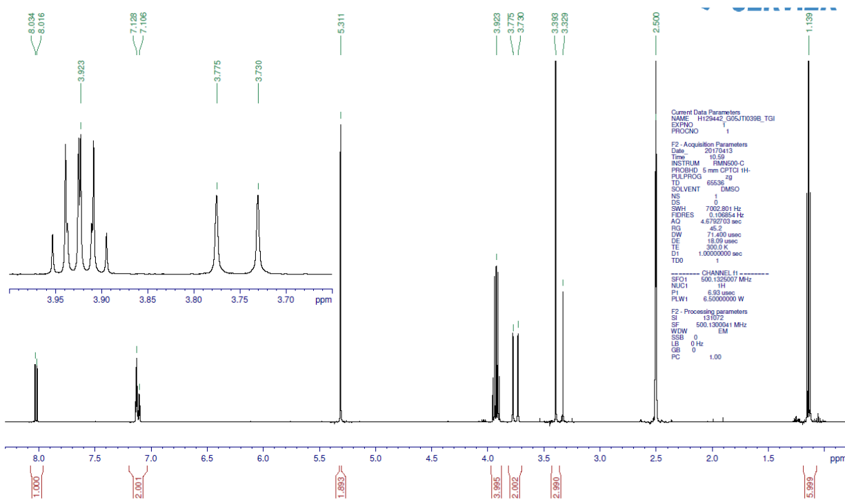
Figure S22. ^1\text{H} -NMR spectrum of 33 measured at 500 MHz in DMSO- d_6
