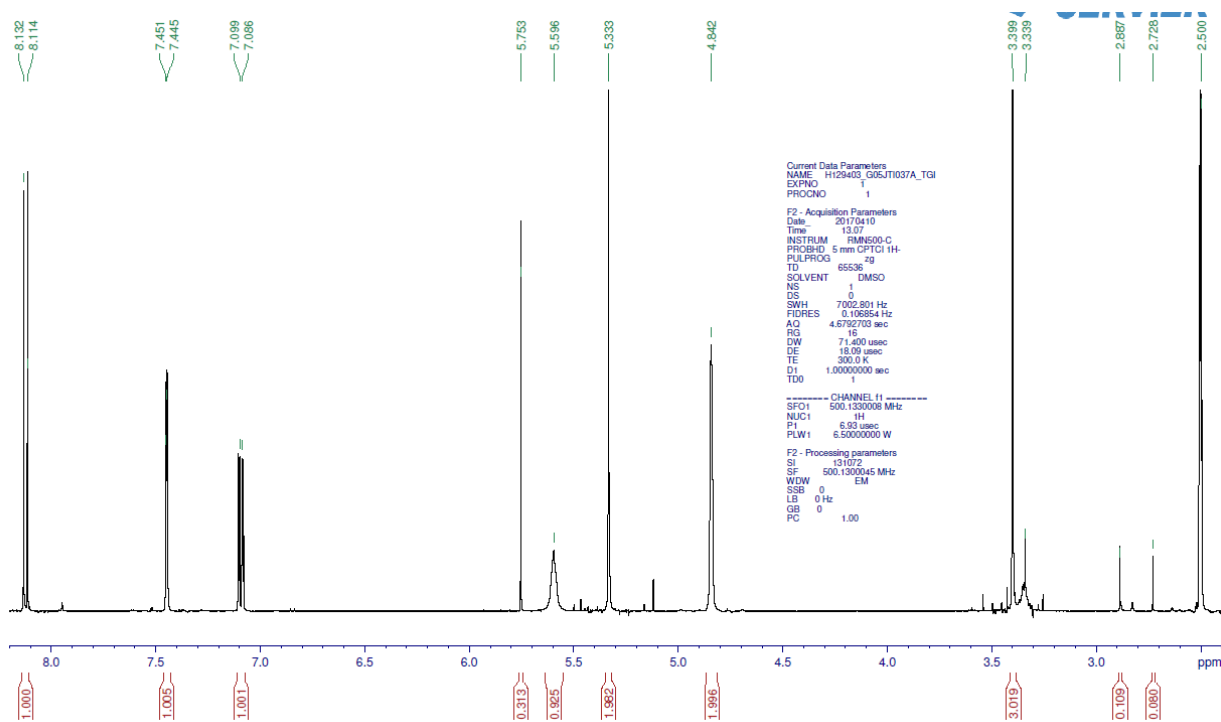
Figure S18. ^1\text{H} -NMR spectrum of 31 measured at 500 MHz in DMSO- d_6
