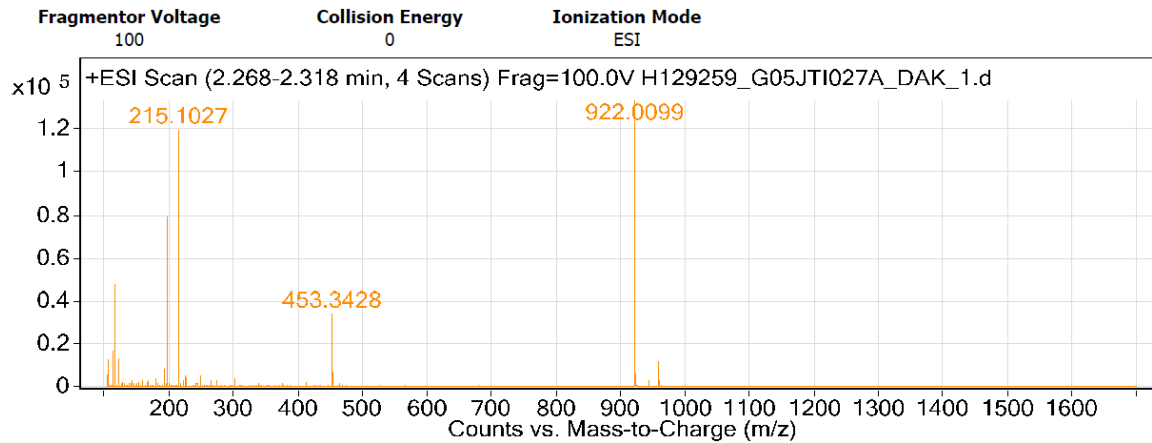
Figure S13. HRMS spectrum of 28
