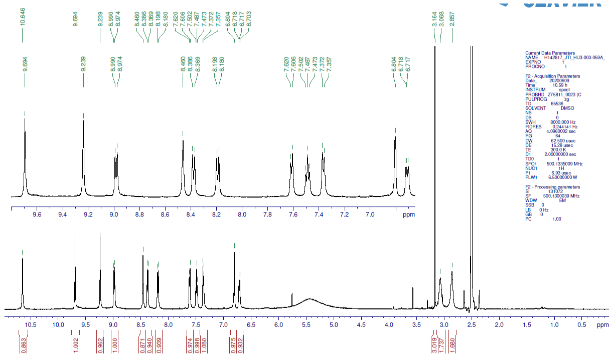
Figure S38. 1 H-NMR spectrum of 26 measured at 500 MHz in DMSO-d 6
