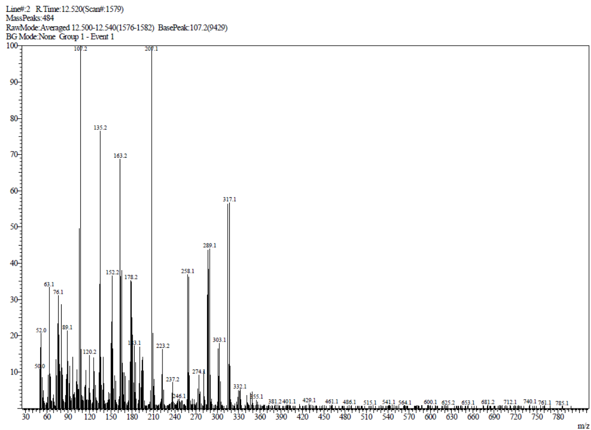
Figure S1. MS spectrum of 20
