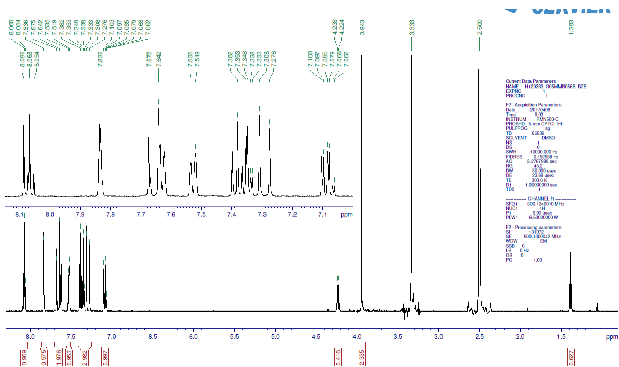
Figure S2. ^1\text{H-NMR} spectrum of 20 measured at 500 MHz in DMSO- d_6
