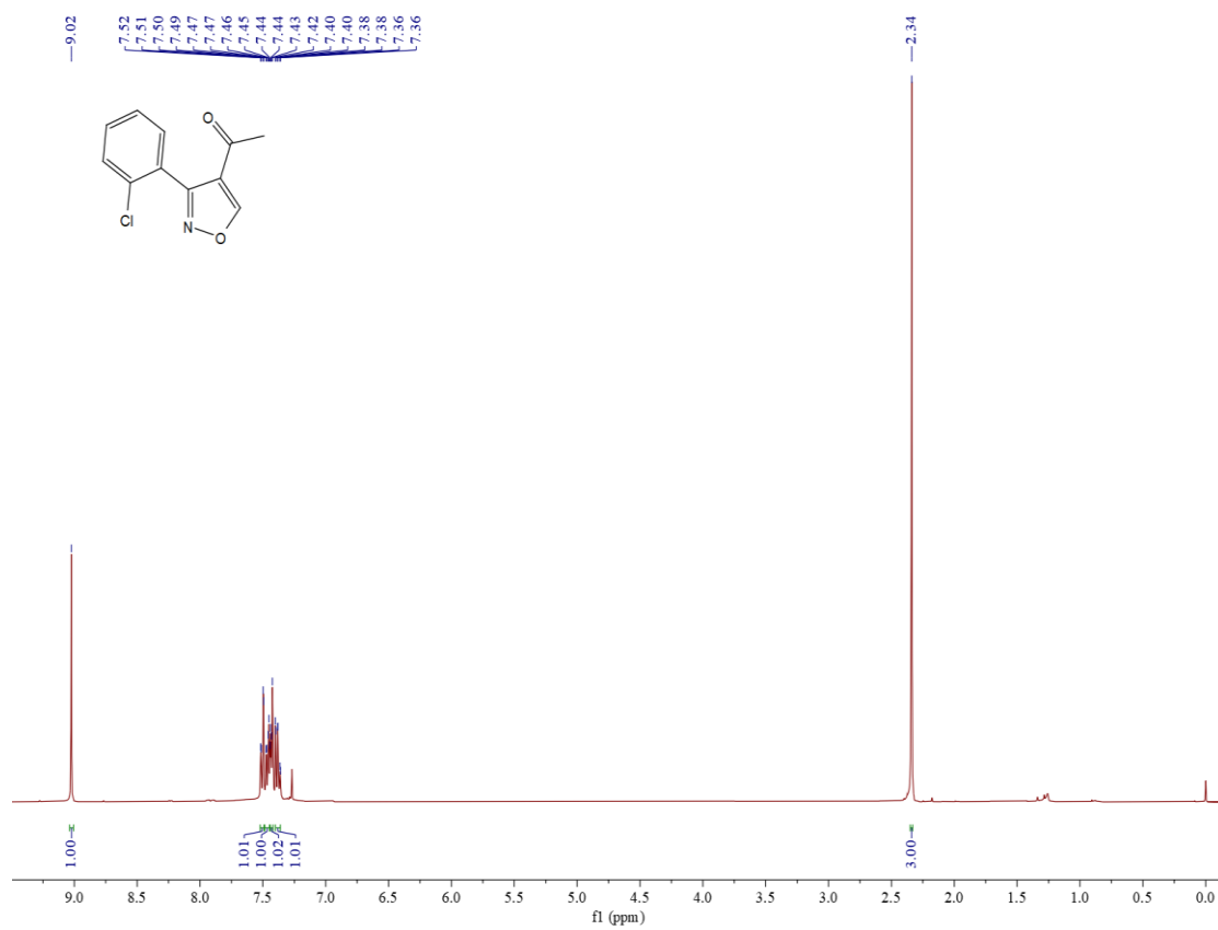
Figure S55 1 H NMR spectrum of compound 5a
