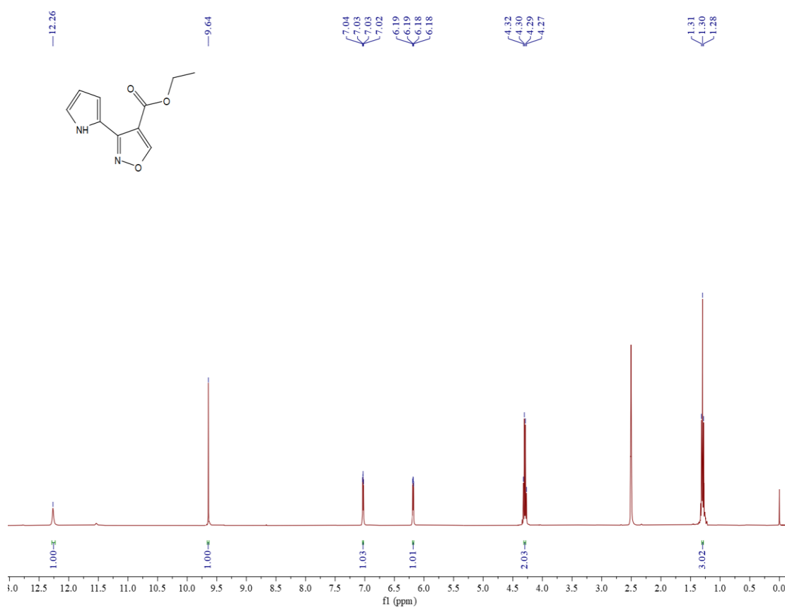
Figure S76 1 H NMR spectrum of compound 5h
