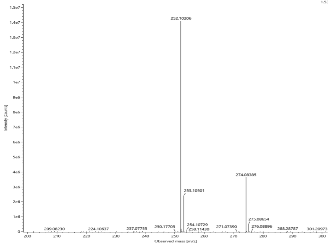
Figure S15 HRMS spectrum of compound 3e
