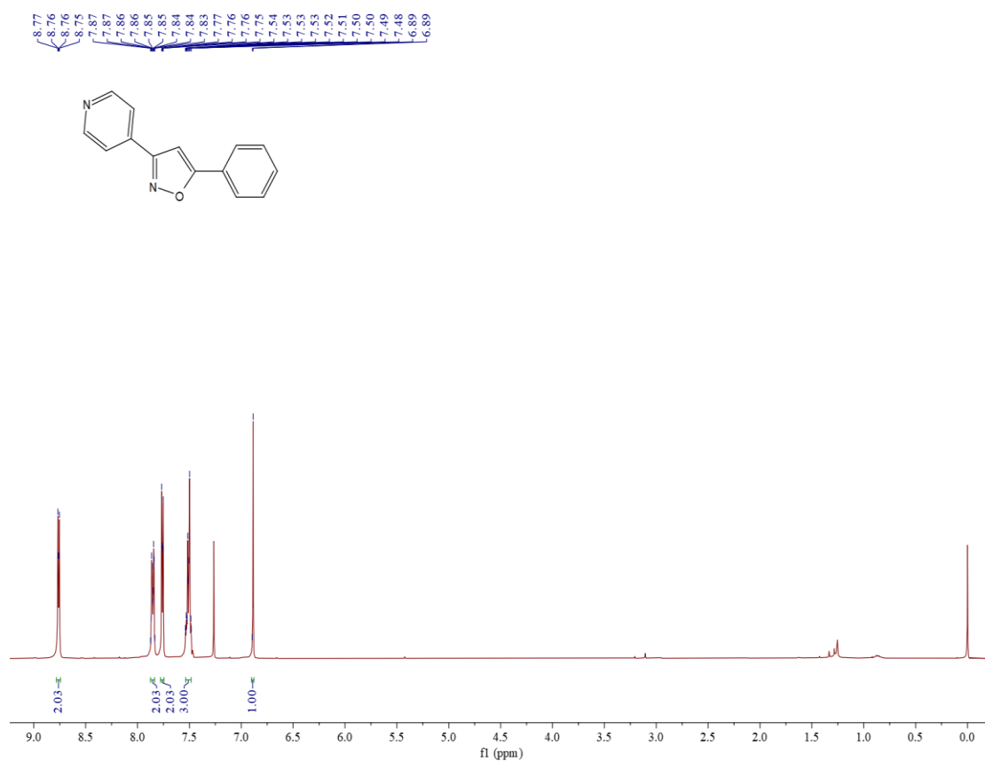
Figure S28 ^1H NMR spectrum of compound 3j
