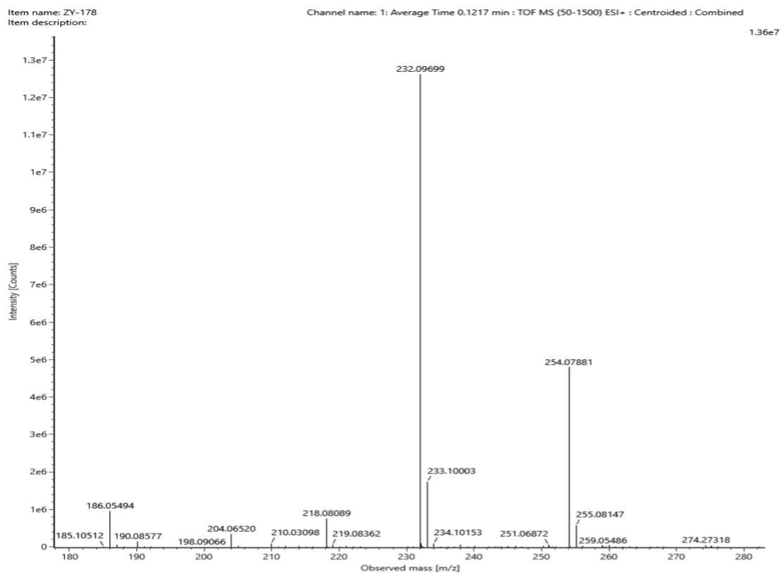
Figure S69 HRMS spectrum of compound 5e
