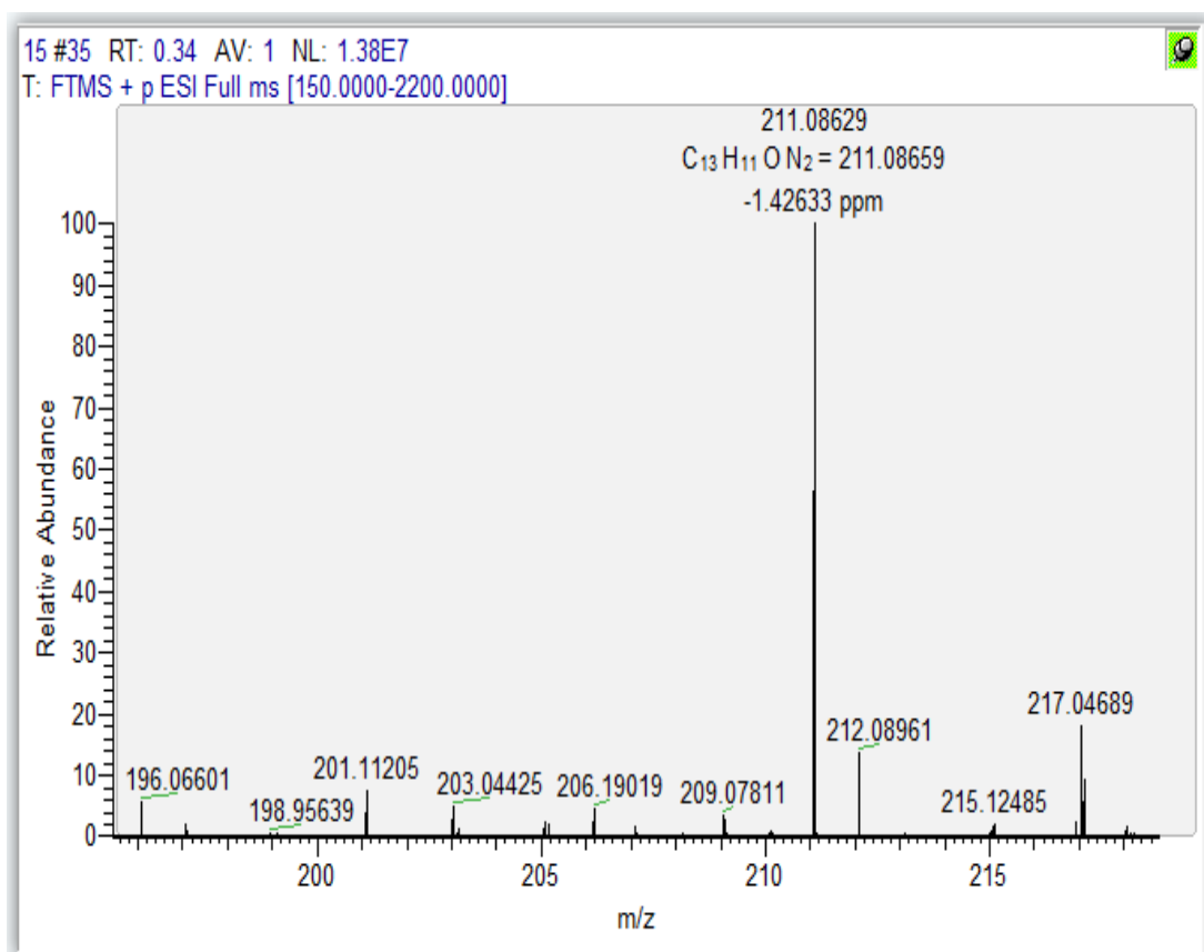
Figure S24 HRMS spectrum of compound 3h
