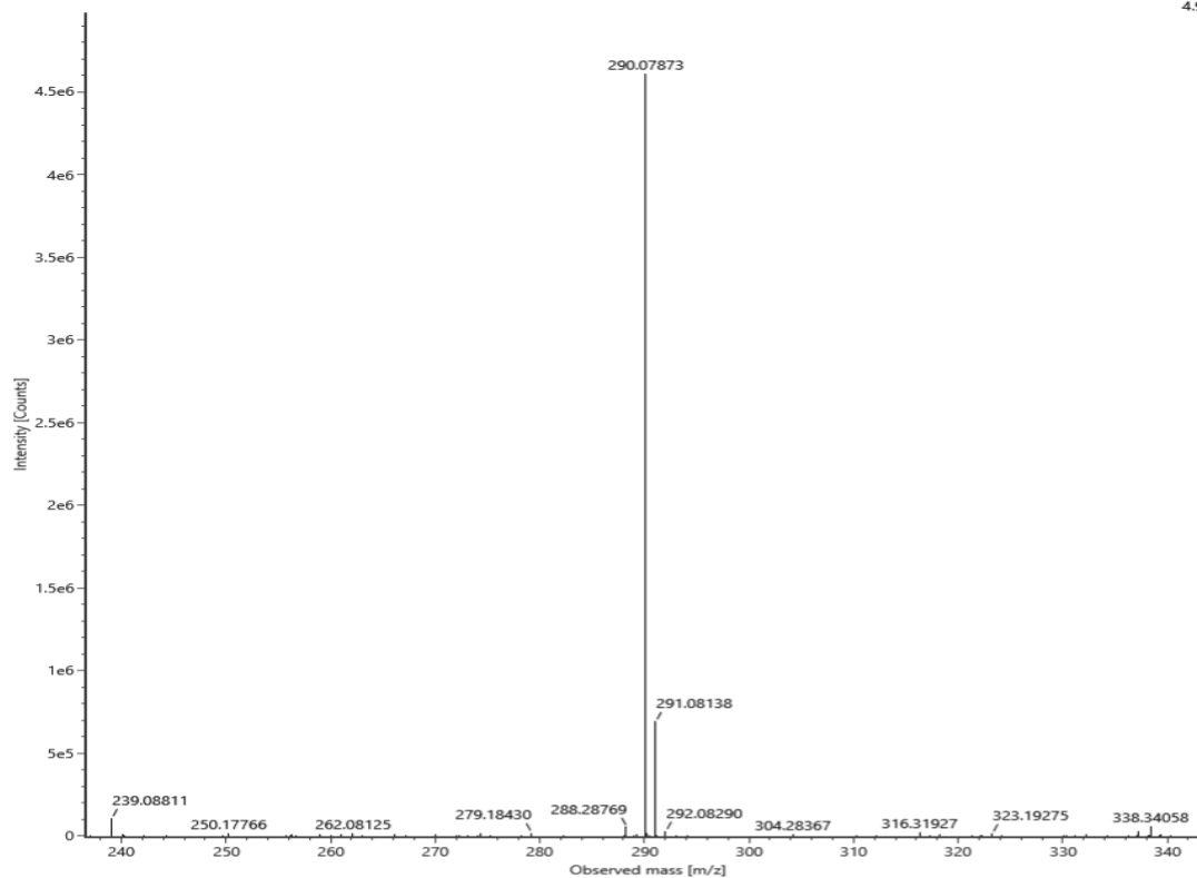
Figure S21 HRMS spectrum of compound 3g
