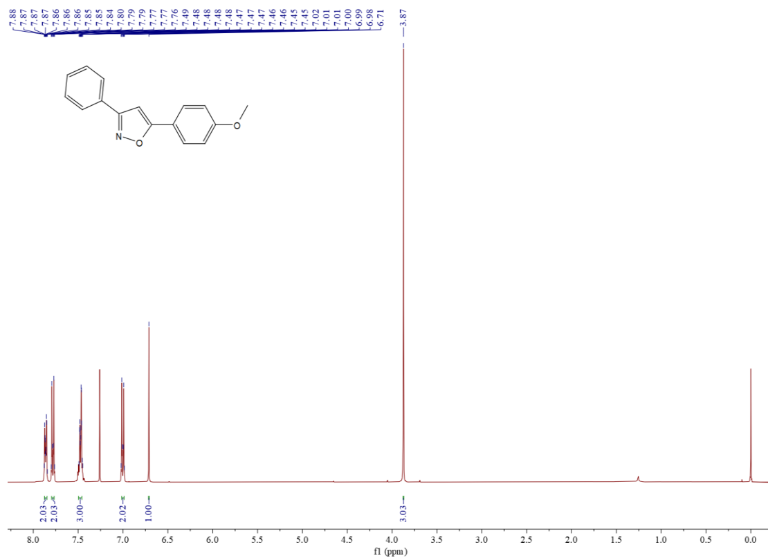
Figure S43 1 H NMR spectrum of compound 3o
