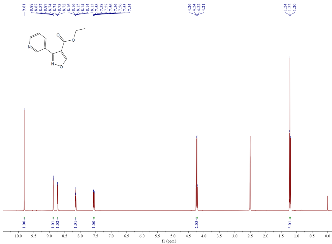
Figure S82 1 H NMR spectrum of compound 5j
