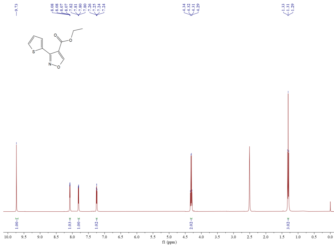
Figure S79 1 H NMR spectrum of compound 5i
