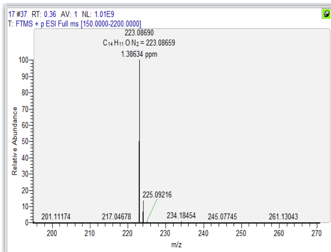
Figure S30 HRMS spectrum of compound 3j
