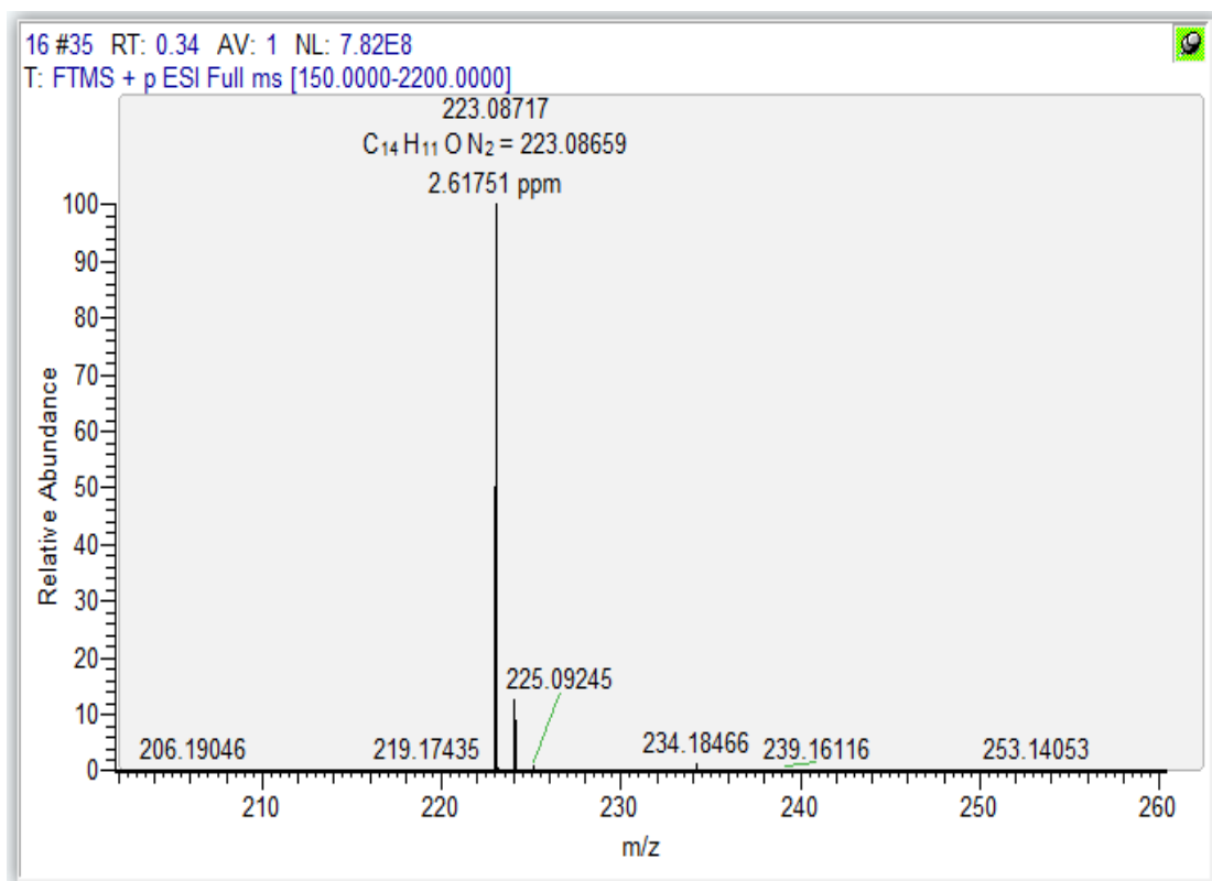
Figure S27 HRMS spectrum of compound 3i
