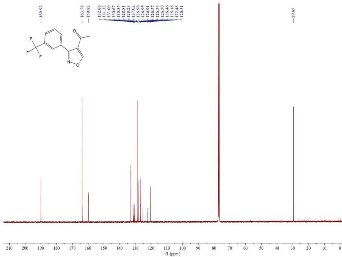
Figure S62 13 C NMR spectrum of compound 5c
