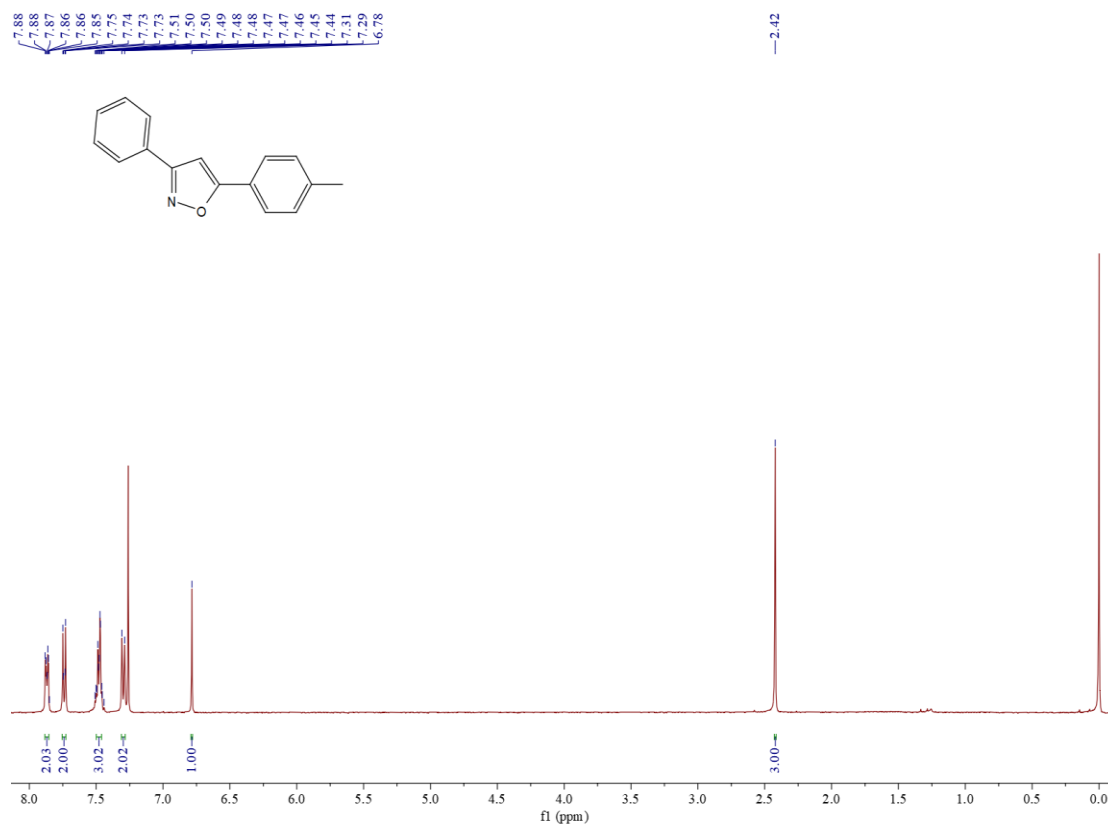
Figure S40 ^1H NMR spectrum of compound 3n
