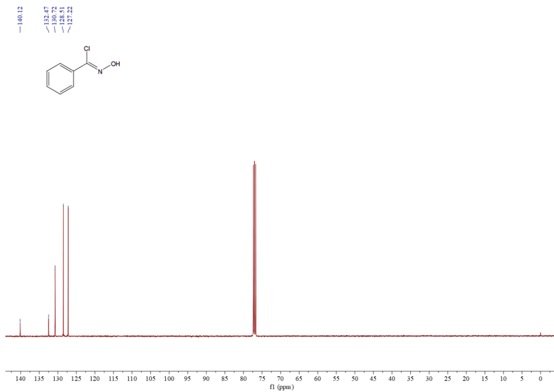
Figure S89 ^{13}\text{C} NMR spectrum of compound 6a
