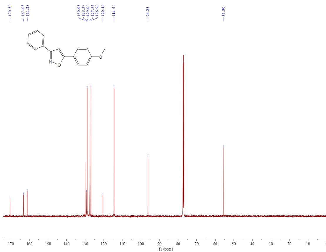
Figure S44 13 C NMR spectrum of compound 3o
