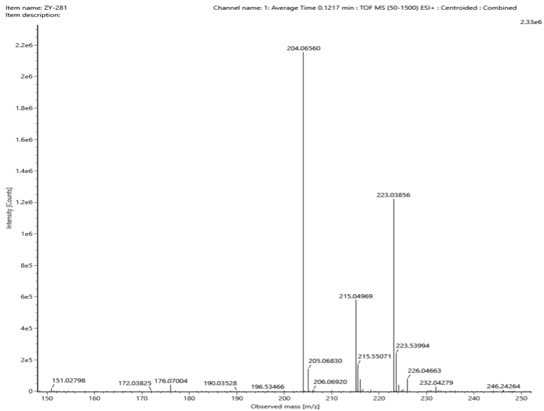
Figure S54 HRMS spectrum of compound 3r
