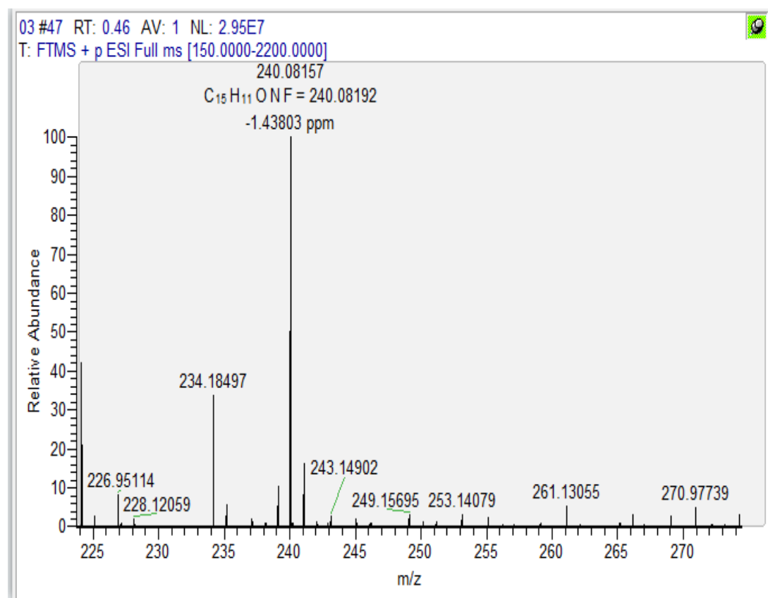
Figure S36 HRMS spectrum of compound 31
