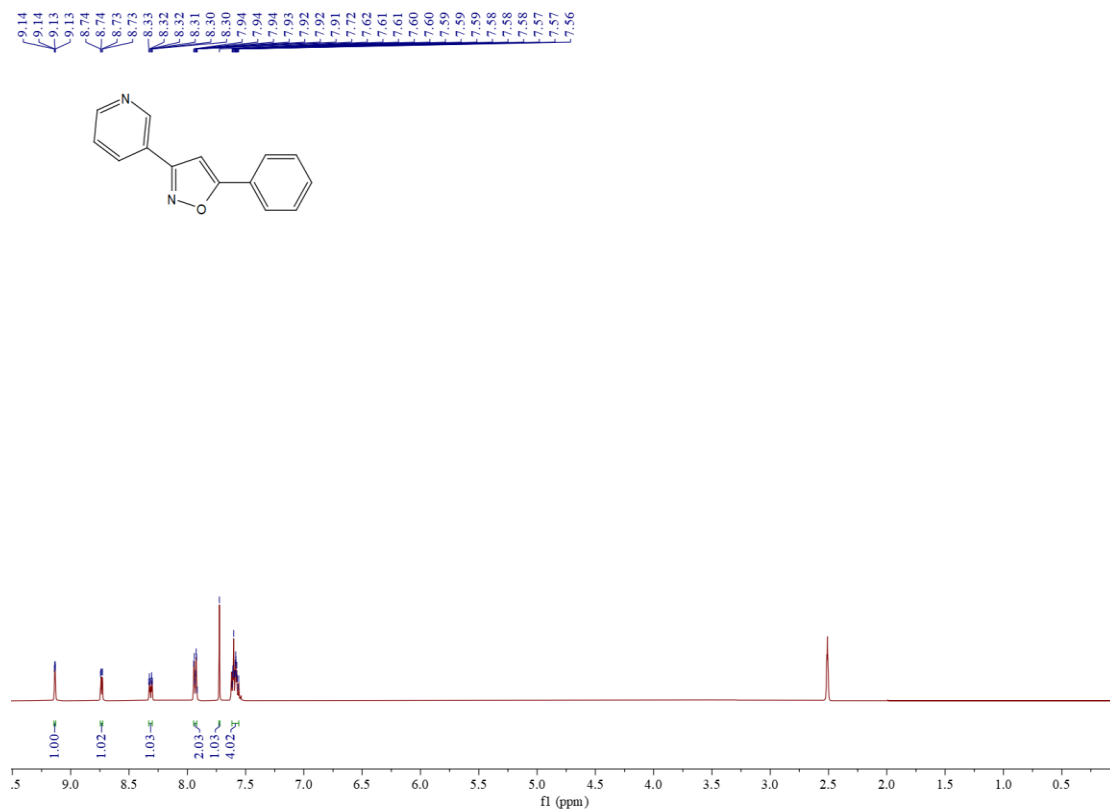
Figure S25 1 H NMR spectrum of compound 3i
