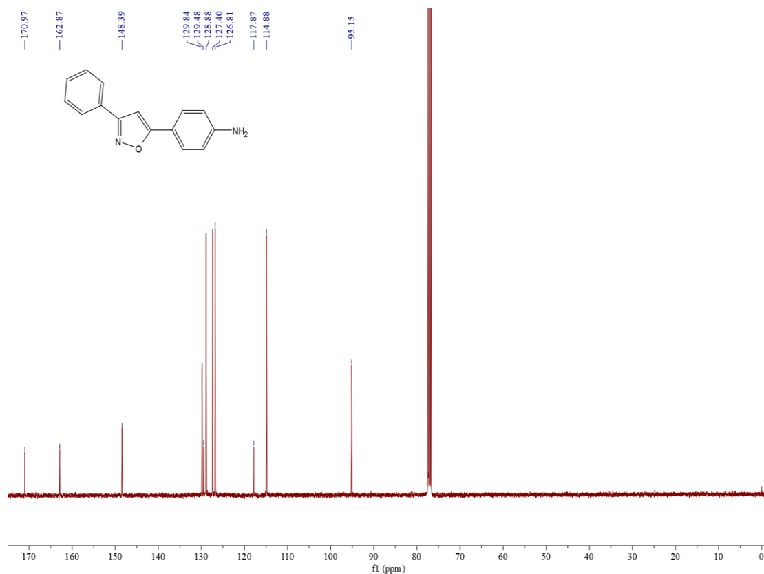
Figure S47 ^{13}\text{C} NMR spectrum of compound 3p
