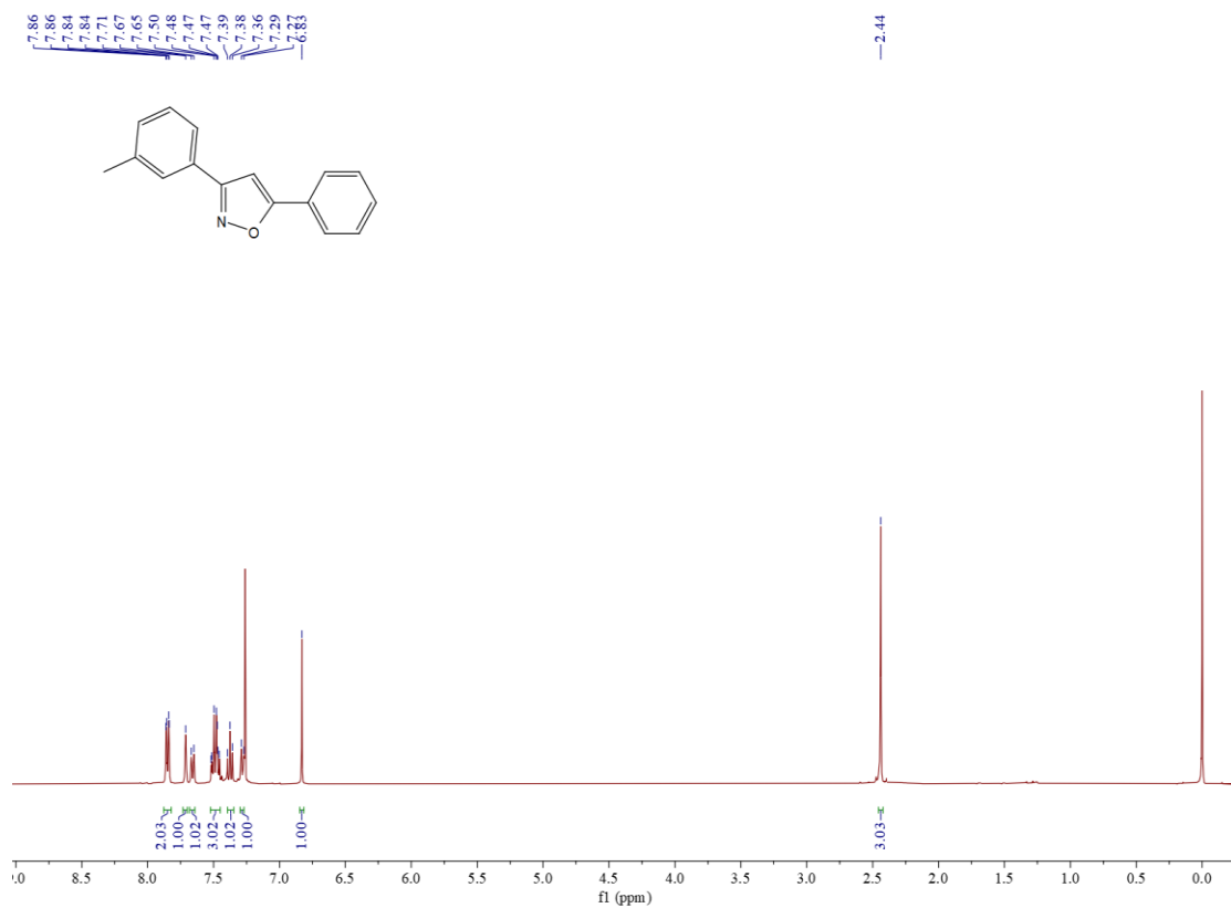
Figure S7 1 H NMR spectrum of compound 3c
