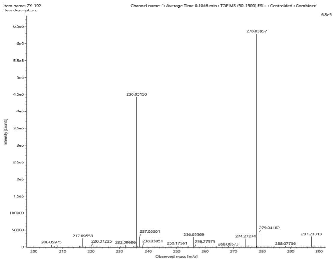
Figure S60 HRMS spectrum of compound 5b
