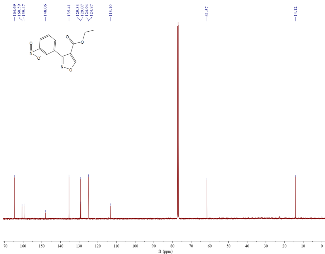
Figure S74 13 C NMR spectrum of compound 5g
