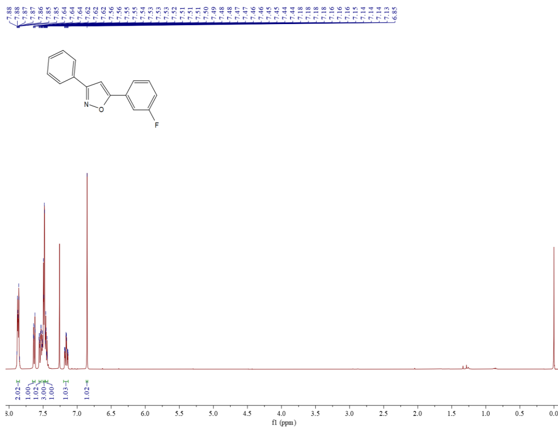
Figure S34 ^1H NMR spectrum of compound 3l
