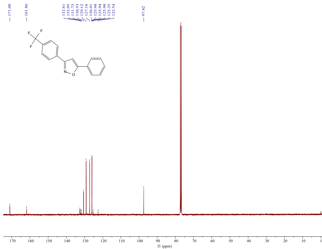
Figure S20 13 C NMR spectrum of compound 3g
