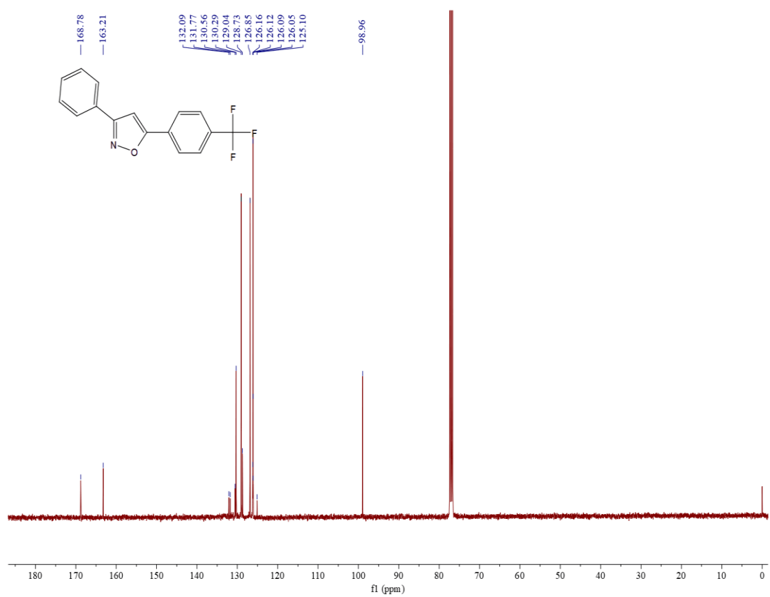
Figure S50 13 C NMR spectrum of compound 3q
