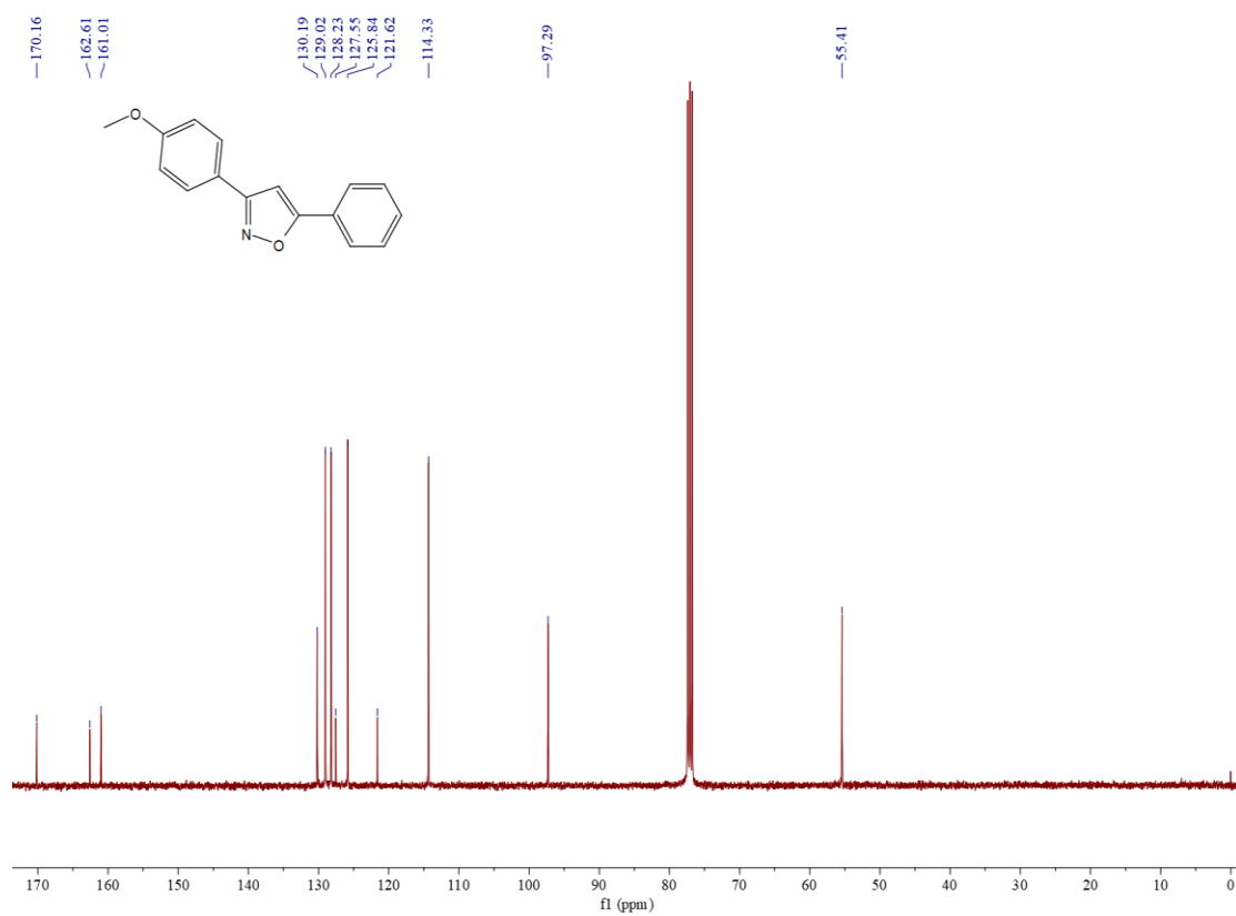
Figure S14 13 C NMR spectrum of compound 3e
