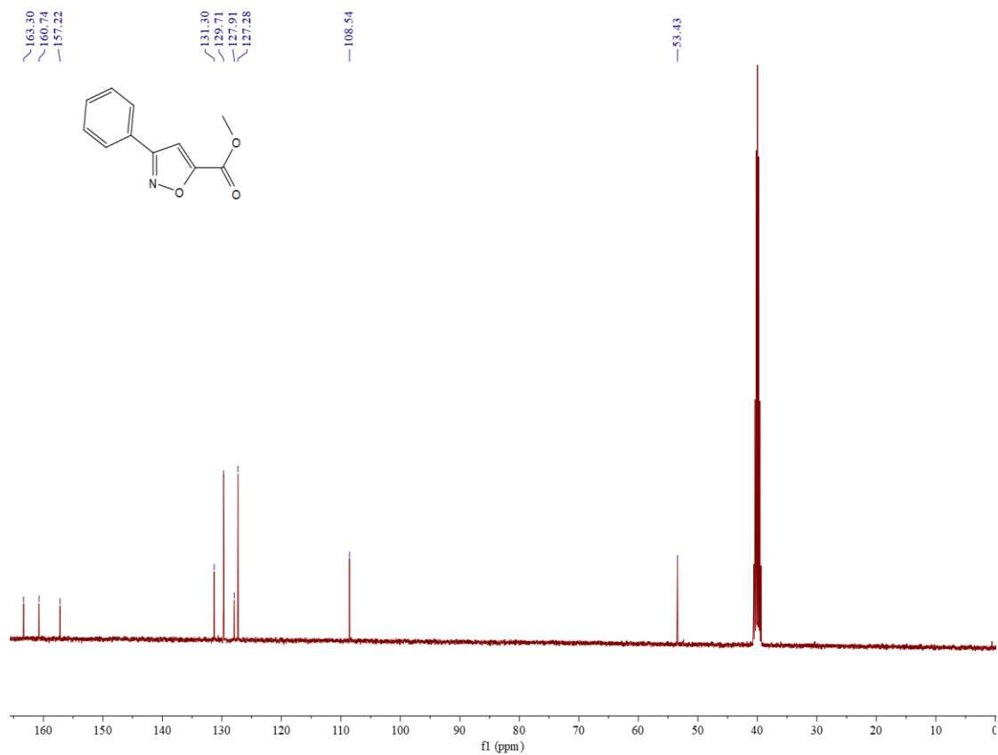
Figure S53 13 C NMR spectrum of compound 3r
