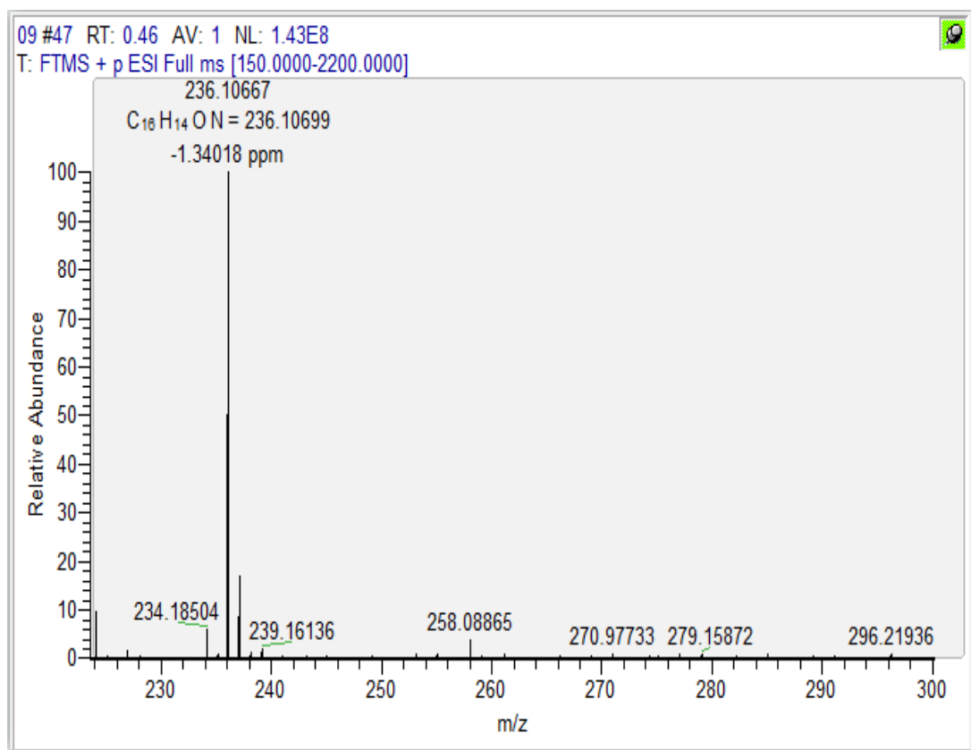
Figure S12 HRMS spectrum of compound 3d
