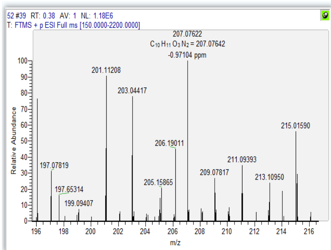
Figure S78 HRMS spectrum of compound 5h
