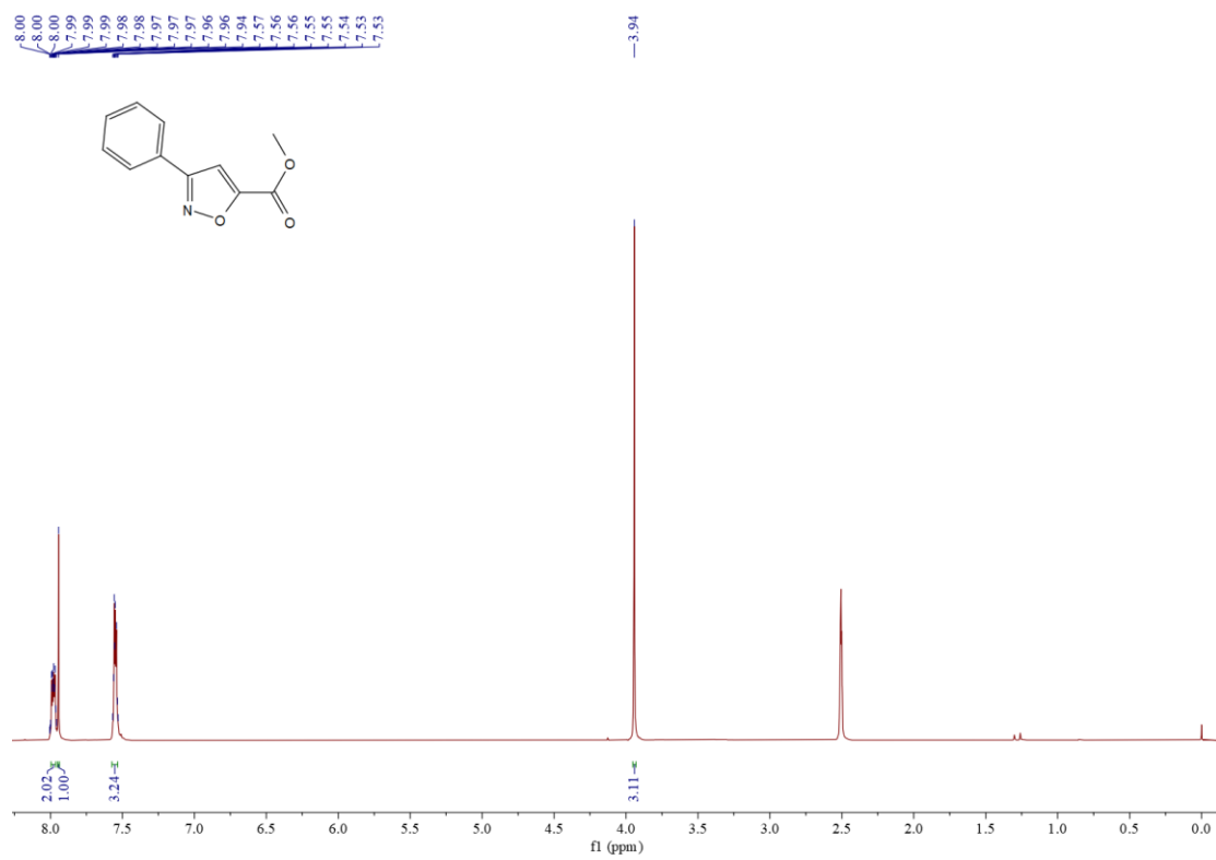
Figure S52 ^1H NMR spectrum of compound 3r
