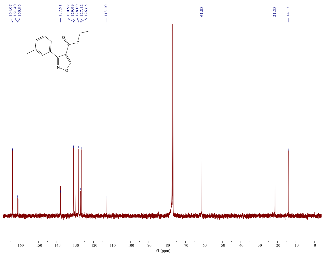
Figure S68 13 C NMR spectrum of compound 5e
