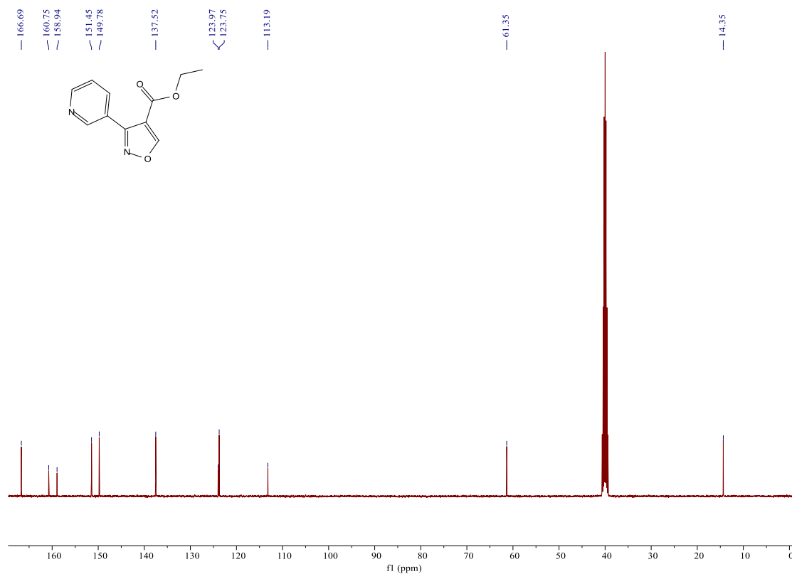
Figure S83 13 C NMR spectrum of compound 5j
