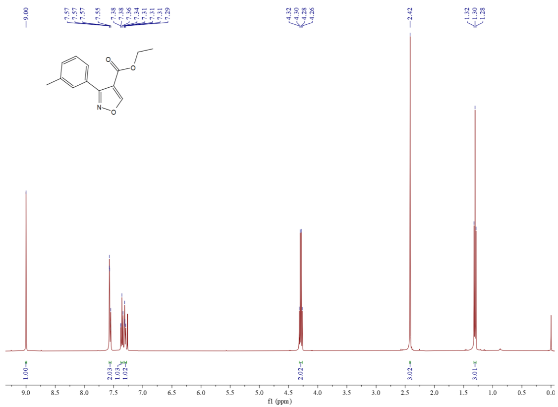
Figure S67 1 H NMR spectrum of compound 5e
