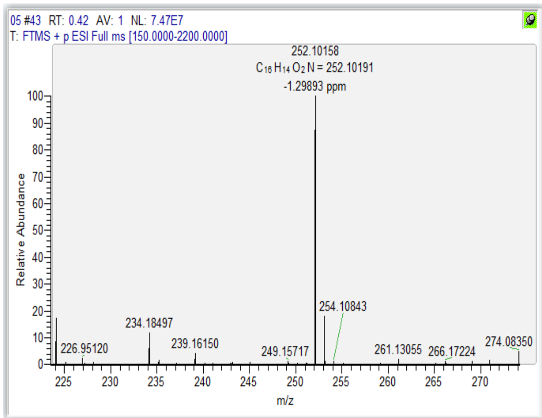
Figure S45 HRMS spectrum of compound 3o
