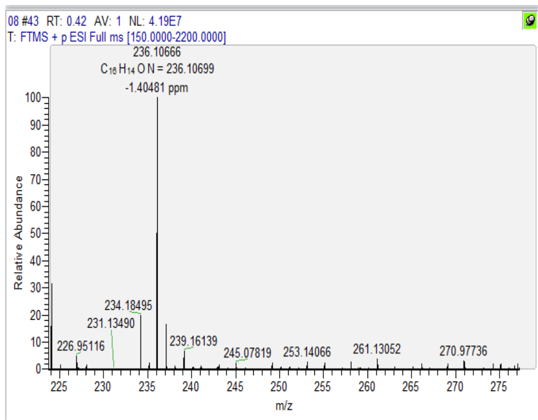
Figure S9 HRMS spectrum of compound 3c
