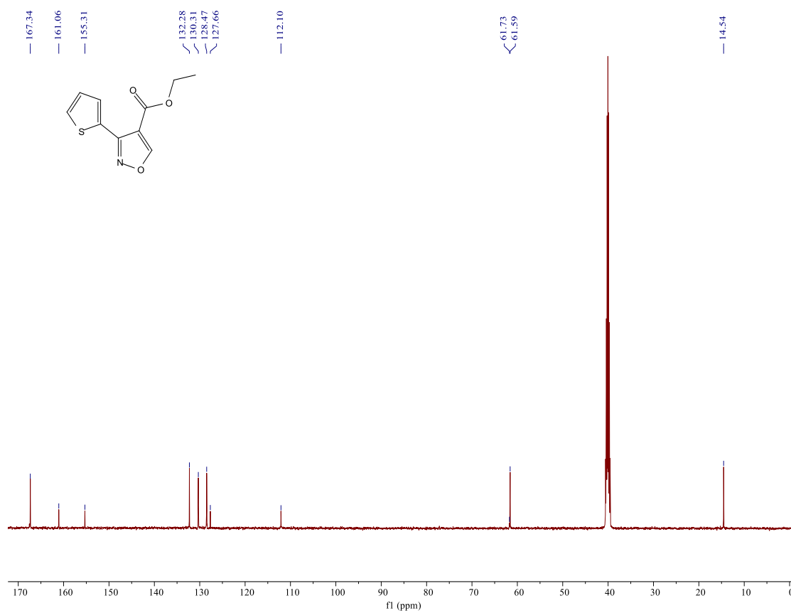
Figure S80 13 C NMR spectrum of compound 5i
