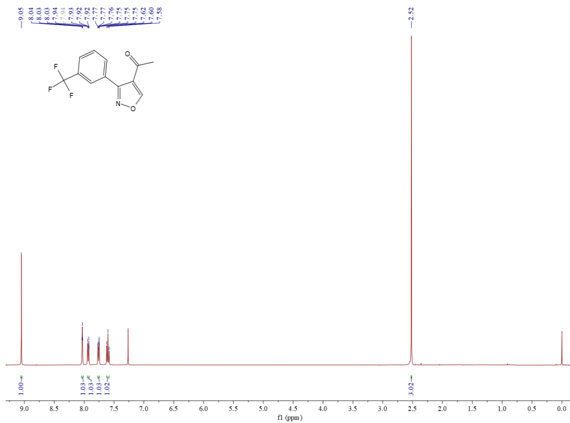
Figure S61 1 H NMR spectrum of compound 5c
