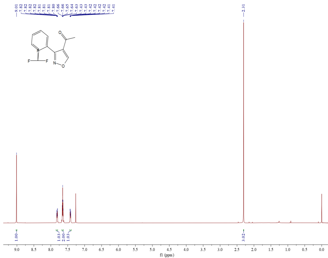
Figure S58 1 H NMR spectrum of compound 5b
