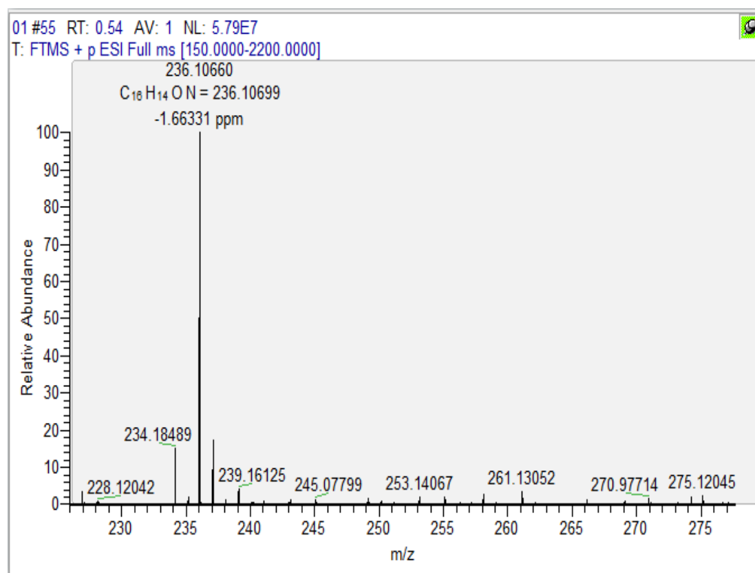
Figure S42 HRMS spectrum of compound 3n
