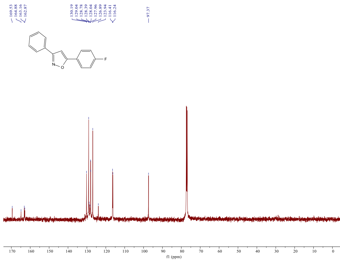
Figure S38 13 C NMR spectrum of compound 3m
