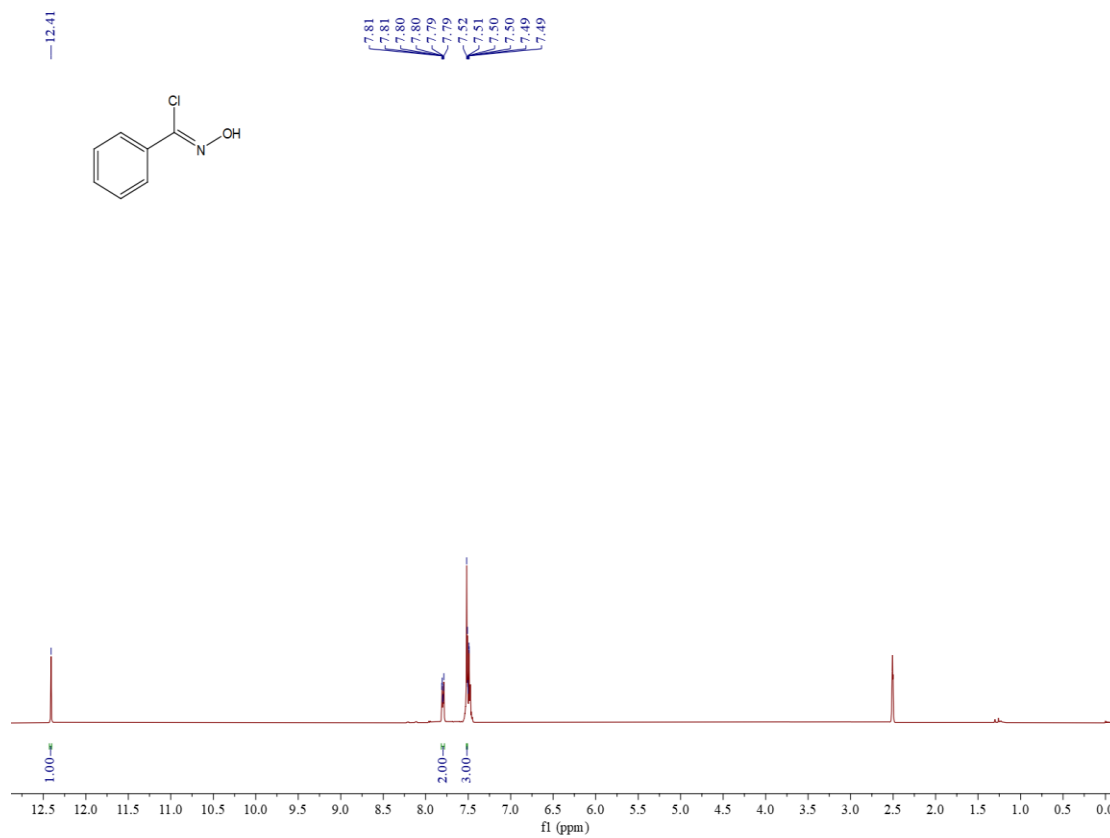
Figure S88 ^1H NMR spectrum of compound 6a
