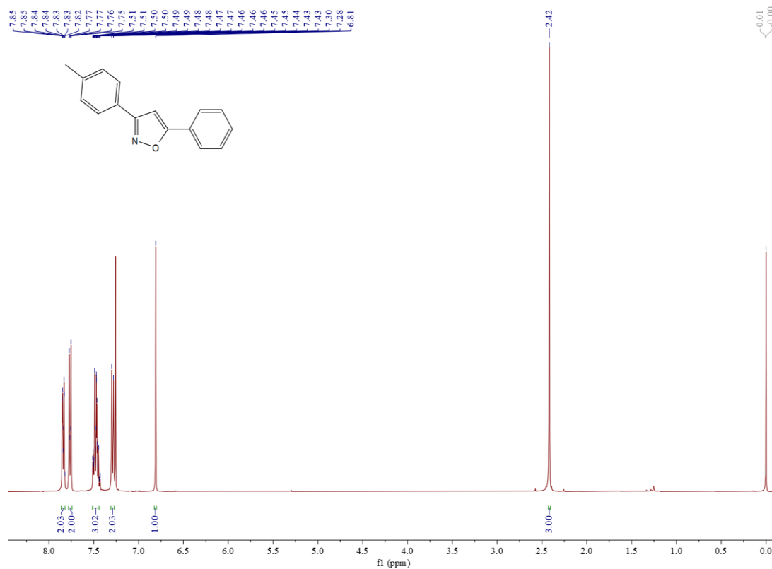
Figure S10 ^1H NMR spectrum of compound 3d
