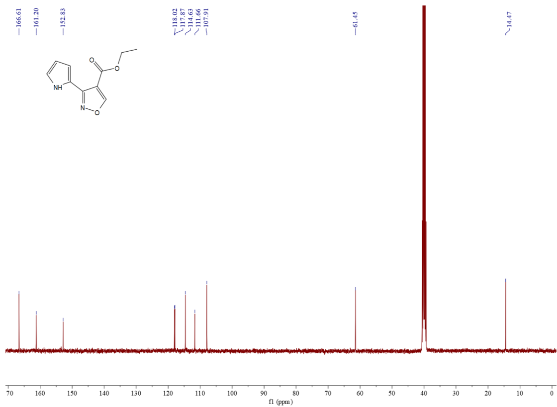
Figure S77 13 C NMR spectrum of compound 5h
