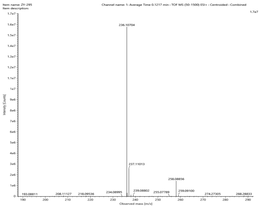
Figure S6 HRMS spectrum of compound 3b
