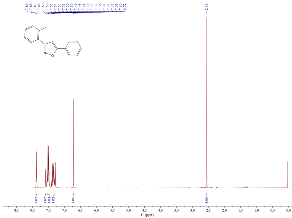
Figure S4 1 H NMR spectrum of compound 3b
