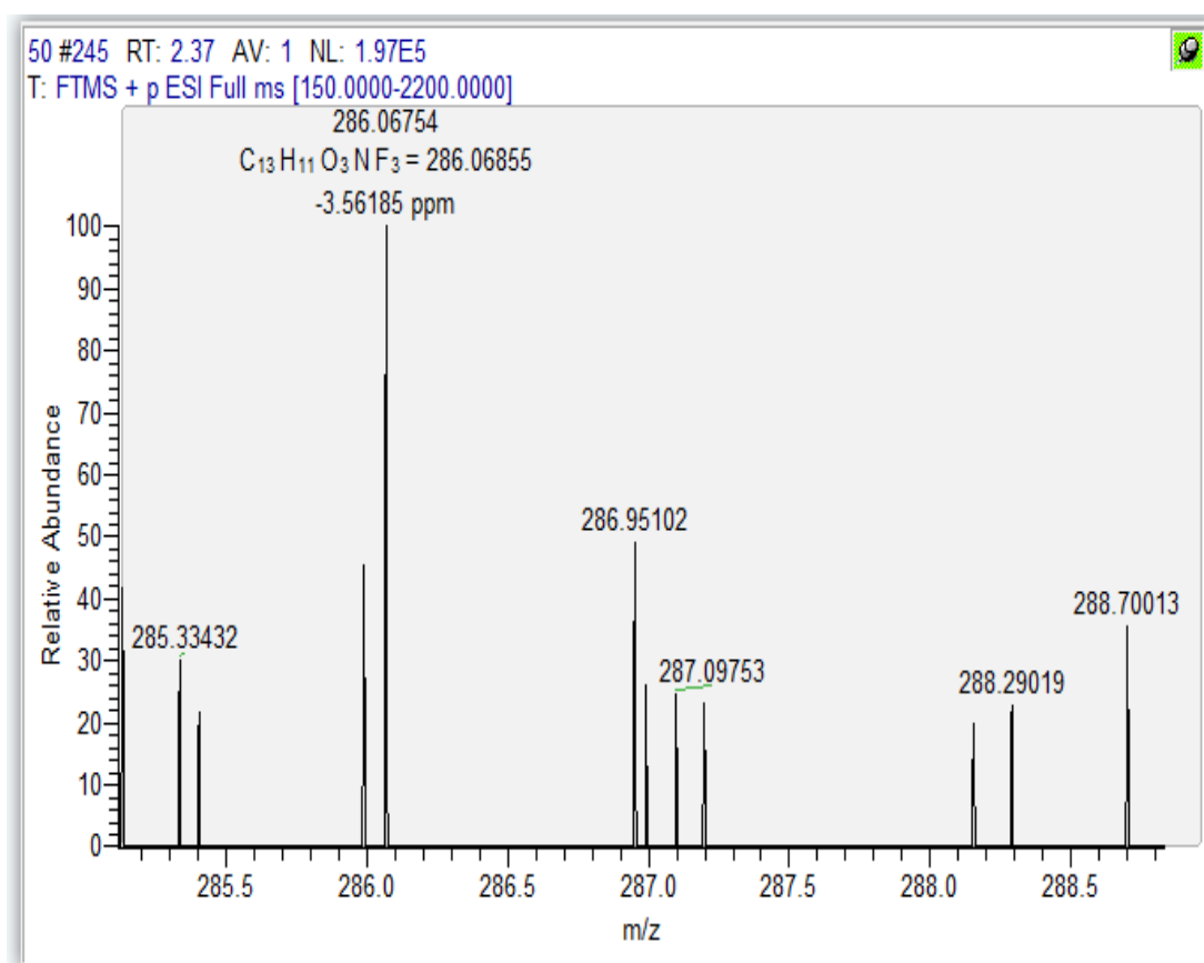
Figure S72 HRMS spectrum of compound 5f
