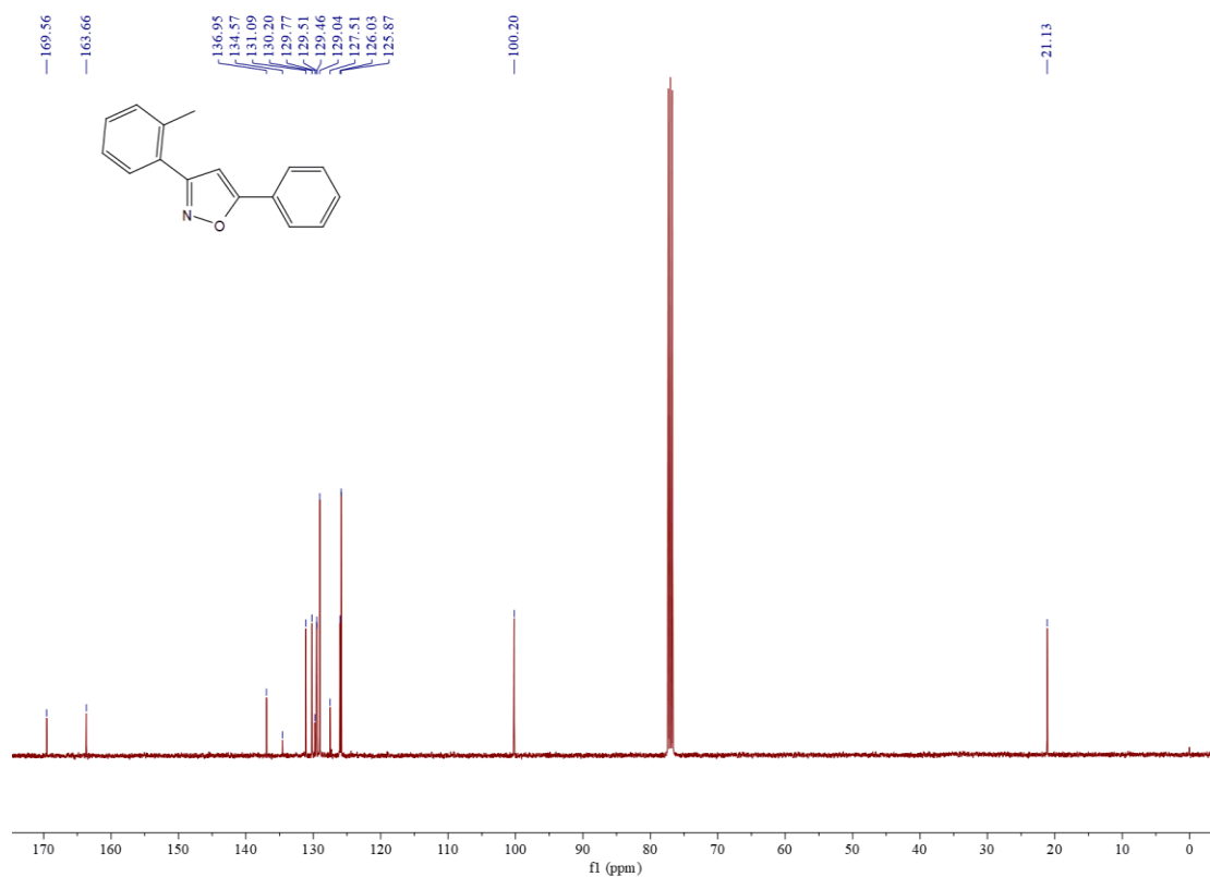
Figure S5 13 C NMR spectrum of compound 3b
