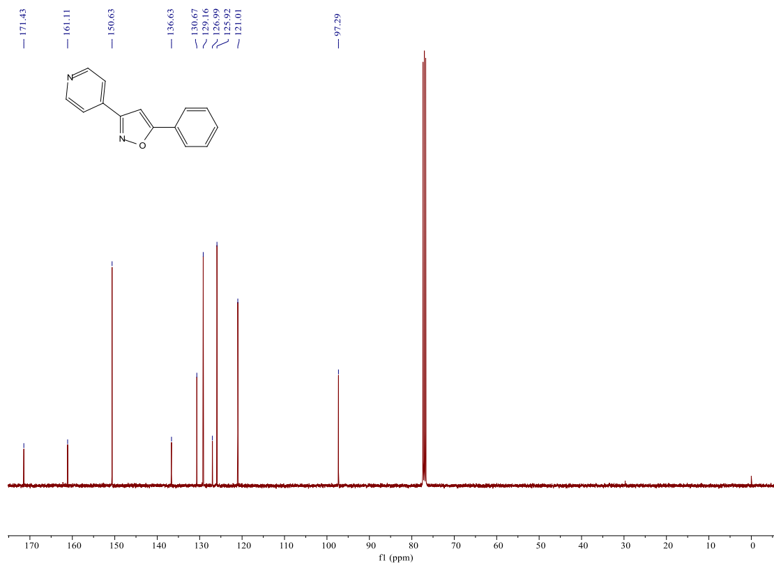
Figure S29 13 C NMR spectrum of compound 3j
