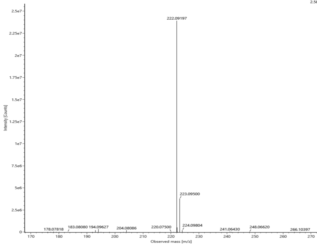
Figure S3 HRMS spectrum of compound 3a
