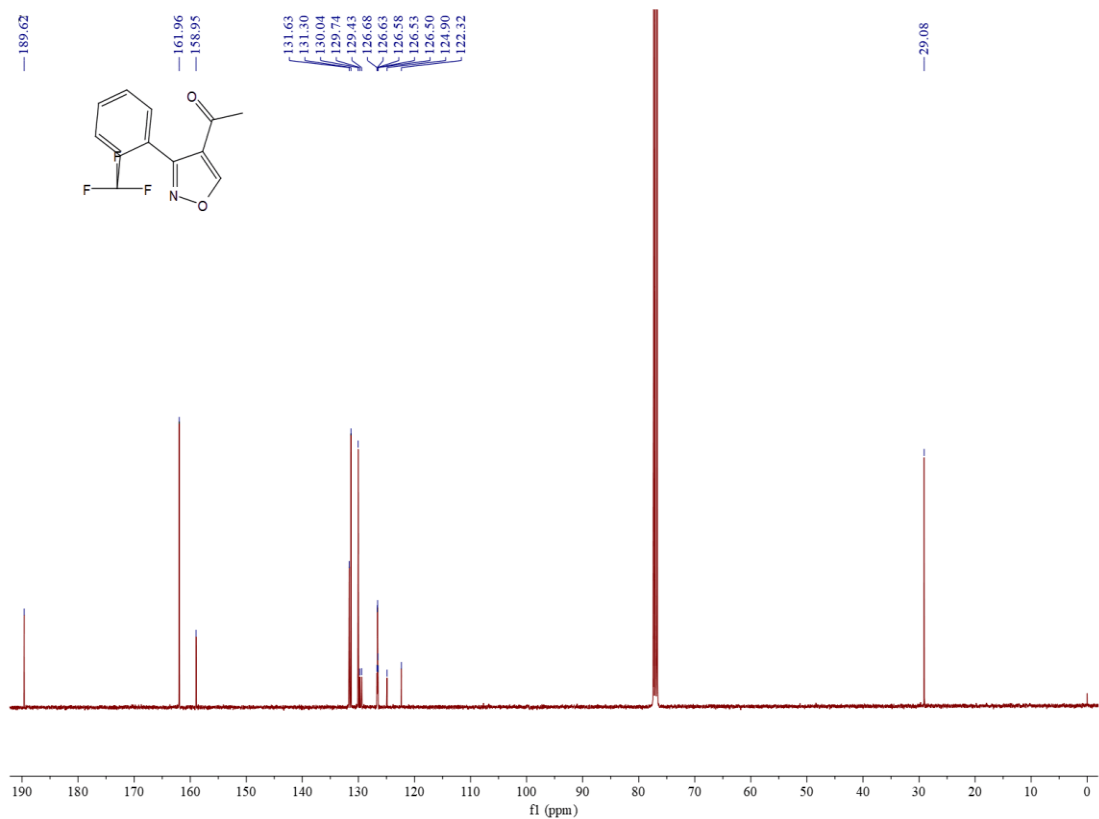
Figure S59 13 C NMR spectrum of compound 5b
