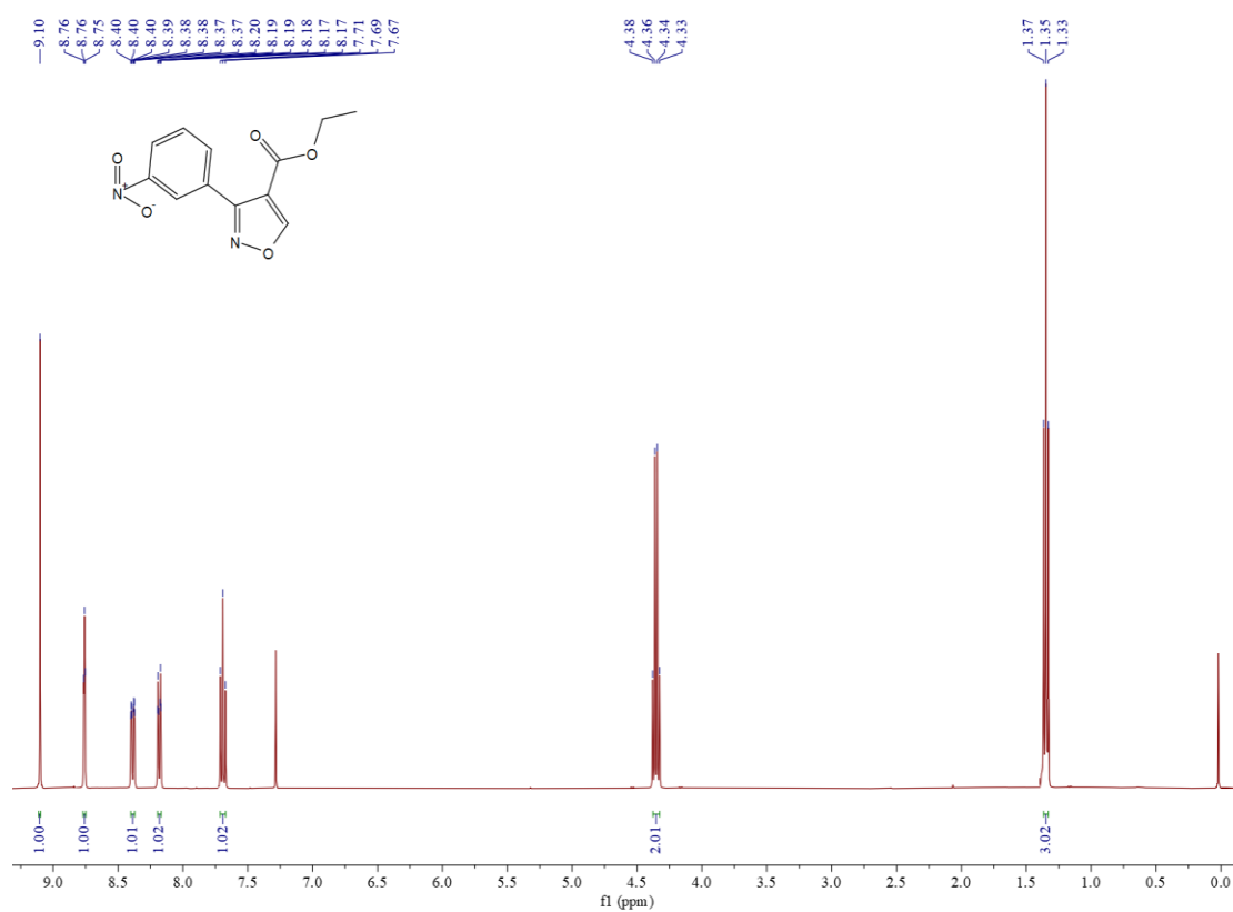
Figure S73 1 H NMR spectrum of compound 5g
