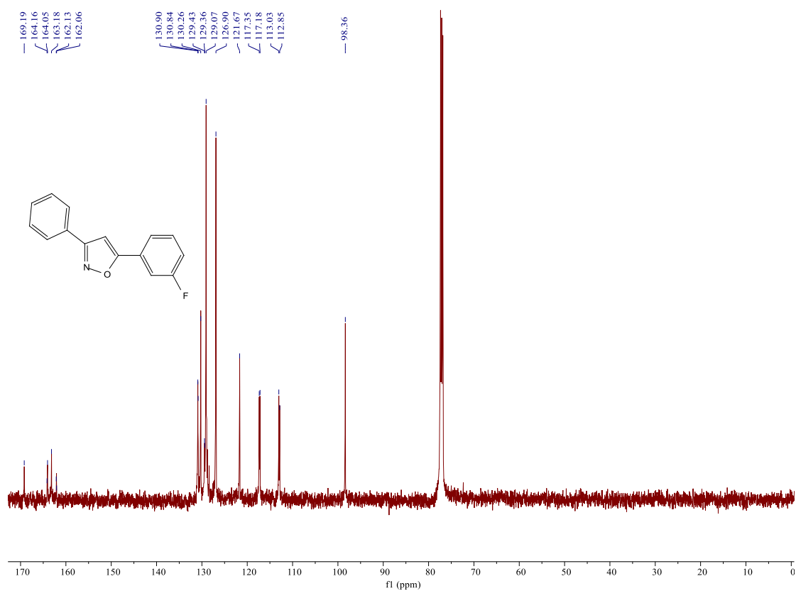
Figure S35 13 C NMR spectrum of compound 31
