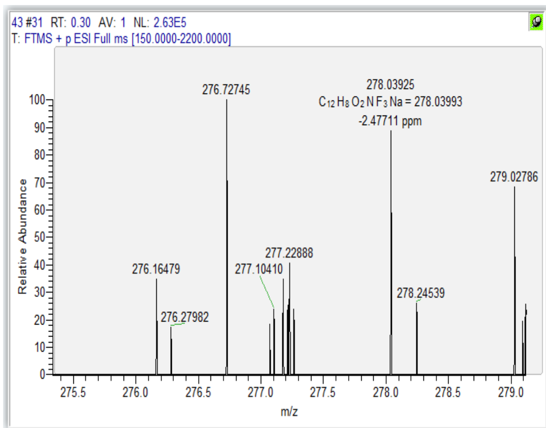
Figure S63 HRMS spectrum of compound 5c
