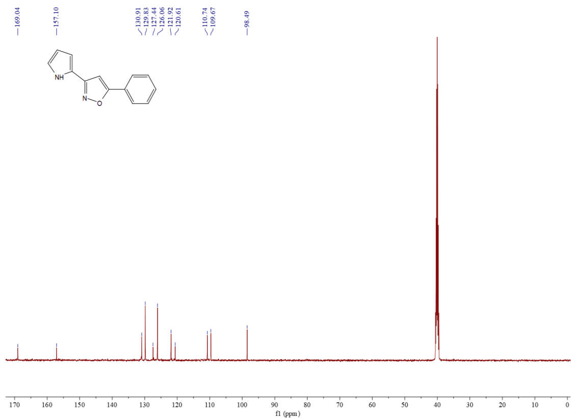
Figure S23 13 C NMR spectrum of compound 3h
