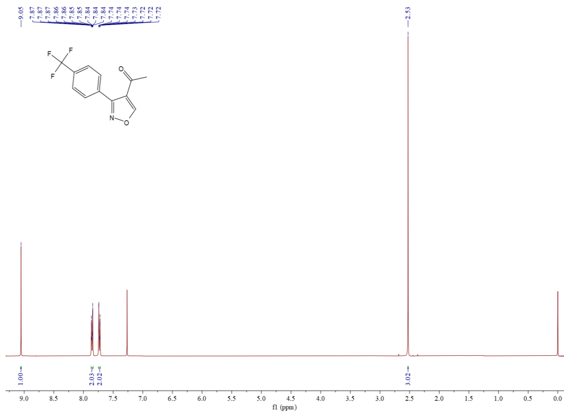
Figure S64 ^1H NMR spectrum of compound 5d
