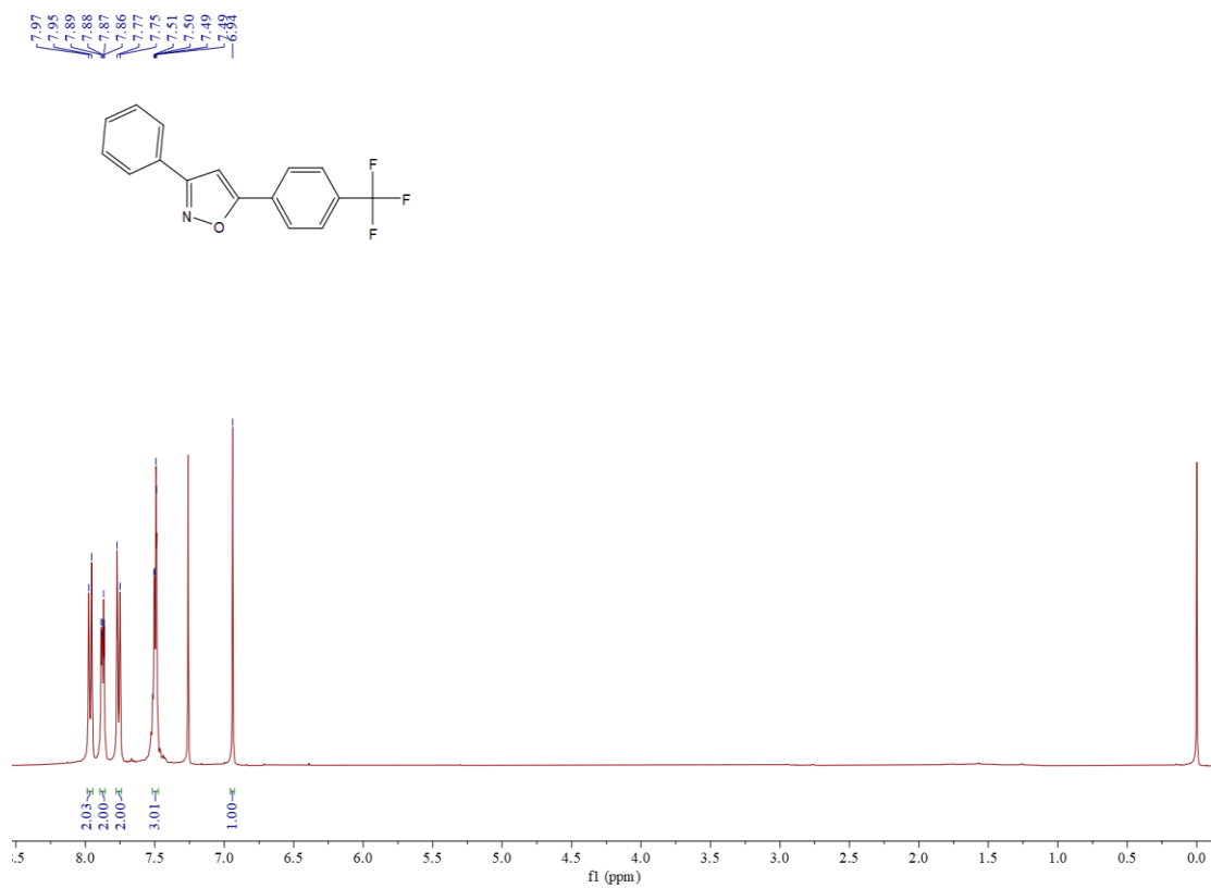
Figure S49 1 H NMR spectrum of compound 3q
