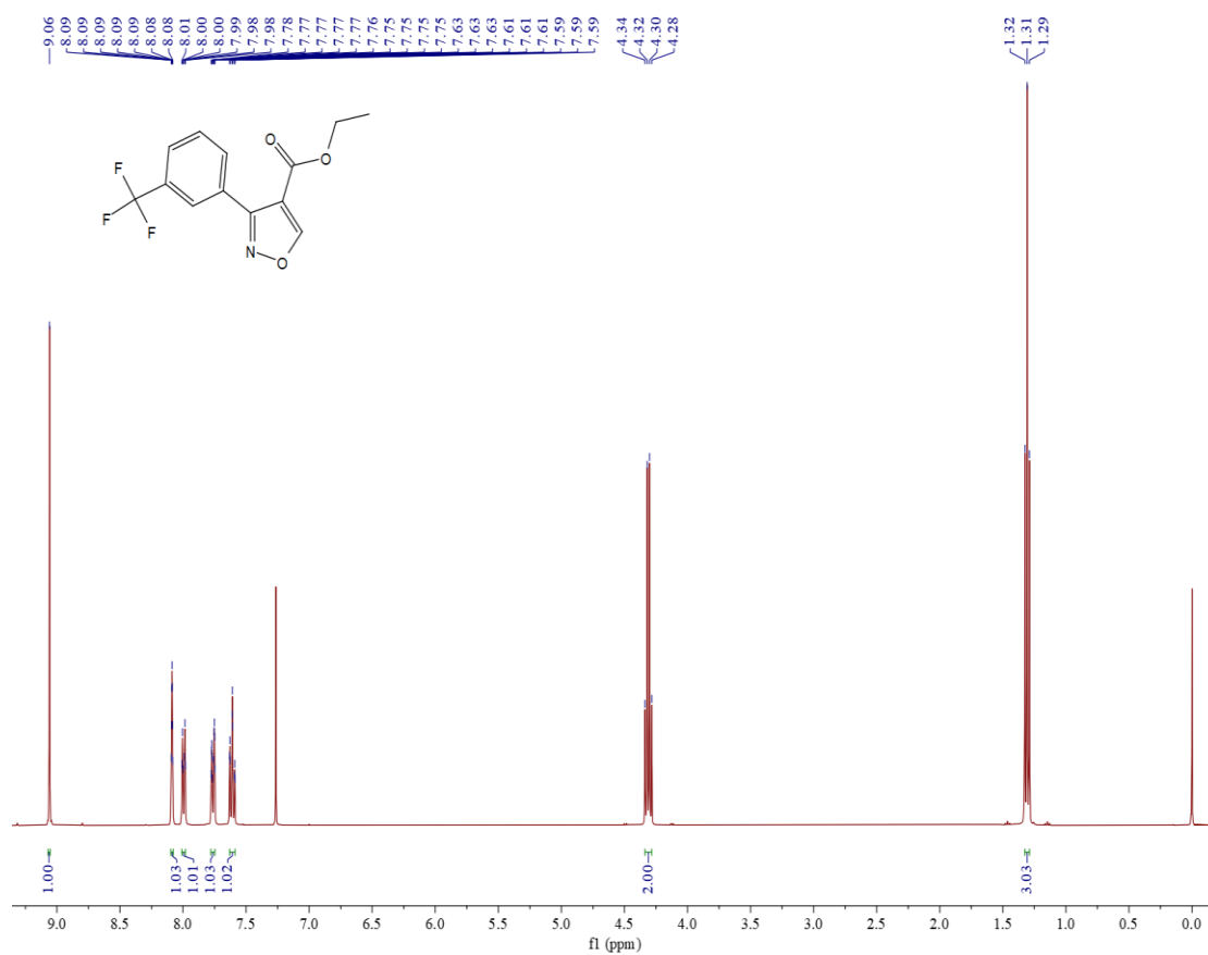
Figure S70 1 H NMR spectrum of compound 5f
