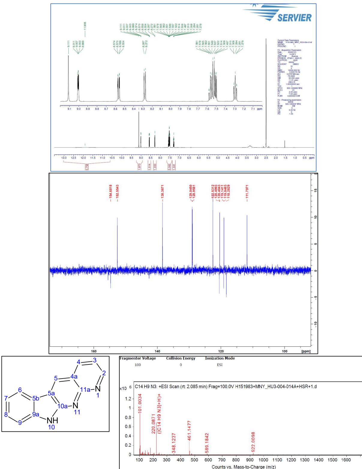
Figure S23. 1 H-NMR and 13 C-NMR and HRMS spectrum of 6a 3,7-10 H -Indolo[2,3- b ][1,8]naphthyridine
