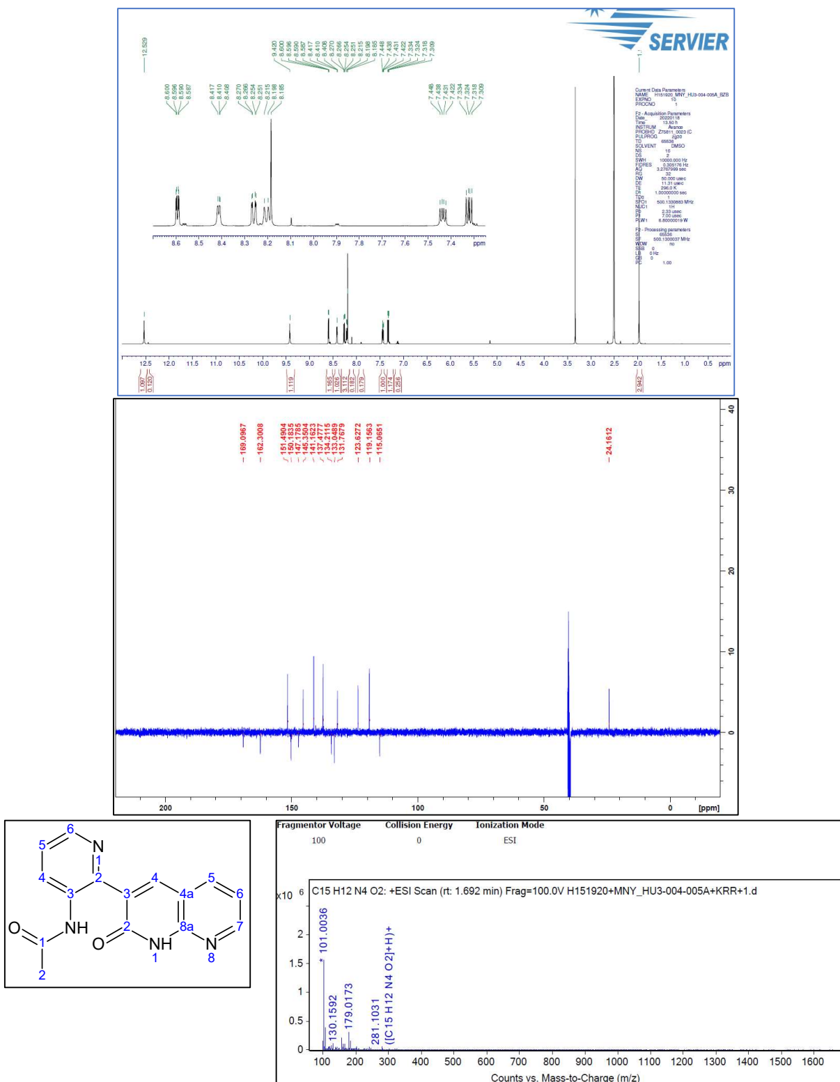
Figure S47. 1 H-NMR and 13 C-NMR and HRMS spectrum of 11e N -[2-(2-Oxo-1,2-dihydro-1,8-naphthyridin-3-yl)pyridin-3-yl]acetamide
