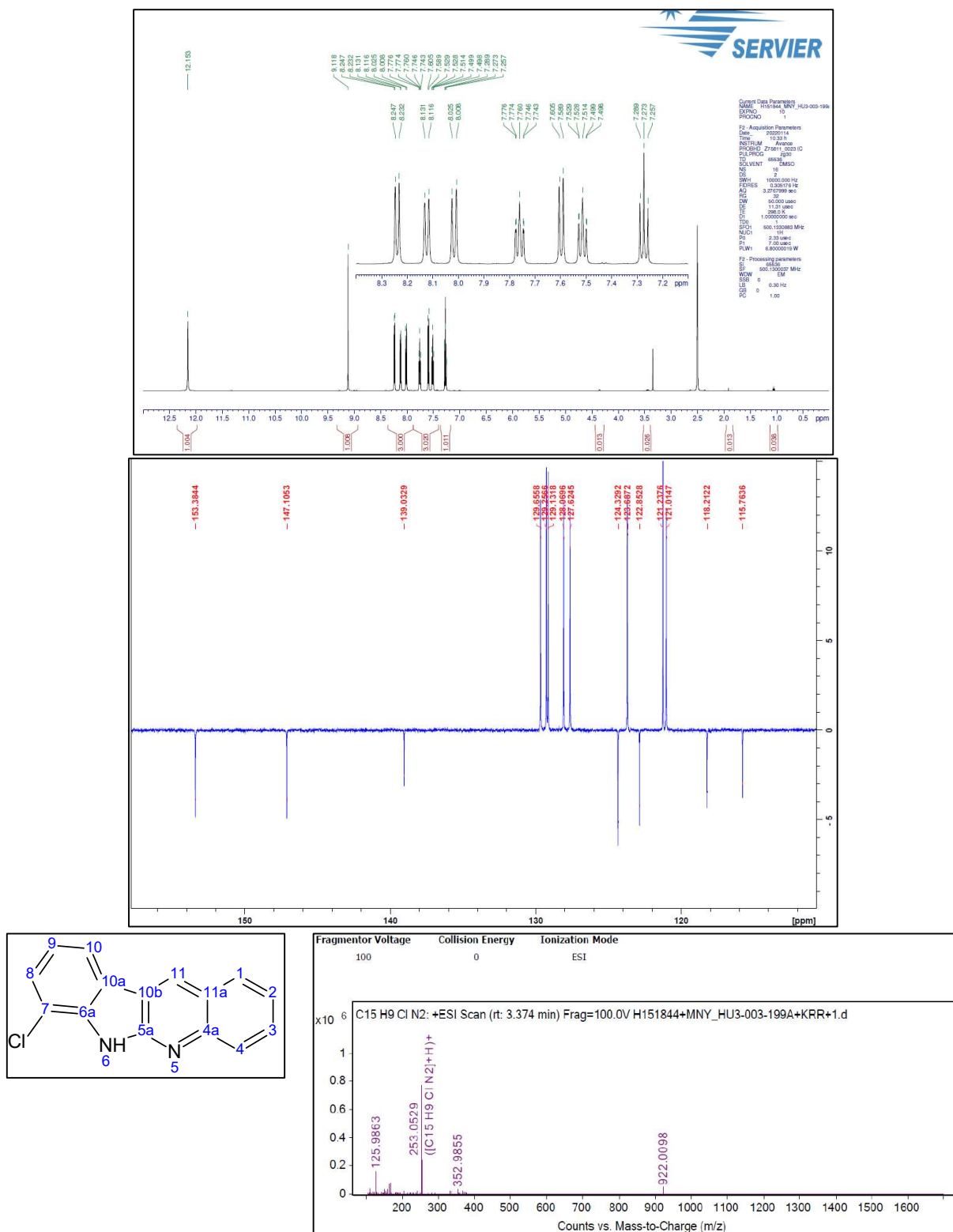
Figure S5. 1 H-NMR and 13 C-NMR and HRMS spectrum of 4b 7-Chloro-6H-indolo[2,3-b]quinoline
