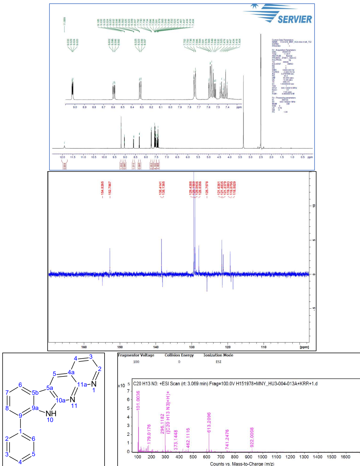
Figure S29. 1 H-NMR and 13 C-NMR and HRMS spectrum of 6g 9-Phenyl-10H-indolo[2,3-b][1,8]naphthyridine
