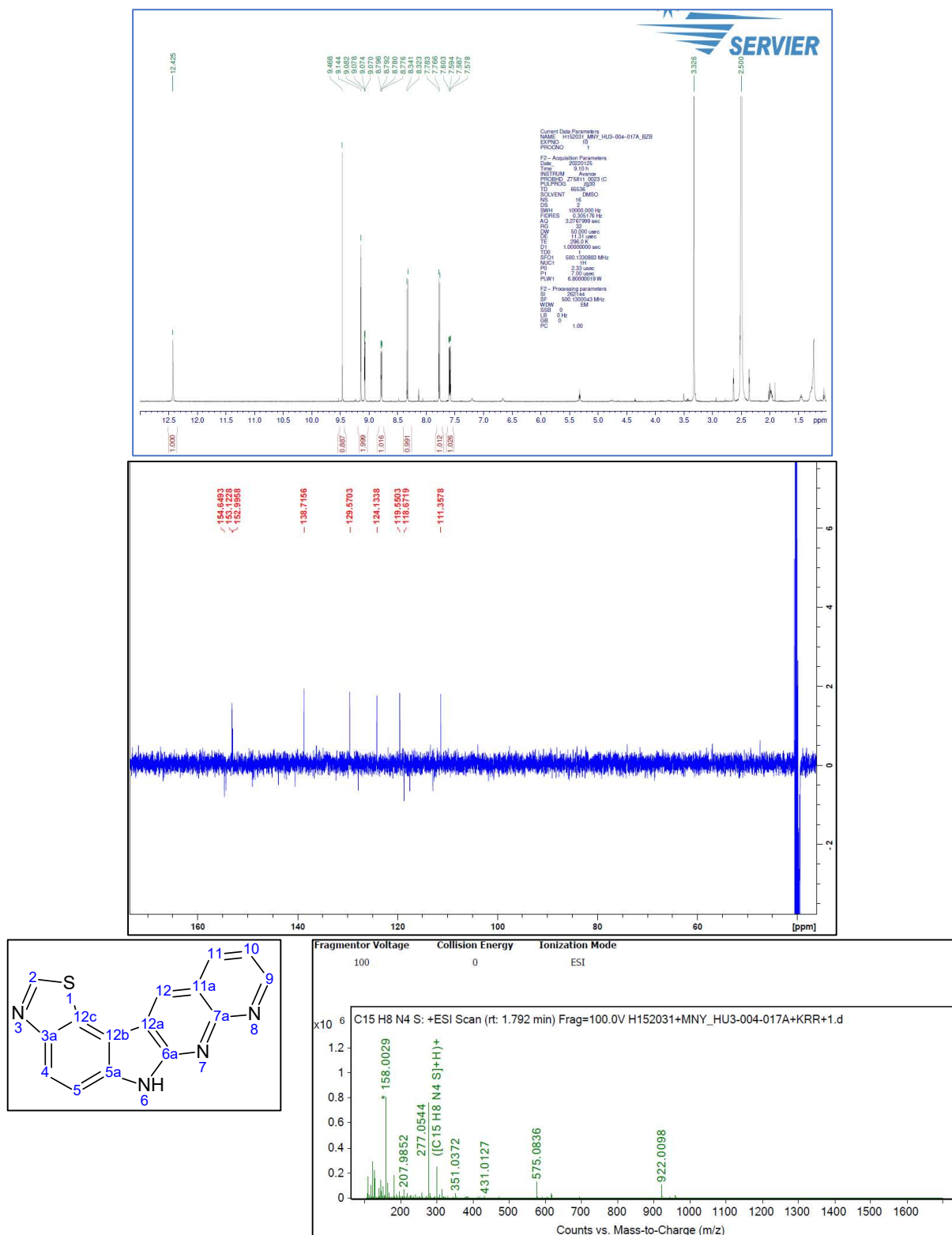
Figure S52. 1 H-NMR and 13 C-NMR and HRMS spectrum of 13e 6 H -[1,3]Thiazolo[5',4':4,5]indolo[2,3- b ][1,8]naphthyridine
