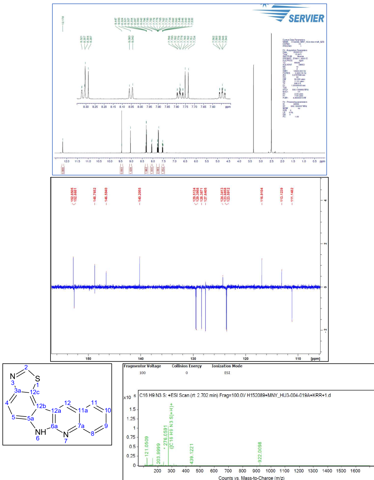
Figure S48. 1 H-NMR and 13 C-NMR and HRMS spectrum of 13a 6H-[1,3]Thiazolo[5',4':4,5]indolo[2,3-b]quinoline
