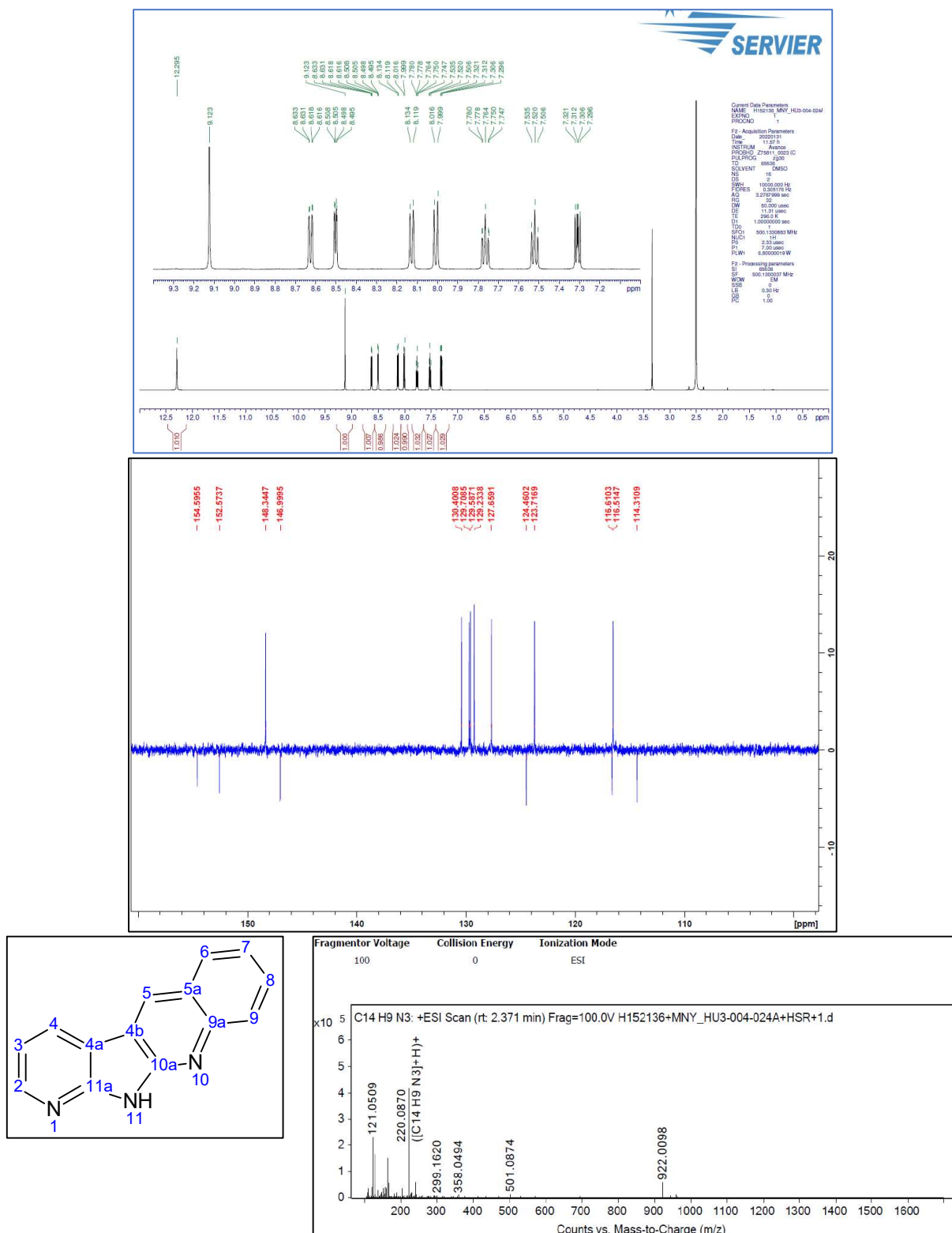
Figure S35. 1 H-NMR and 13 C-NMR and HRMS spectrum of 8d 11H-Pyrido[3',2':4,5]pyrrolo[2,3-b]quinoline
