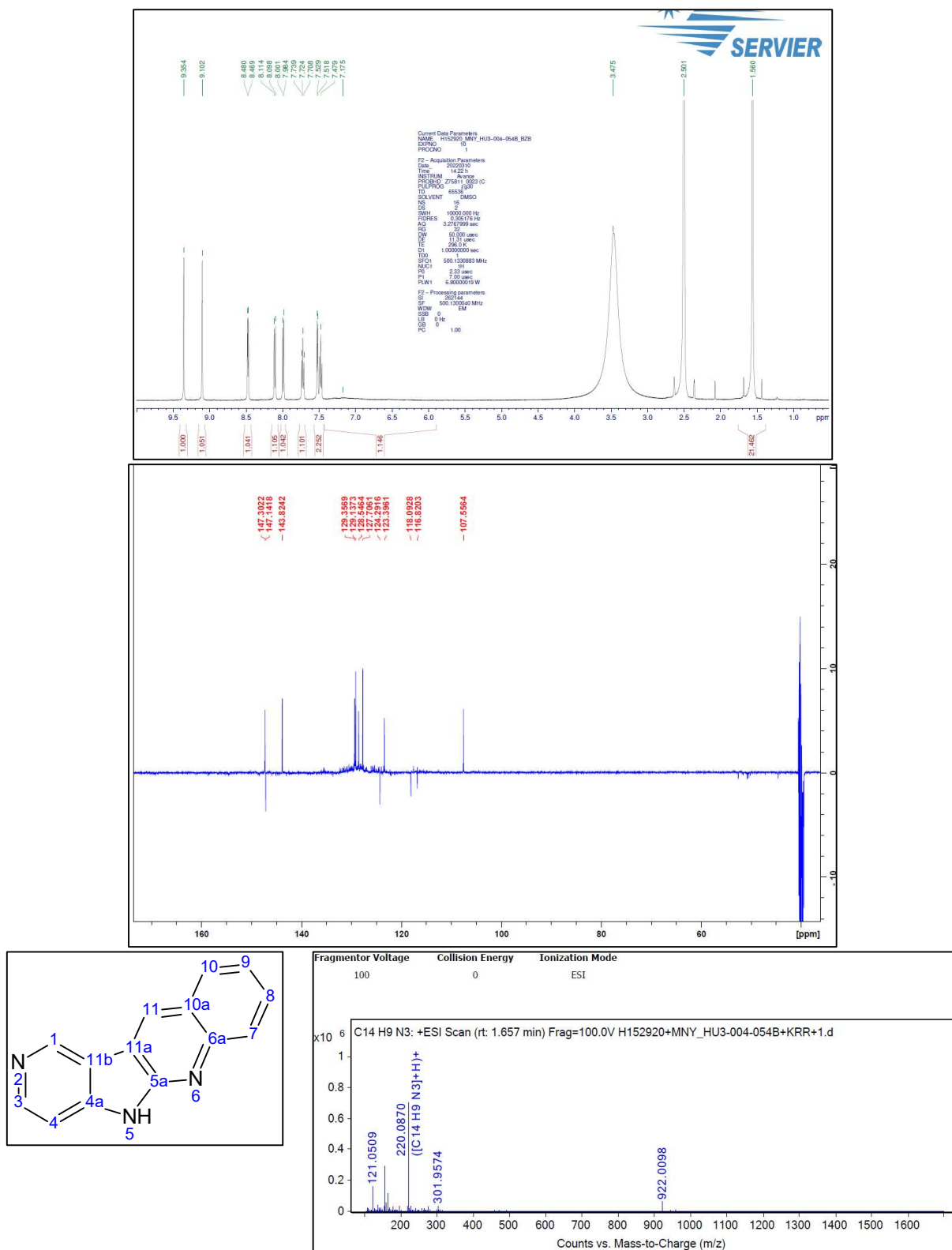
Figure S41. 1 H-NMR and 13 C-NMR and HRMS spectrum of 8k 5H-pyrido[3',4':4,5]pyrrolo[2,3-b]quinoline
