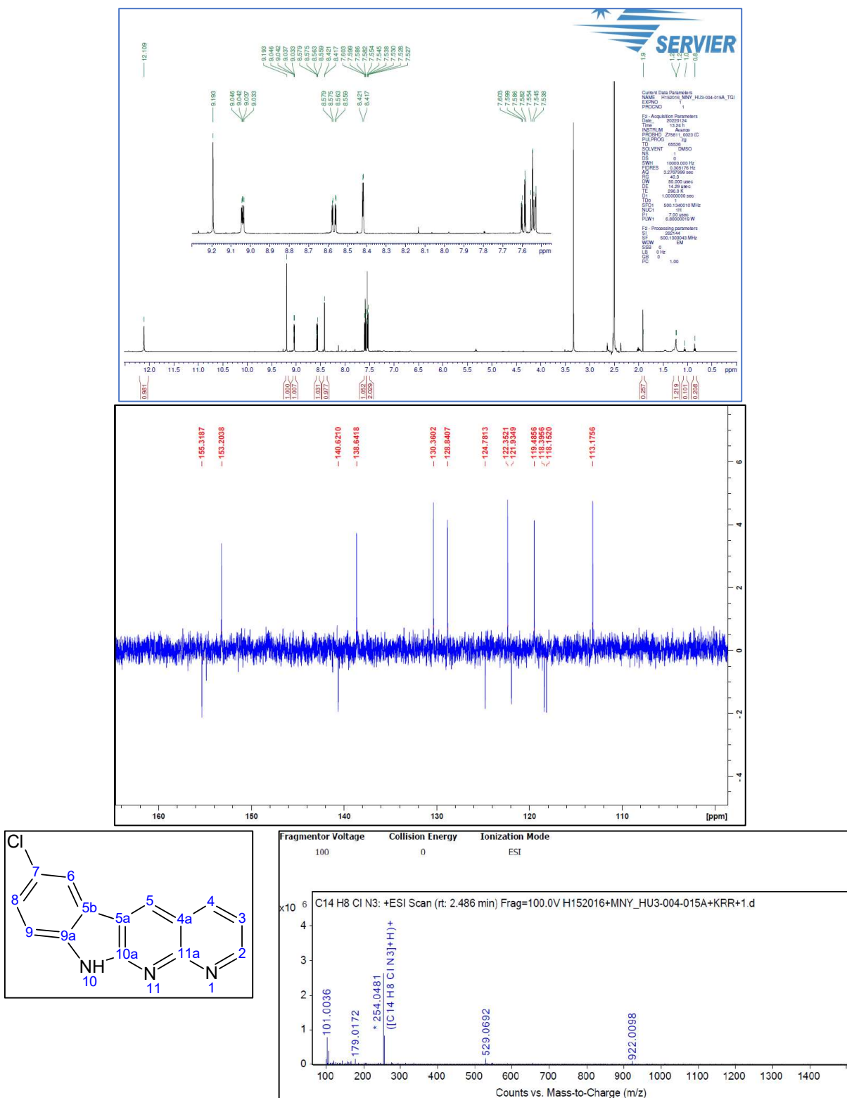
Figure S26. 1 H-NMR and 13 C-NMR and HRMS spectrum of 6d 7-Chloro-10H-indolo[2,3-b][1,8]naphthyridine
