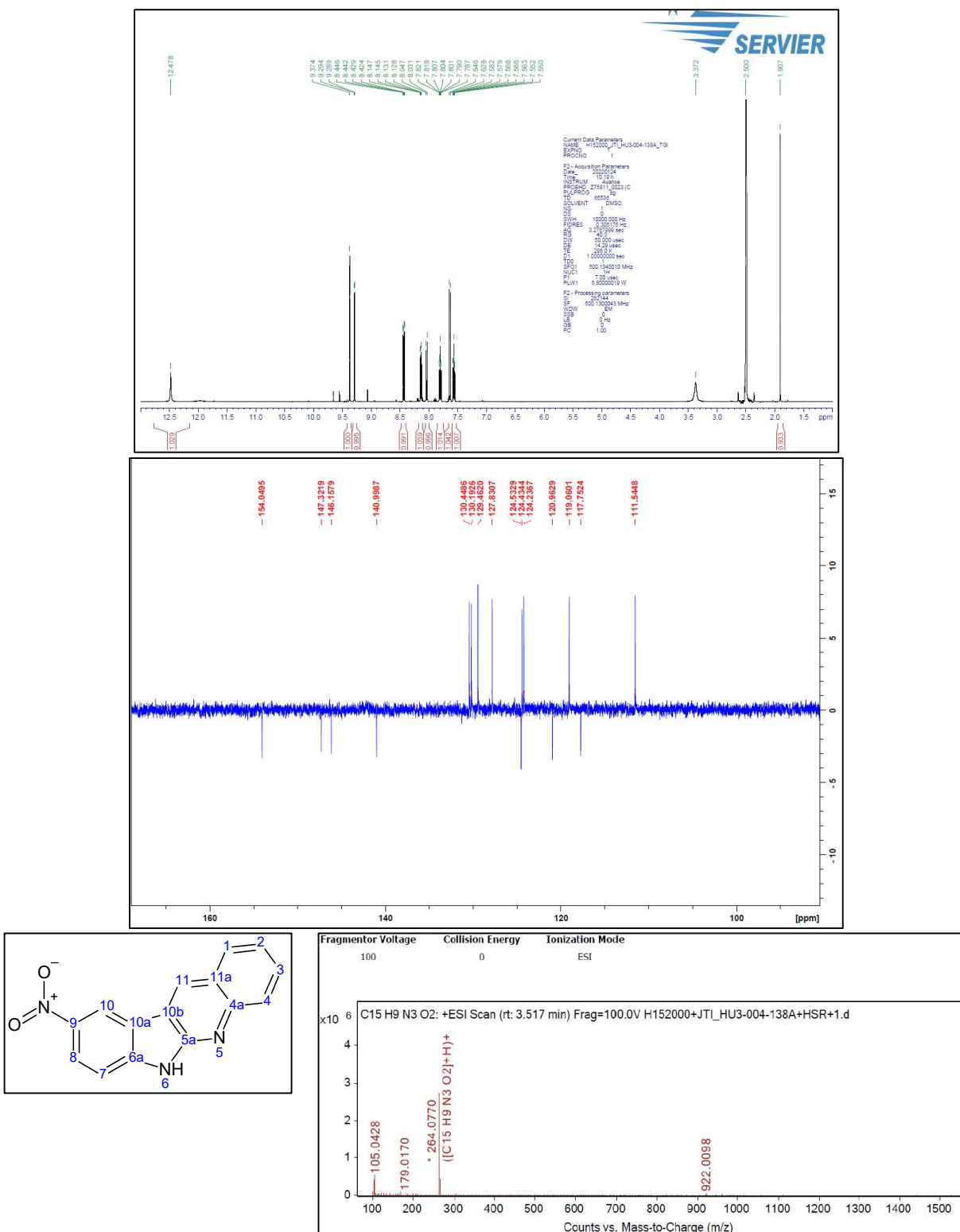
Figure S18. 1 H-NMR and 13 C-NMR and HRMS spectrum of 4o 9-Nitro-6H-indolo[2,3-b]quinoline
