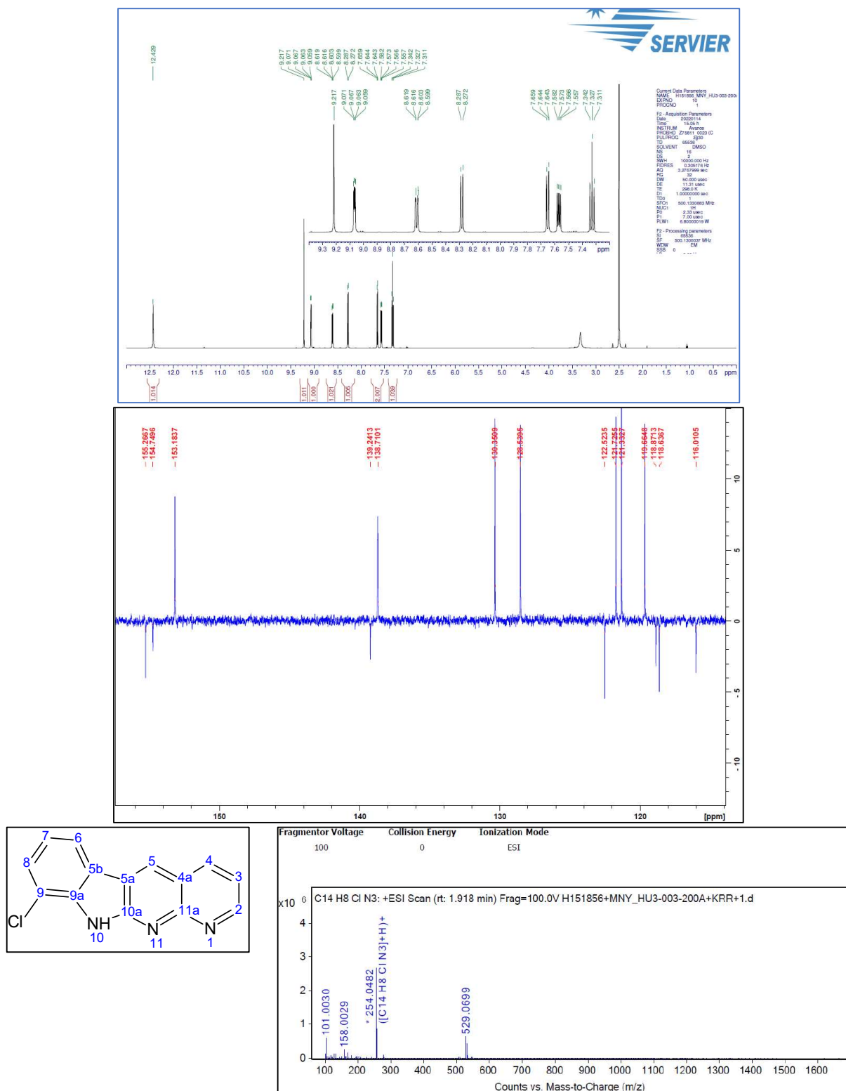
Figure S24. 1 H-NMR and 13 C-NMR and HRMS spectrum of 6b 9-Chloro-10H-indolo[2,3-b][1,8]naphthyridine
