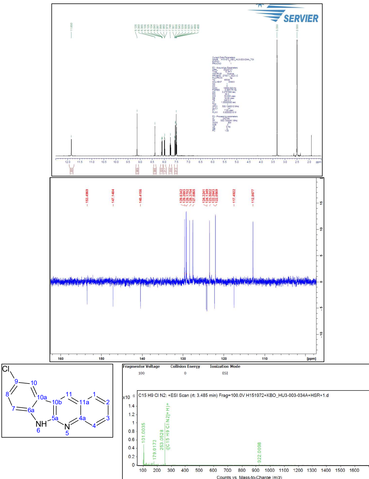
Figure S10. 1 H-NMR and 13 C-NMR and HRMS spectrum of 4g 9-Chloro-6H-indolo[2,3-b]quinoline
