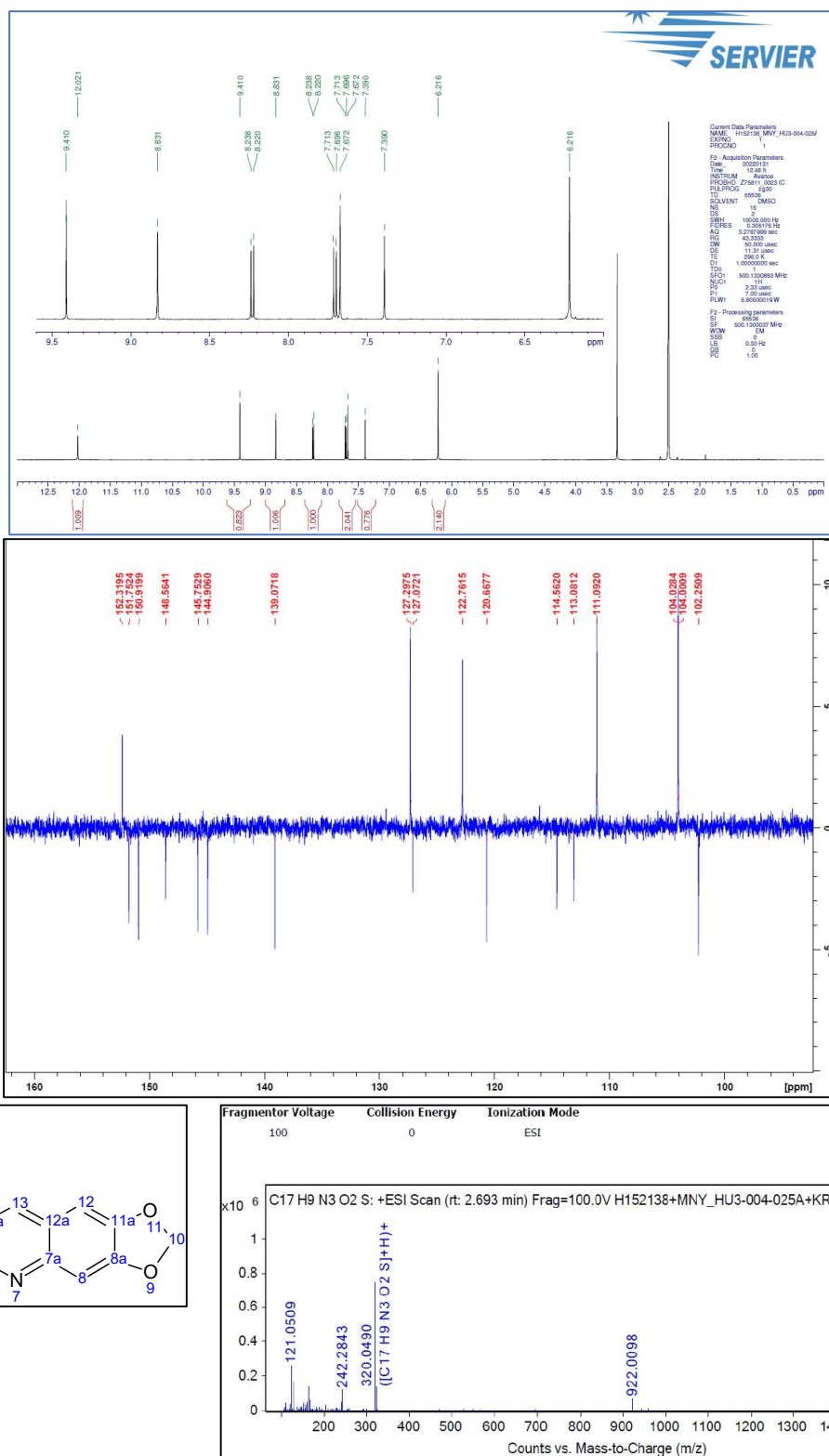
Figure S50. 1 H-NMR and 13 C-NMR and HRMS spectrum of 13c 6H,10H-[1,3]Dioxolo[4,5-g][1,3]thiazolo[5',4':4,5]indolo[2,3-b]quinoline
