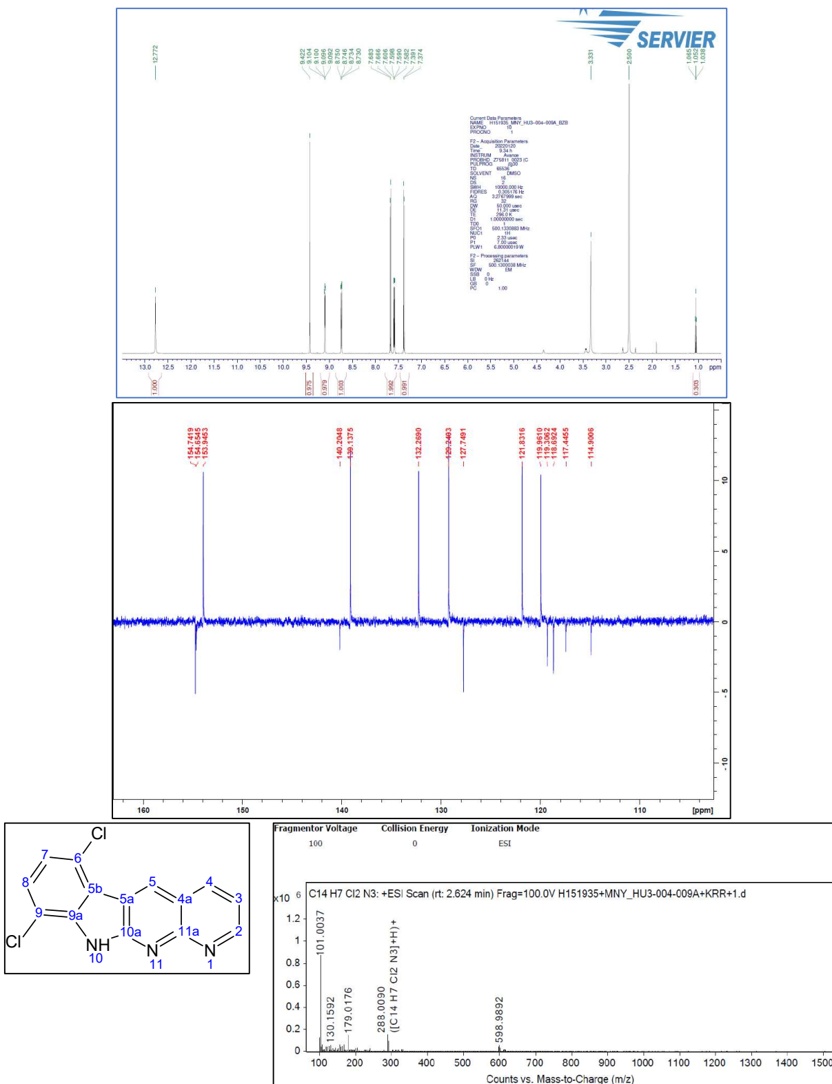
Figure S28. 1 H-NMR and 13 C-NMR and HRMS spectrum of 6f , 6,9-Dichloro-10H-indolo[2,3-b][1,8]naphthyridine
