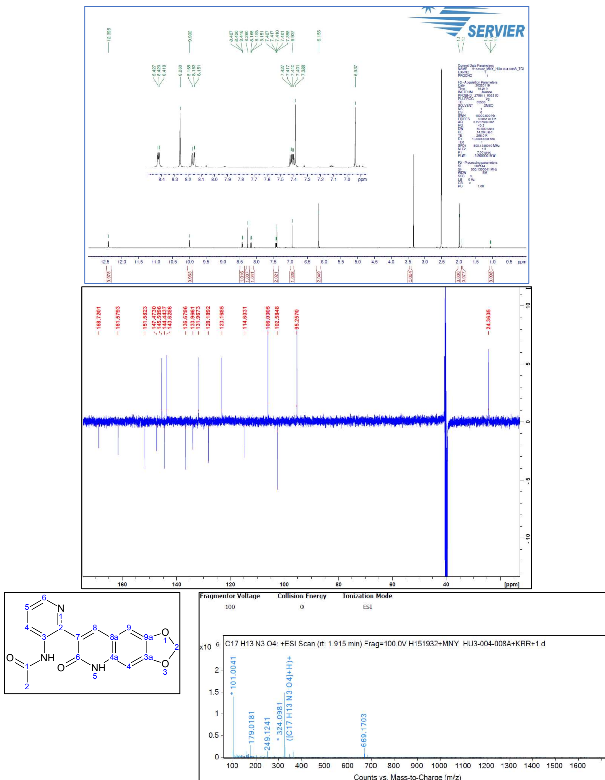
Figure S45. 1 H-NMR and 13 C-NMR and HRMS spectrum of 11c N -[2-(6-Oxo-5,6-dihydro-2 H -[1,3]dioxolo[4,5- g ]quinolin-7-yl)pyridin-3-yl]acetamide
