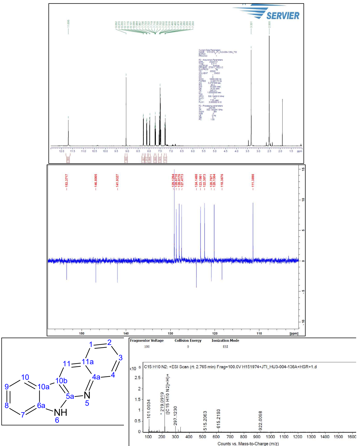
Figure S4. 1 H-NMR and 13 C-NMR and HRMS spectrum of 4a 6H-Indolo[2,3- b ]quinoline
