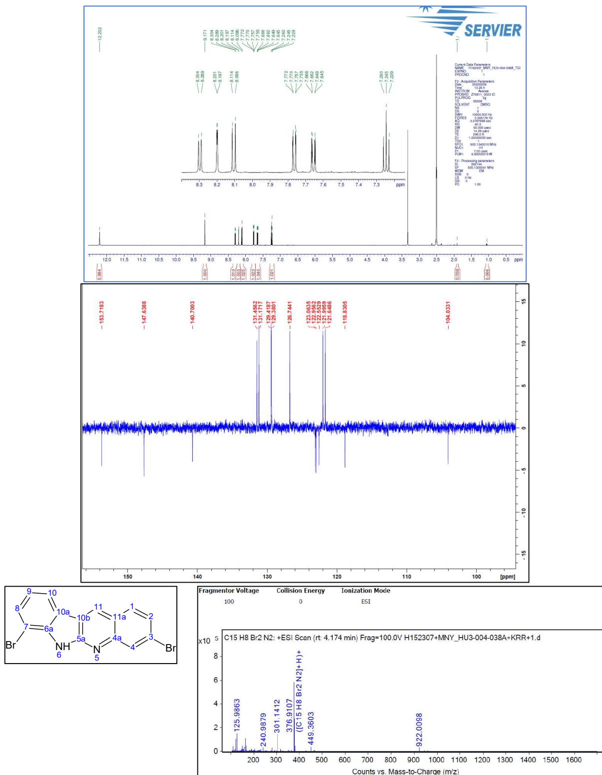
Figure S22. 1 H-NMR and 13 C-NMR and HRMS spectrum of 4s 3,7-Dibromo-6H-indolo[2,3-b]quinoline
