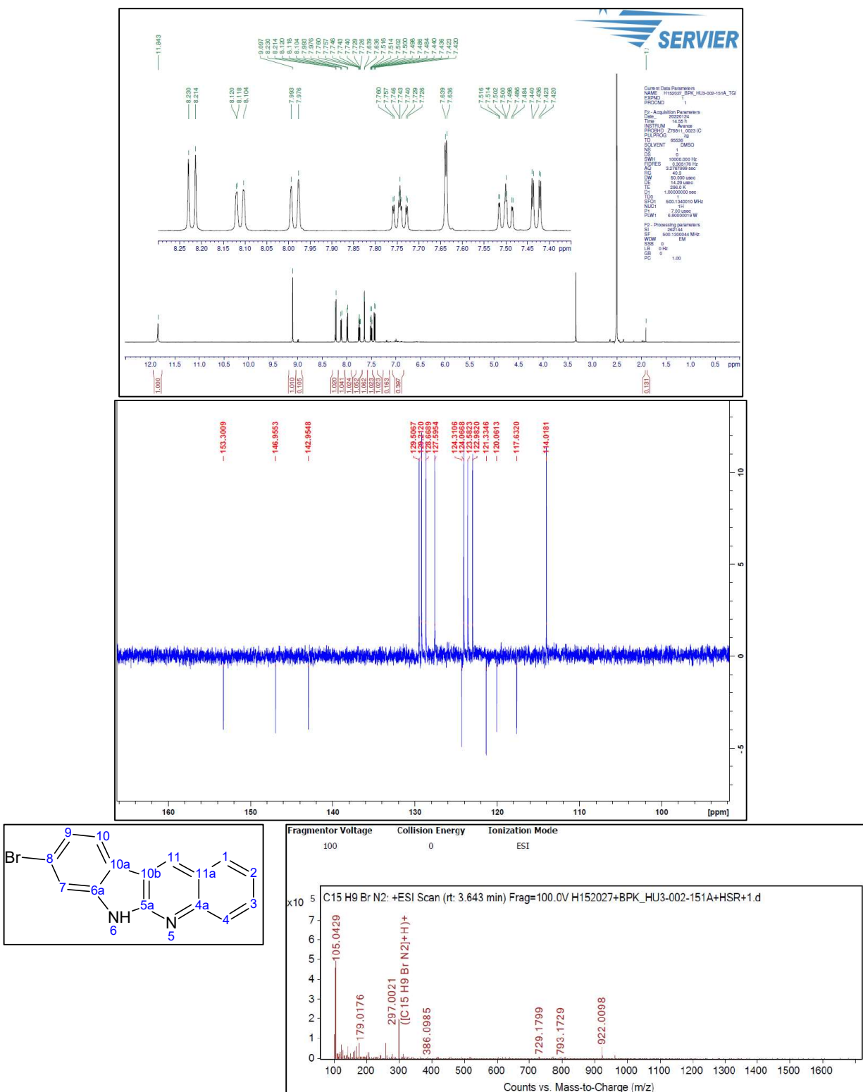
Figure S8. 1 H-NMR and 13 C-NMR and HRMS spectrum of 4e 8-bromo-6H-indolo[2,3-b]quinoline
