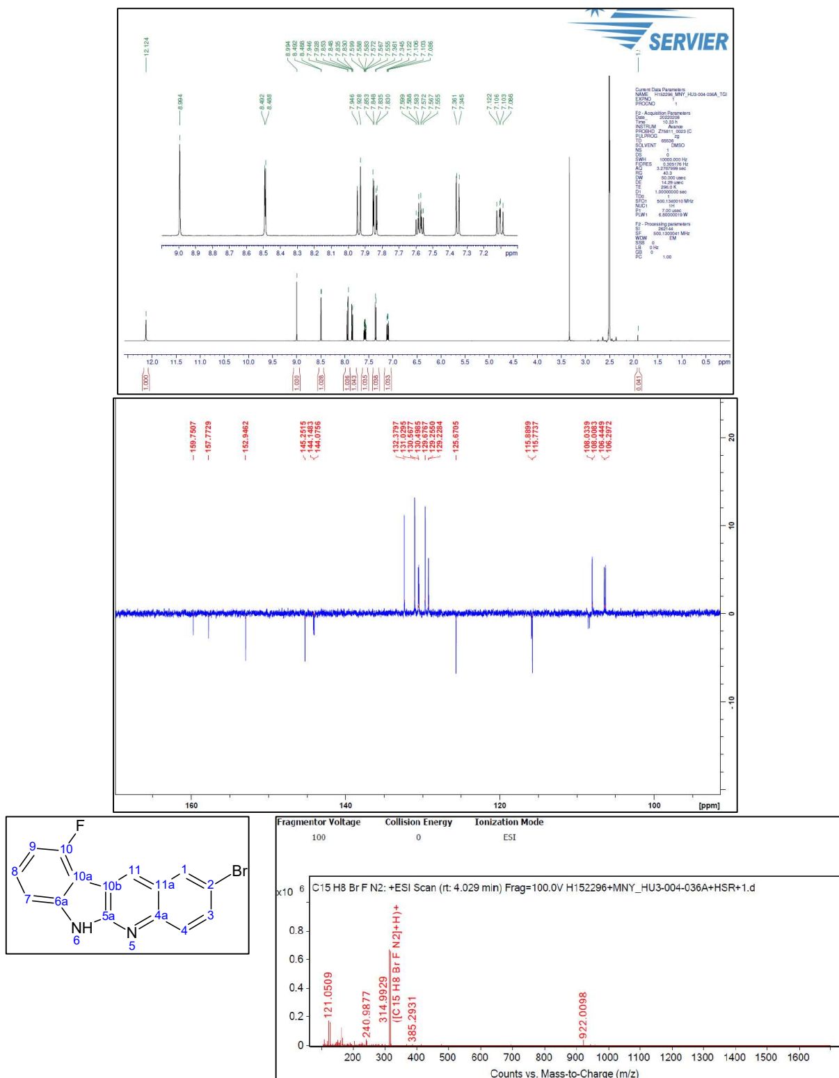
Figure S20. 1 H-NMR and 13 C-NMR and HRMS spectrum of 4q 2-Bromo-10-fluoro-6H-indolo[2,3-b]quinoline
