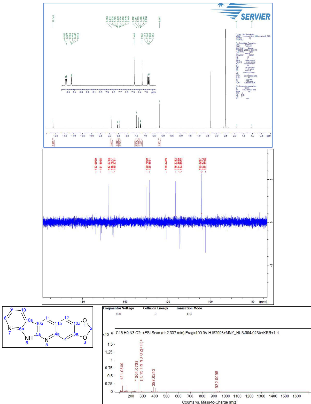
Figure S34. 1 H-NMR and 13 C-NMR and HRMS spectrum of 8c 2H,6H-[1,3]Dioxolo[4,5-g]pyrido[3',2':4,5]pyrrolo[2,3-b]quinoline
