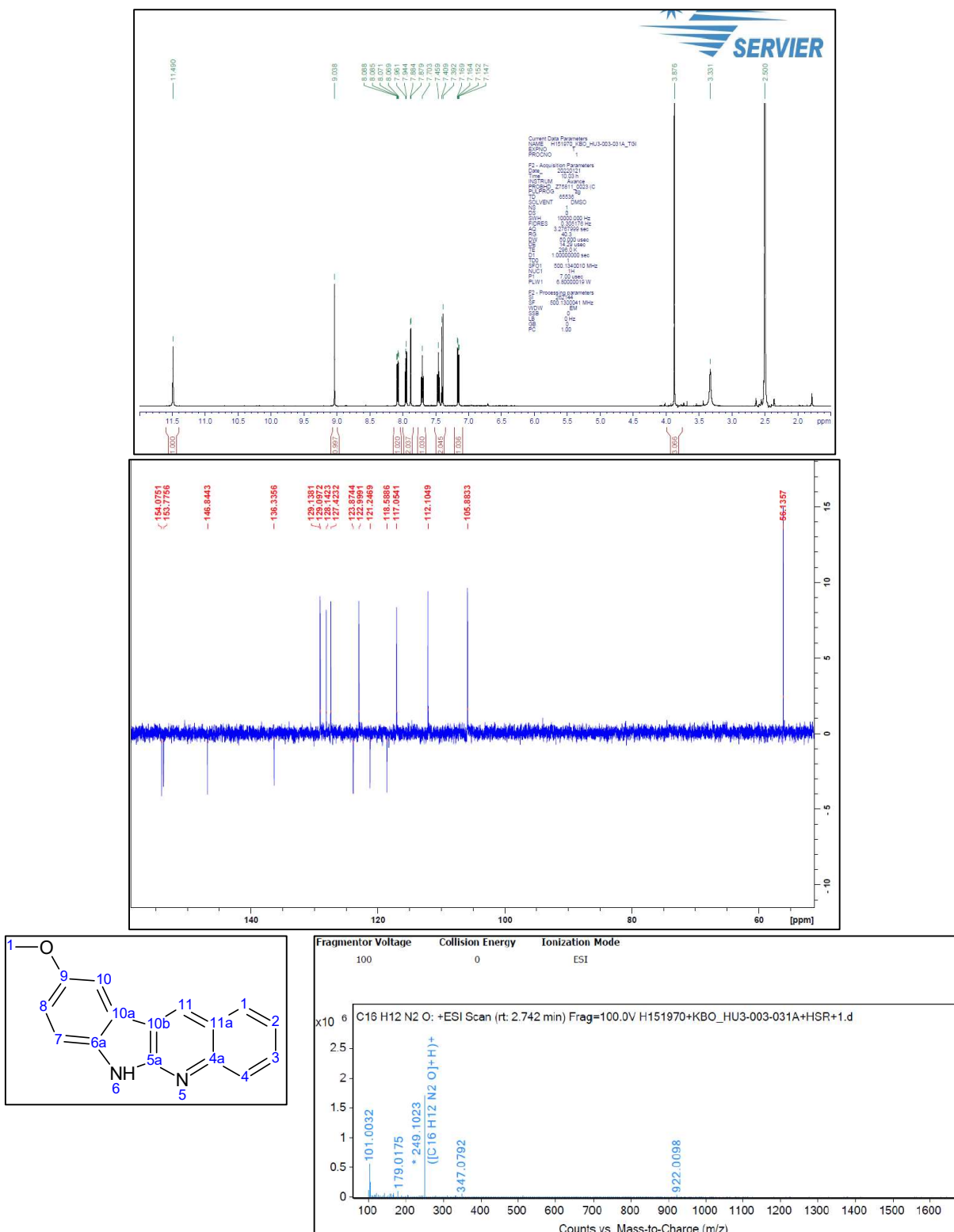
Figure S13. 1 H-NMR and 13 C-NMR and HRMS spectrum of 4j 9-Methoxy-6H-indolo[2,3-b]quinoline
