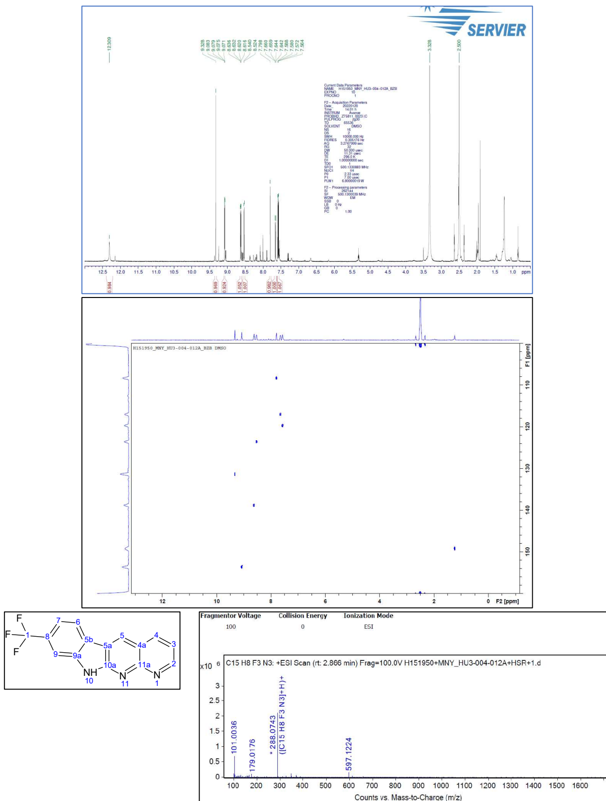
Figure S25. 1 H-NMR and HSQC and HRMS spectrum of 6c 8-(Trifluoromethyl)-10 H -indolo[2,3- b ][1,8]naphthyridine
