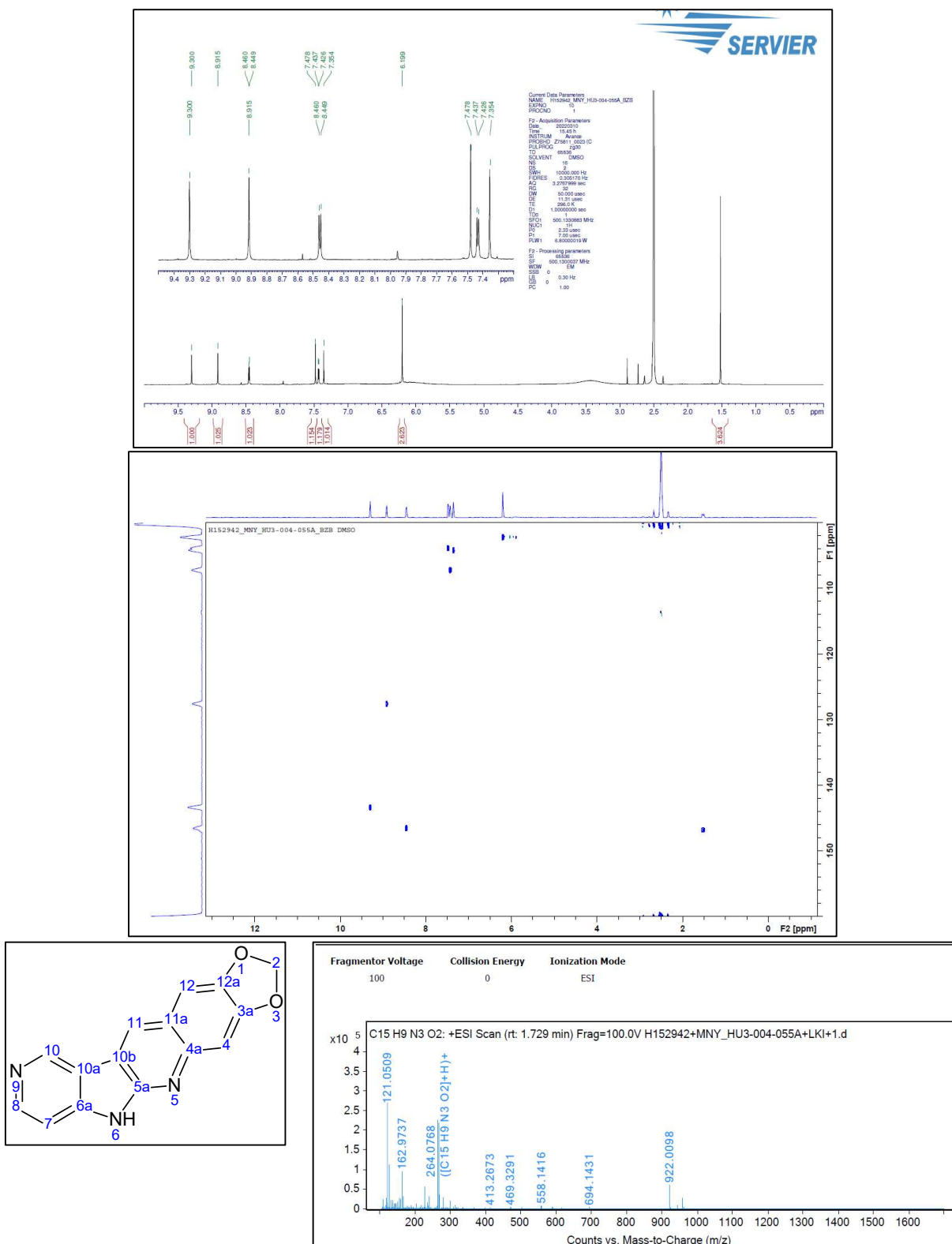
Figure S42. 1 H-NMR and HSQC and HRMS spectrum of 81 2 H ,6 H -[1,3]dioxolo[4,5- g ]pyrido[3',4':4,5]pyrrolo[2,3- b ]quinoline
