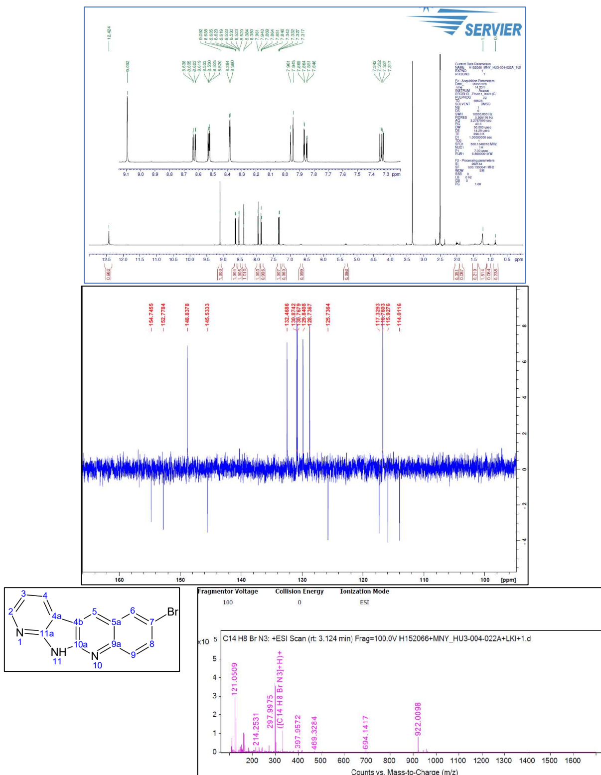
Figure S33. 1 H-NMR and 13 C-NMR and HRMS spectrum of 8b 7-Bromo-1H-pyrido[3',2':4,5]pyrrolo[2,3-b]quinoline
