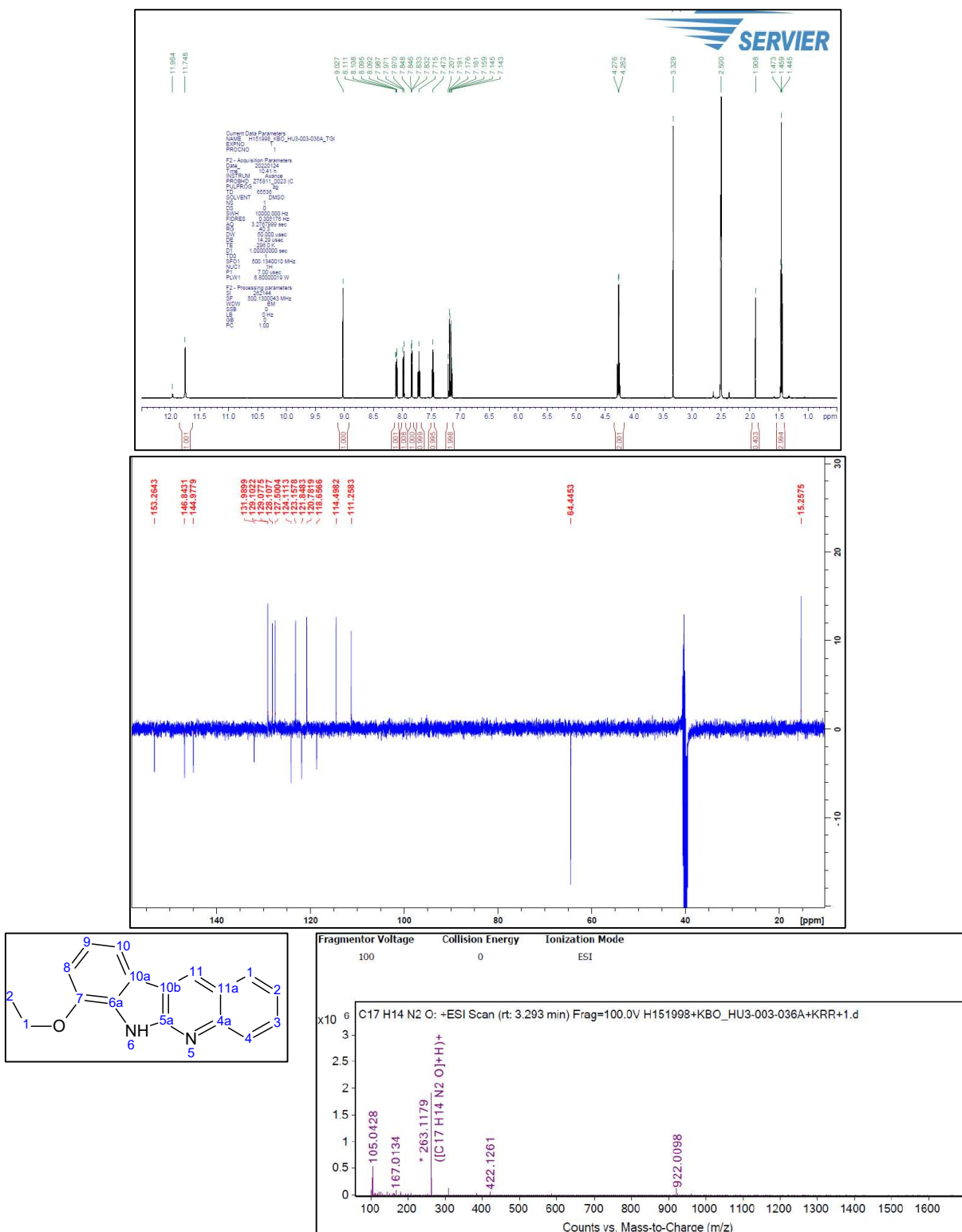
Figure S15. 1 H-NMR and 13 C-NMR and HRMS spectrum of 41 7-Ethoxy-6H-indolo[2,3-b]quinoline
