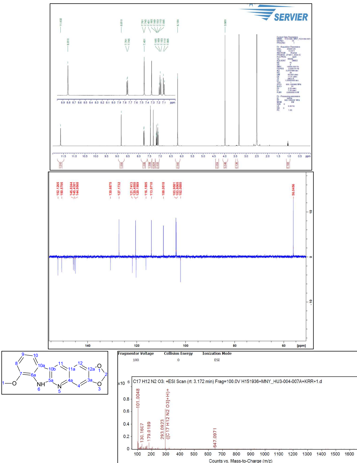
Figure S12. 1 H-NMR and 13 C-NMR and HRMS spectrum of 4i 7-Methoxy-2 H ,6 H -[1,3]dioxolo[4,5- g ]indolo[2,3- b ]quinoline
