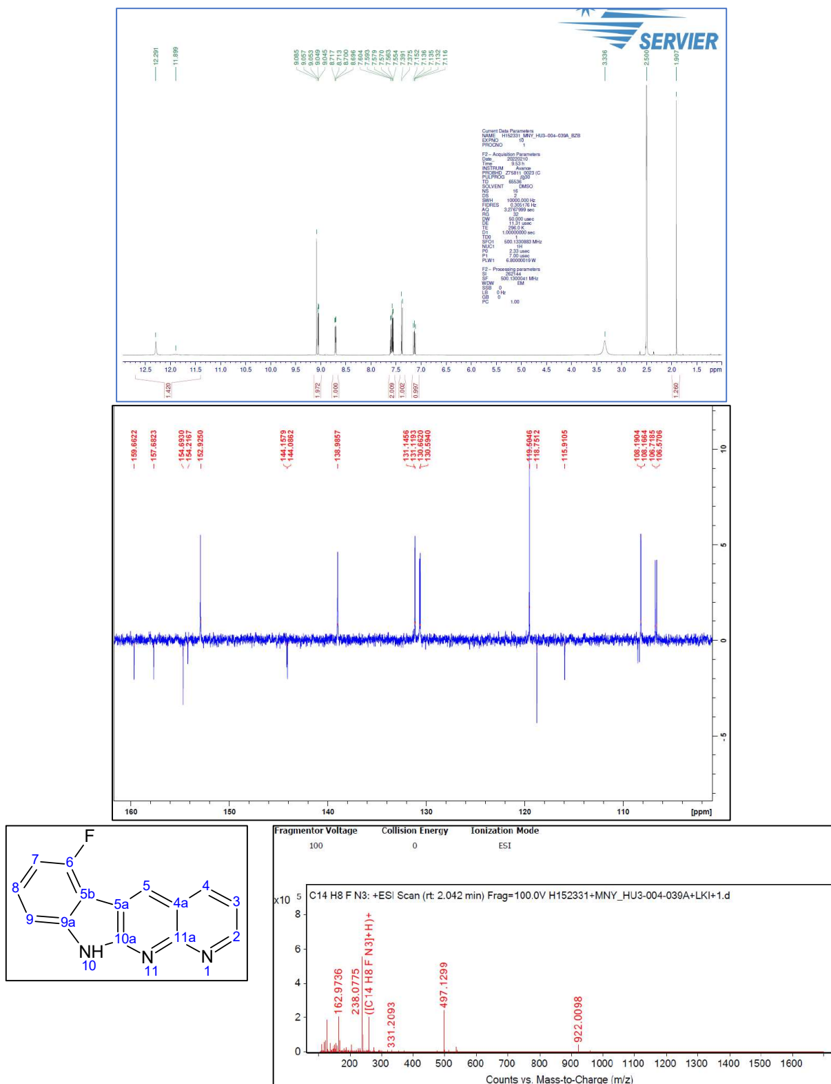
Figure S27. 1 H-NMR and 13 C-NMR and HRMS spectrum of 6e 6-Fluoro-10H-indolo[2,3-b][1,8]naphthyridine
