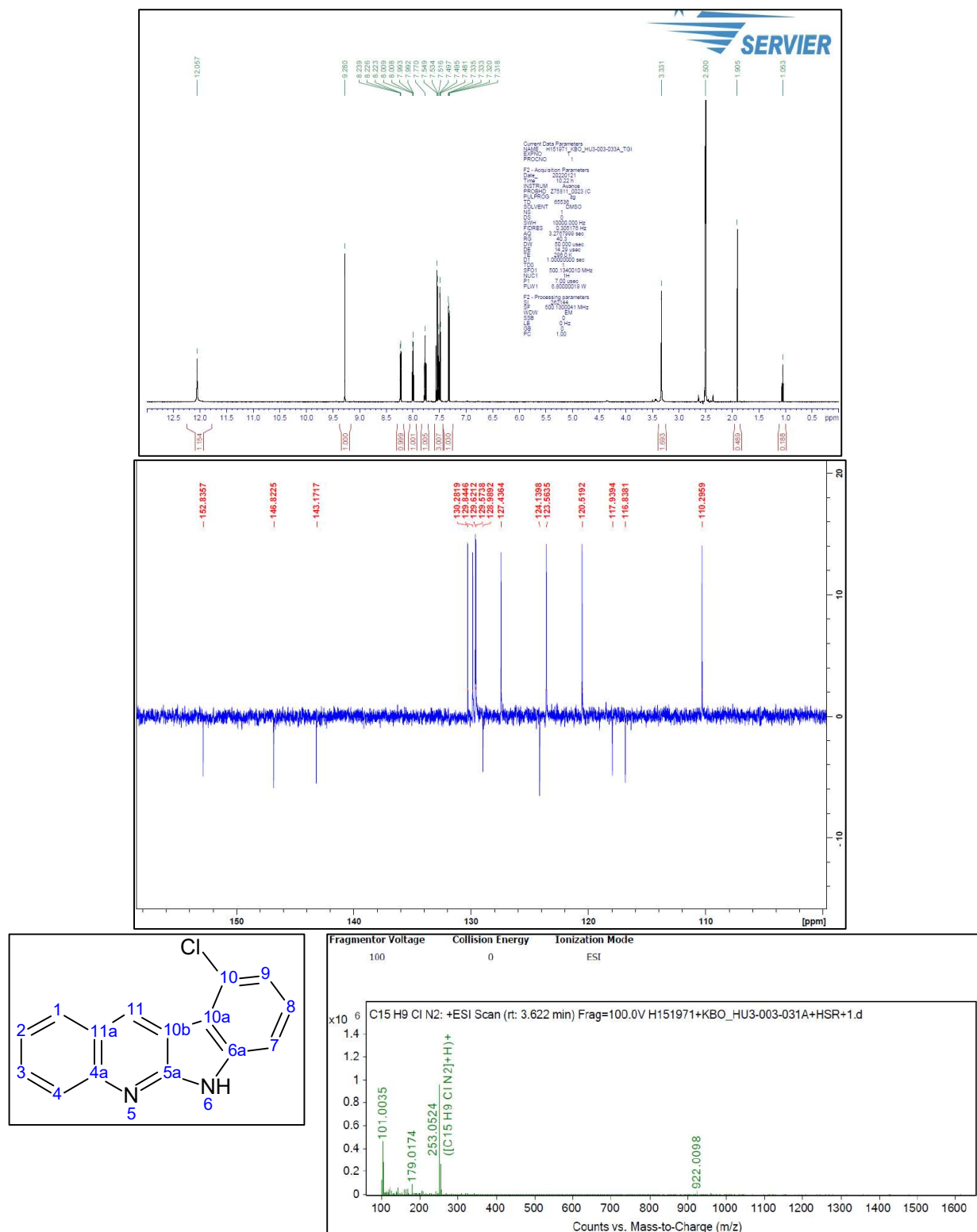
Figure S14. 1 H-NMR and 13 C-NMR and HRMS spectrum of 4k 10-Chloro-6 H -indolo[2,3- b ]quinoline
