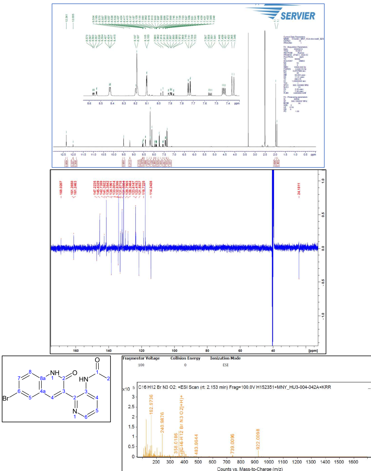
Figure S46. 1 H-NMR and 13 C-NMR and HRMS spectrum of 11d N -[2-(6-Bromo-2-oxo-1,2-dihydroquinolin-3-yl)pyridin-3-yl]acetamide
