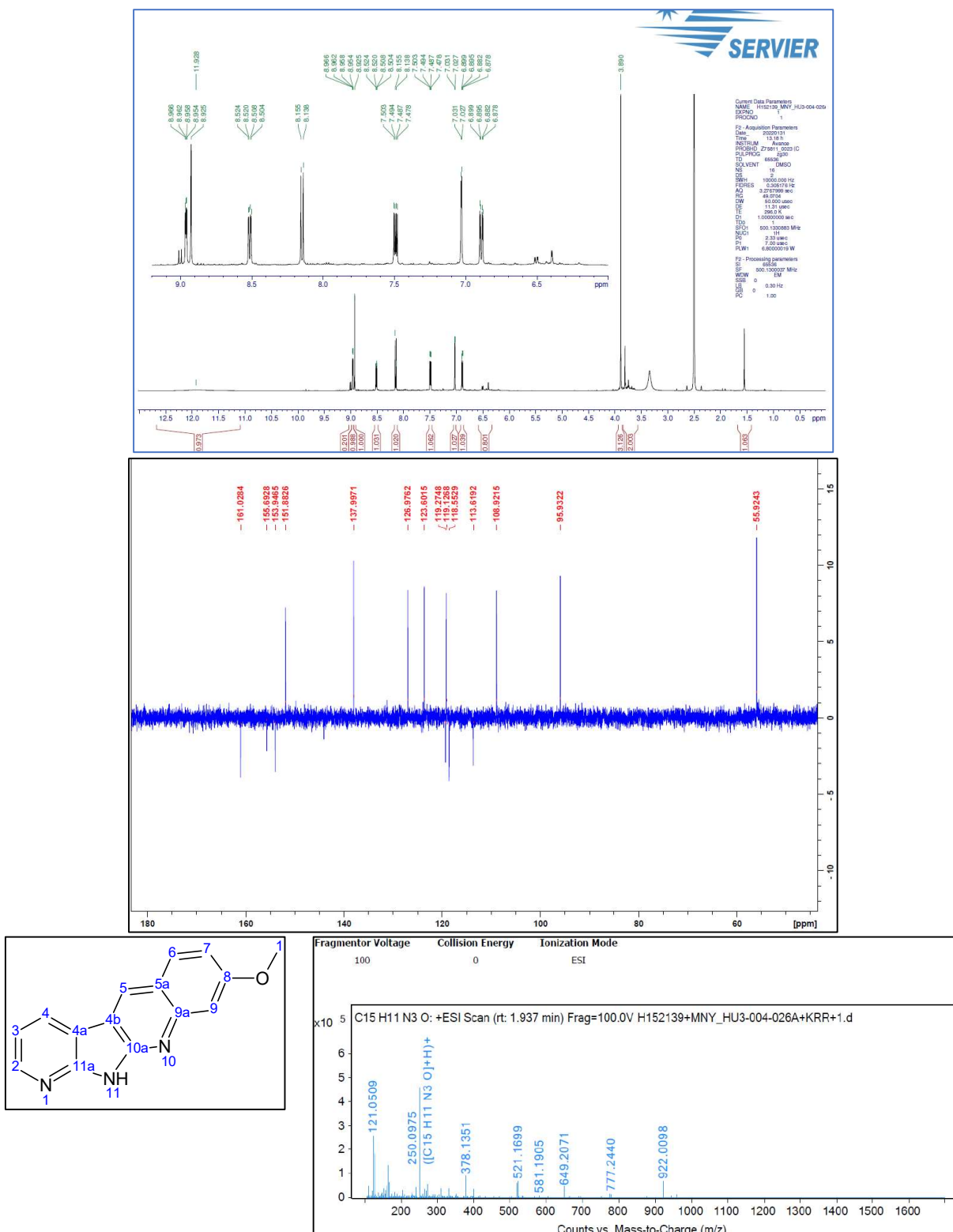
Figure S36. 1 H-NMR and 13 C-NMR and HRMS spectrum of 8f 8-Methoxy-1H-pyrido[3',2':4,5]pyrrolo[2,3-b]quinoline
