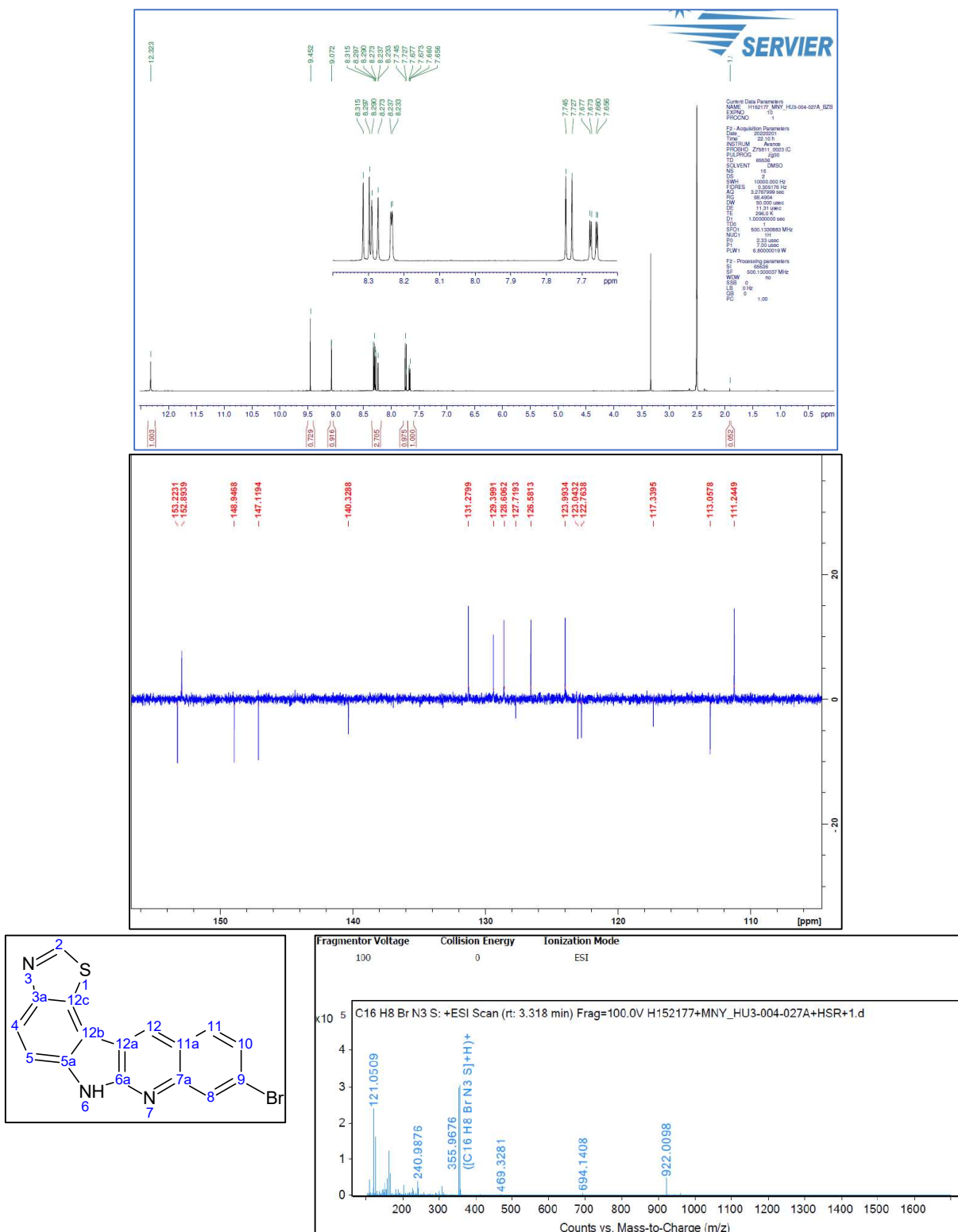
Figure S49. 1 H-NMR and 13 C-NMR and HRMS spectrum of 13b 9-Bromo-6H-[1,3]thiazolo[5',4':4,5]indolo[2,3-b]quinoline
