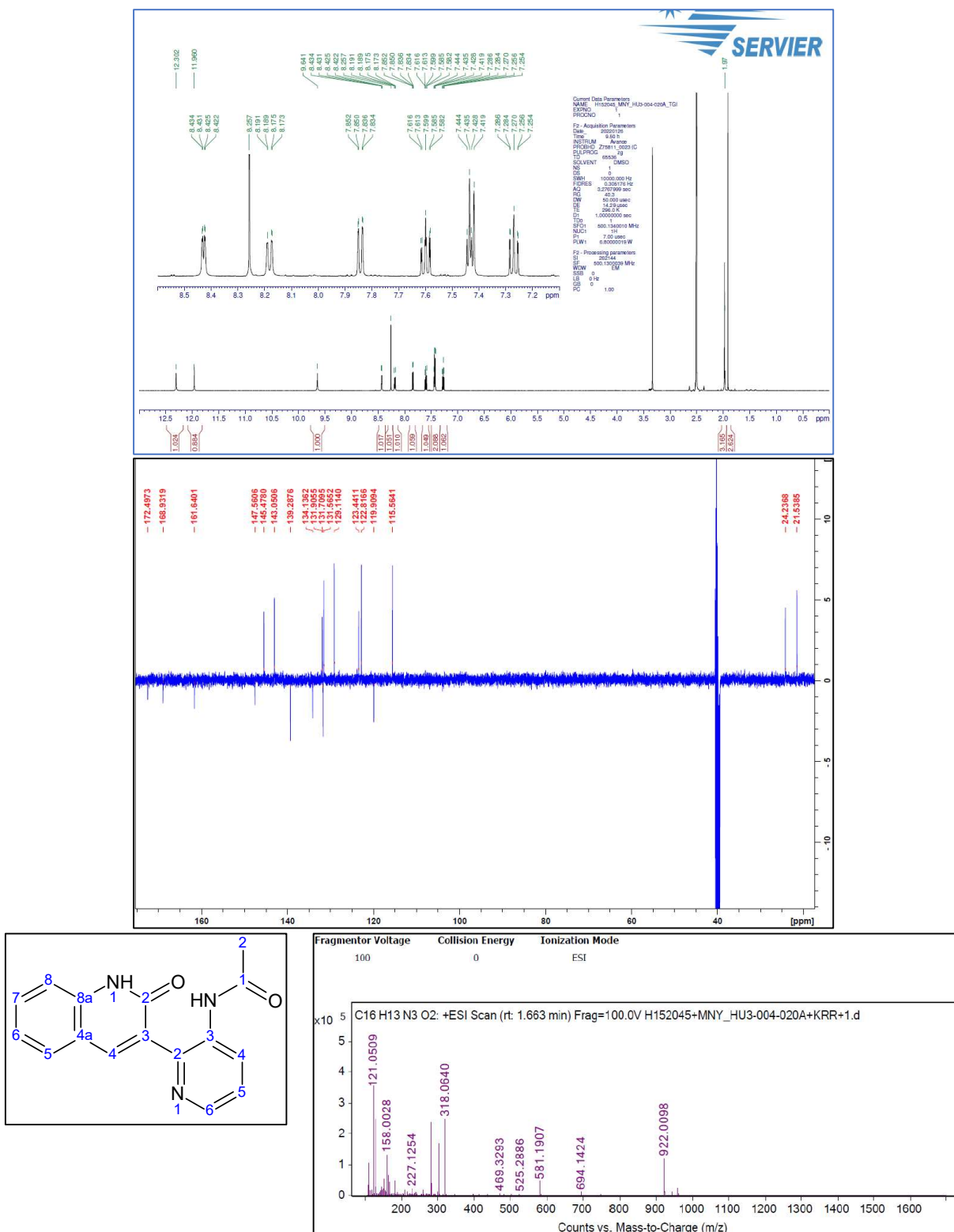
Figure S43. 1 H-NMR and 13 C-NMR and HRMS spectrum of 11a N -[2-(2-Oxo-1,2-dihydroquinolin-3-yl)pyridin-3-yl]acetamide
