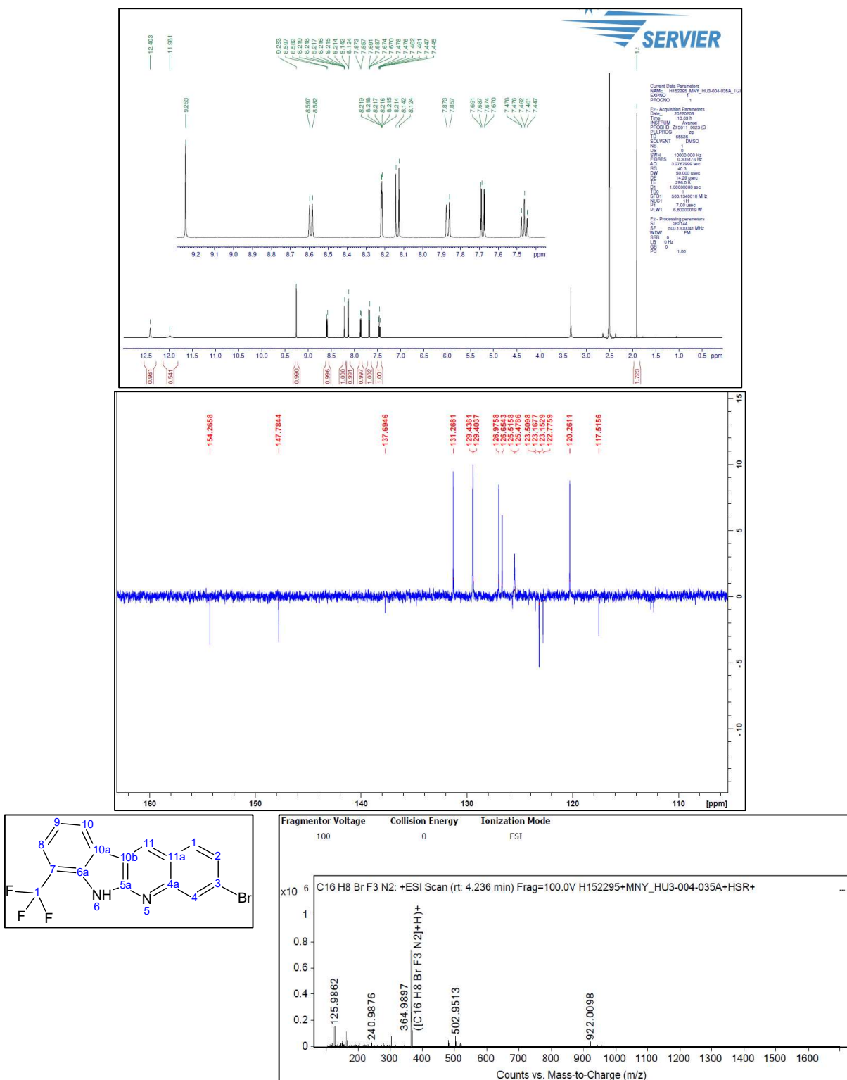
Figure S19. 1 H-NMR and 13 C-NMR and HRMS spectrum of 4p 3-Bromo-7-(trifluoromethyl)-6H-indolo[2,3-b]quinoline
