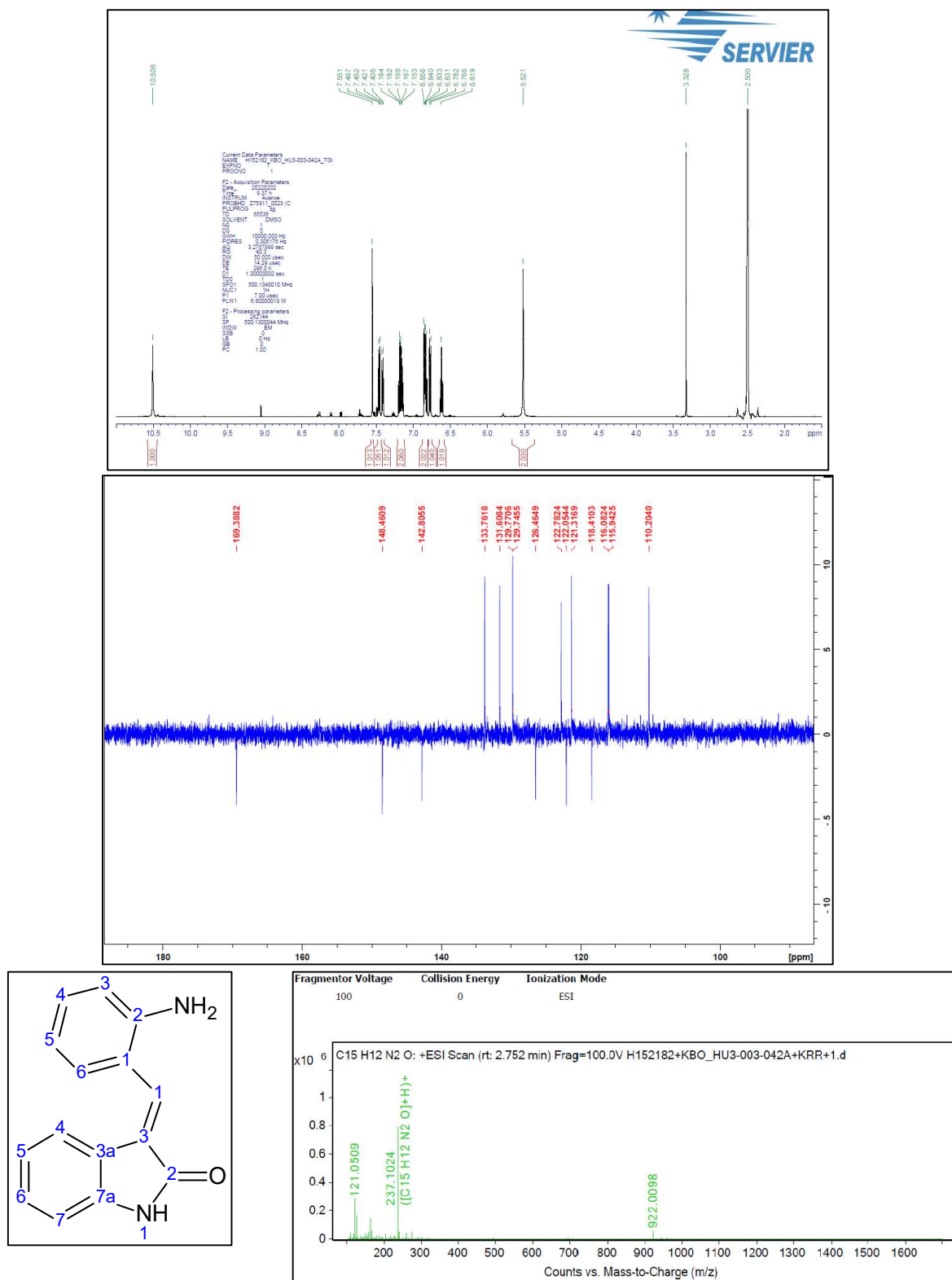
Figure S1. 1 H-NMR and 13 C-NMR and HRMS spectrum of 3a ( 3E )-3-[(2-aminophenyl)methylidene]-1,3-dihydro-2 H -indol-2-one
