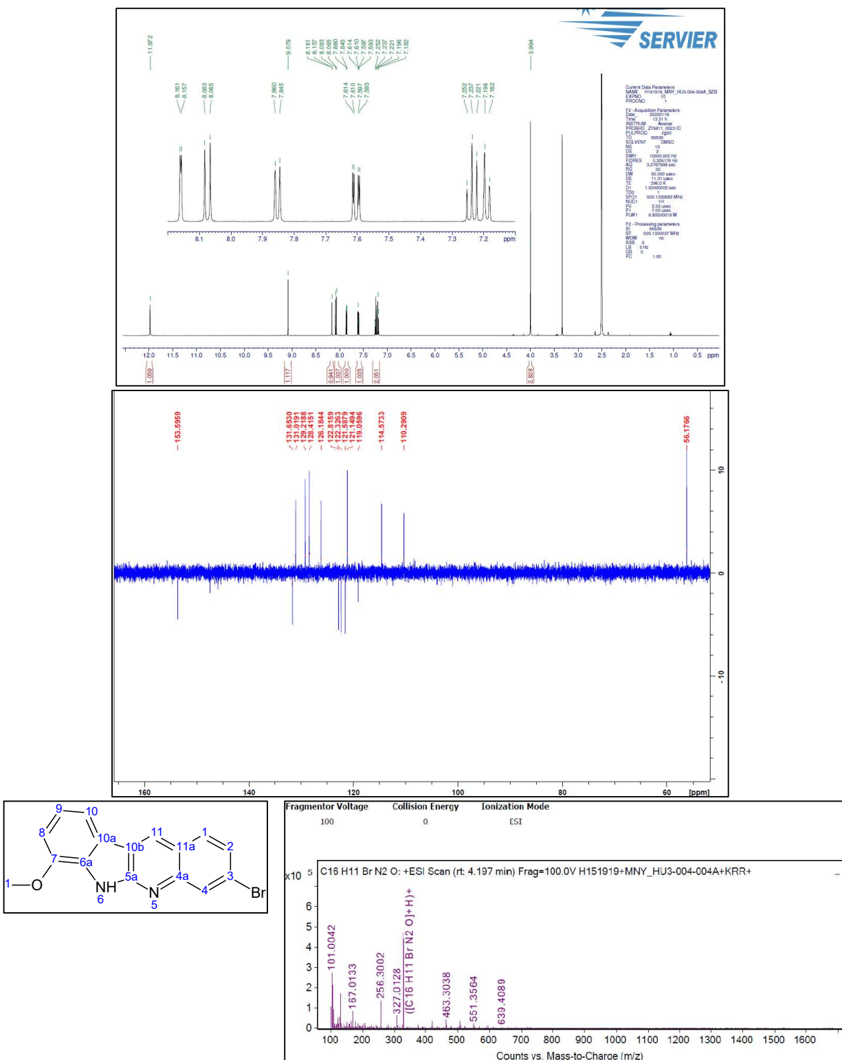
Figure S11. 1 H-NMR and 13 C-NMR and HRMS spectrum of 4h 3-Bromo-7-methoxy-6H-indolo[2,3-b]quinoline
