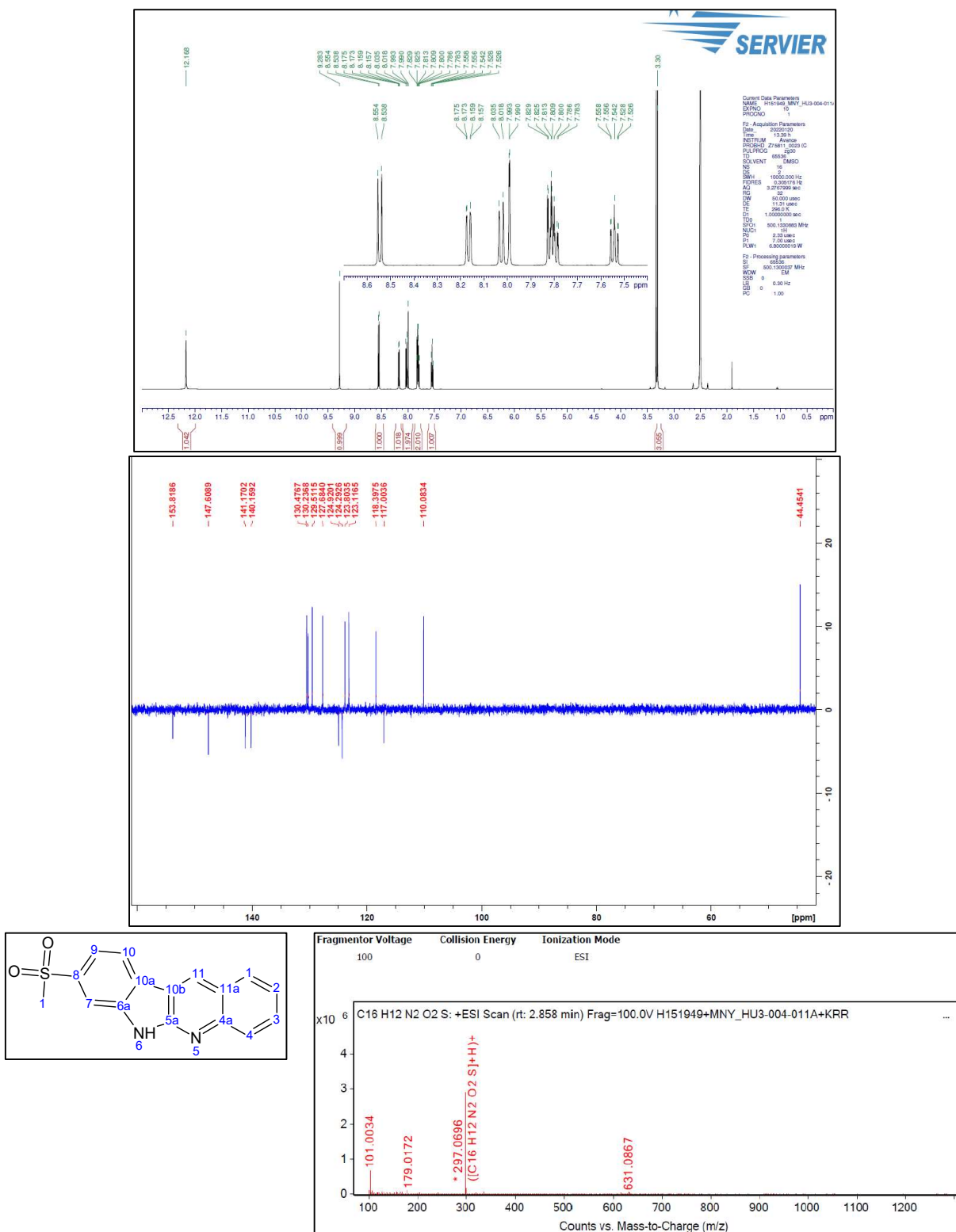
Figure S17. 1 H-NMR and 13 C-NMR and HRMS spectrum of 4n 8-(Methanesulfonyl)-6H-indolo[2,3-b]quinoline
