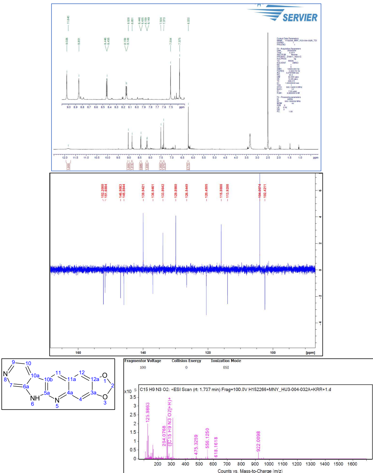
Figure S37. 1 H-NMR and 13 C-NMR and HRMS spectrum of 8g 2 H ,6 H -[1,3]Dioxolo[4,5- g ]pyrido[4',3':4,5]pyrrolo[2,3- b ]quinoline
