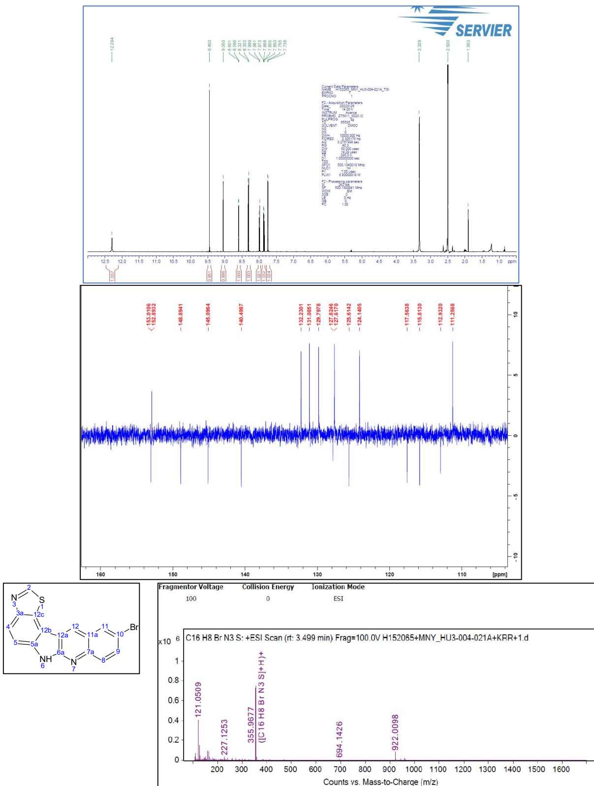
Figure S51. 1 H-NMR and 13 C-NMR and HRMS spectrum of 13d 10-Bromo-6 H -[1,3]thiazolo[5',4':4,5]indolo[2,3- b ]quinoline
