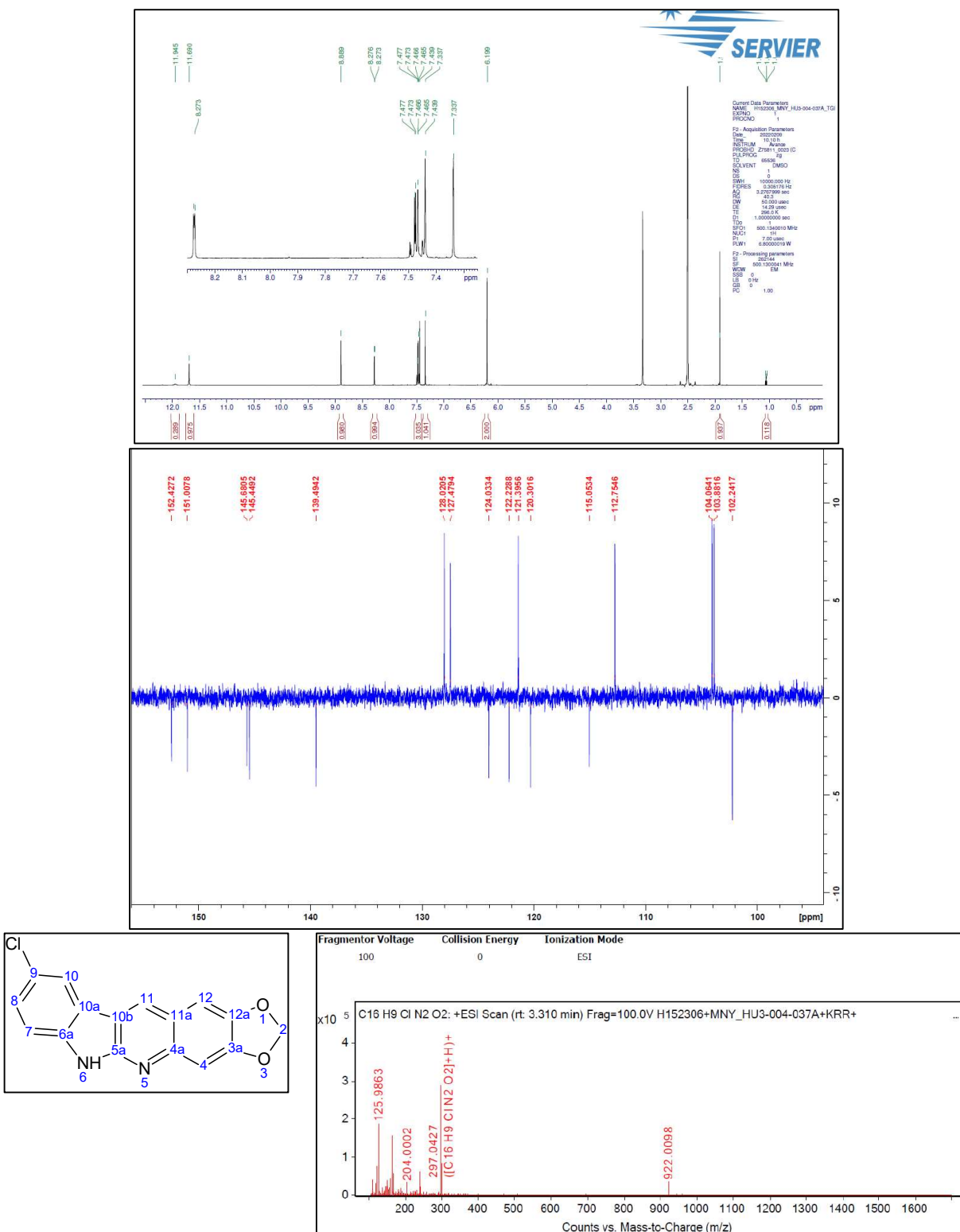
Figure S21. 1 H-NMR and 13 C-NMR and HRMS spectrum of 4r 9-Chloro-2H,6H-[1,3]dioxolo[4,5-g]indolo[2,3-b]quinoline
