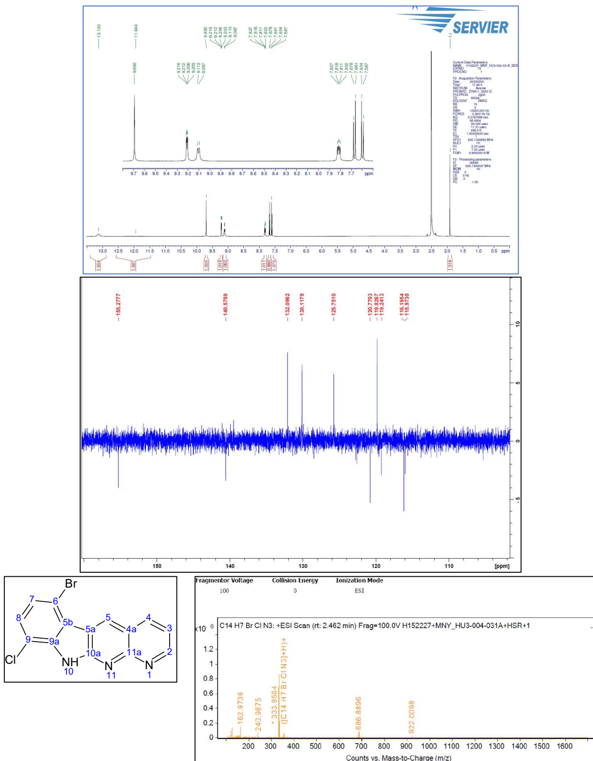
Figure S31. 1 H-NMR and 13 C-NMR and HRMS spectrum of 6i 6-Bromo-9-chloro-10 H -indolo[2,3- b ][1,8]naphthyridine
