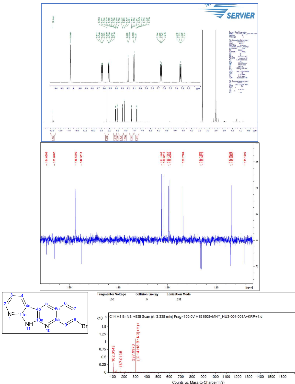
Figure S32. 1 H-NMR and 13 C-NMR and HRMS spectrum of 8a 8-Bromo-11H-pyrido[3',2':4,5]pyrrolo[2,3-b]quinoline
