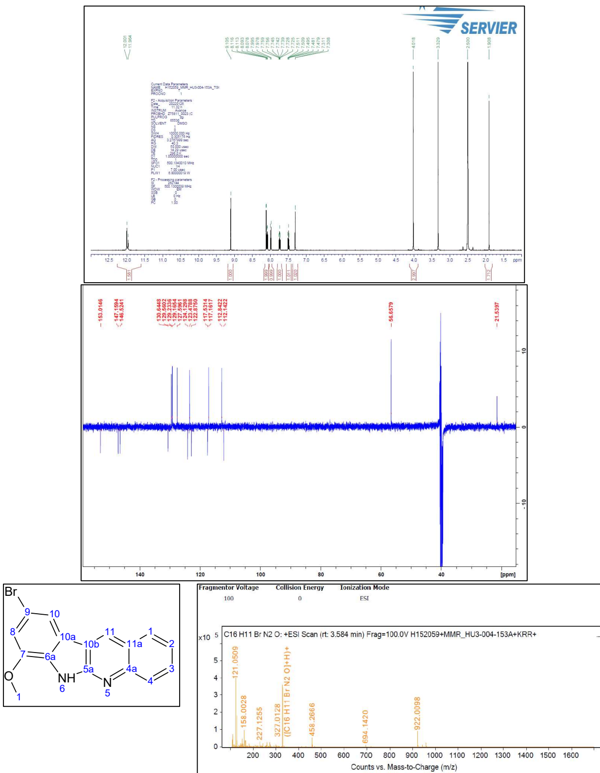
Figure S16. 1 H-NMR and 13 C-NMR and HRMS spectrum of 4m 9-Bromo-7-methoxy-6H-indolo[2,3-b]quinoline
