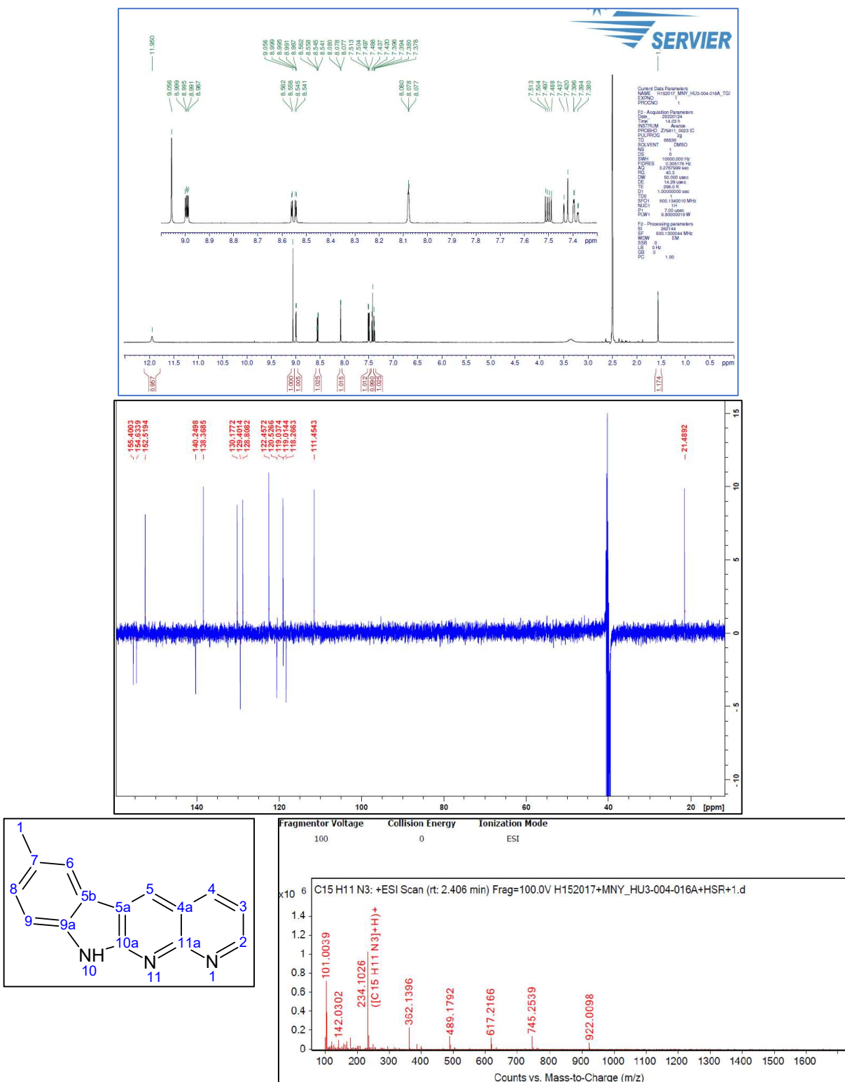
Figure S30. 1 H-NMR and 13 C-NMR and HRMS spectrum of 6h 7-Methyl-10H-indolo[2,3-b][1,8]naphthyridine
