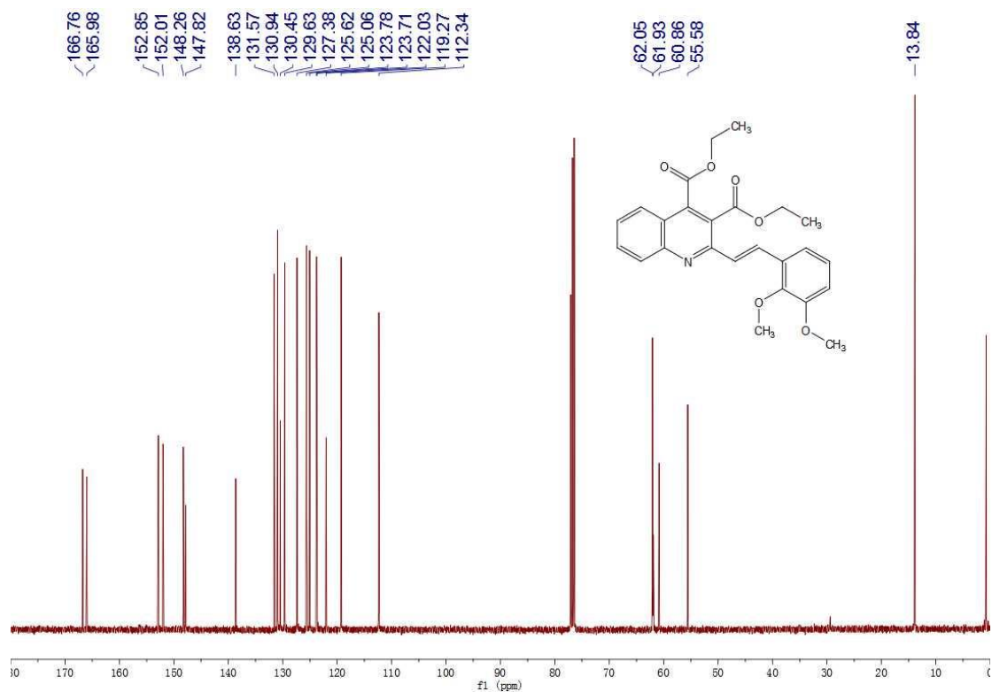
Fig. S16 ^{13}\text{C} NMR spectrum of 3h
