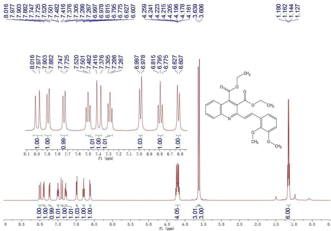
Fig. S15 ^1\text{H} NMR spectrum of 3h
