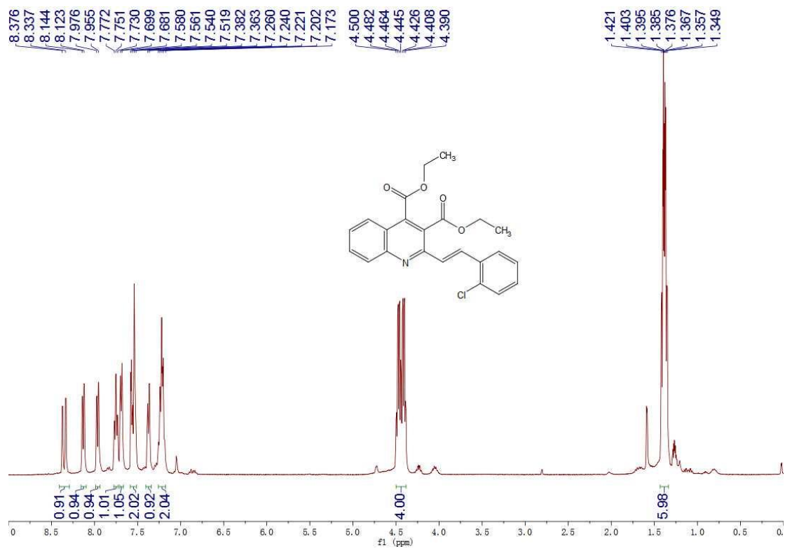
Fig. S23 1 H NMR spectrum of 3I
