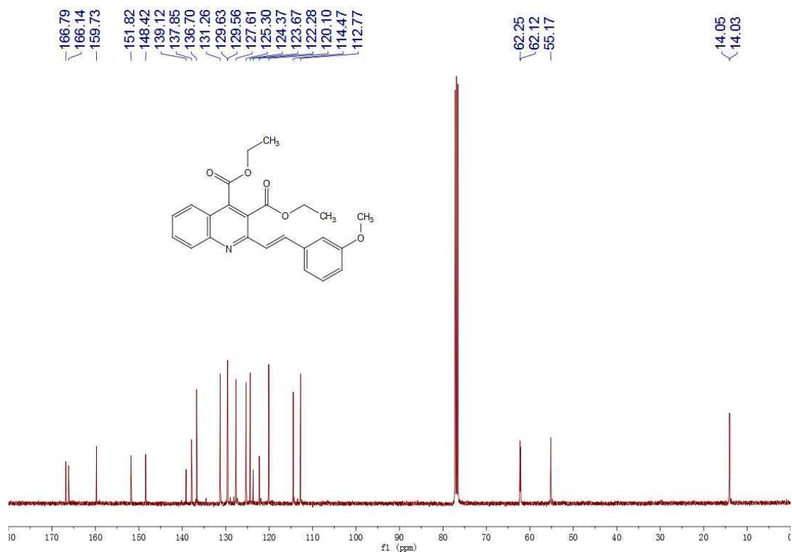
Fig. S14 13 C NMR spectrum of 3g
