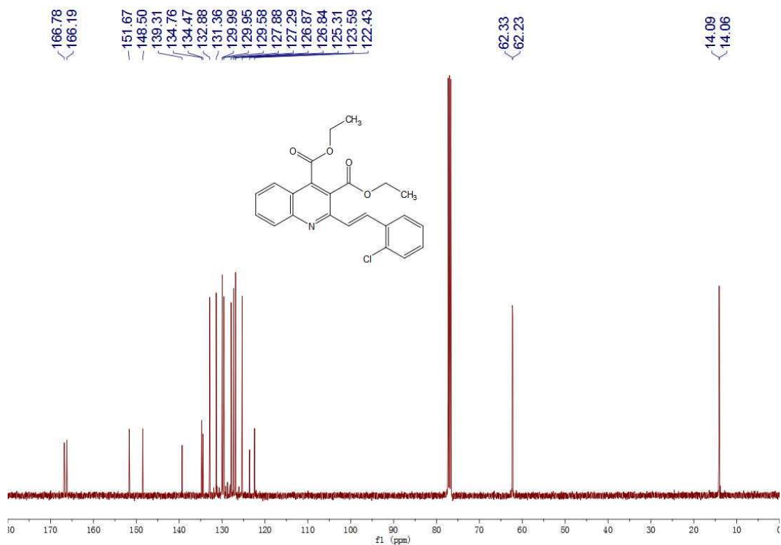
Fig. S24 13 C NMR spectrum of 3I
