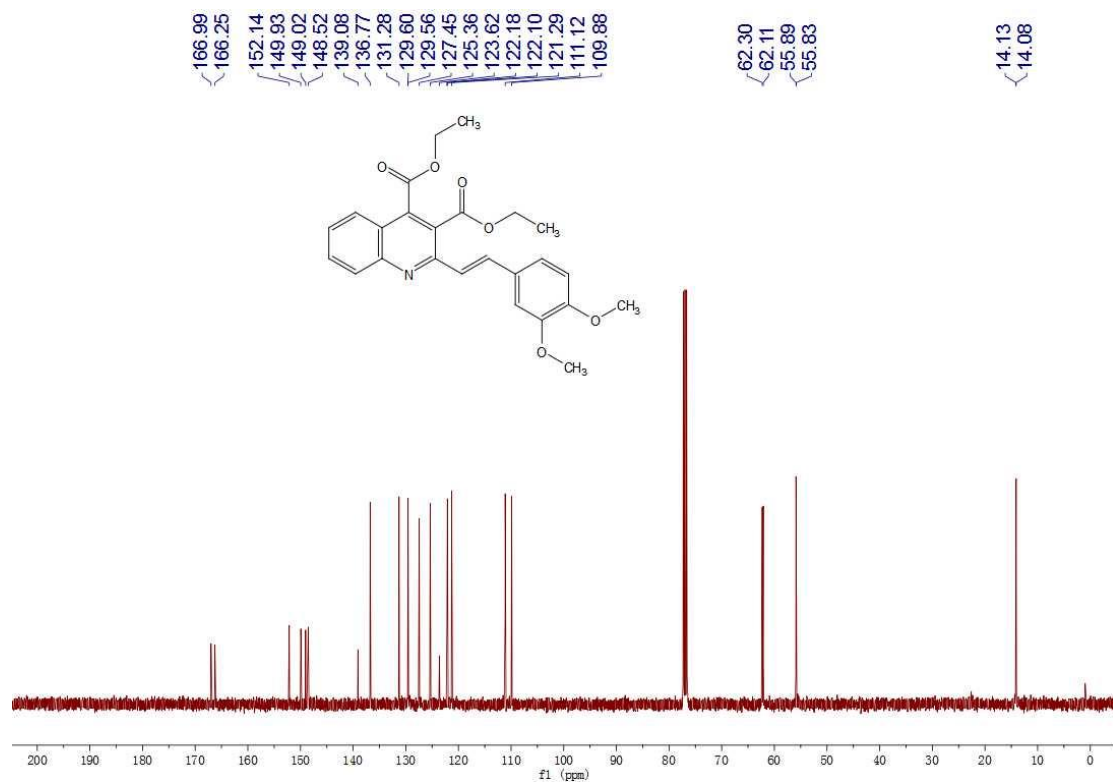
Fig. S20 ^{13}\text{C} NMR spectrum of 3j
