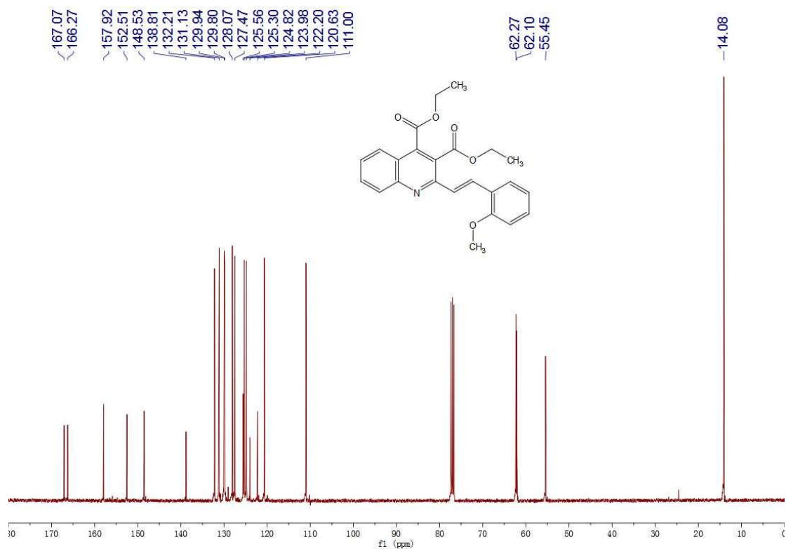
Fig. S12 ^{13}\text{C} NMR spectrum of 3f
