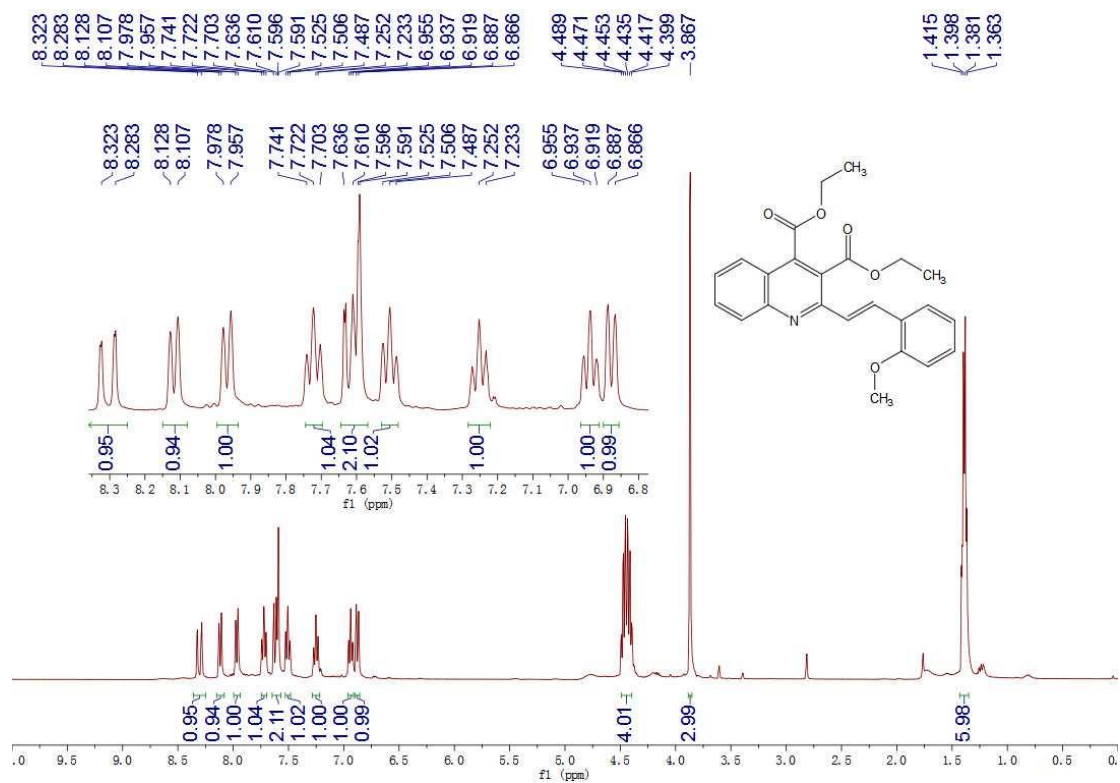
Fig. S11 ^1\text{H} NMR spectrum of 3f
