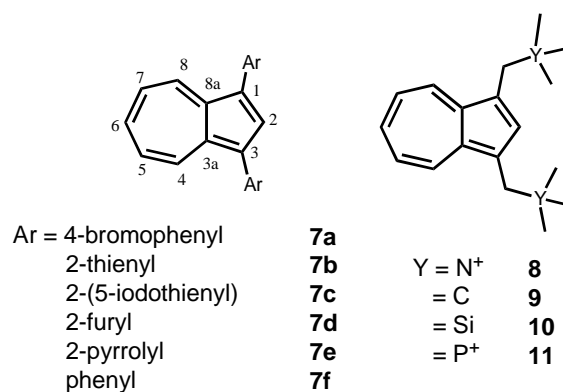
Figure 2. 1,3- Disubstituted azulenes.
