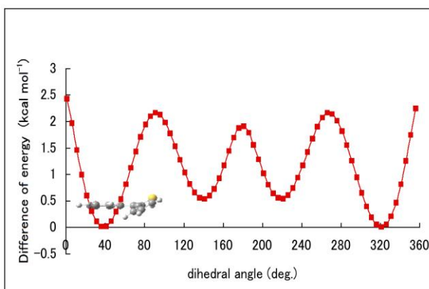
Figure 8. 1-Phenyl- and 1-heterolylazulenes.
