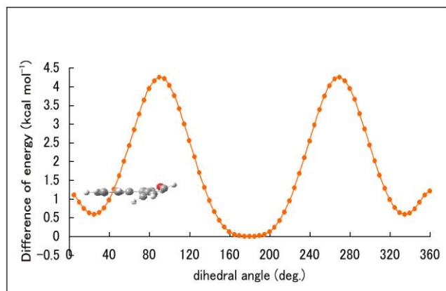
Figure 11. Inter-ring torsional energy profiles for 13c . Figure 12. Inter-ring torsional energy profiles for 13d .
