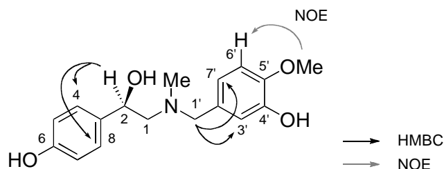
Figure 4. Selected HMBC and NOE correlations of 2
