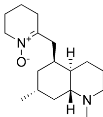
lycoserramine-Y ( 40 ) 51 C_{17}H_{30}N_2O
