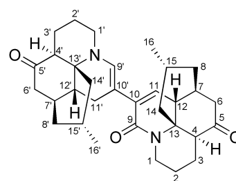
complanadine C ( 50 )
