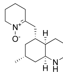
lycoserramine-Z ( 41 ) 51 C_{16}H_{28}N_2O
