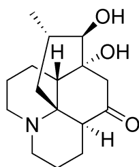
sauroine ( 5 )
