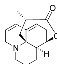
lannotinidine G ( 23 ) 43 C 16 H 21 NO 2
