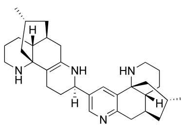
complanadine D ( 51 )
