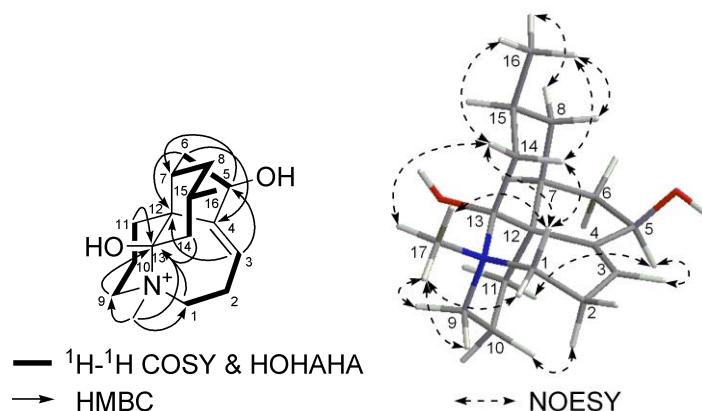
Figure 4. Selected 2D NMR correlations for lycovatine A ( 16 ).
