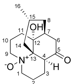
12-epilycodoline N -oxide ( 2 )
