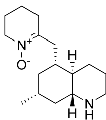
lycoserramine-X ( 39 ) 51 C_{16}H_{28}N_2O
