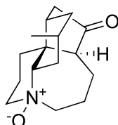
lannotinidine B ( 18 ) 43 C 16 H 25 NO 2
