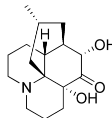
4,6 \alpha -dihydroxylycopodine ( 4 )
