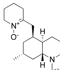
lycoposerramine-Y ( 40 )
