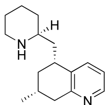
lycoserramine-V ( 37 ) 50 C_{16}H_{24}N_2
