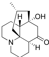
7-hydroxylycopodine ( 3 )
