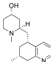
lycoserramine-W ( 38 ) 50 C_{17}H_{26}N_2O
