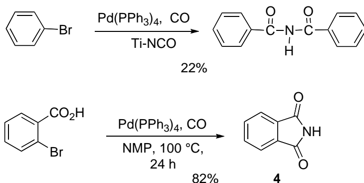
Scheme 3. Reaction of Aryl Halide with 2 under CO in the Presence of Pd(PPh 3 ) 4
