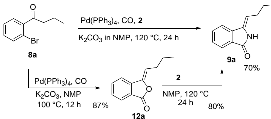
Scheme 5. Synthesis of Isoindolinone Using Pd(PPh 3 ) 4 and 2 under CO
