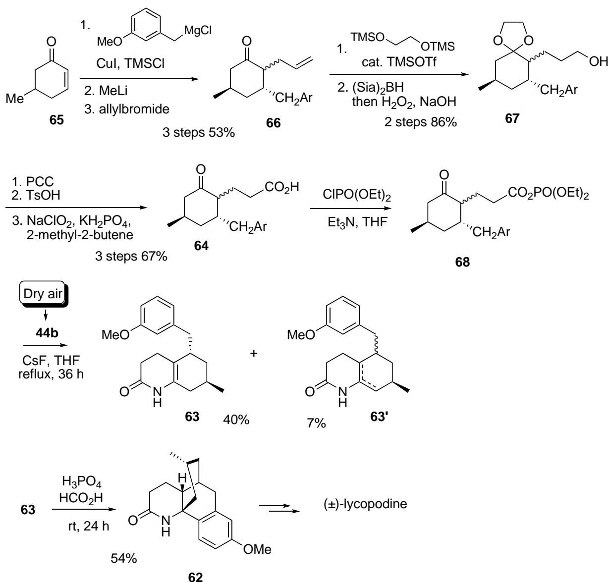
Scheme 22. Formal Total Synthesis of ( \pm )-Lycopodine.
