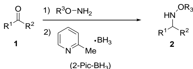
Scheme 1. Synthesis of alkoxyamines by reductive alkoxyamination via oxime ethers
