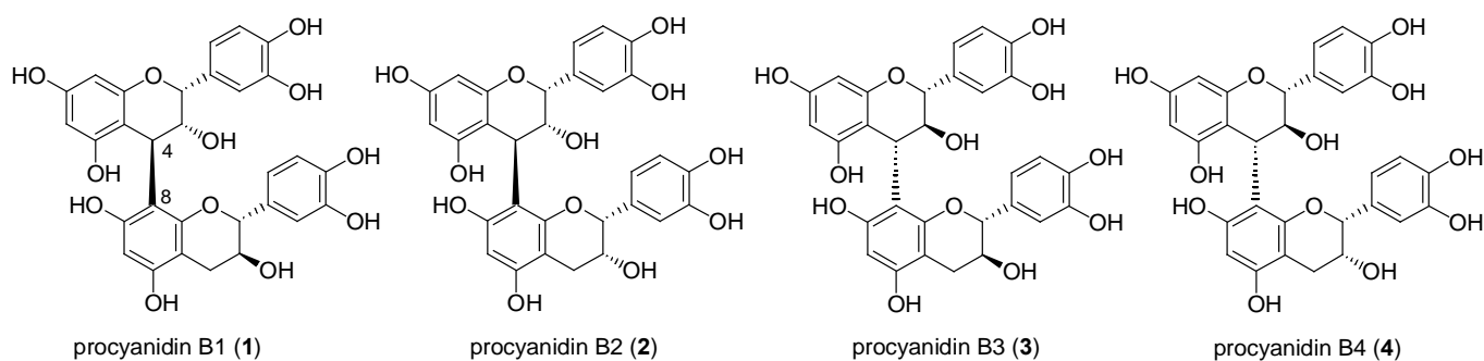
Figure 1. The structures of procyanidin B1-B4 ( 1-4 )
