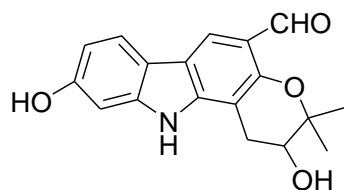
clausine-T ( 81 )
