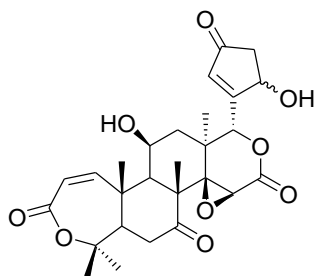
(11 \beta )-21,23-dihydro-11,21-dihydroxy-23-oxoobacunone ( 112 )
