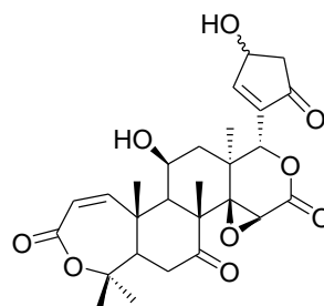
(11 \beta )-21,23-dihydro-11,23-dihydroxy-21-oxoobacunone ( 113 )
