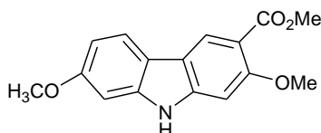
clausine-W ( 84 )
