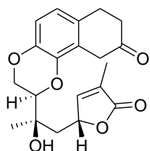
clauslactone-T (24)
