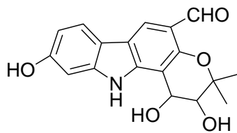
clausine-W ( 84 )
