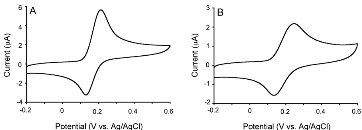
Figure 2. Cyclic voltammograms at 25 ^{\circ}\text{C} of (A) 2 (0.5 mM) and (B) 4 (0.5 mM) in 65 mM phosphate (pH 7.0) with a scanning rate of 0.1 V/s, a gold working electrode, a saturated Ag/AgCl reference electrode, and a platinum wire auxiliary electrode.
