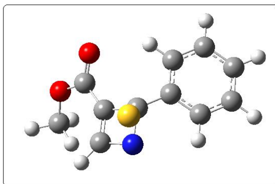
Figure 8. Transition state in the direct conversion 6→9.
