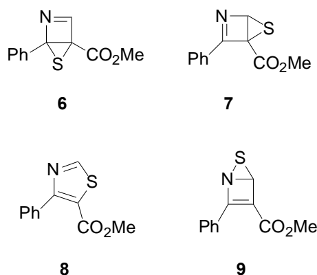
Figure 7. Possible intermediates involved in the reaction 4 → 5.
