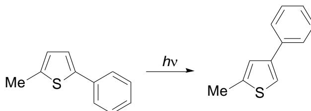
Scheme 3. Photoisomerization of 5-methyl-2-phenylthiophene.
